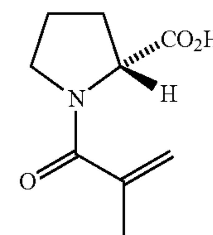
(2R)-1-Methacryloylpyrrolidin-2-carboxylic Acid
