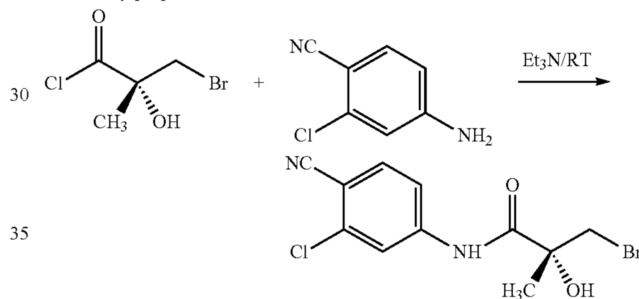
(R)-3-bromo-2-hydroxy-2-methylpropanoic acid
