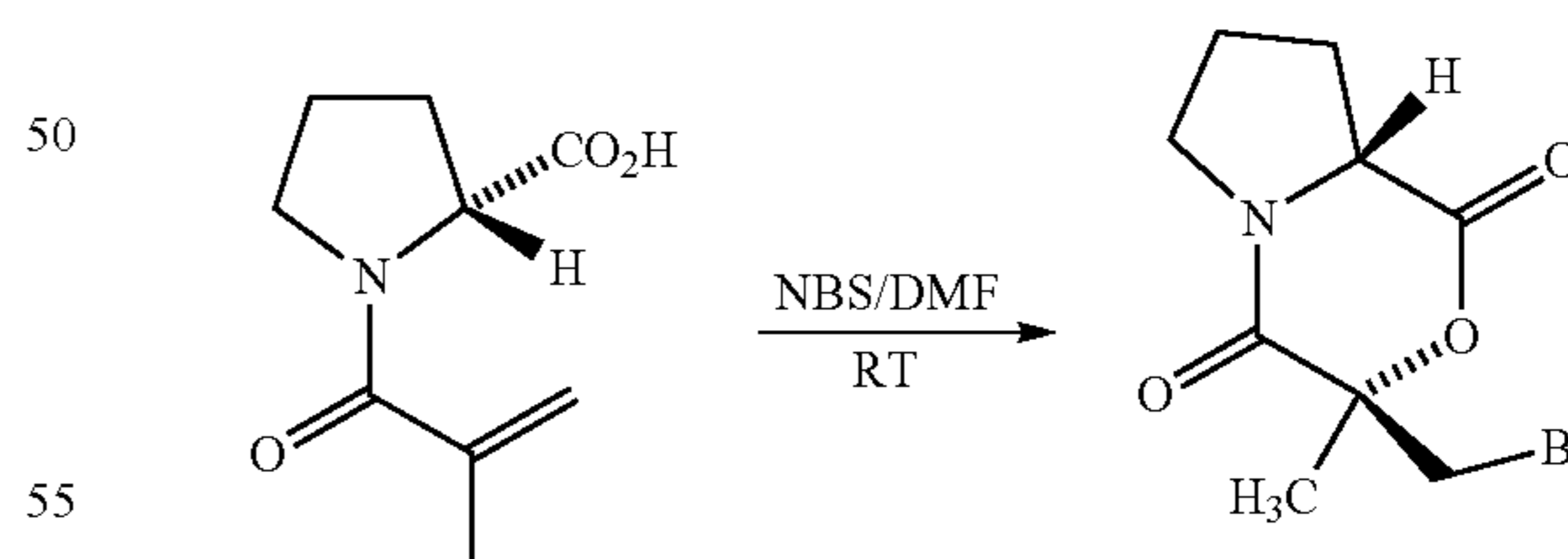
(3R,8aR)-3-Bromomethyl-3-methyl-tetrahydro-pyrrolo[2,1-c][1,4]oxazine-1,4-dione
