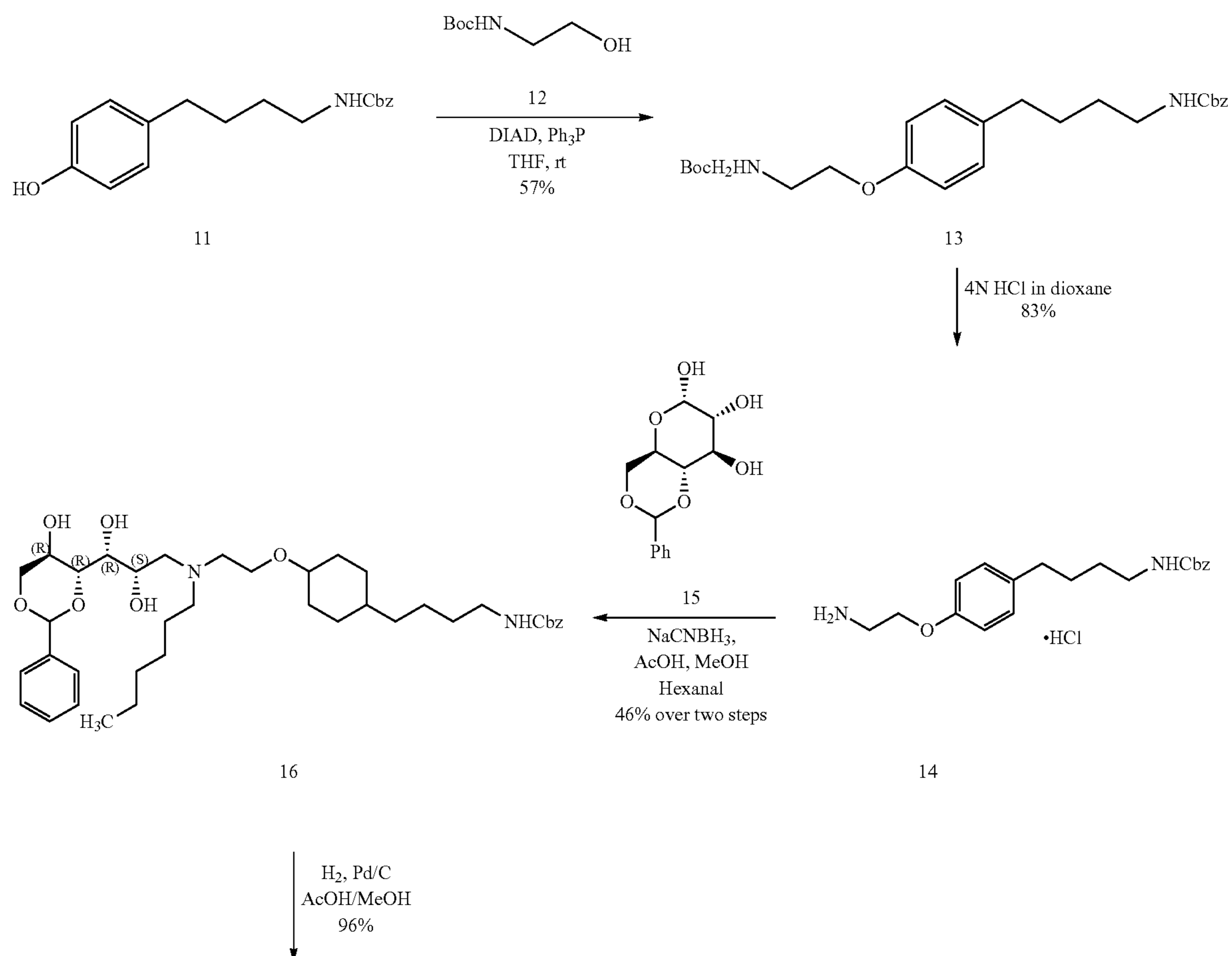
Scheme 2. Preparation of 3,5-Diamino-6-chloro-N-(N-(4-(4-(2-(hexyl((2S,3R,4R,5R)-2,3,4,5,6-pentahydroxyhexyl)amino)ethoxy)phenyl)butyl)carbamimidoyl)pyrazine-2-carboxamide
