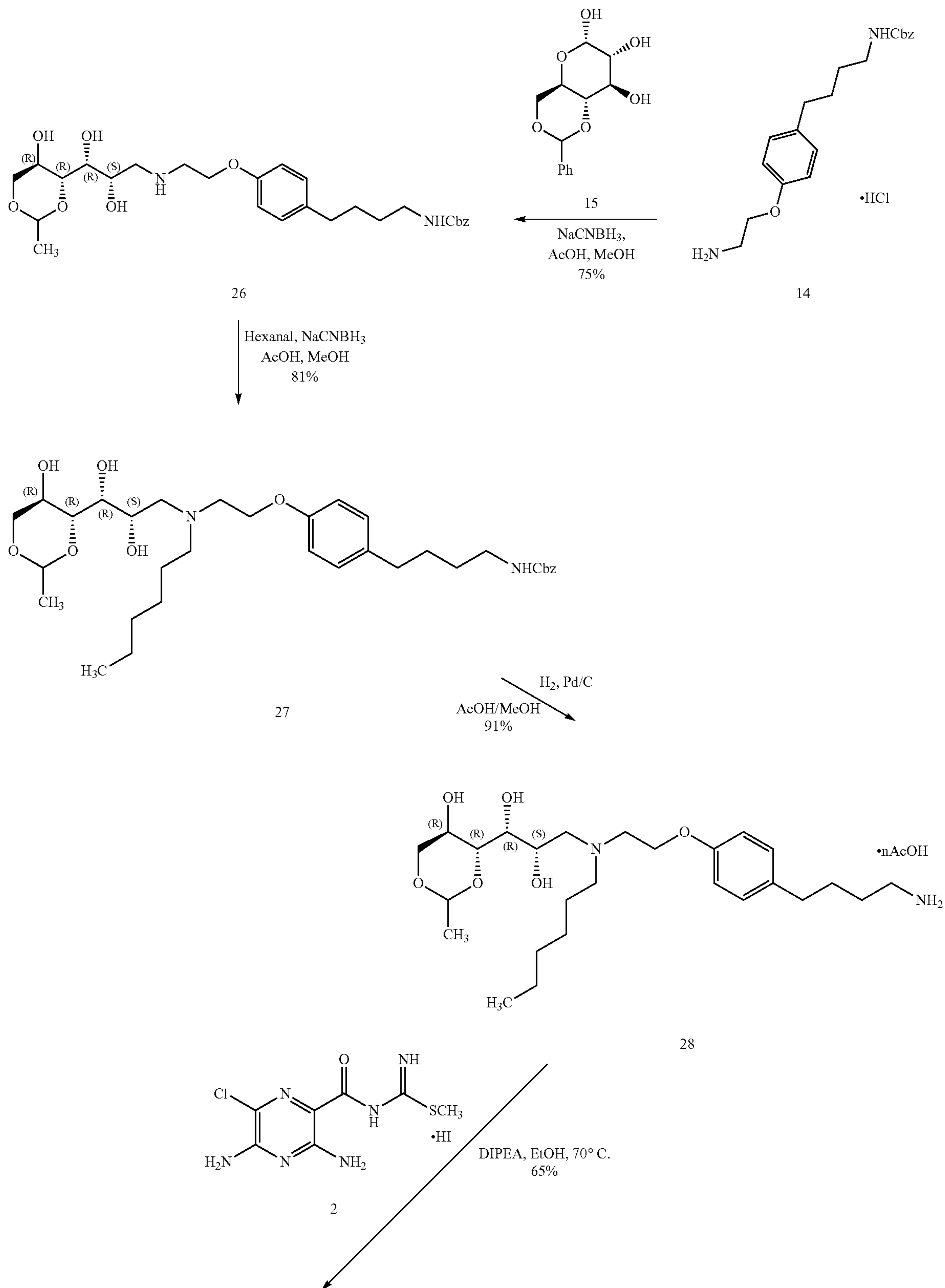
Scheme 3. Alternate Preparation of 3,5-Diamino-6-chloro-N-(N-(4-(4-(2-(hexyl((2S,3R,4R,5R)-2,3,4,5,6-pentahydroxyhexyl)amino)ethoxy)phenyl)butyl)carbamimidoyl)pyrazine-2-carboxamide
