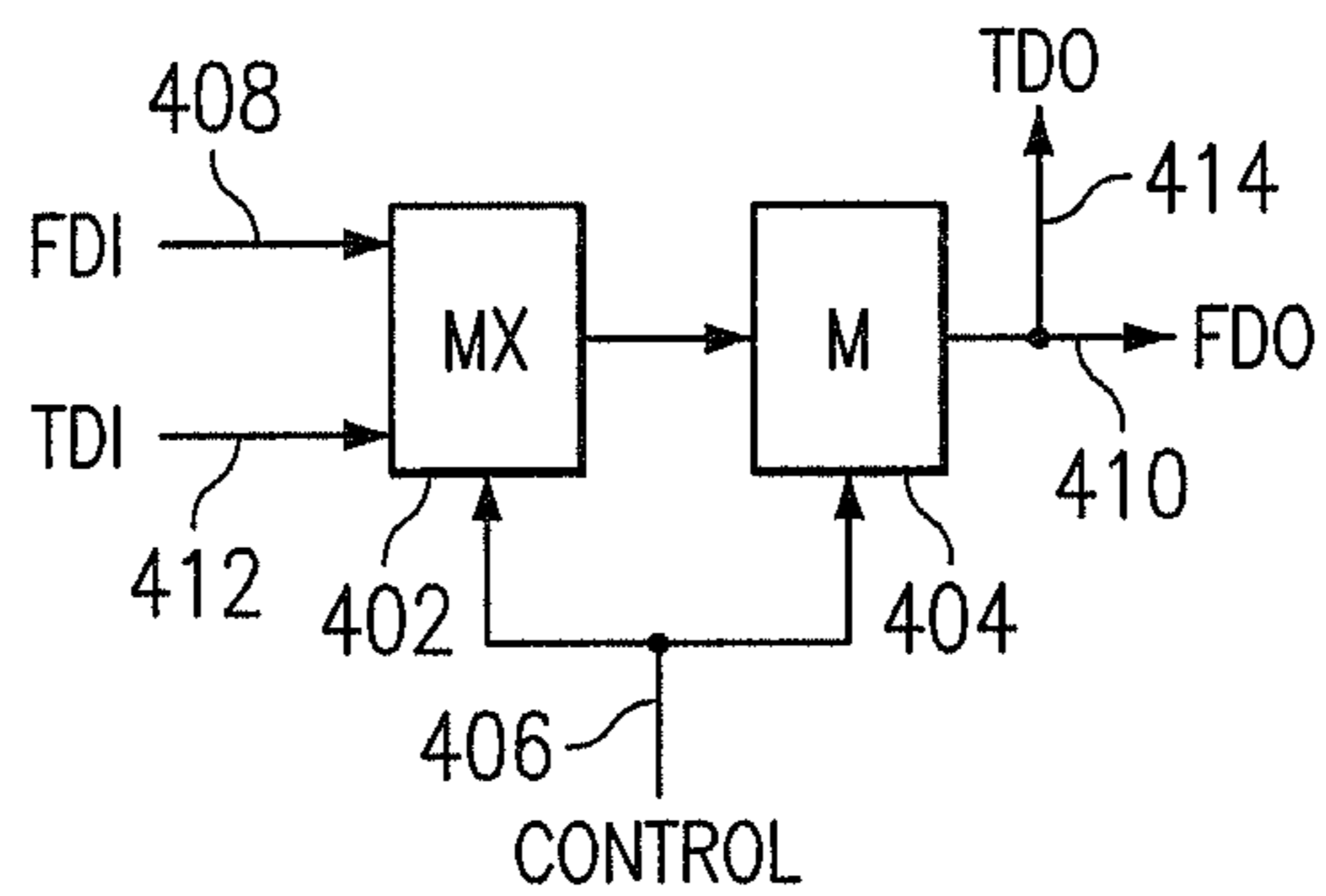
FIG. 4 (PRIOR ART)
