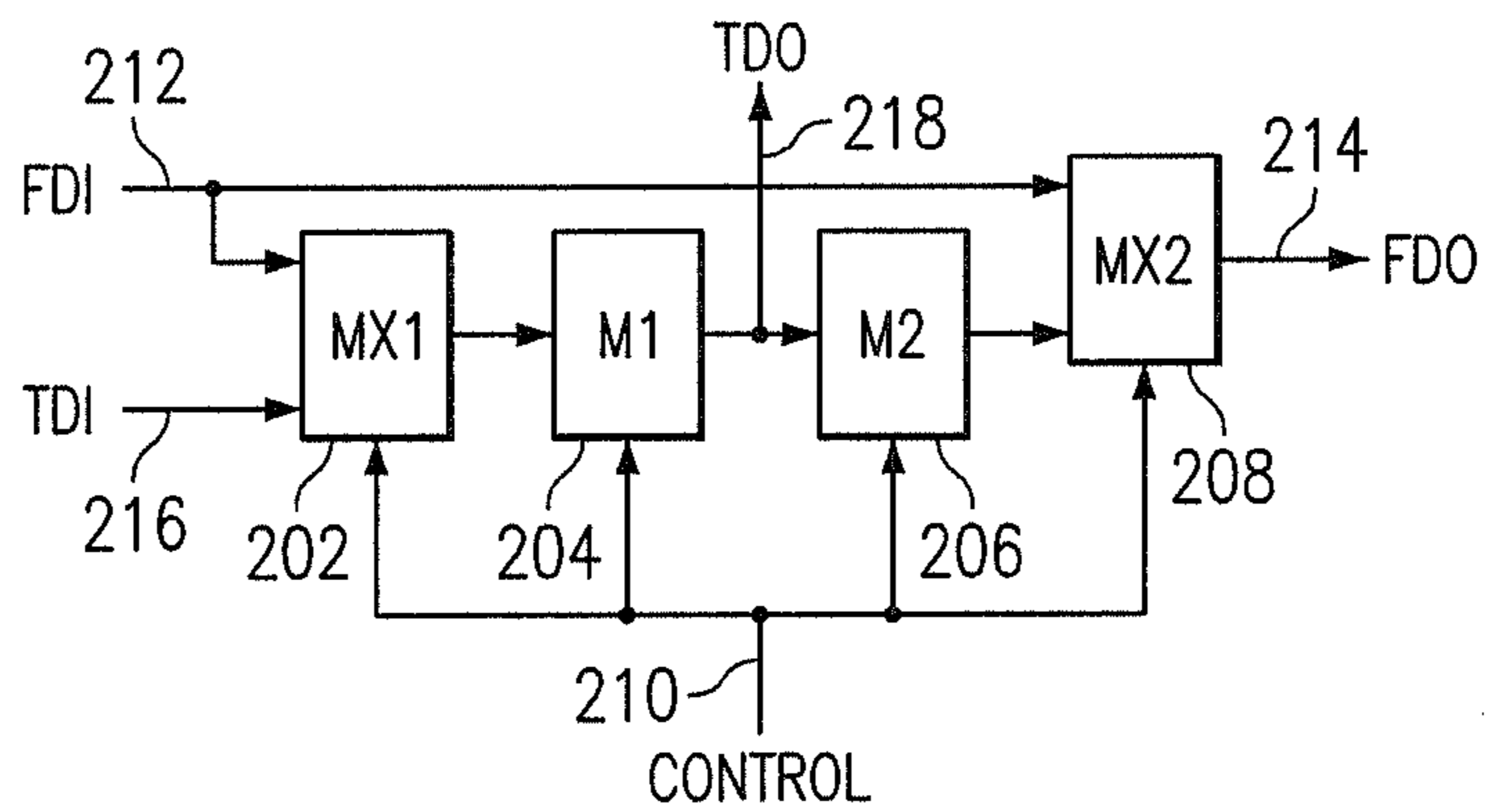
FIG. 2 (PRIOR ART)
