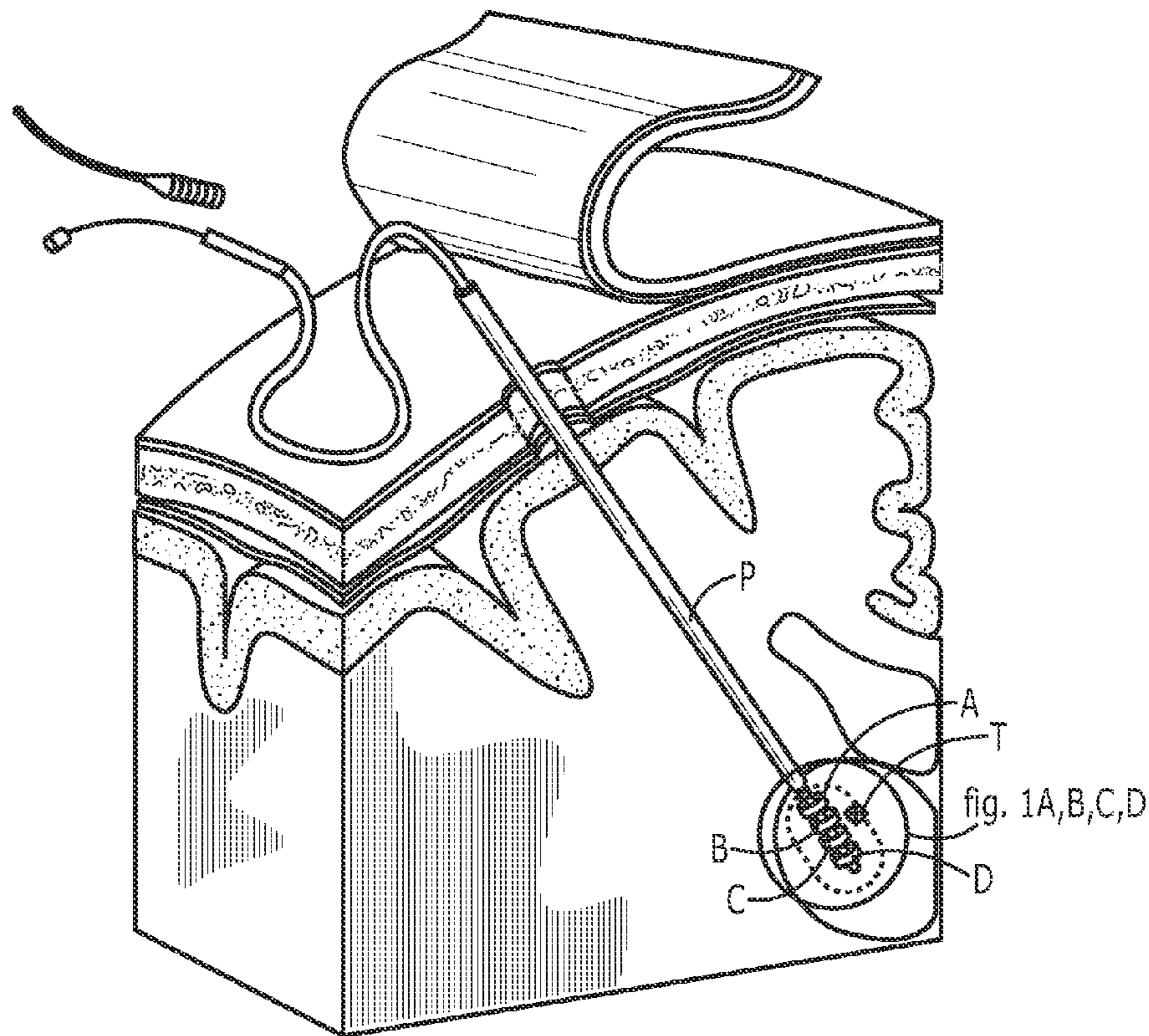
FIG. 1 (PRIOR ART)
