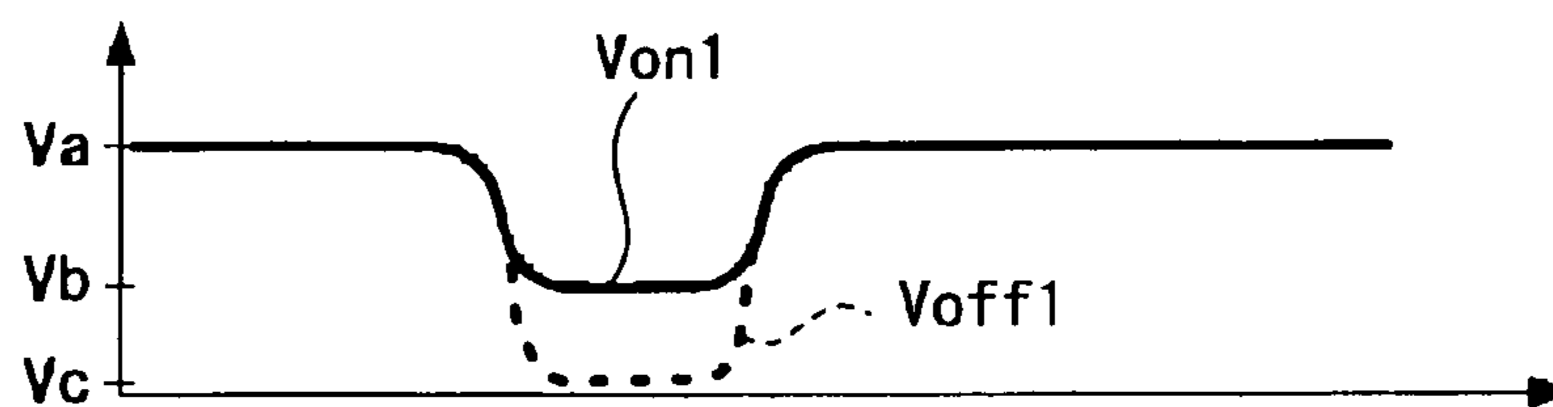
FIG. 8B Light-Receiving Output Voltage
