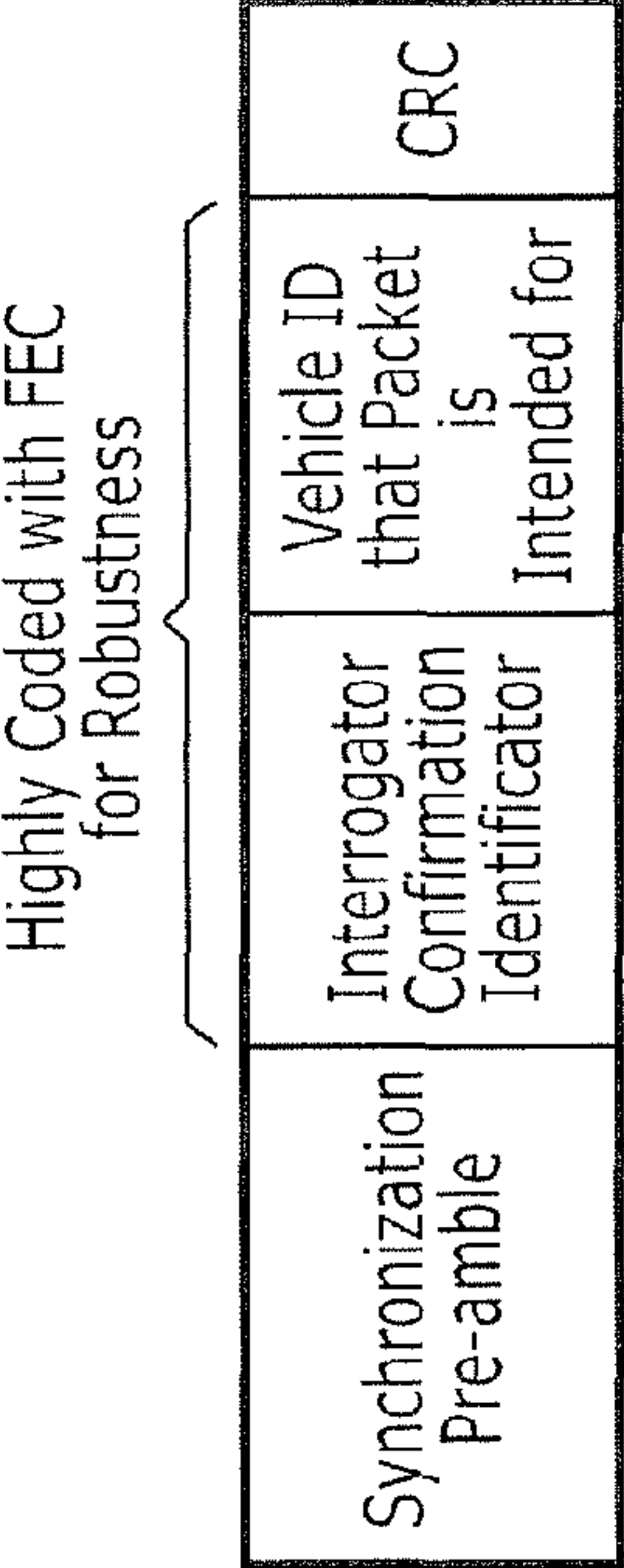
Illustrative Confirmation Packet Sent to Transponder by Interrogator. FIG. 4
