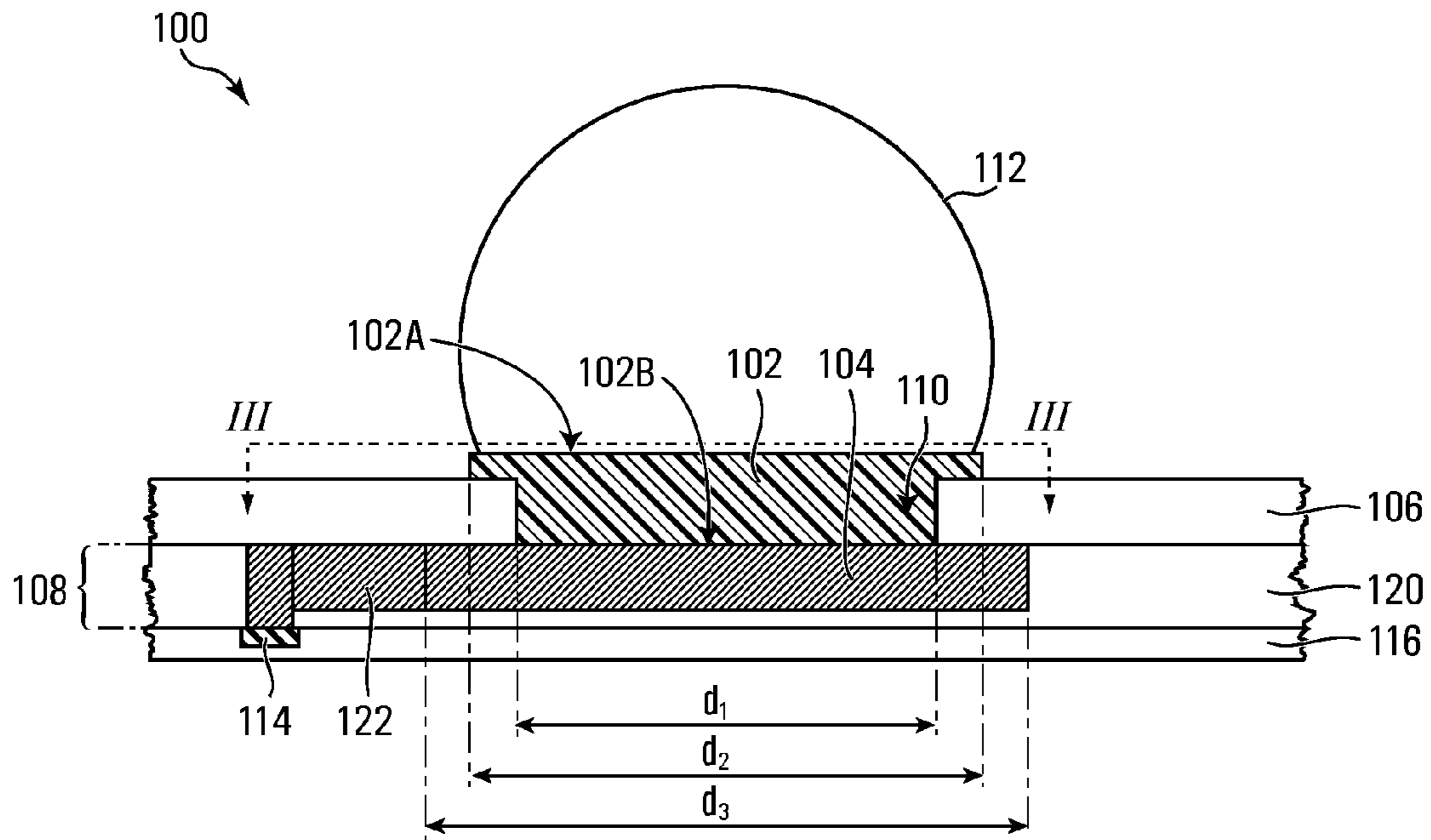
FIG. 2 Prior Art
