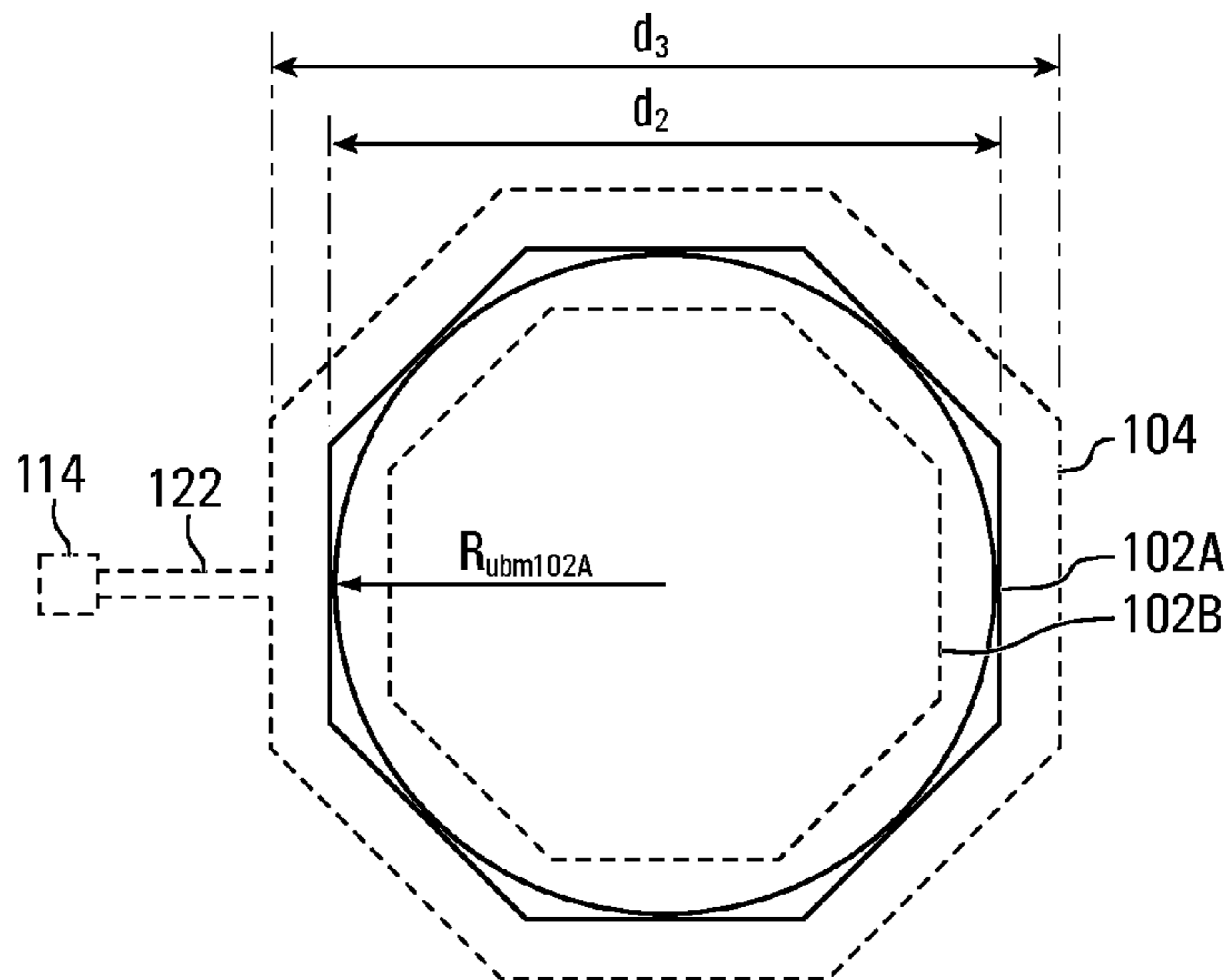
FIG. 3 Prior Art
