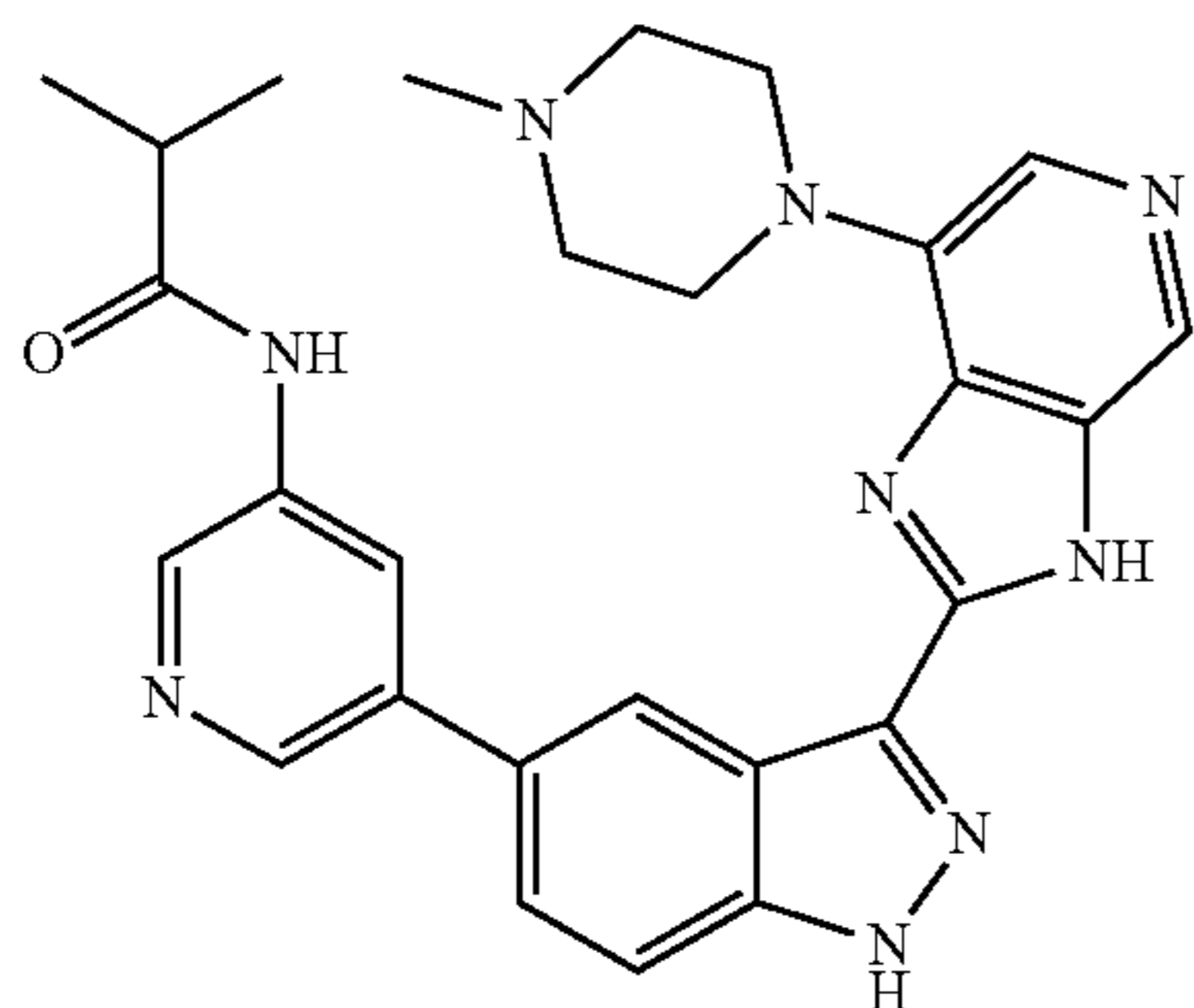
N-(5-(3-(7-(4-methylpiperazin-1-yl)-3H-imidazo[4,5-c]pyridin-2-yl)-1H-indazol-5-yl)pyridin-3-yl)isobutyramide 2
