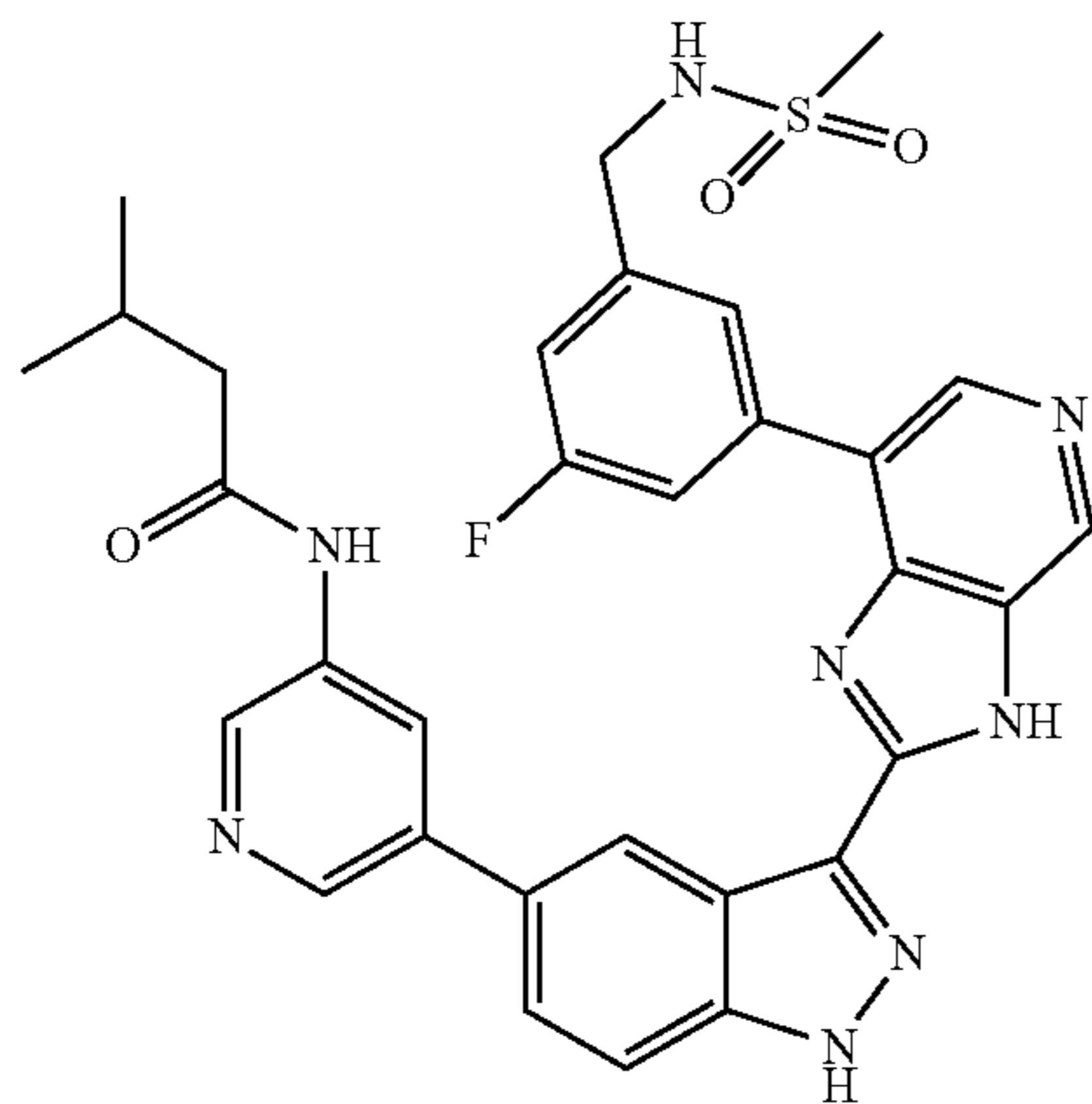
N-(5-(3-(7-(3-Fluoro-5-(methylsulfonamidomethyl)phenyl)-3H-imidazo[4,5-c]pyridin-2-yl)-1H-indazol-5-yl)pyridin-3-yl)-3-methylbutanamide 373
