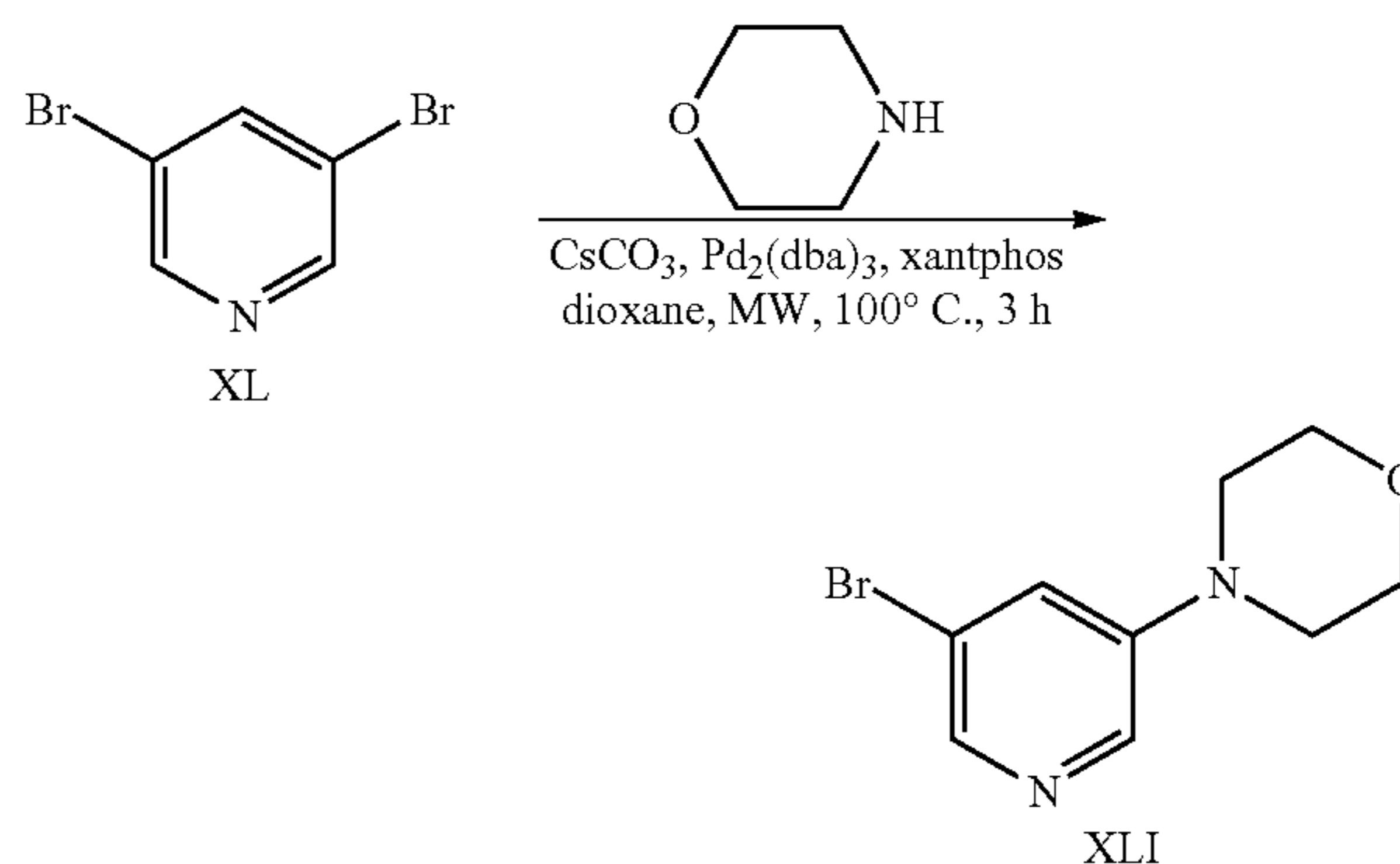
Scheme 7
