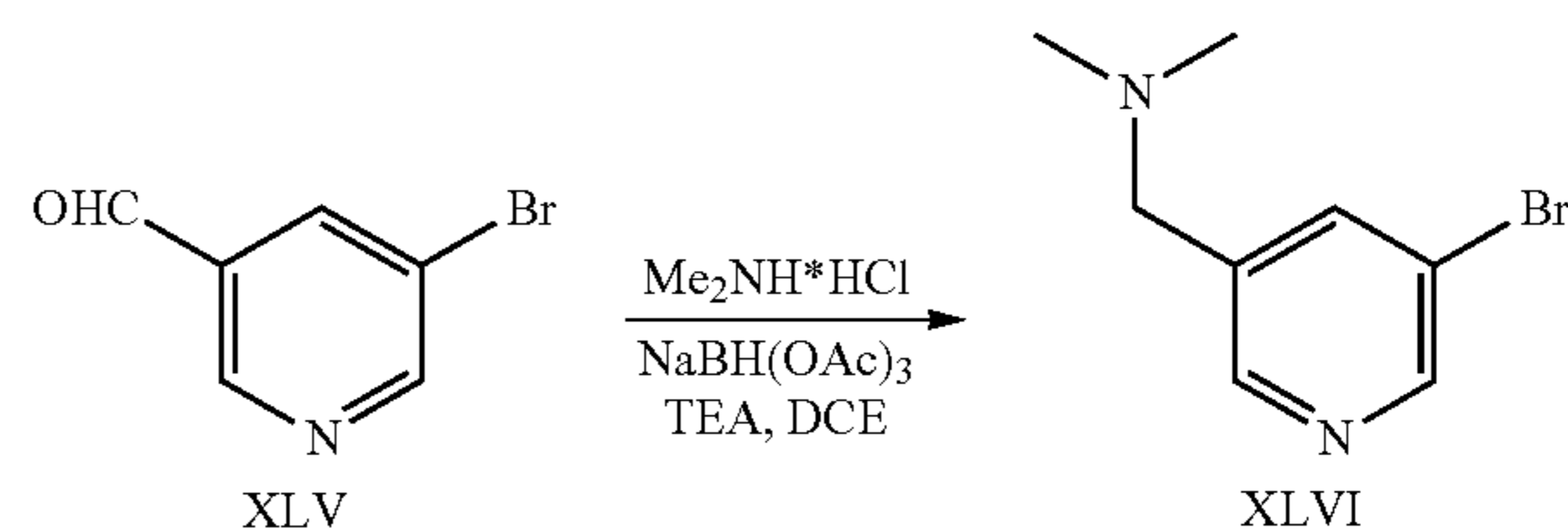
Scheme 10
