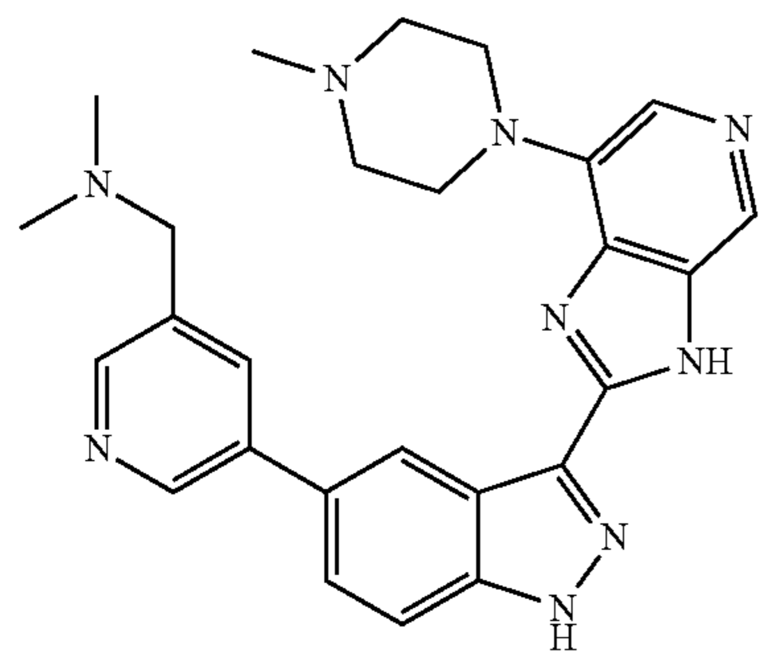
N,N-dimethyl-1-(5-(3-(7-(4-methylpiperazin-1-yl)-3H-imidazo[4,5-c]pyridin-2-yl)-1H-indazol-5-yl)pyridin-3-yl)methanamine 3
