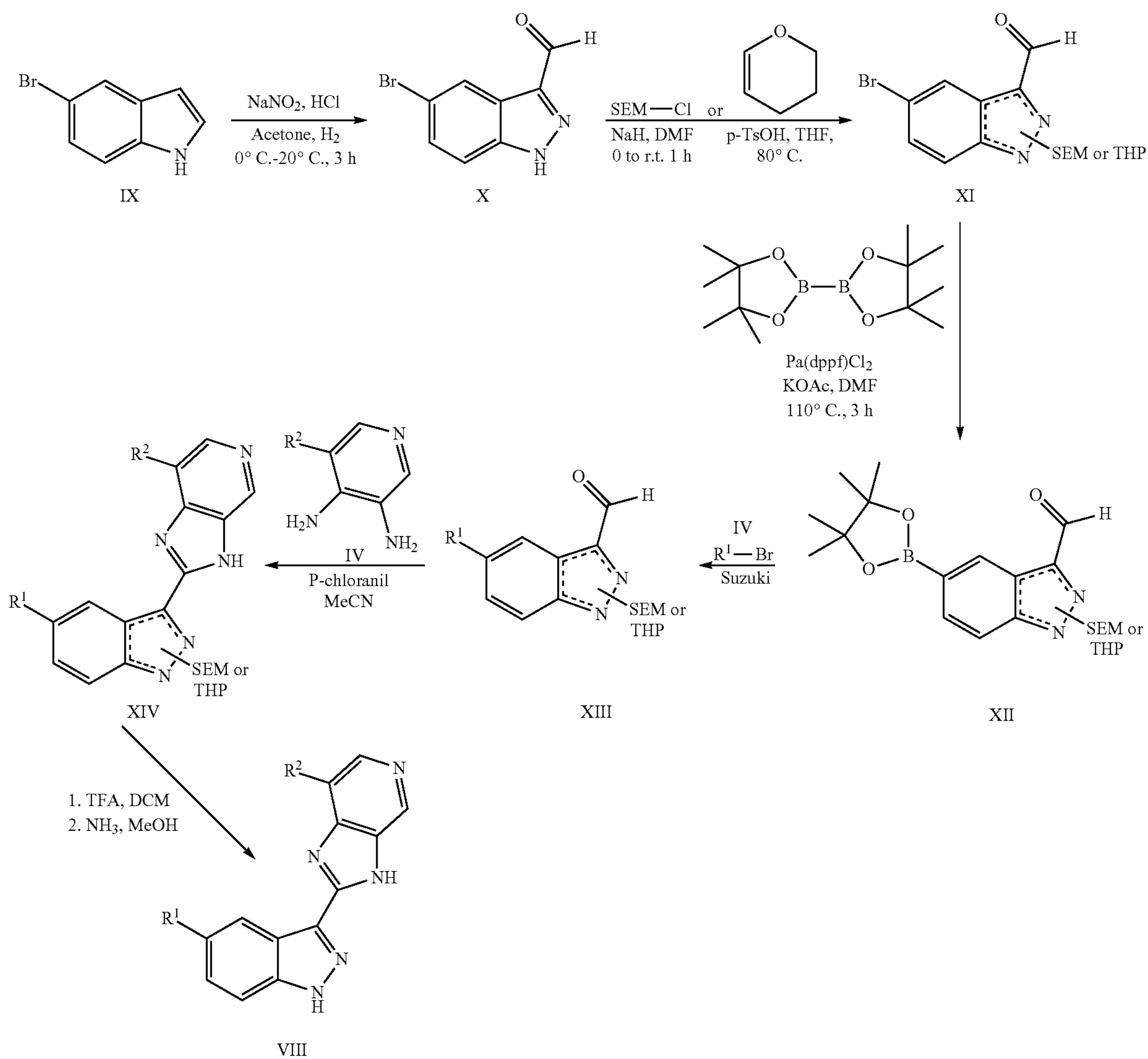
Scheme 2
