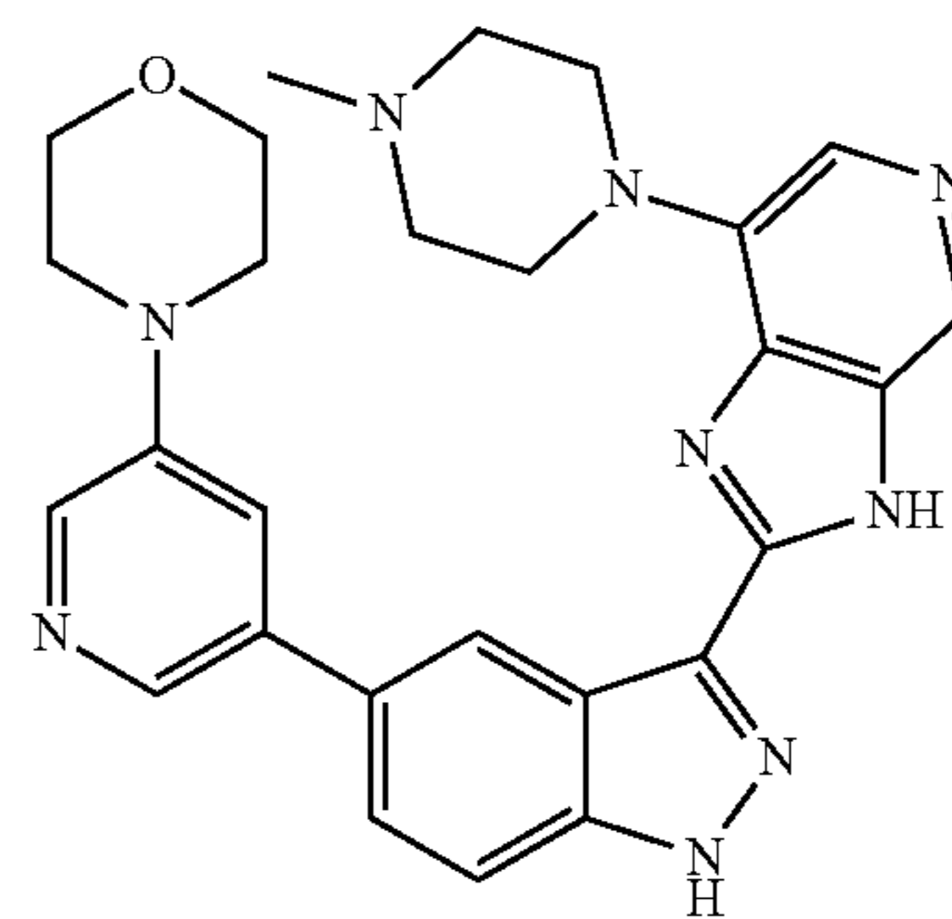
4-(5-(3-(7-(4-methylpiperazin-1-yl)-3H-imidazo[4,5-c]pyridin-2-yl)-1H-indazol-5-yl)pyridin-3-yl)morpholine 5
