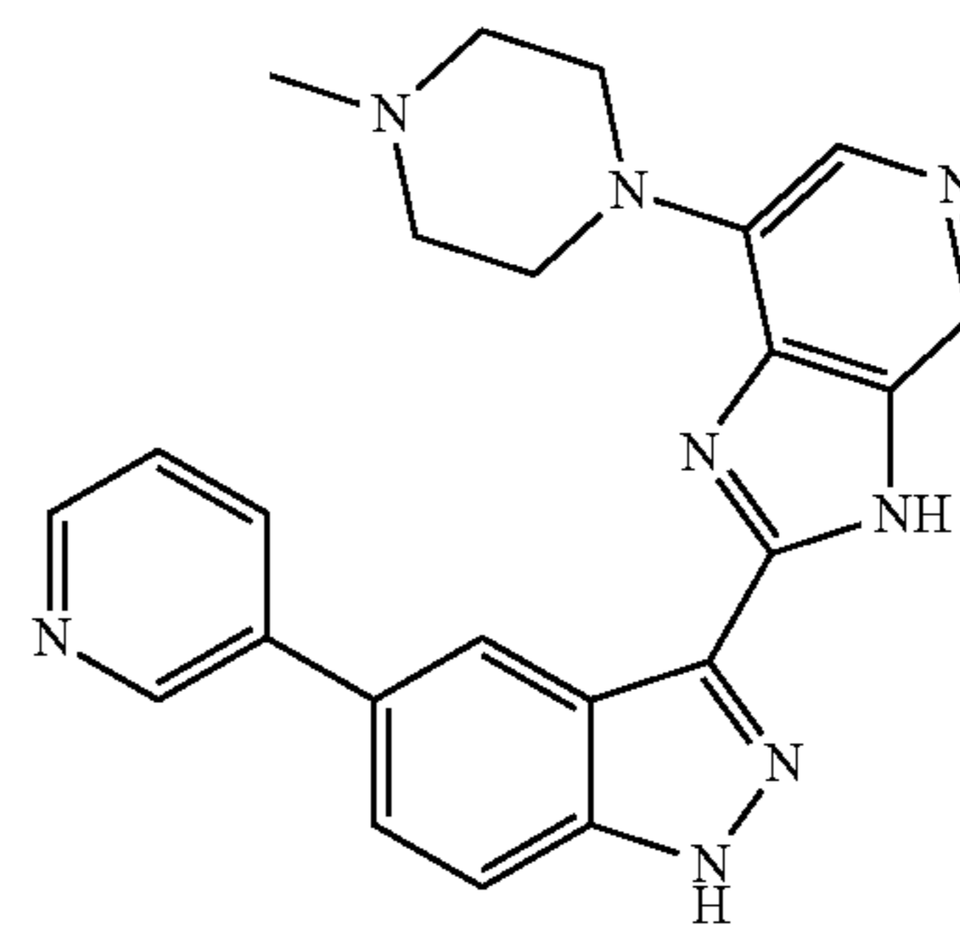
7-(4-methylpiperazin-1-yl)-2-(5-(pyridin-3-yl)-1H-indazol-3-yl)-3H-imidazo[4,5-c]pyridine 4
