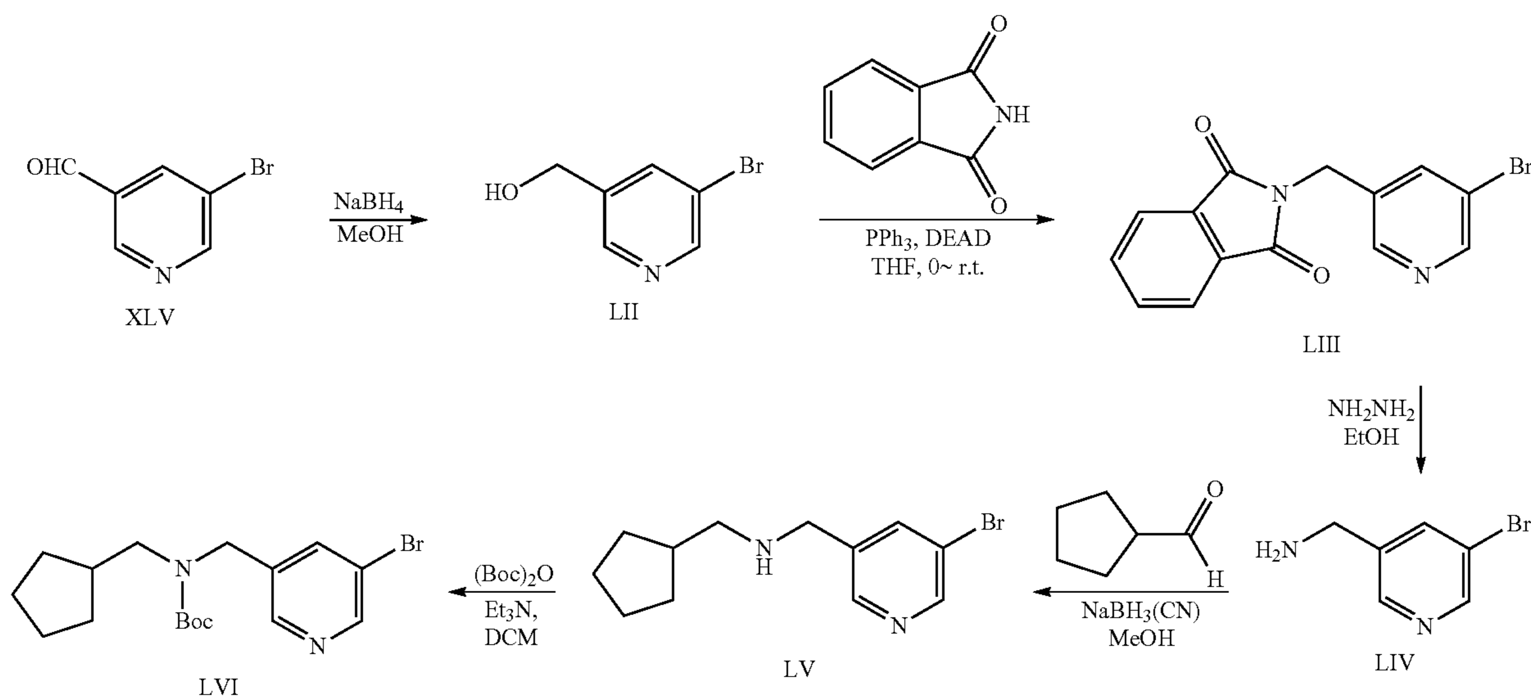
Scheme 11
