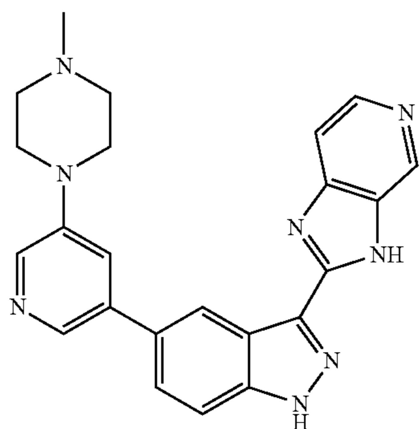
2-(5-(5-(4-methylpiperazin-1-yl)pyridin-3-yl)-1H-indazol-3-yl)-3H-imidazo[4,5-c]pyridine 7
