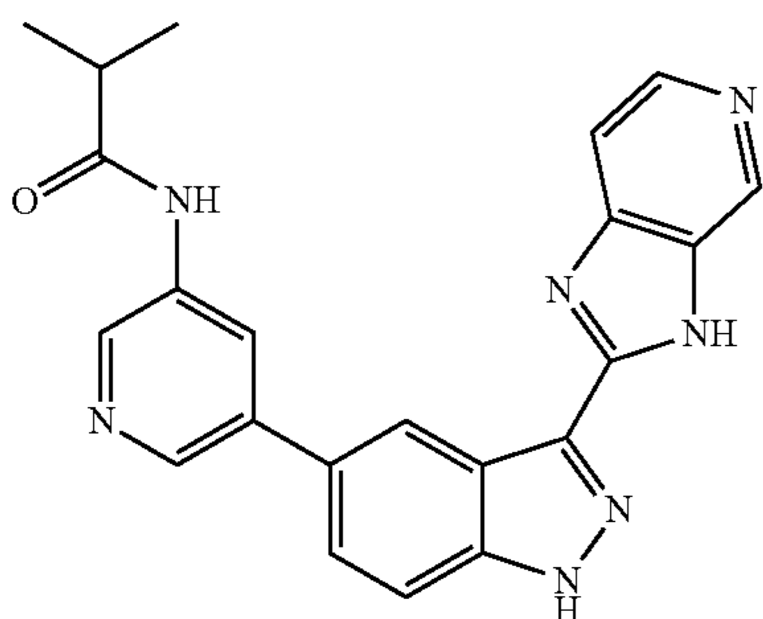
N-(5-(3-(3H-imidazo[4,5-c]pyridin-2-yl)-1H-indazol-5-yl)pyridin-3-yl)isobutyramide 9
