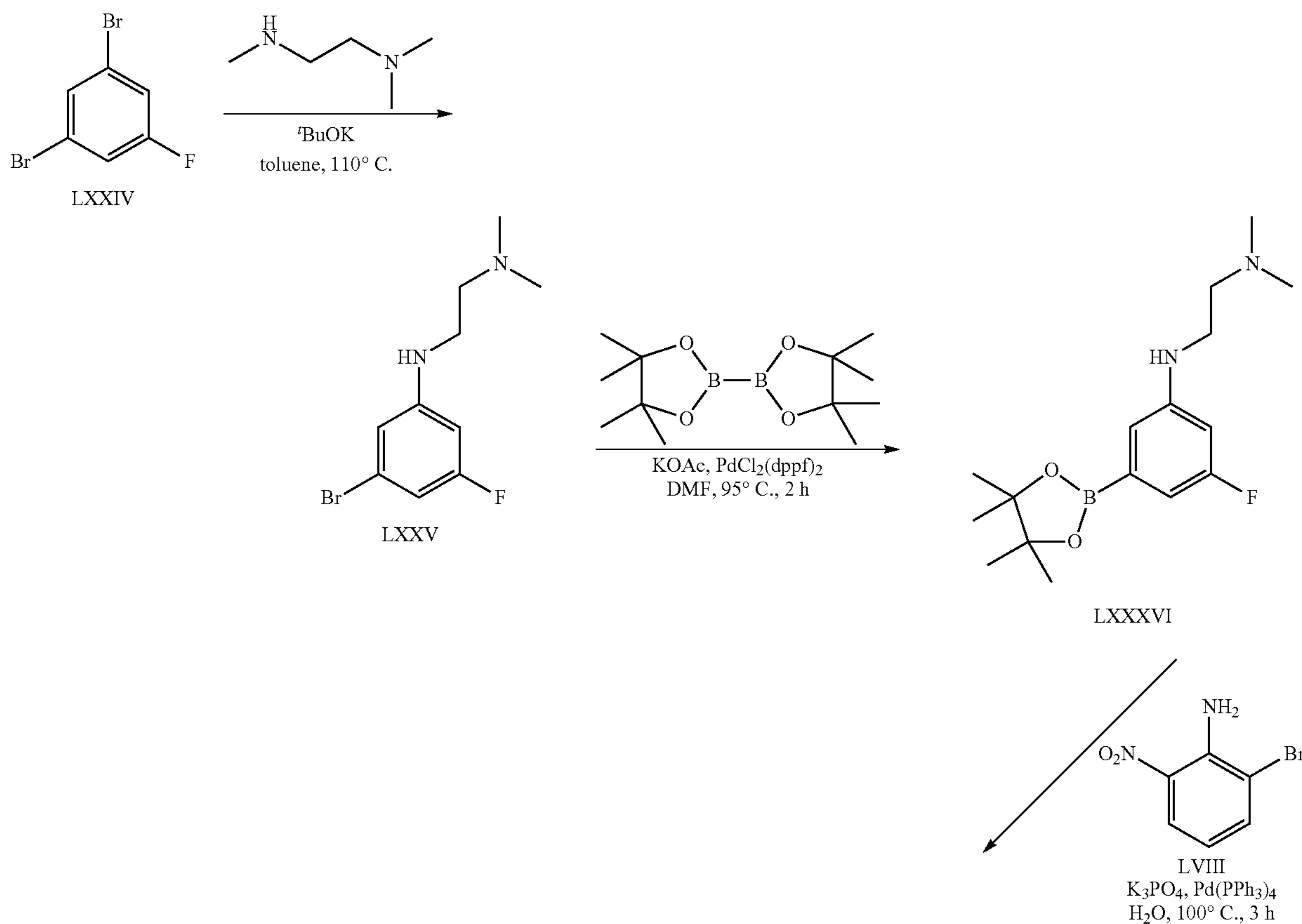
Scheme 14
