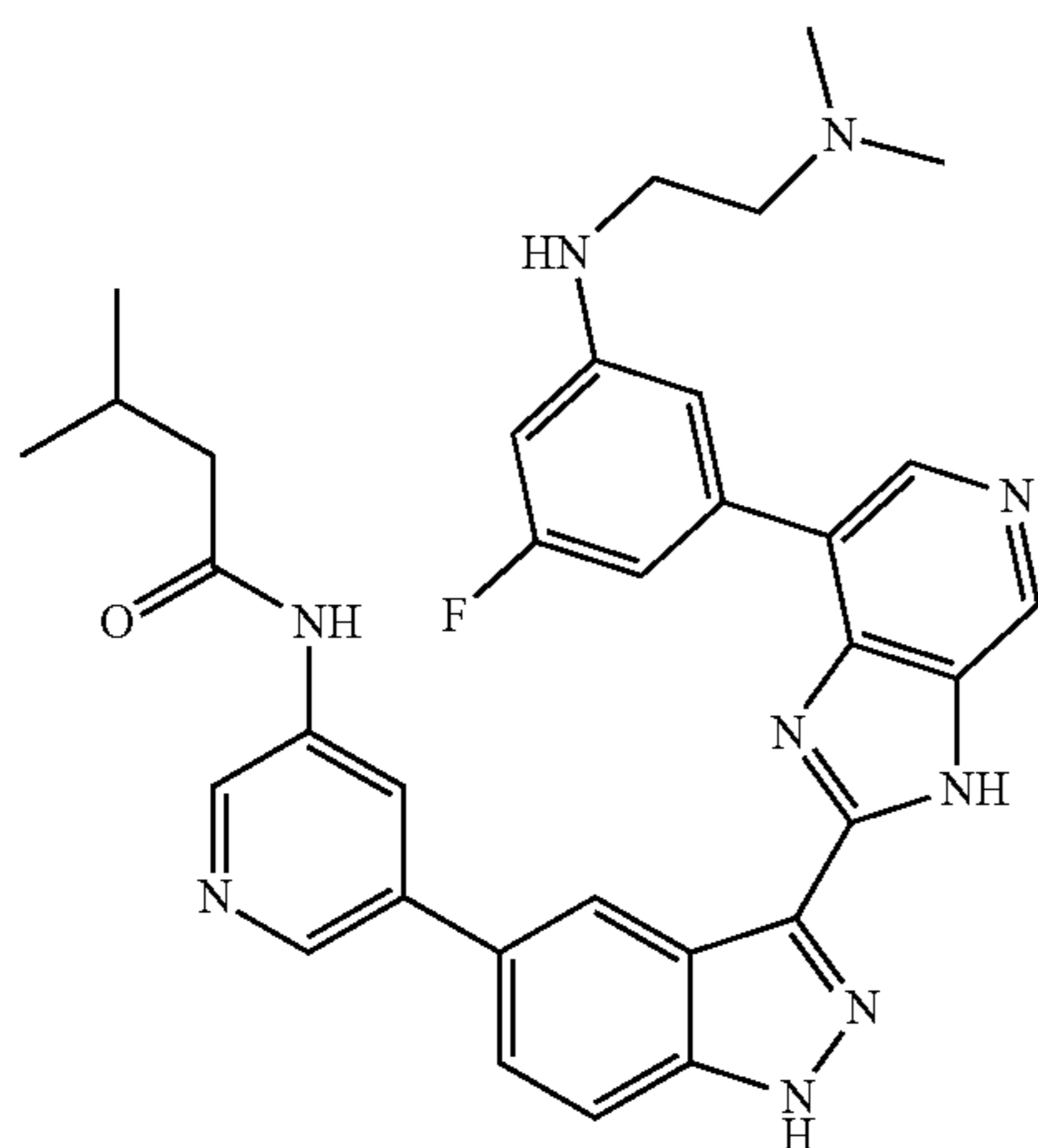
N-(5-(3-(7-(3-(2-(Dimethylamino)ethylamino)-5-fluorophenyl)-3H-imidazo[4,5-c]pyridin-2-yl)-1H-indazol-5-yl)pyridin-3-yl)-3-methylbutanamide 349
