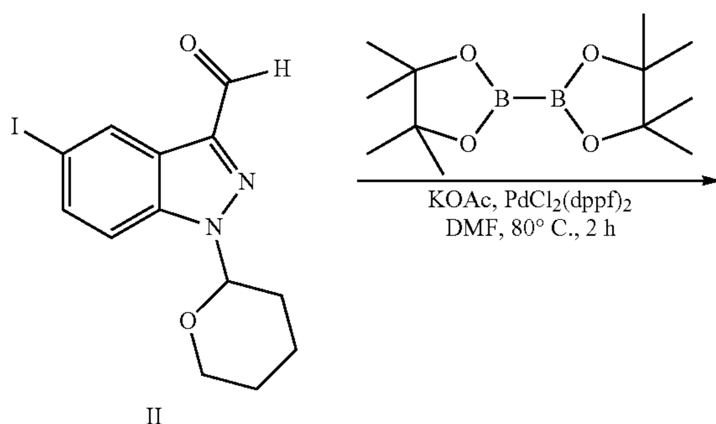
Scheme 16
