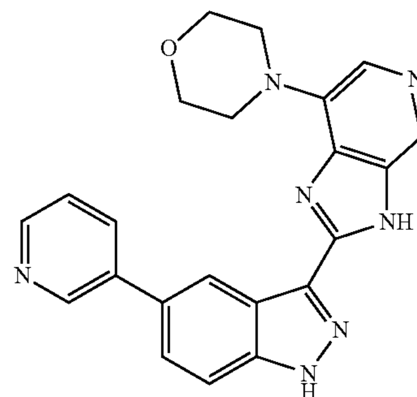
4-(2-(5-(pyridin-3-yl)-1H-indazol-3-yl)-3H-imidazo[4,5-c]pyridin-7-yl)morpholine 6
