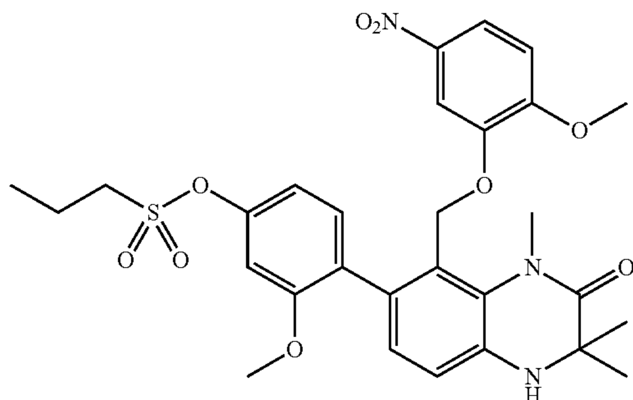
8-(2-Methoxy-5-nitrophenoxy-methyl)-7-(2-methoxy-4-propylsulfonyloxyphenyl)-1,3,3-trimethyl-3,4-dihydro-1H-quinoxalin-2-one (Compound No. 1-31)
