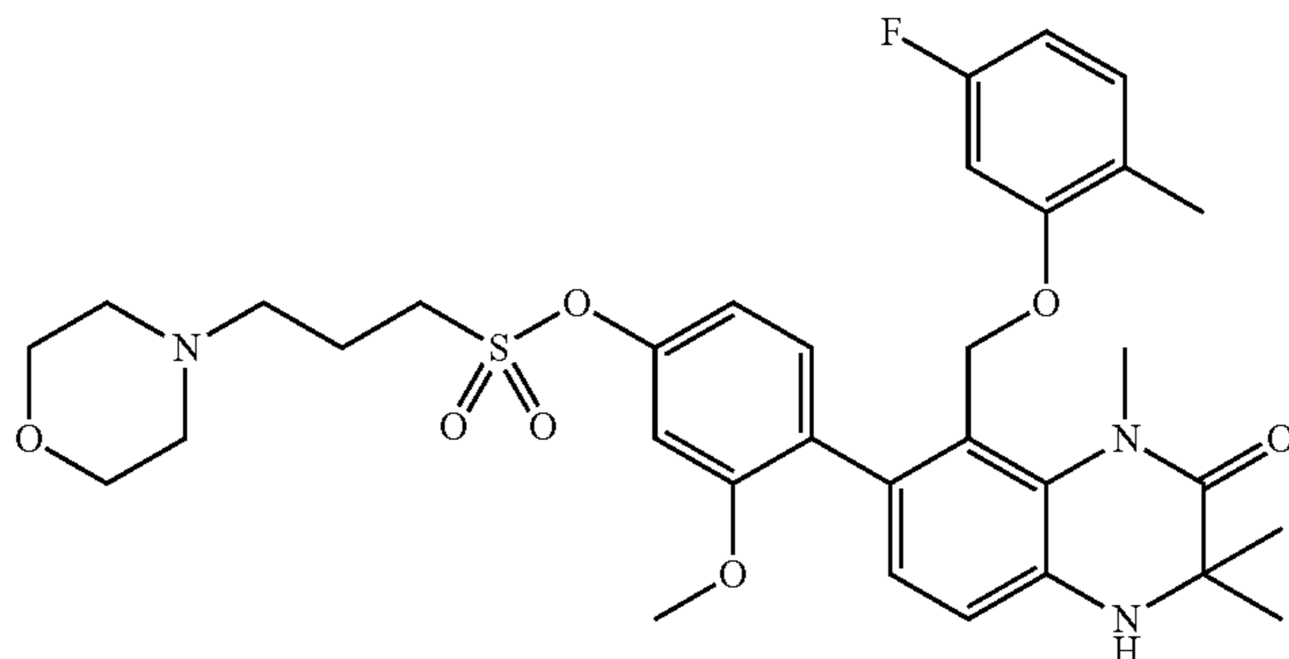
8-(5-Fluoro-2-methylphenoxy)methyl-7-[2-methoxy-4-[3-(morpholin-4-yl)propylsulfonyloxy]phenyl]-1,3,3-trimethyl-3,4-dihydro-1H-quinoxalin-2-one (Compound No. 3-3)
