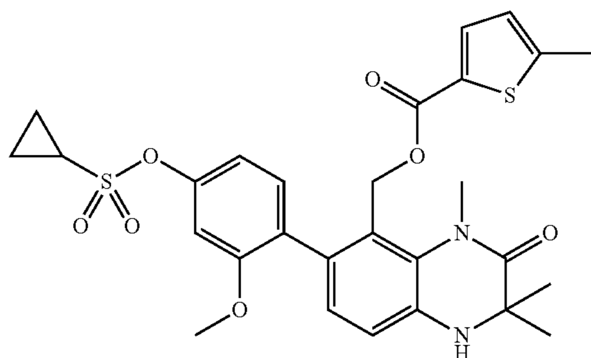
7-[2-Methoxy-4-(3,3,3-trifluoropropylsulfonyloxy)phenyl]-8-(5-methylthiophen-2-ylcarbonyloxymethyl)-1,3,3-trimethyl-3,4-dihydro-1H-quinoxalin-2-one (Compound No. 1-20)
