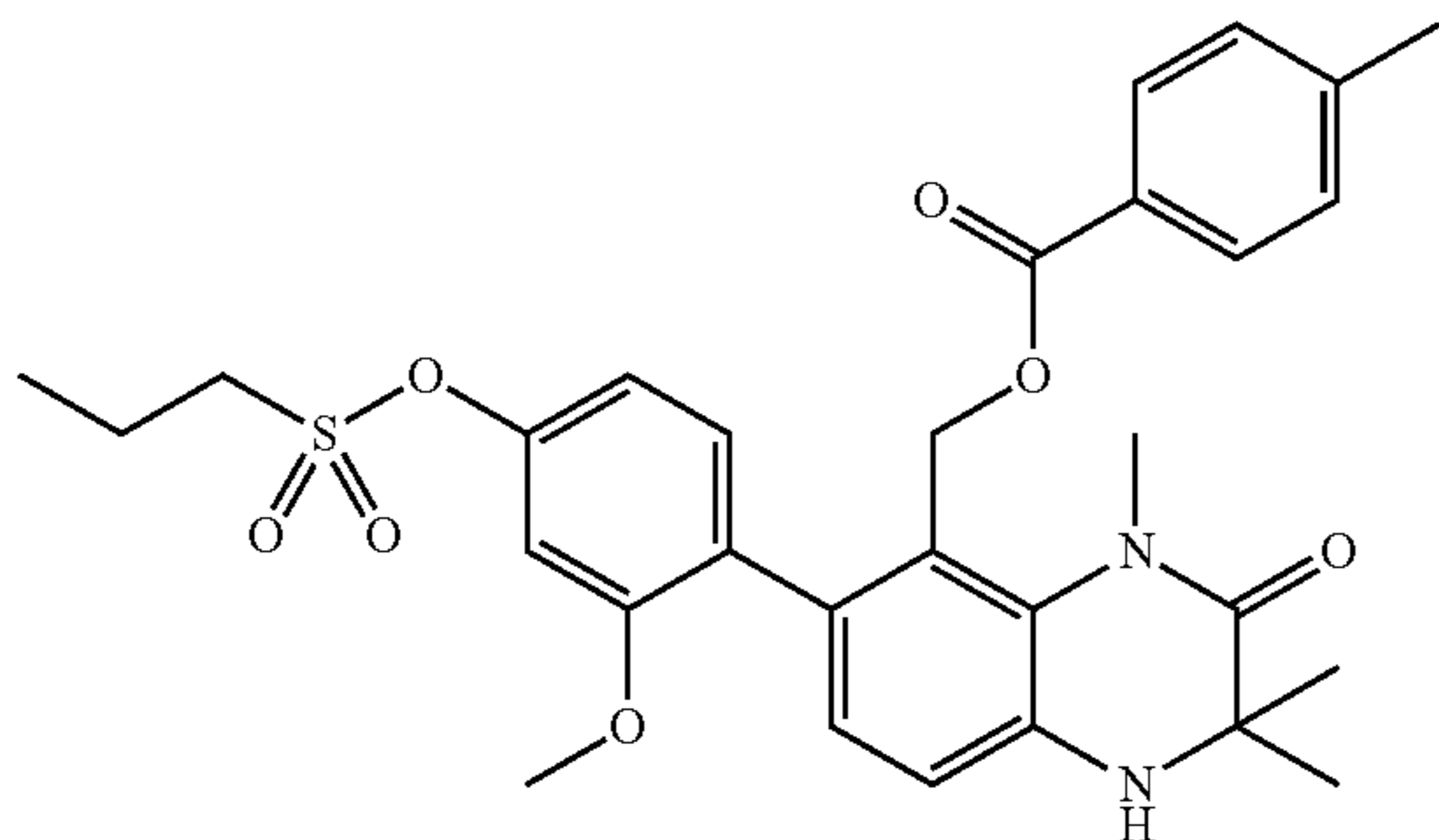
7-(2-Methoxy-4-propylsulfonyloxyphenyl)-8-(4-methylbenzoyloxymethyl)-1,3,3-trimethyl-3,4-dihydro-1H-quinoxalin-2-one (Compound No. 1-39)
