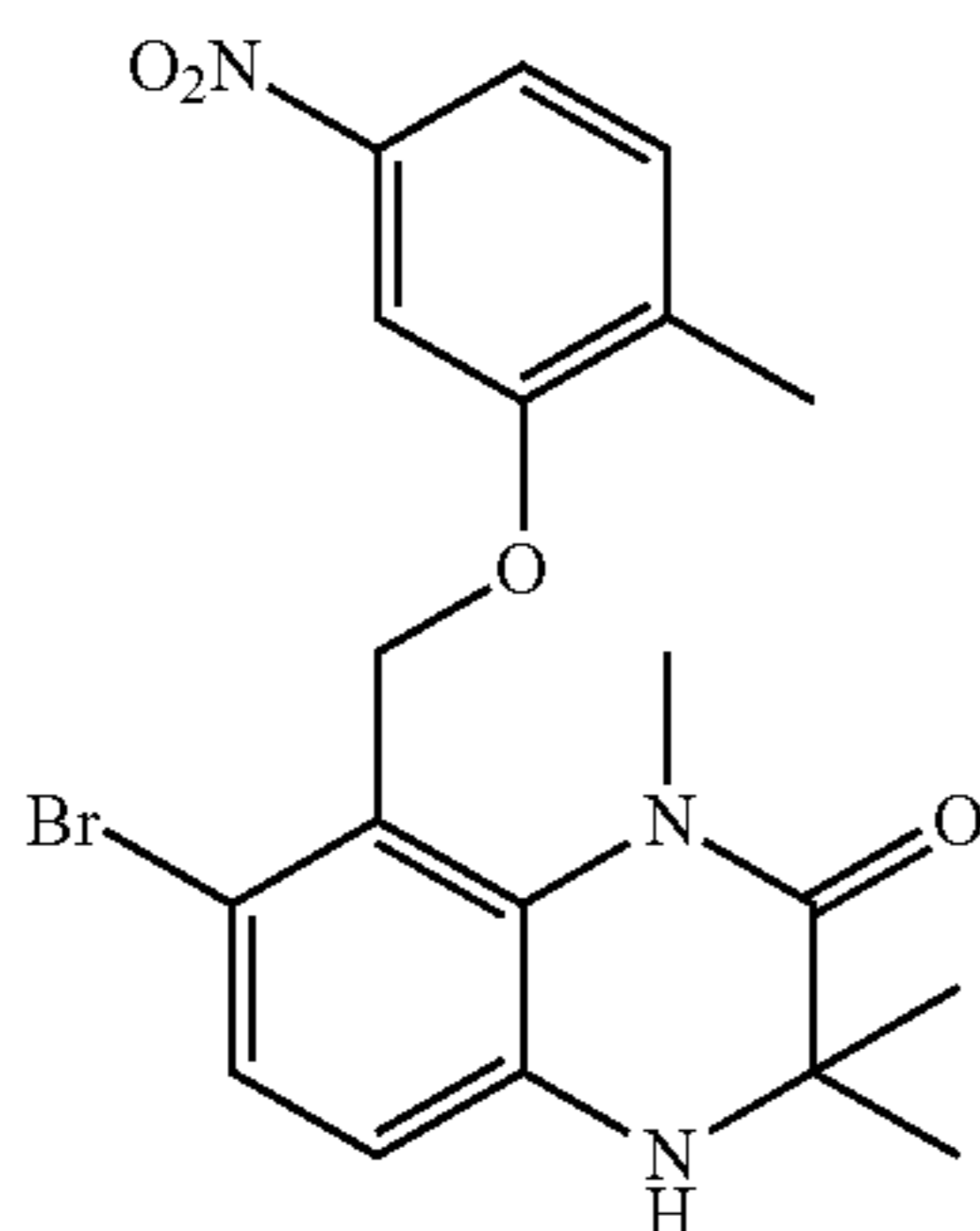
7-Bromo-8-(2-methyl-5-nitrophenoxymethyl)-1,3,3-trimethyl-3,4-dihydro-1H-quinoxalin-2-one (Reference Compound No. 3-3)
