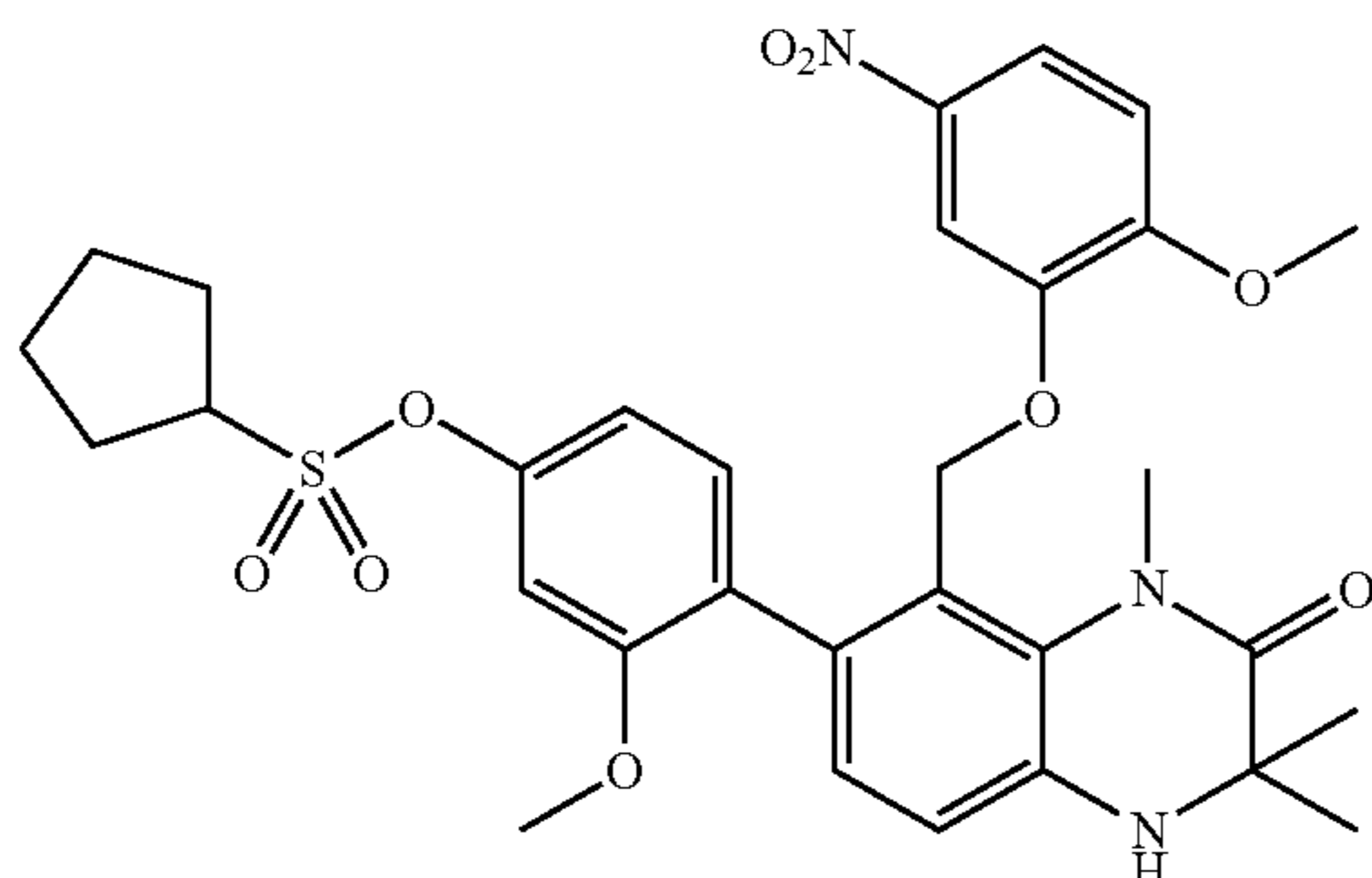
7-(4-Cyclopentylsulfonyloxy-2-methoxyphenyl)-8-(2-methoxy-5-nitrophenoxymethyl)-1,3,3-trimethyl-3,4-dihydro-1H-quinoxalin-2-one (Compound No. 1-28)
