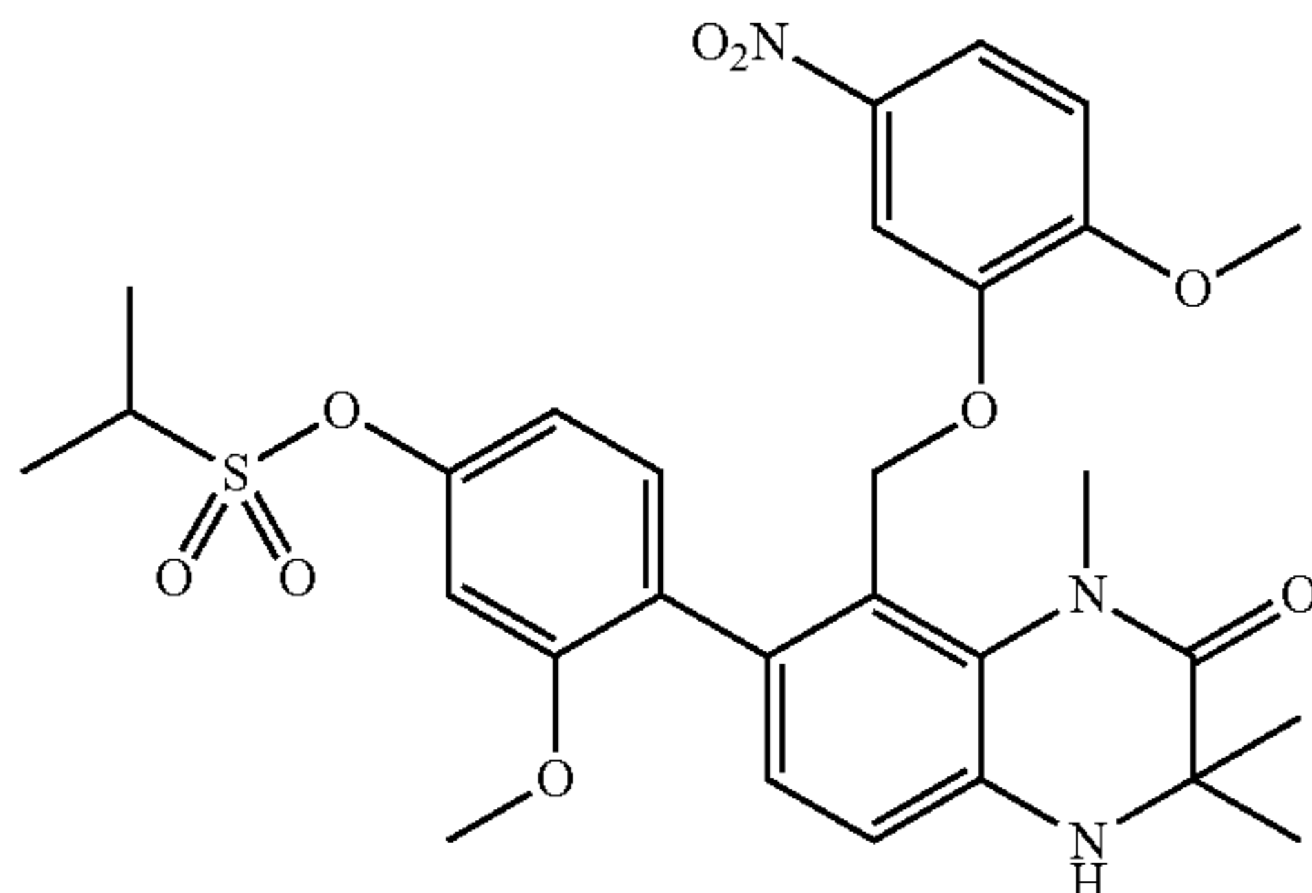
7-(4-Isopropylsulfonyloxy-2-methoxyphenyl)-8-(2-methoxy-5-nitrophenoxy-methyl)-1,3,3-trimethyl-3,4-dihydro-1H-quinoxalin-2-one (Compound No. 1-29)
