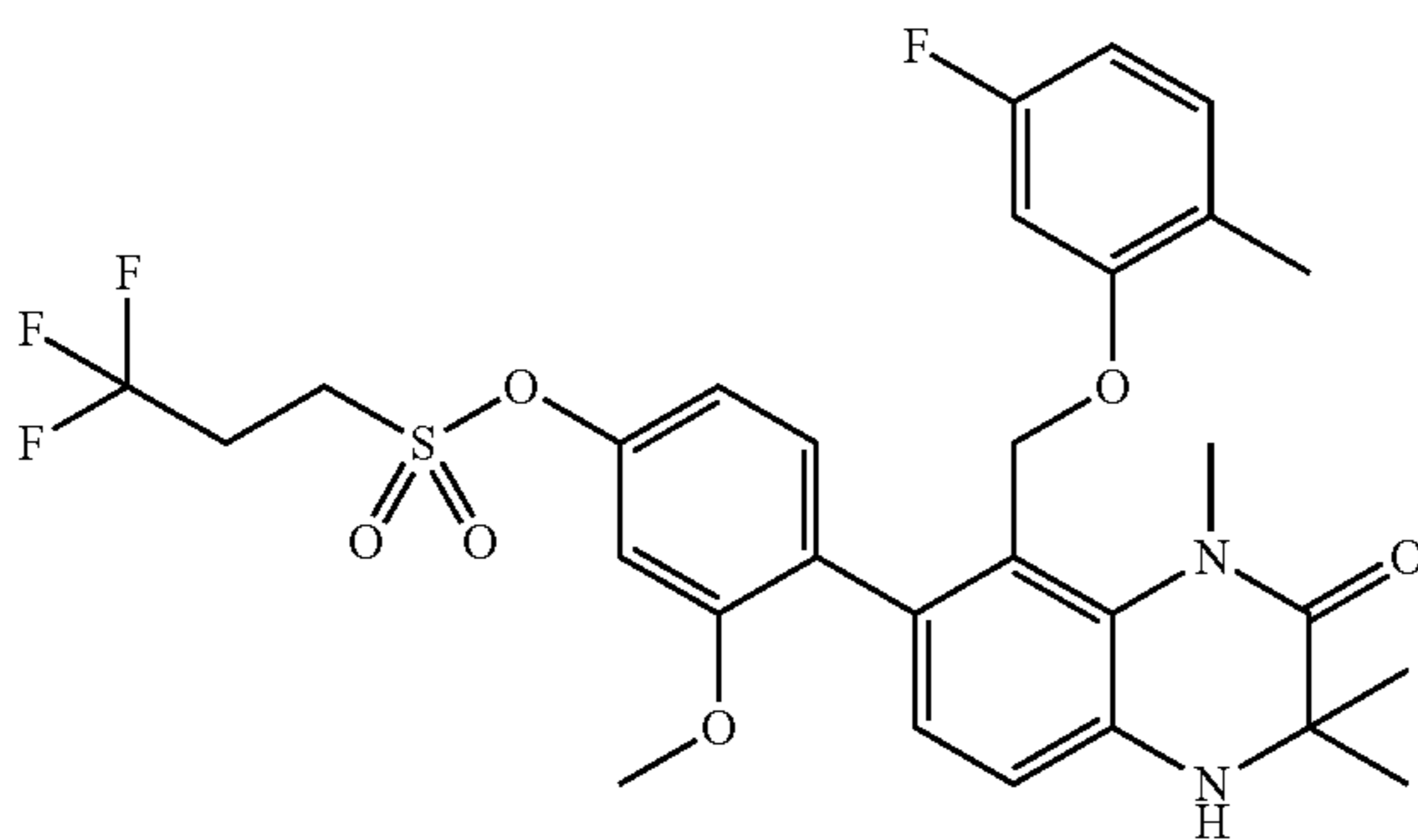
7-(4-Cyclopropylsulfonyloxy-2-methoxyphenyl)-8-(5-fluoro-2-methylphenoxy)-1,3,3-trimethyl-3,4-dihydro-1H-quinoxalin-2-one (Compound No. 1-13)
