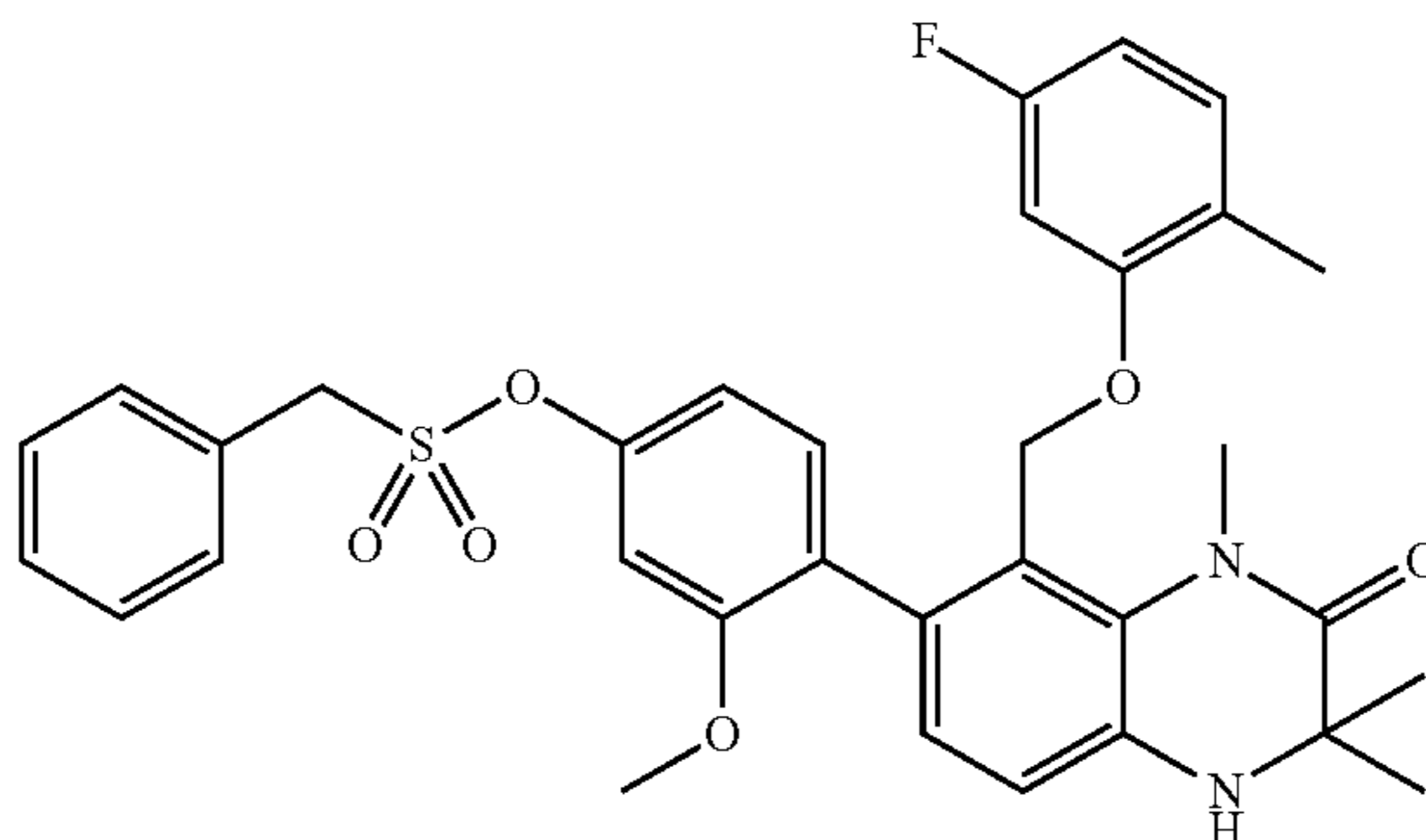
7-(4-Butylsulfonyloxy-2-methoxyphenyl)-8-(5-fluoro-2-methylphenoxy)methyl)-1,3,3-trimethyl-3,4-dihydro-1H-quinoxalin-2-one (Compound No. 1-5)
