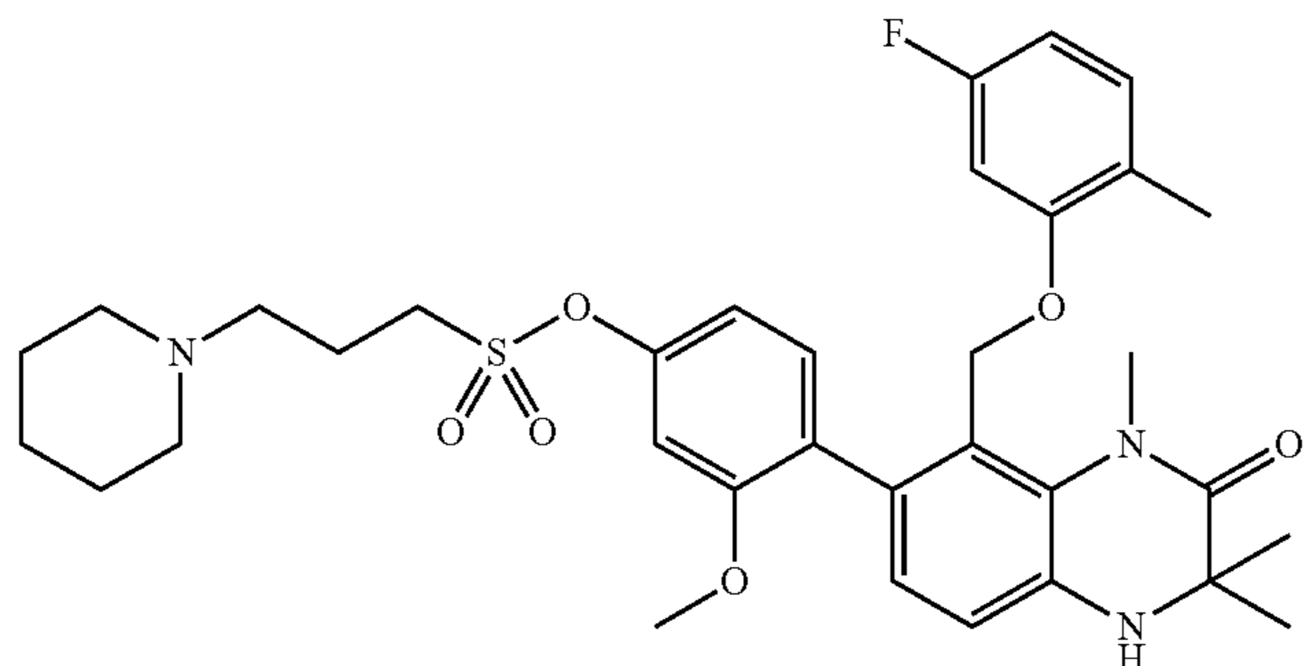
8-(5-Fluoro-2-methylphenoxy)methyl-7-[2-methoxy-4-[3-(piperidin-1-yl)propylsulfonyloxy]phenyl]-1,3,3-trimethyl-3,4-dihydro-1H-quinoxalin-2-one (Compound No. 3-4)
