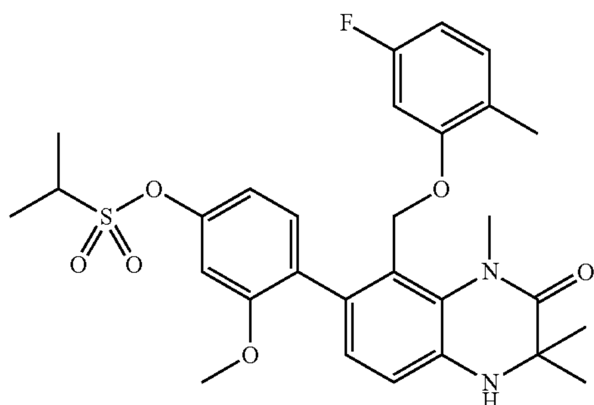
7-[4-(3-Chlorobenzylsulfonyloxy)-2-methoxyphenyl]-8-(5-fluoro-2-methylphenoxy)methyl)-1,3,3-trimethyl-3,4-dihydro-1H-quinoxalin-2-one (Compound No. 1-8)
