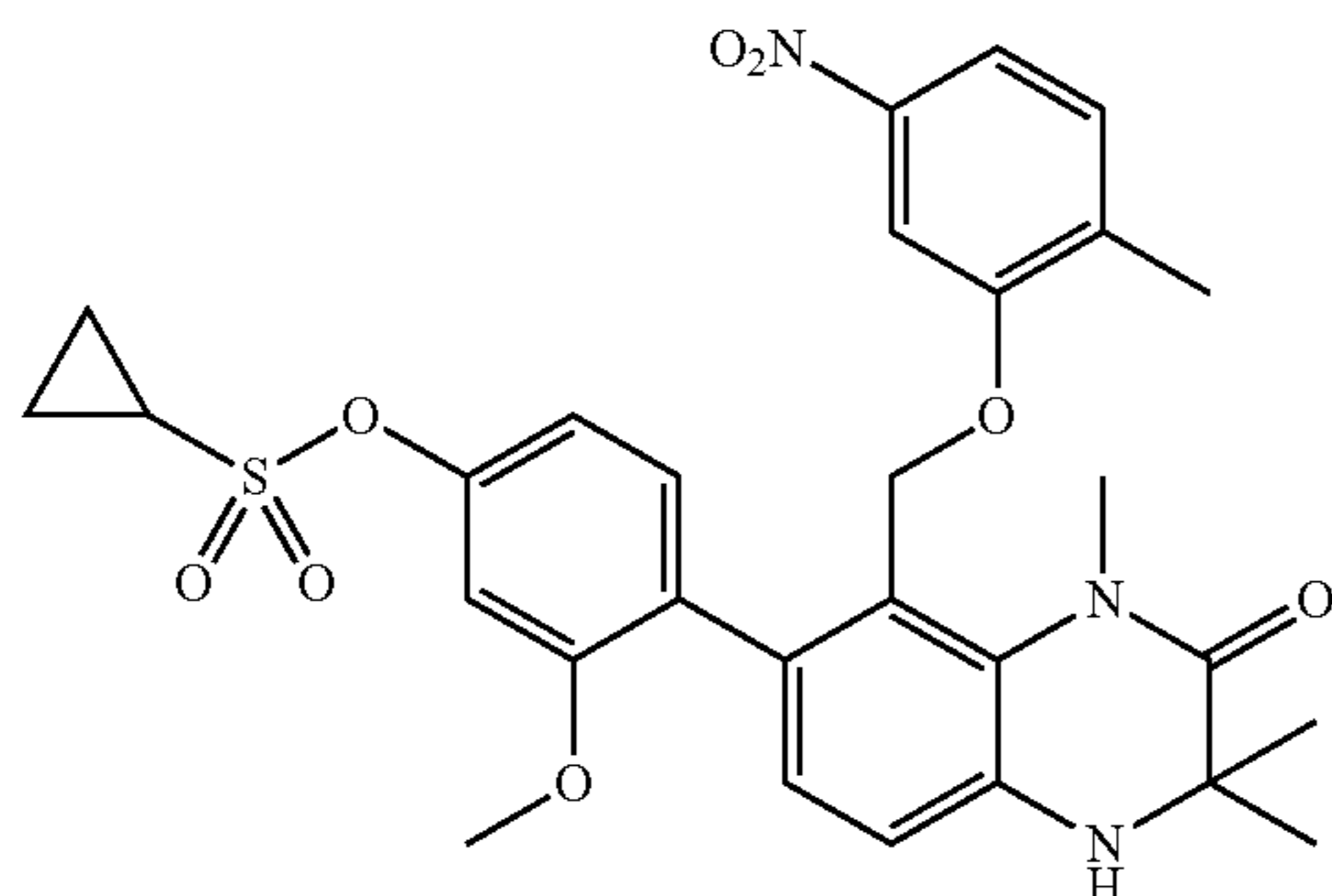
7-(4-Cyclopropylsulfonyloxy-2-methoxyphenyl)-8-(2-methyl-5-nitrophenoxymethyl)-1,3,3-trimethyl-3,4-dihydro-1H-quinoxalin-2-one (Compound No. 1-32)
