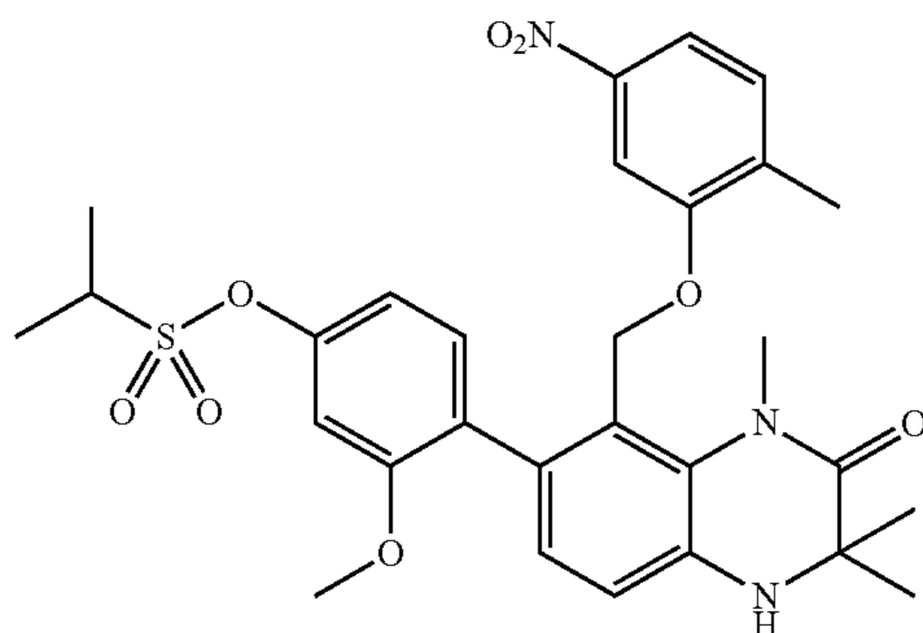
7-(2-Methoxy-4-methylsulfonyloxyphenyl)-8-(2-methyl-5-nitrophenoxymethyl)-1,3,3-trimethyl-3,4-dihydro-1H-quinoxalin-2-one (Compound No. 1-36)
