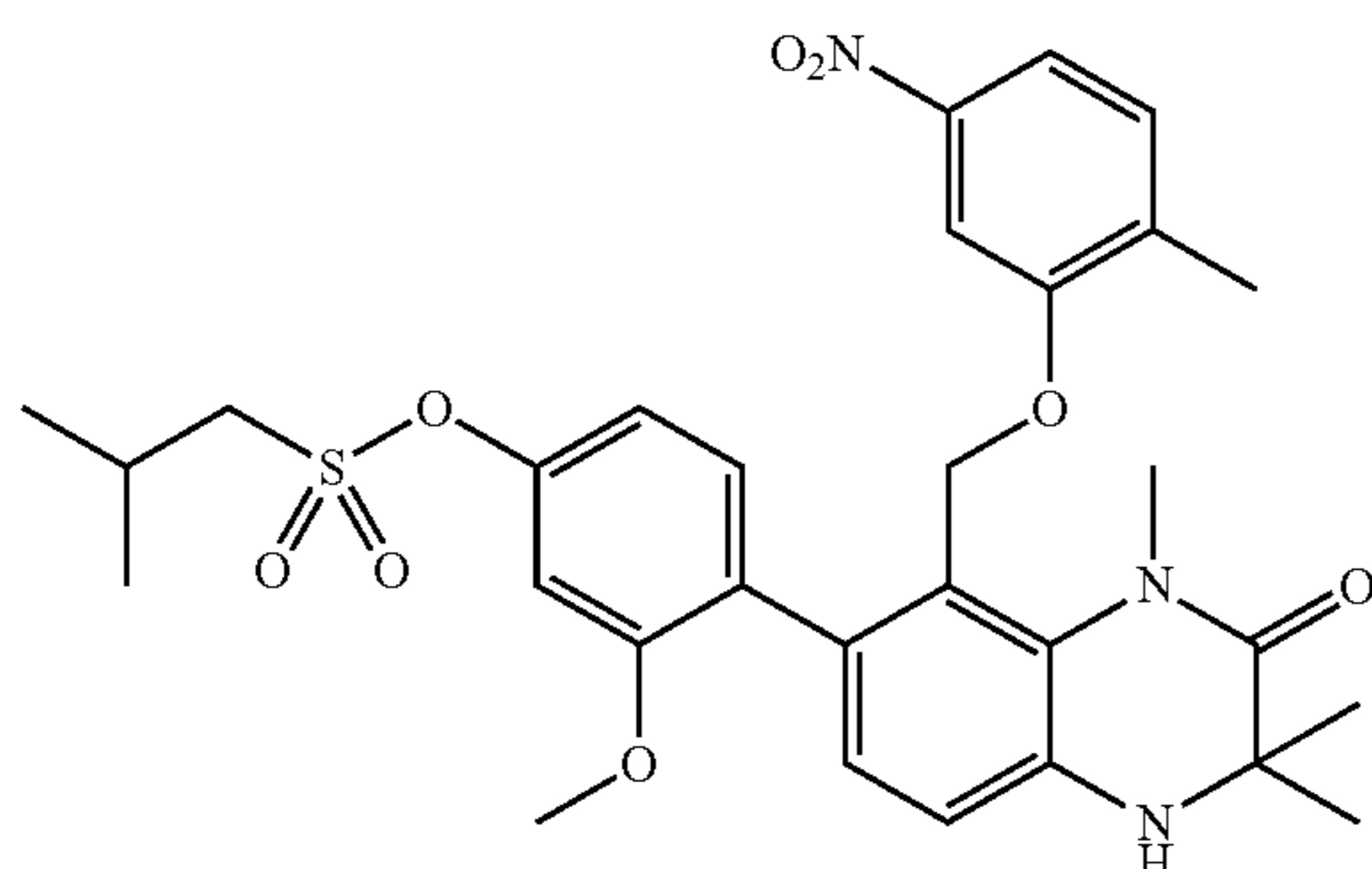
7-(4-Isobutylsulfonyloxy-2-methoxyphenyl)-8-(2-methyl-5-nitrophenoxymethyl)-1,3,3-trimethyl-3,4-dihydro-1H-quinoxalin-2-one (Compound No. 1-34)
