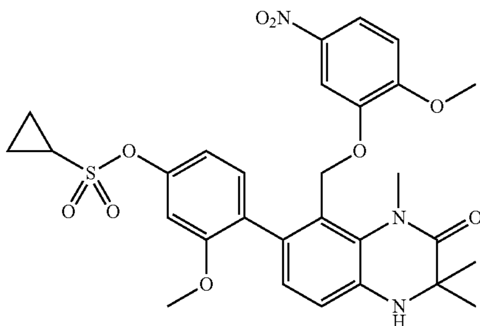
7-(4-Cyclopropylsulfonyloxy-2-methoxyphenyl)-8-(2-methoxy-5-nitrophenoxy-methyl)-1,3,3-trimethyl-3,4-dihydro-1H-quinoxalin-2-one (Compound No. 1-30)
