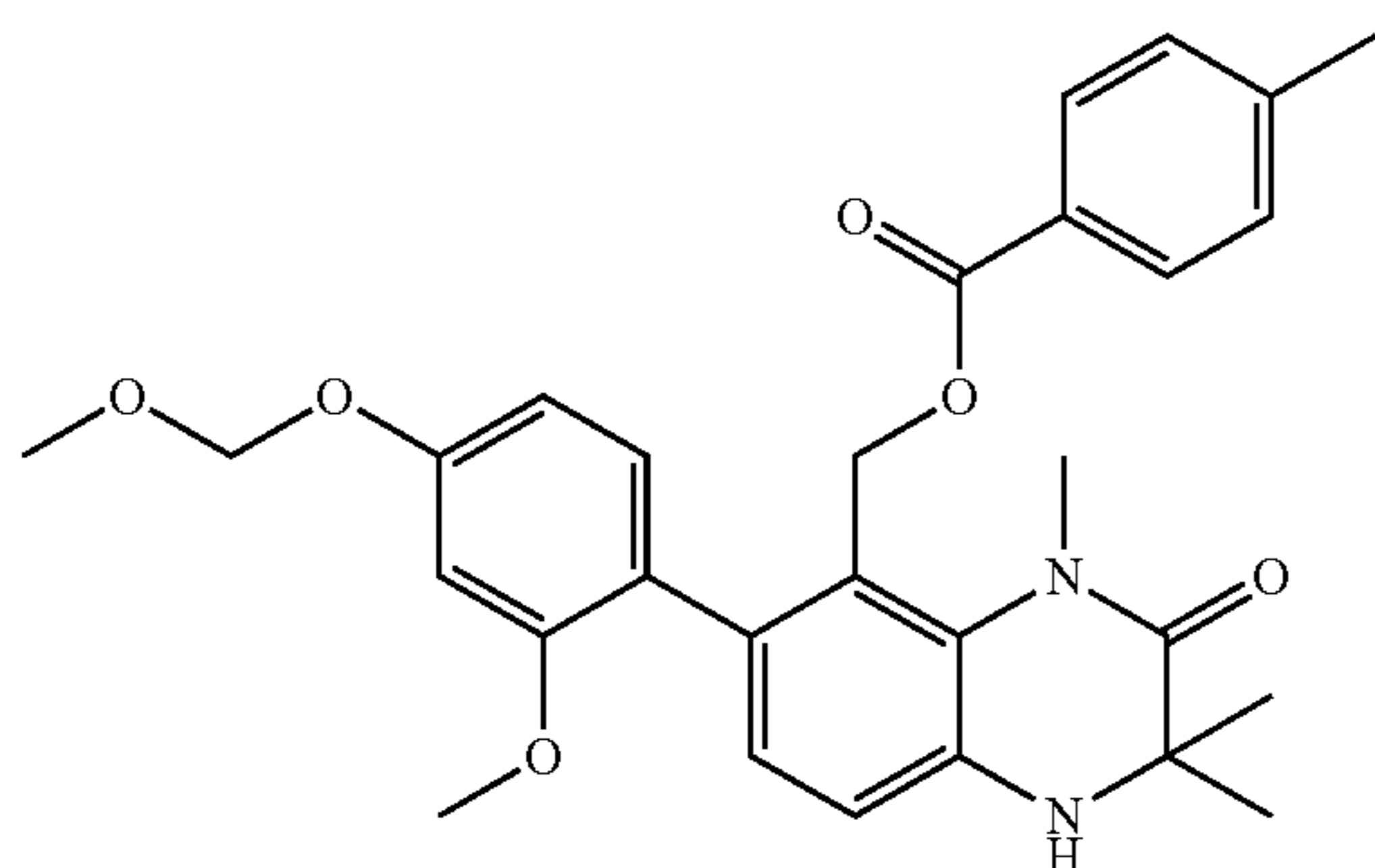
7-(2-Methoxy-4-methoxymethoxyphenyl)-8-(4-methylbenzoyloxymethyl)-1,3,3-trimethyl-3,4-dihydro-1H-quinoxalin-2-one (Reference Compound No. 3-4)
