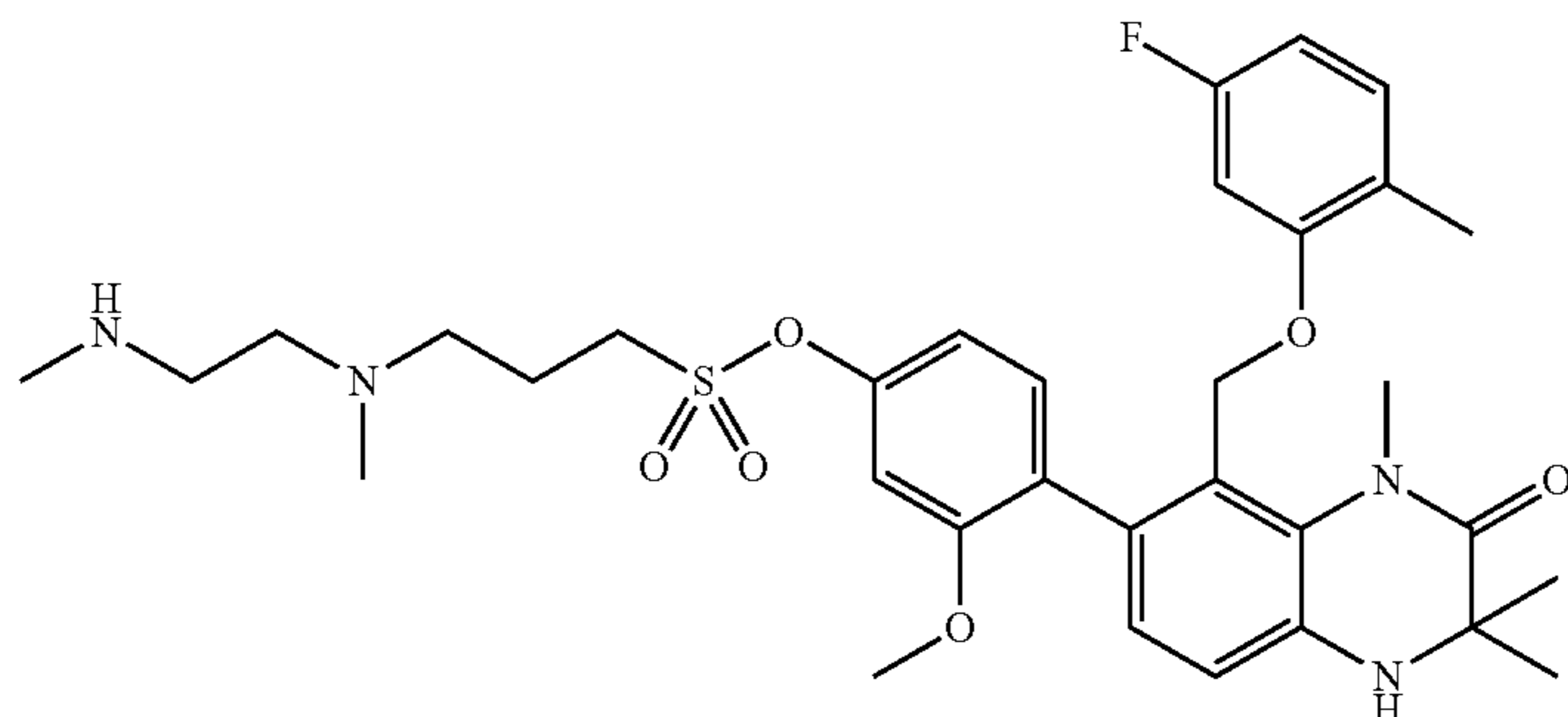
8-(5-Fluoro-2-methylphenoxy)methyl-7-[2-methoxy-4-[3-[N-(2-methylaminoethyl)-N-methylamino]propylsulfonyloxy]phenyl]-1,3,3-trimethyl-3,4-dihydro-1H-quinoxalin-2-one (Compound No. 3-5)
