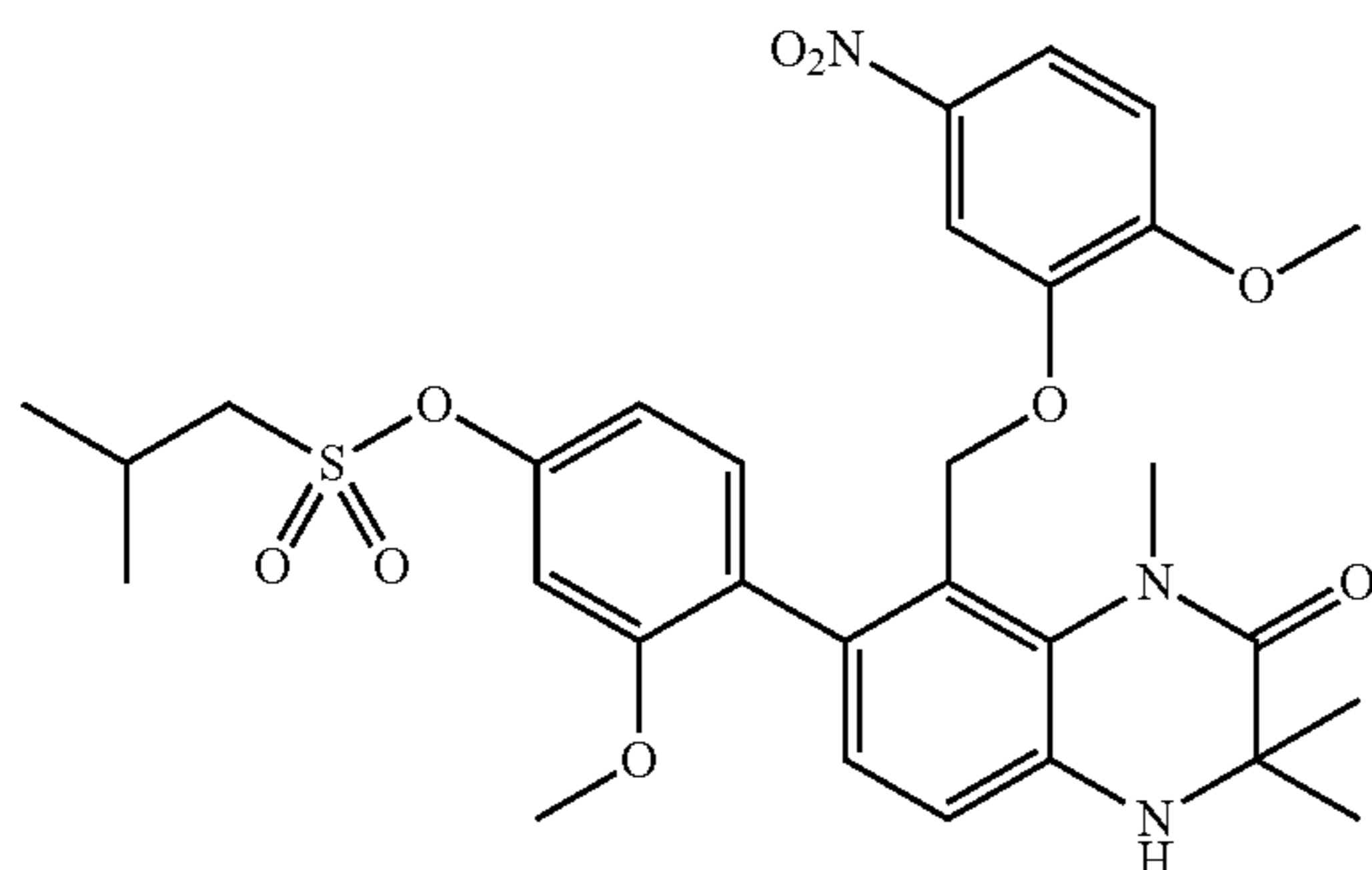
7-(4-Isobutylsulfonyloxy-2-methoxyphenyl)-8-(2-methoxy-5-nitrophenoxymethyl)-1,3,3-trimethyl-3,4-dihydro-1H-quinoxalin-2-one (Compound No. 1-27)
