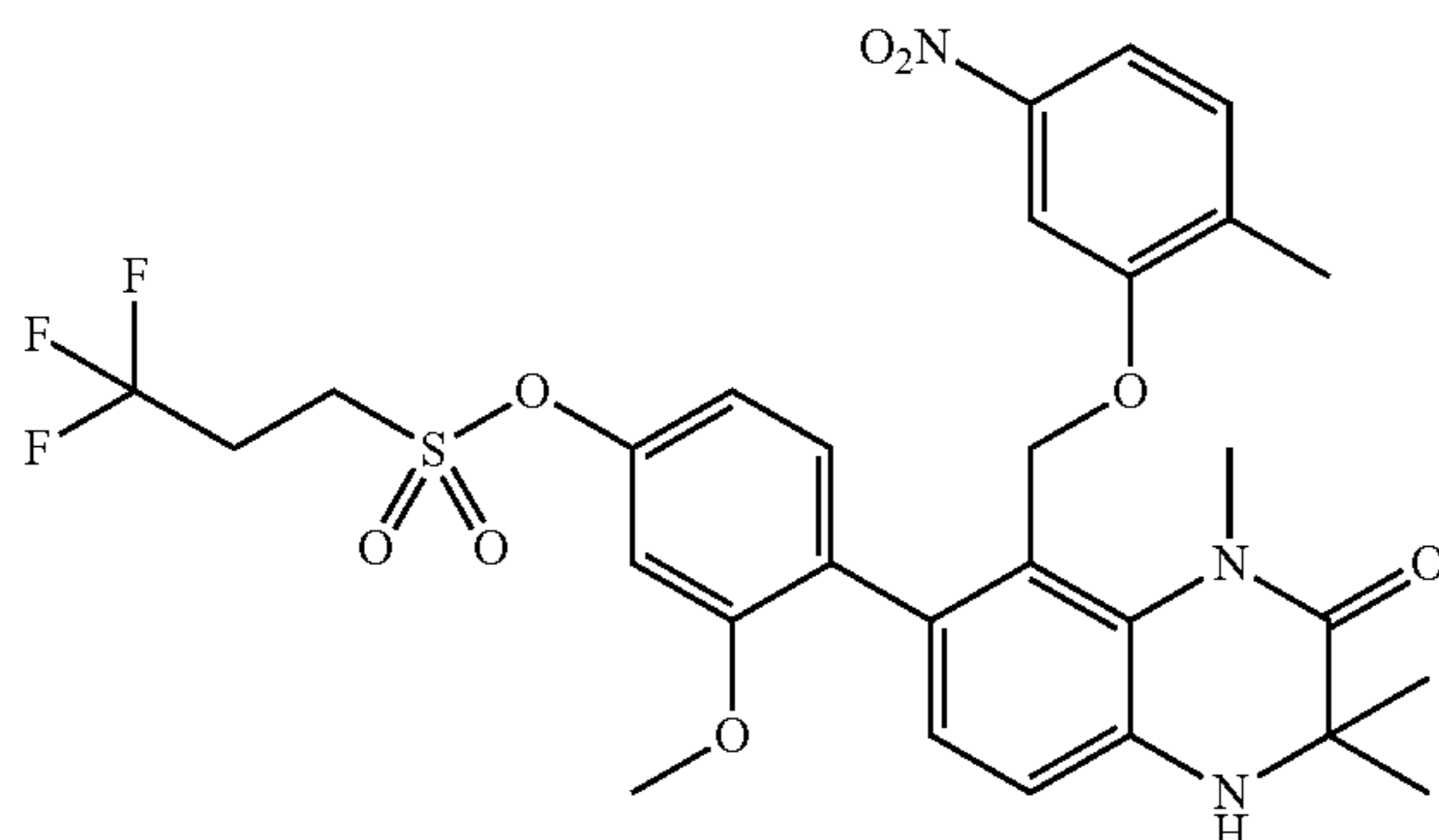
7-[2-Methoxy-4-(3,3,3-trifluoropropylsulfonyloxy)phenyl]-8-(2-methyl-5-nitrophenoxymethyl)-1,3,3-trimethyl-3,4-dihydro-1H-quinoxalin-2-one (Compound No. 1-33)
