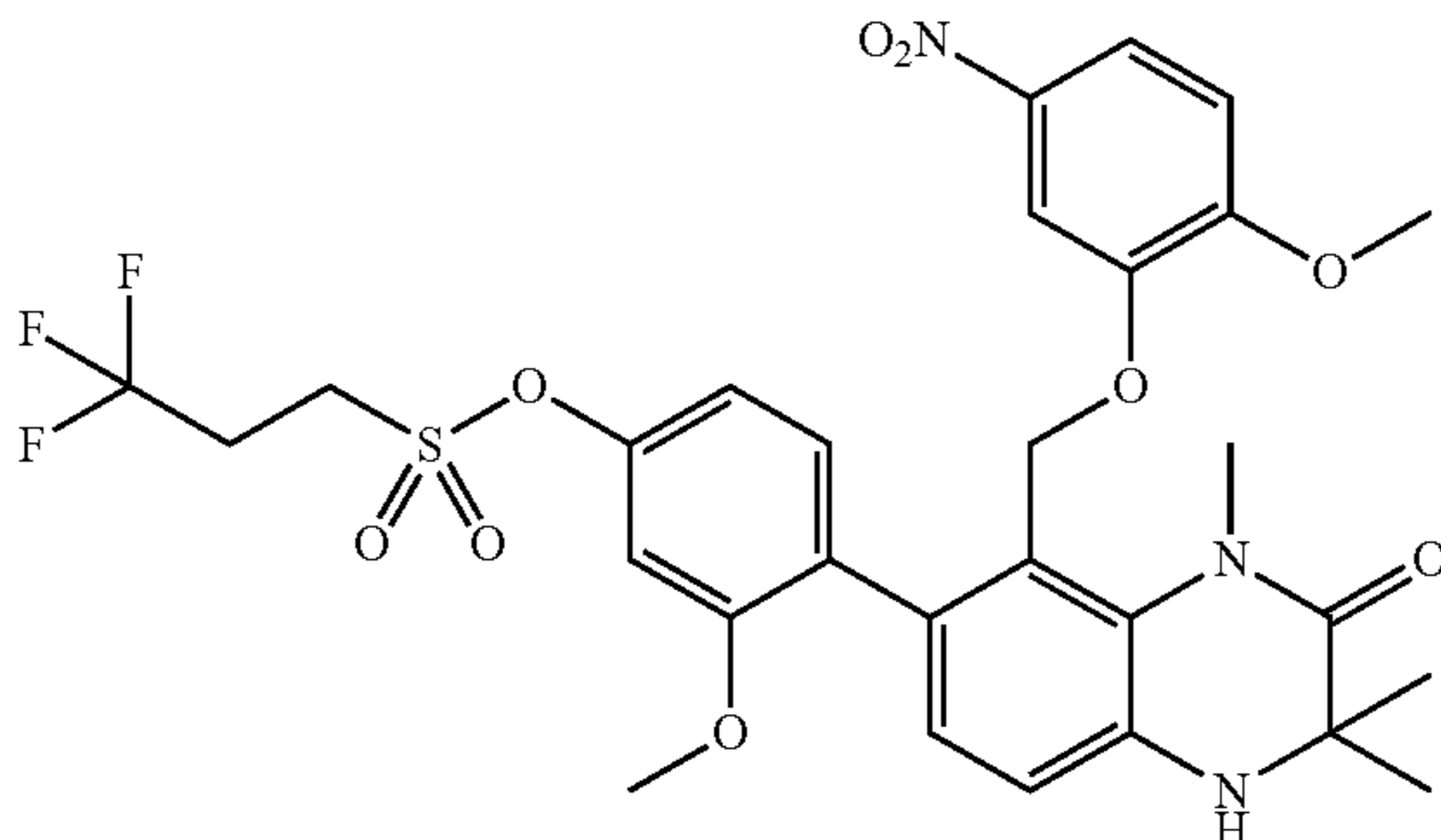
8-(2-Methoxy-5-nitrophenoxymethyl)-7-[2-methoxy-4-(3,3,3-trifluoropropylsulfonyloxy)phenyl]-1,3,3-trimethyl-3,4-dihydro-1H-quinoxalin-2-one (Compound No. 1-26)
