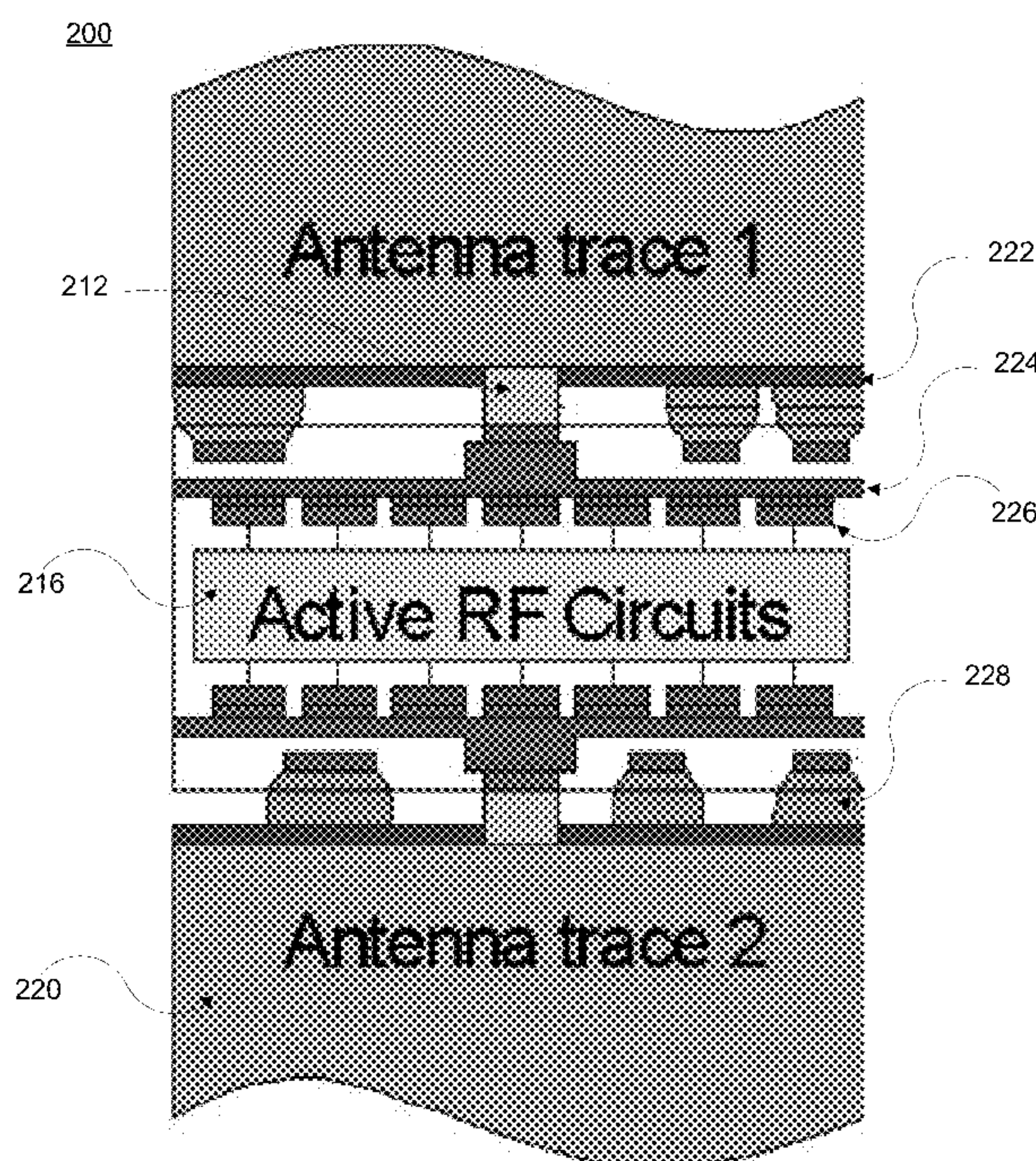
CONCEPTUAL DIAGRAM OF AN ASSEMBLED RFID TAG
