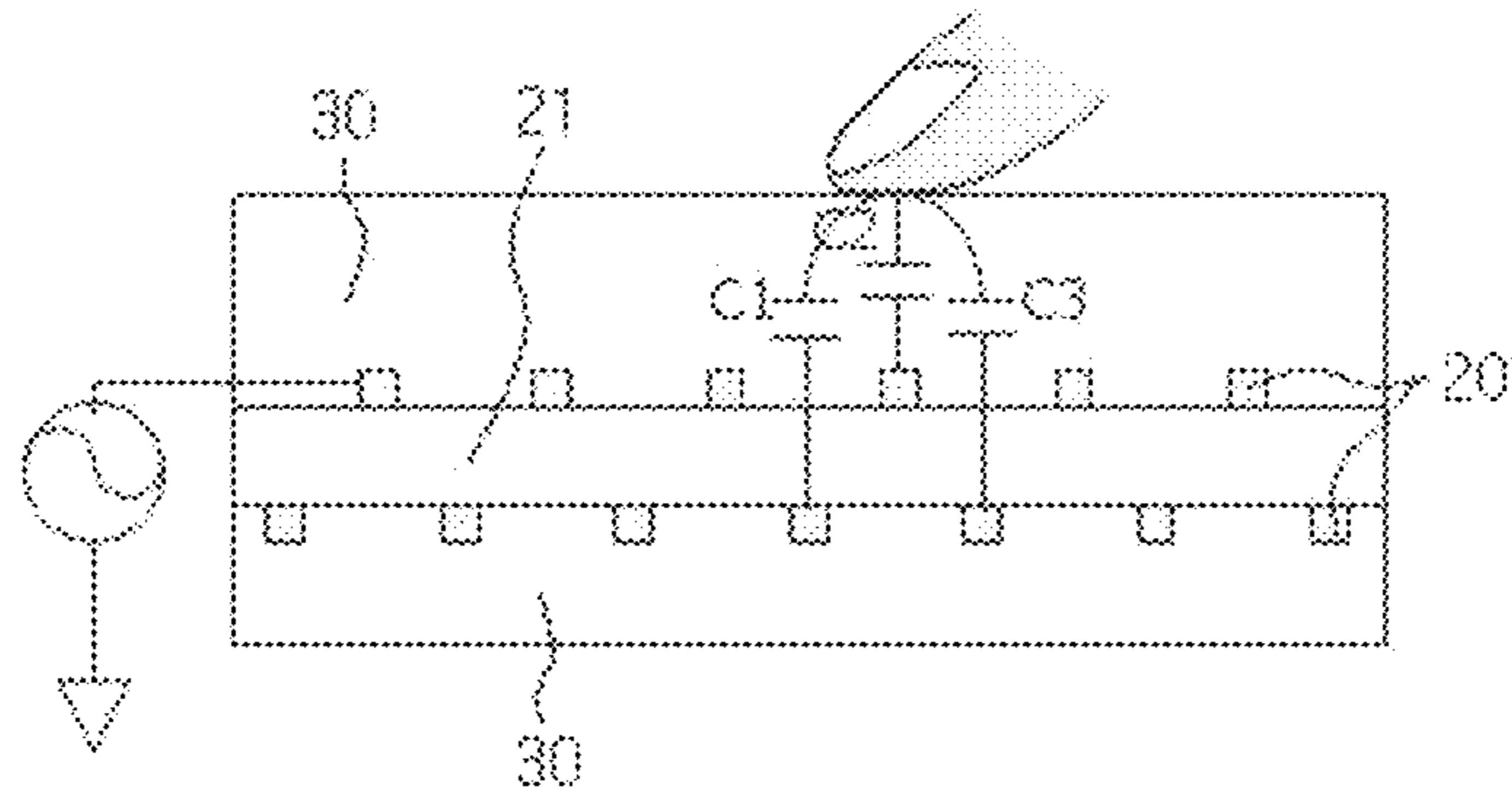
Fig. 5 PRIOR ART
