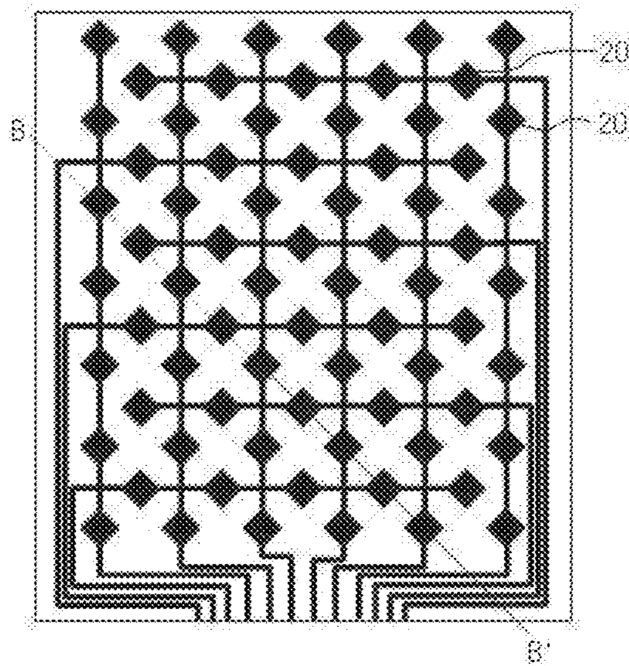
Fig. 2 PRIOR ART
