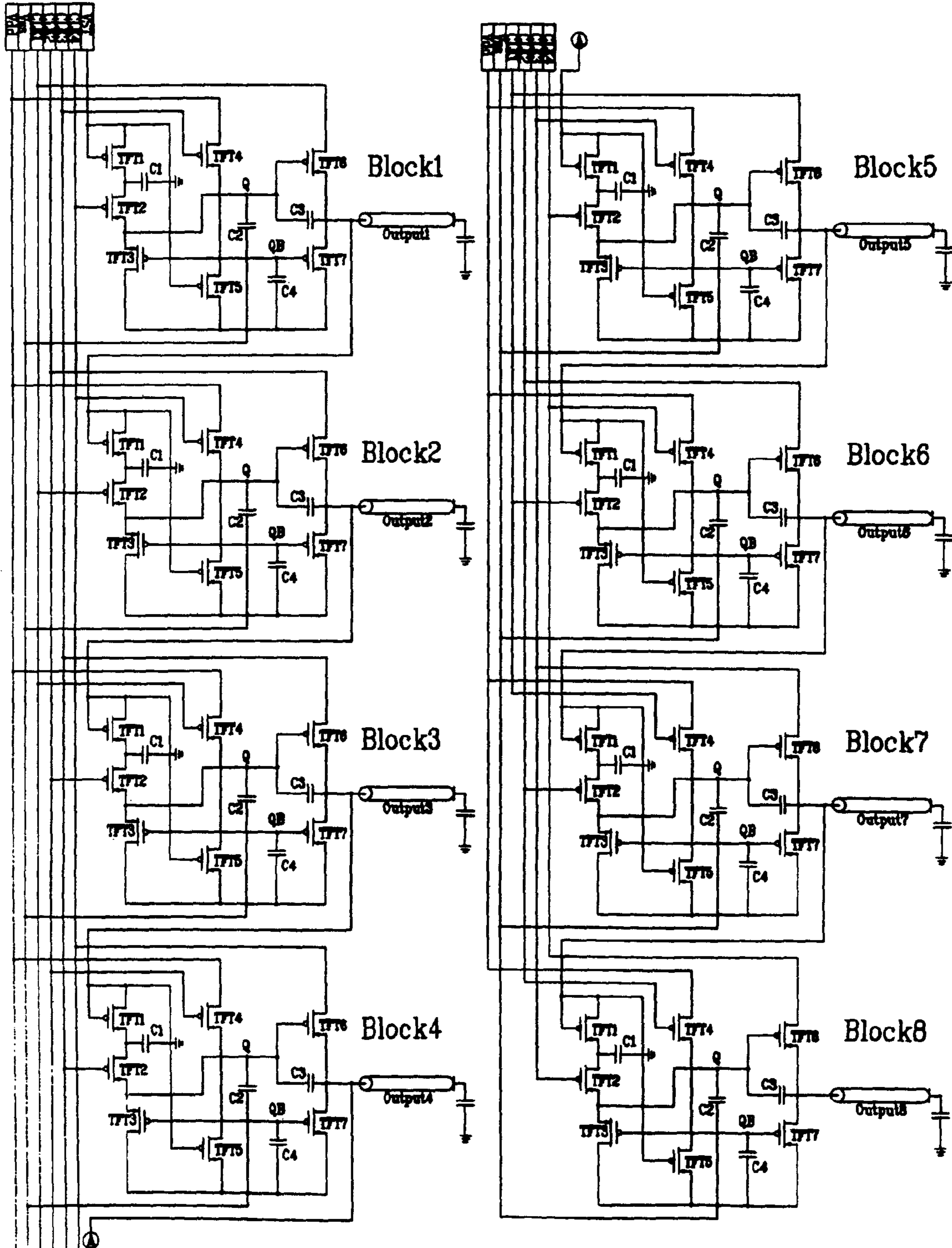
FIG.2 Related Art
