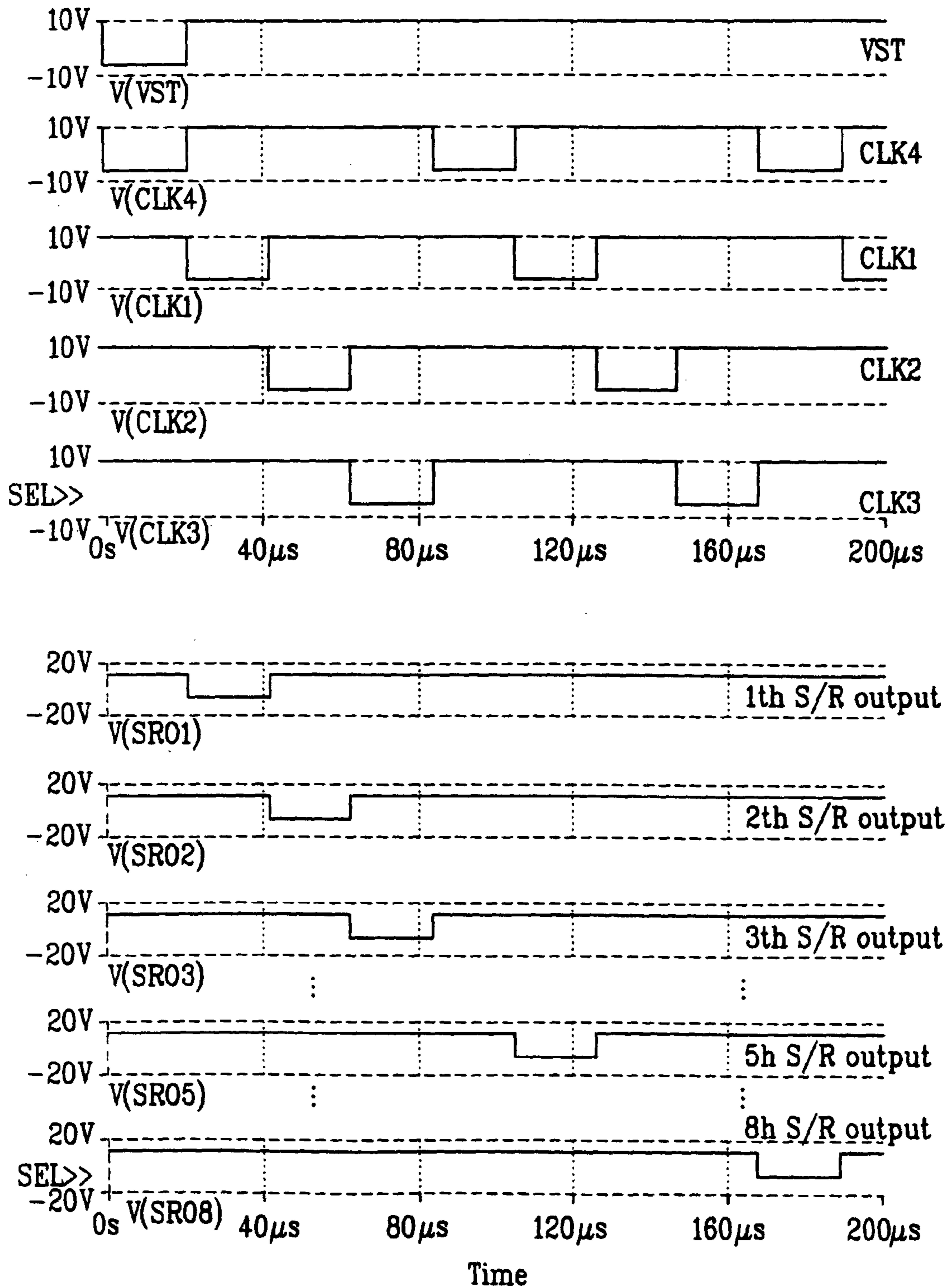
FIG. 3 Related Art
