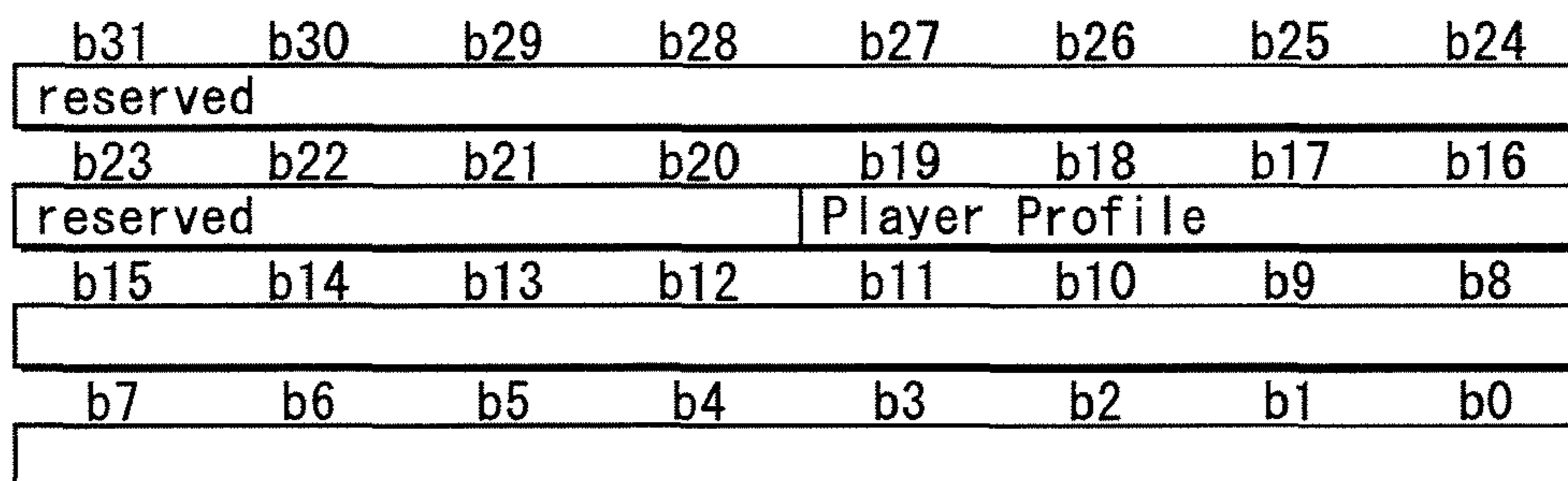
FIG. 27C PSR31:Player Profile/Player Version
