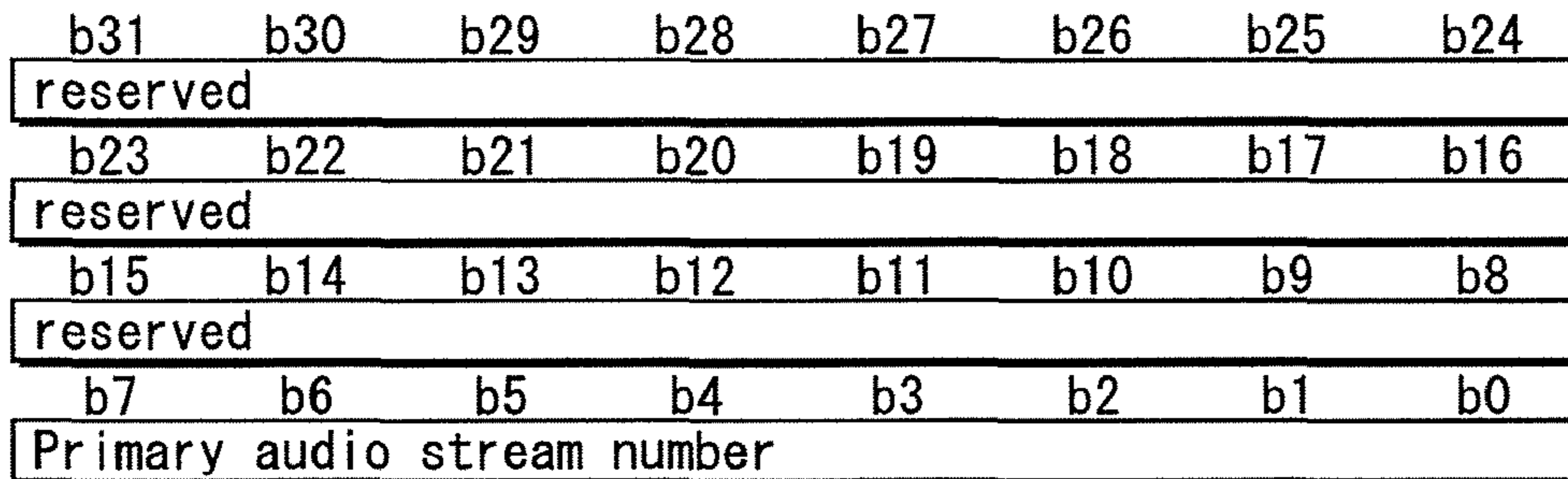
FIG. 27A PSR1:Primary Audio Stream Number
