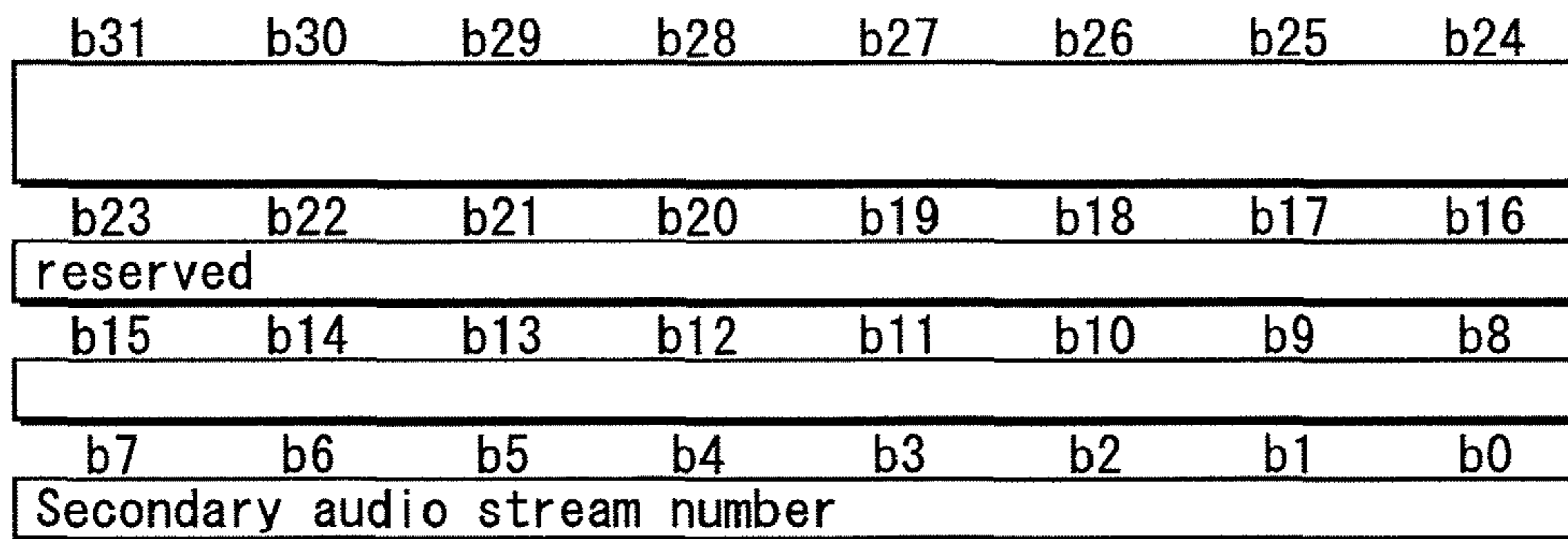
FIG. 27B PSR14:Secondary Audio Stream Number
