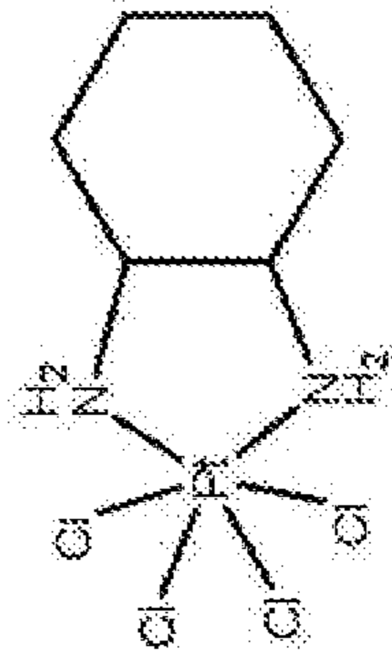
ormaplatin tetraplatin
