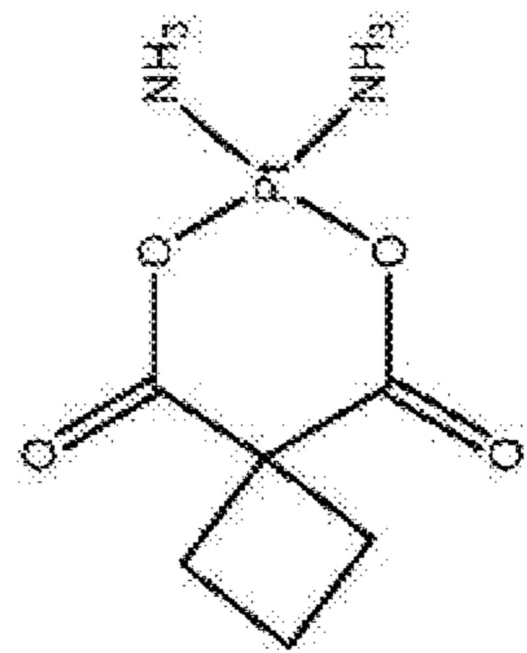
carboplatin
