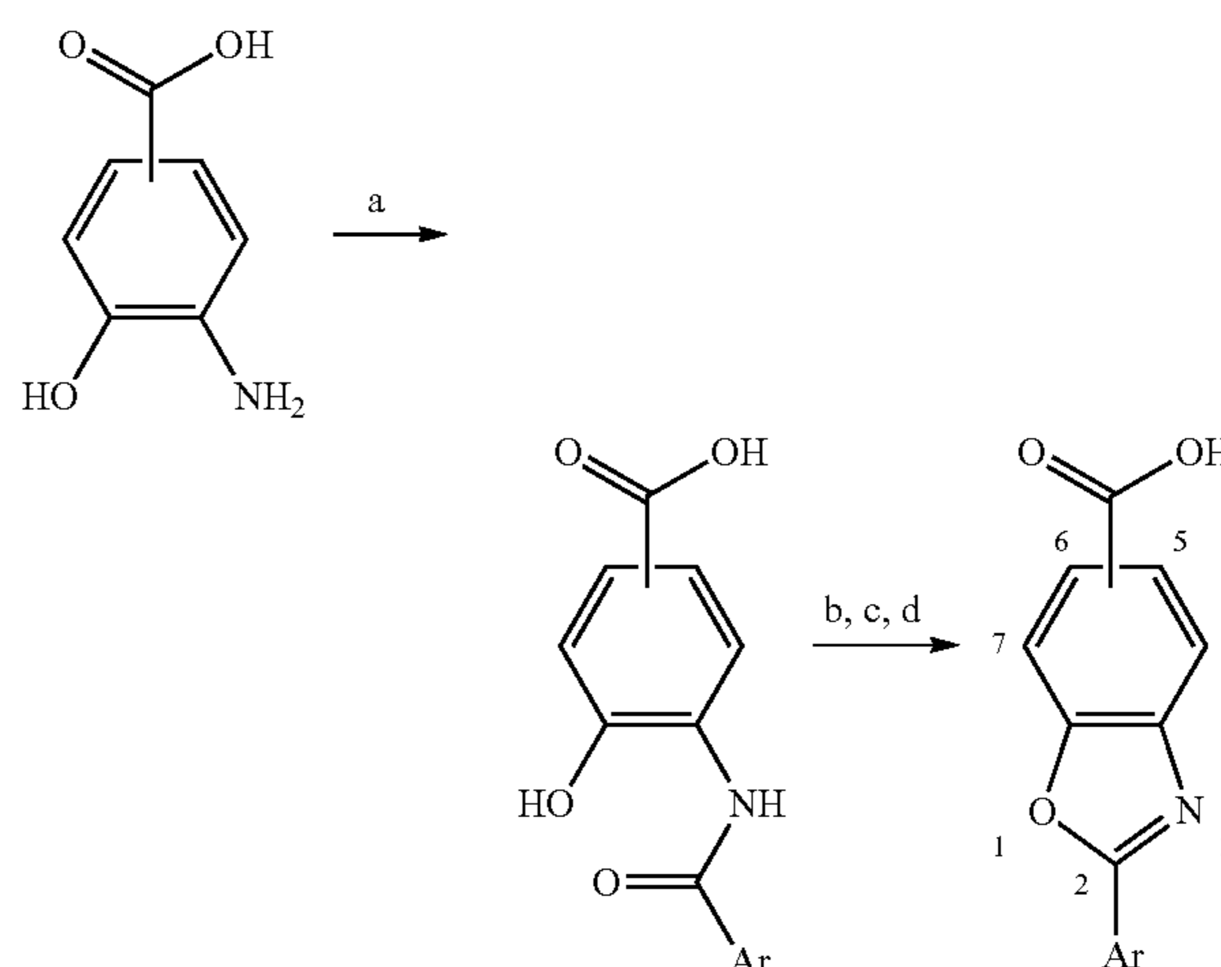
Scheme 1: General Synthesis of Benzoxazoles
