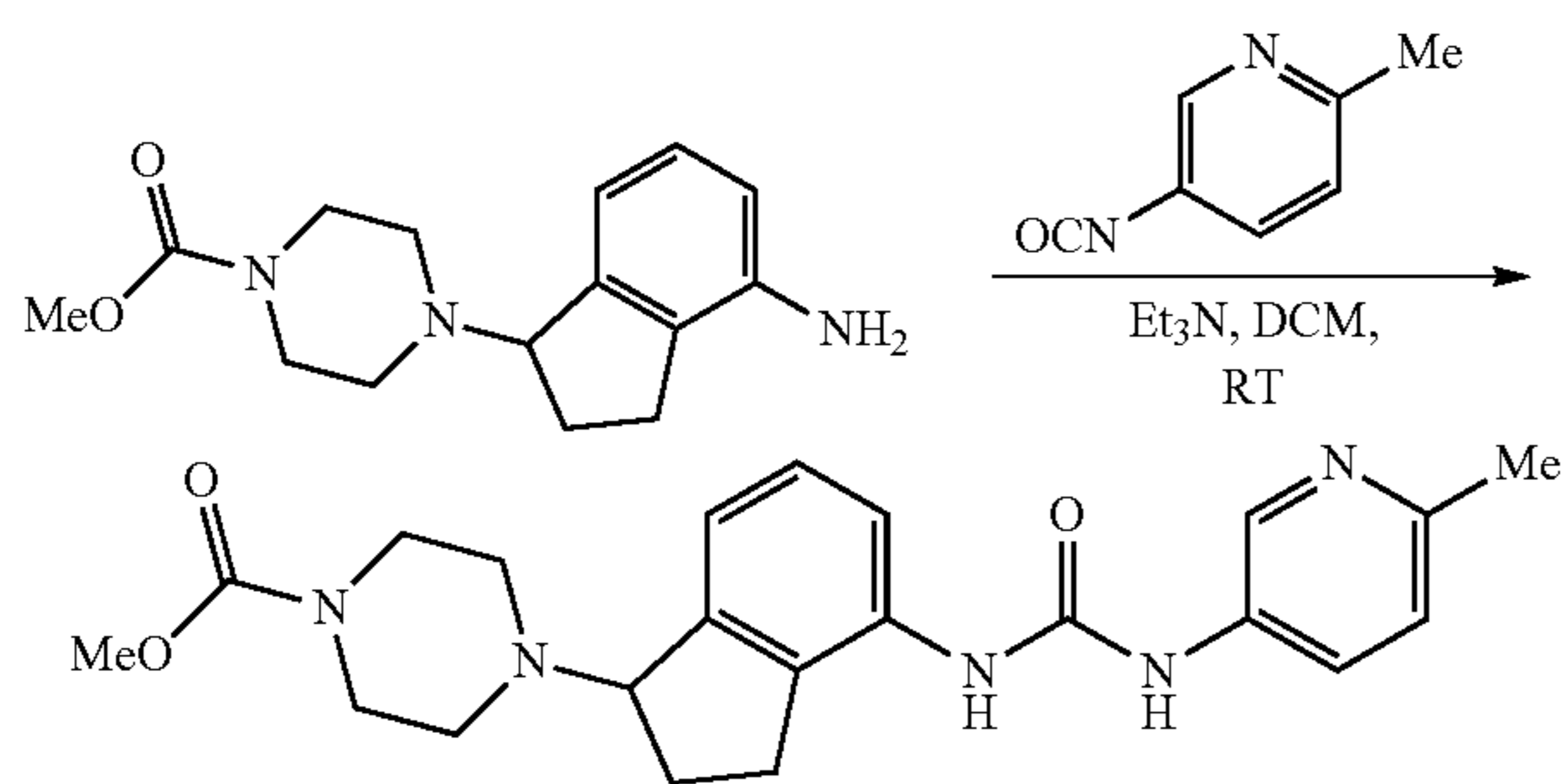
Methyl 4-(4-(3-(6-methylpyridin-3-yl)ureido)-2,3-dihydro-1H-inden-1-yl)piperazine-1-carboxylate
