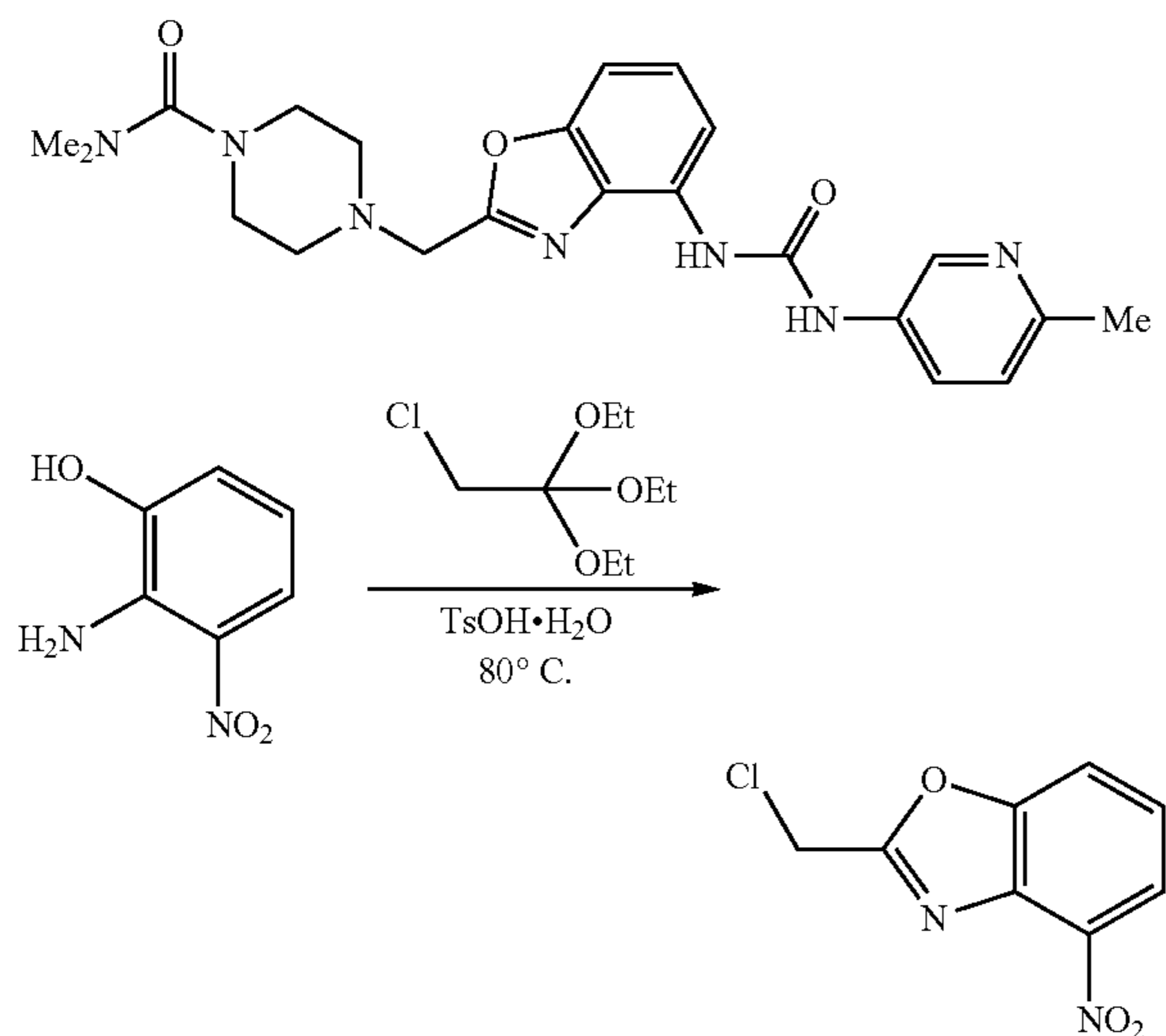
2-(Chloromethyl)-4-nitrobenzo[d]oxazole
