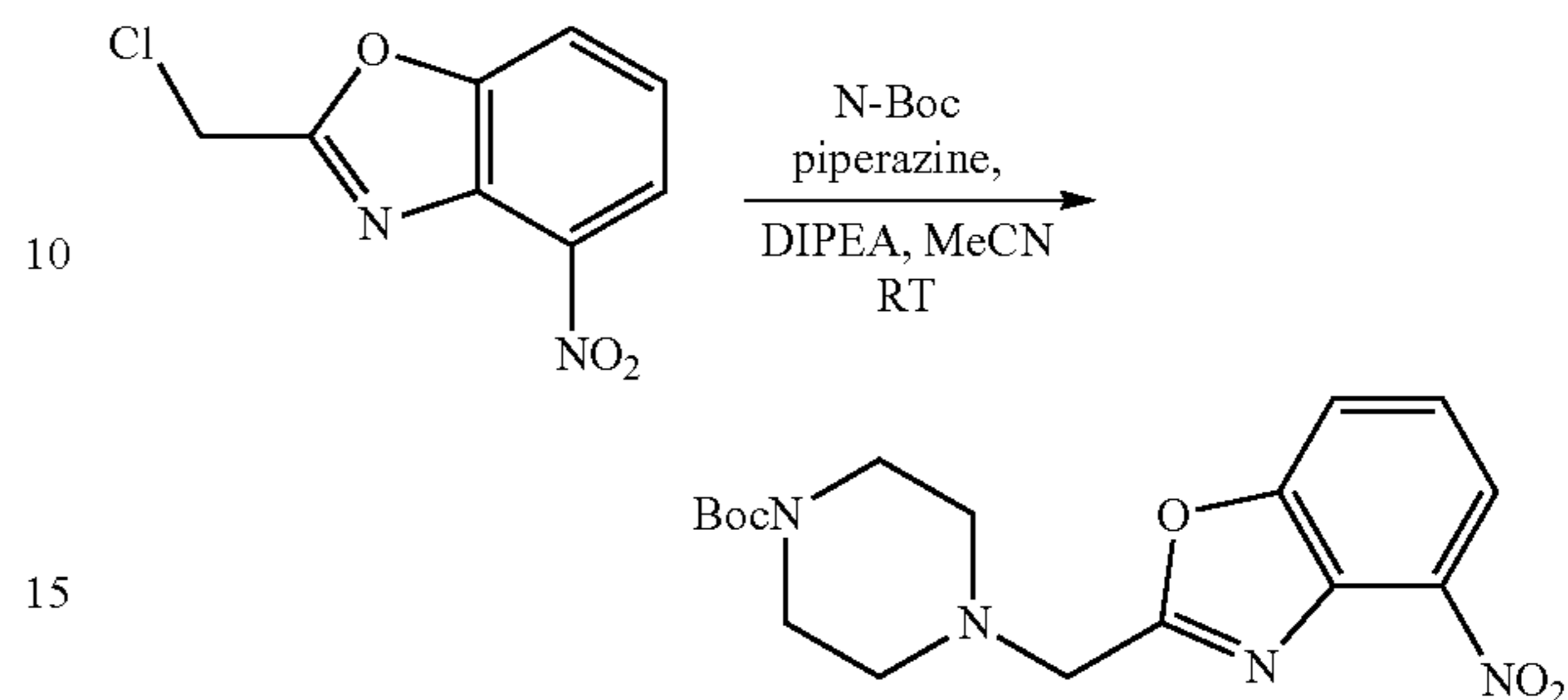
tert-Butyl 4-((4-nitrobenzo[d]oxazol-2-yl)methyl)piperazine-1-carboxylate
