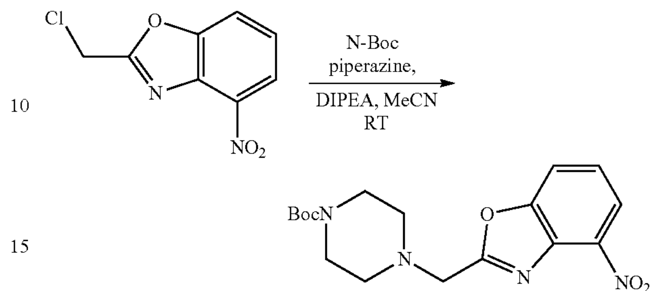
tert-Butyl 4-((4-nitrobenzo[d]oxazol-2-yl)methyl)piperazine-1-carboxylate
