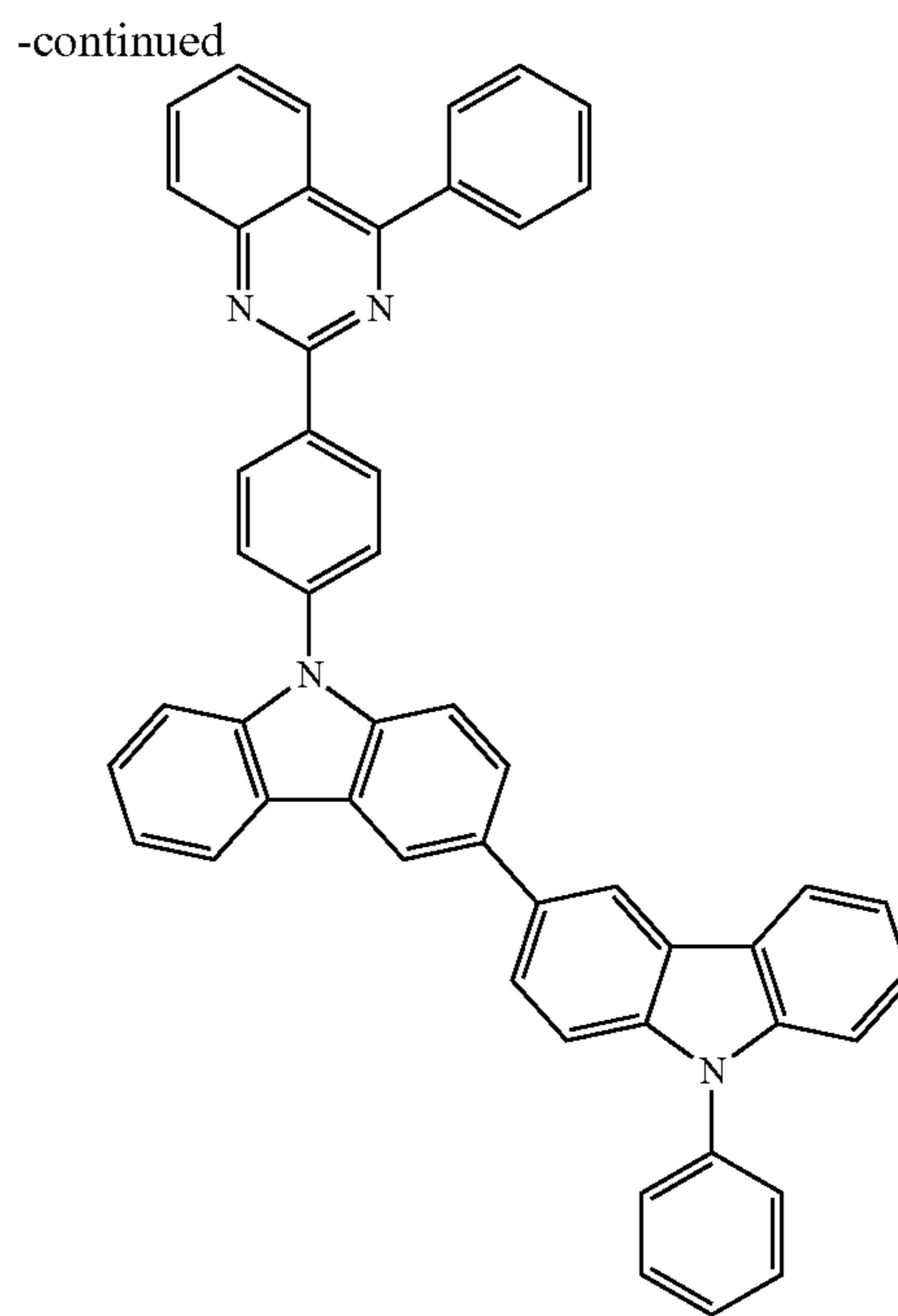
Compound 7
