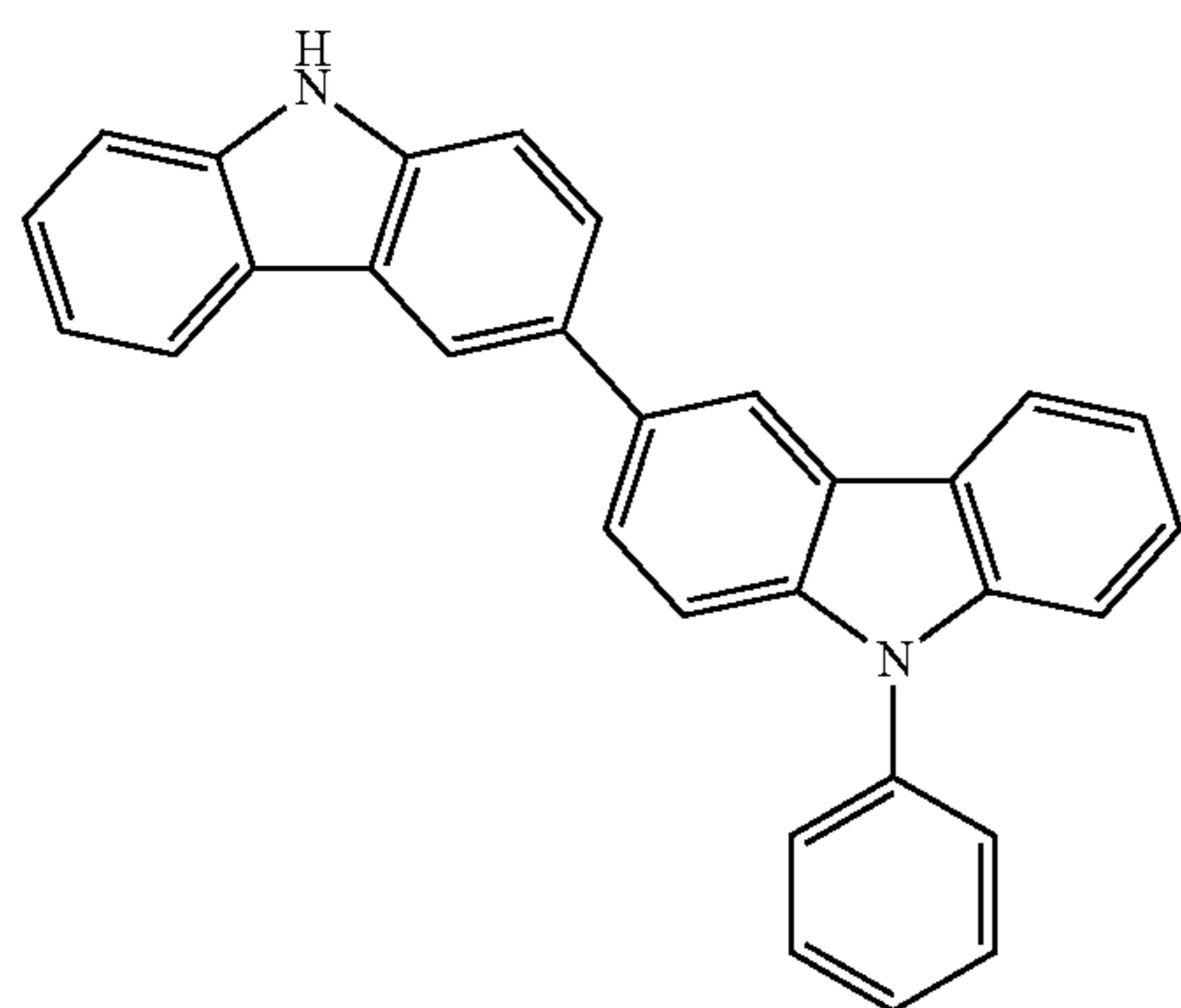
Intermediate body 1-4
