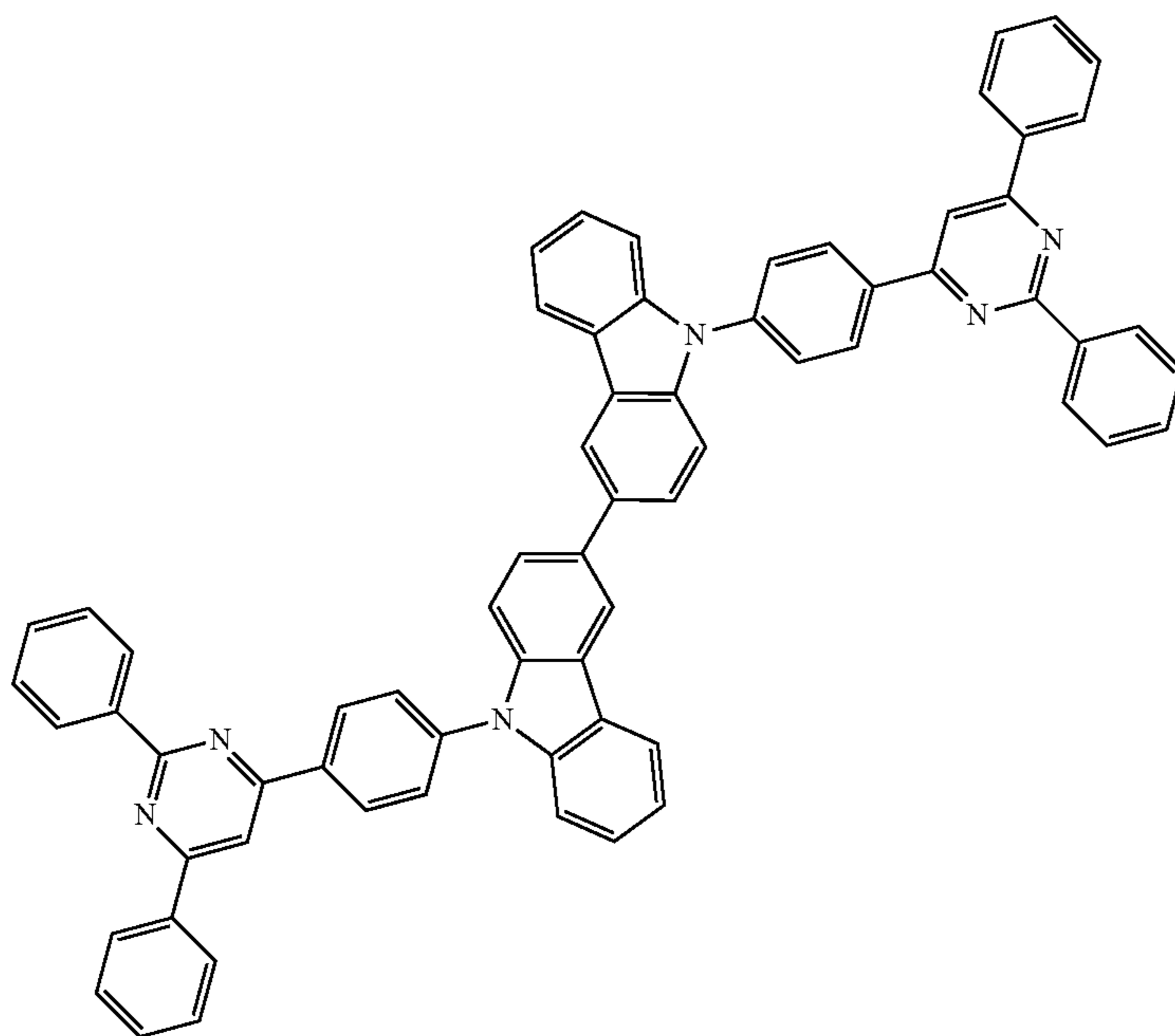
Compound 4
