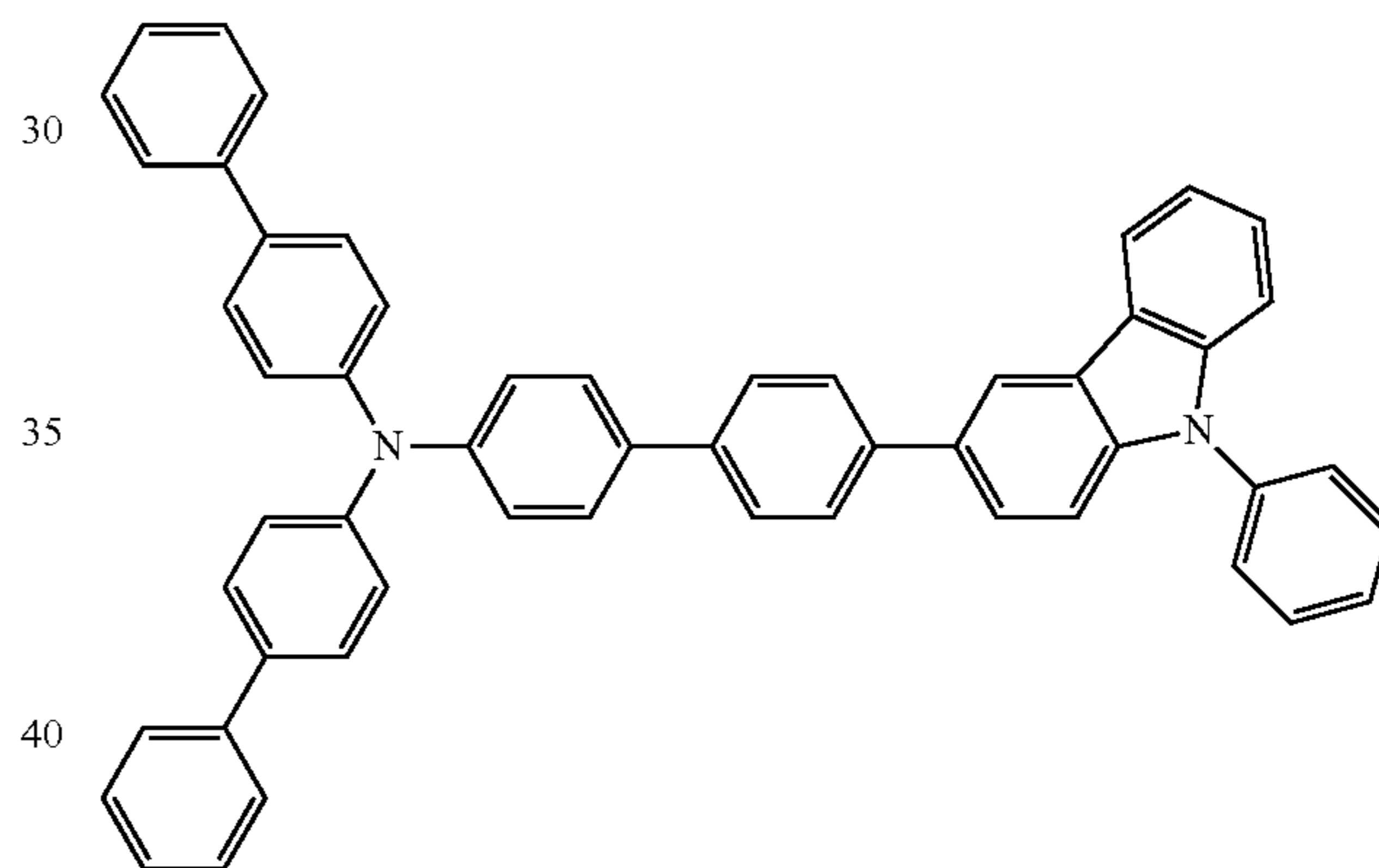
Compound B
