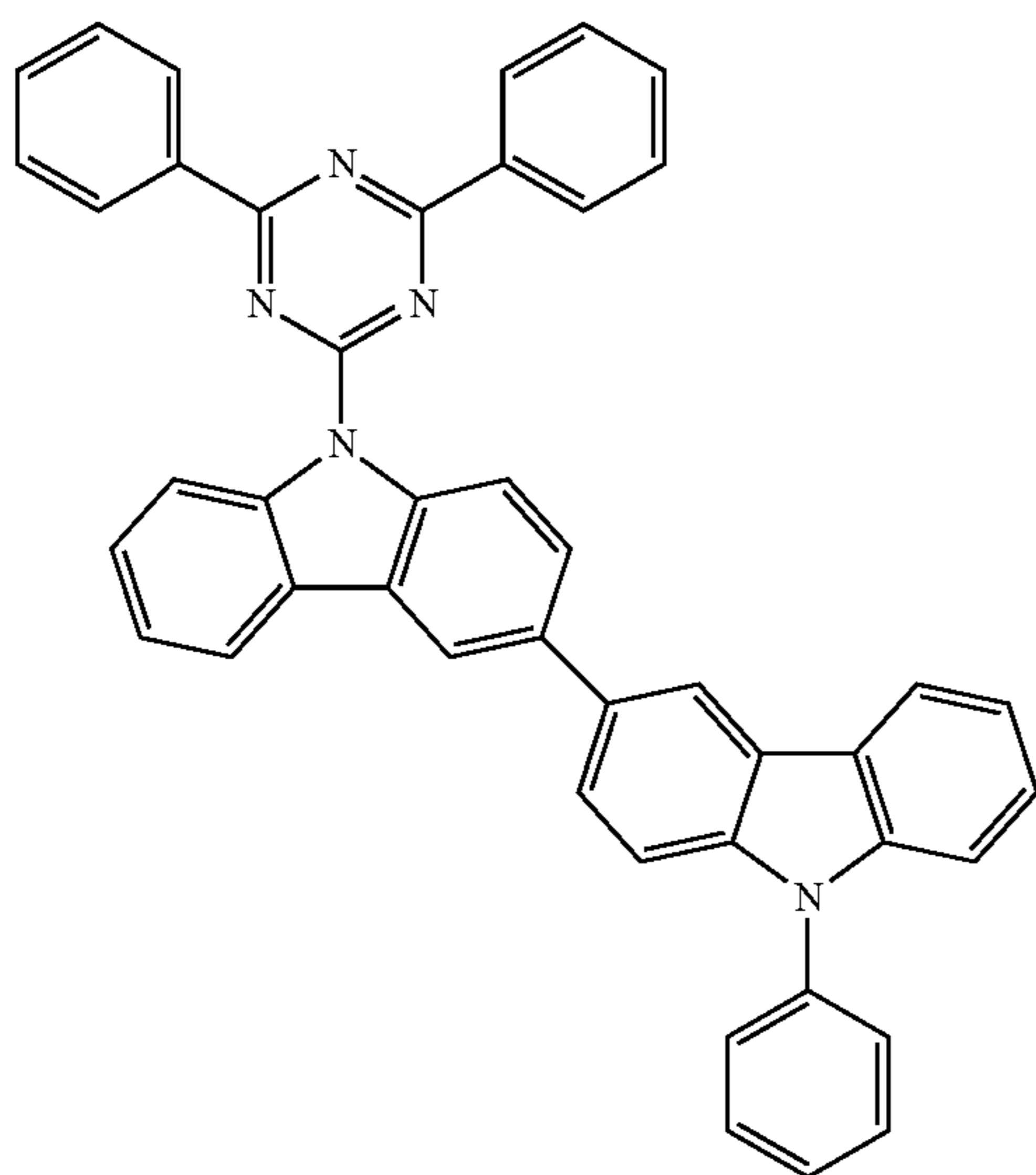
Compound 5
