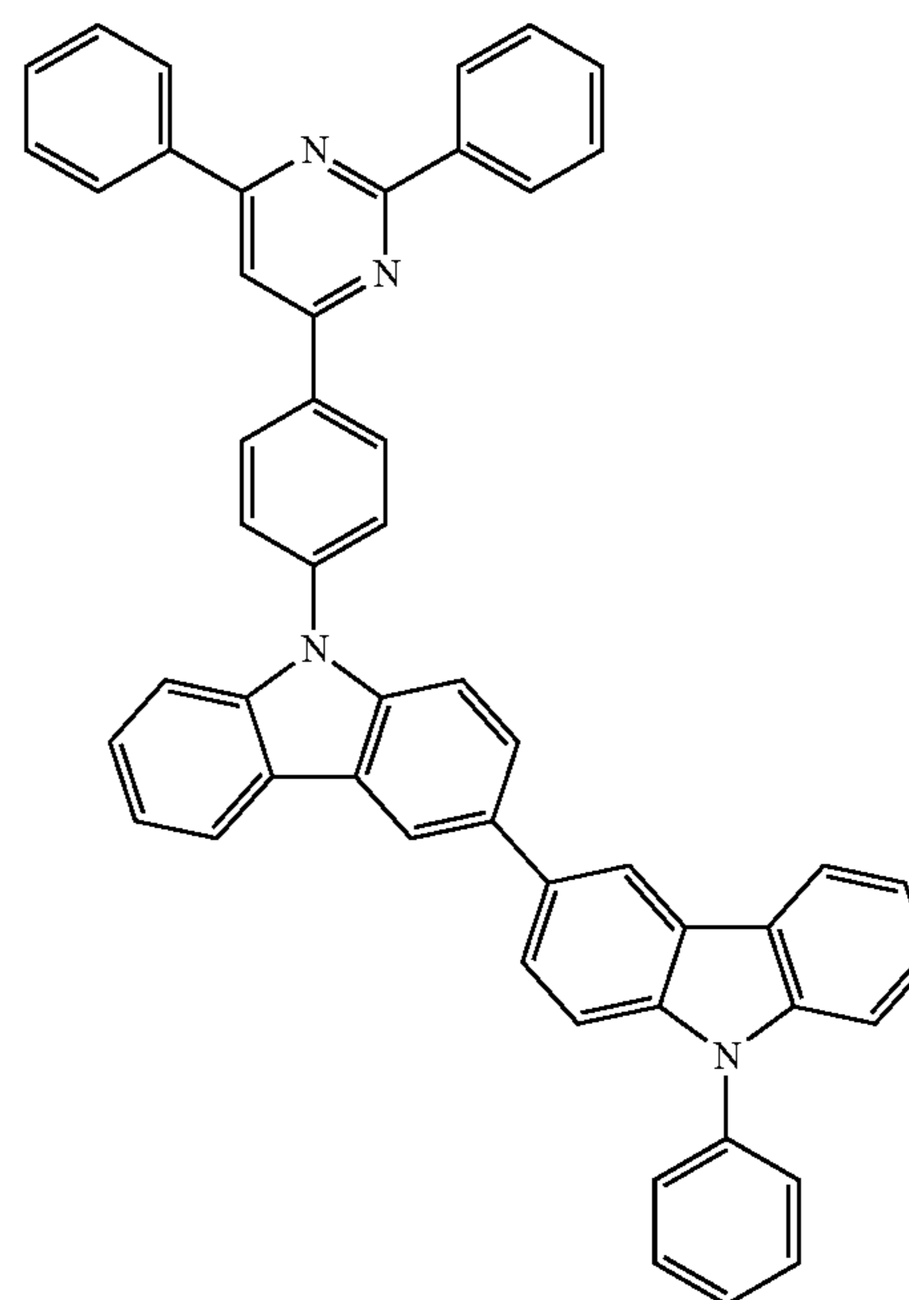
Compound 1
