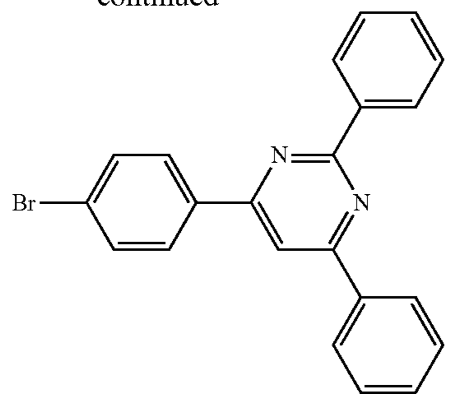
Intermediate body 1-2
