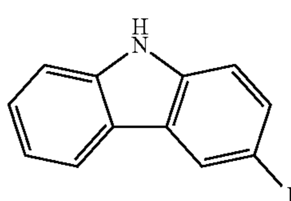
Intermediate body 1-3
