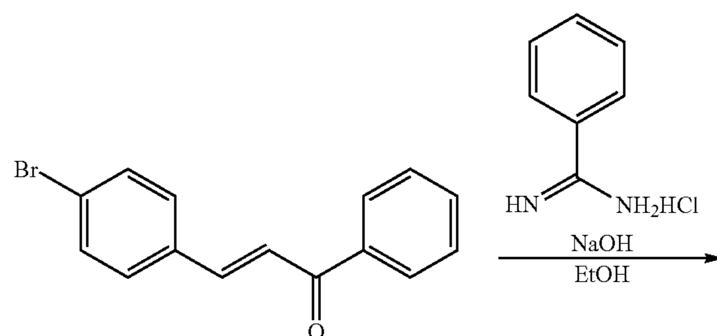
Intermediate body 1-1
