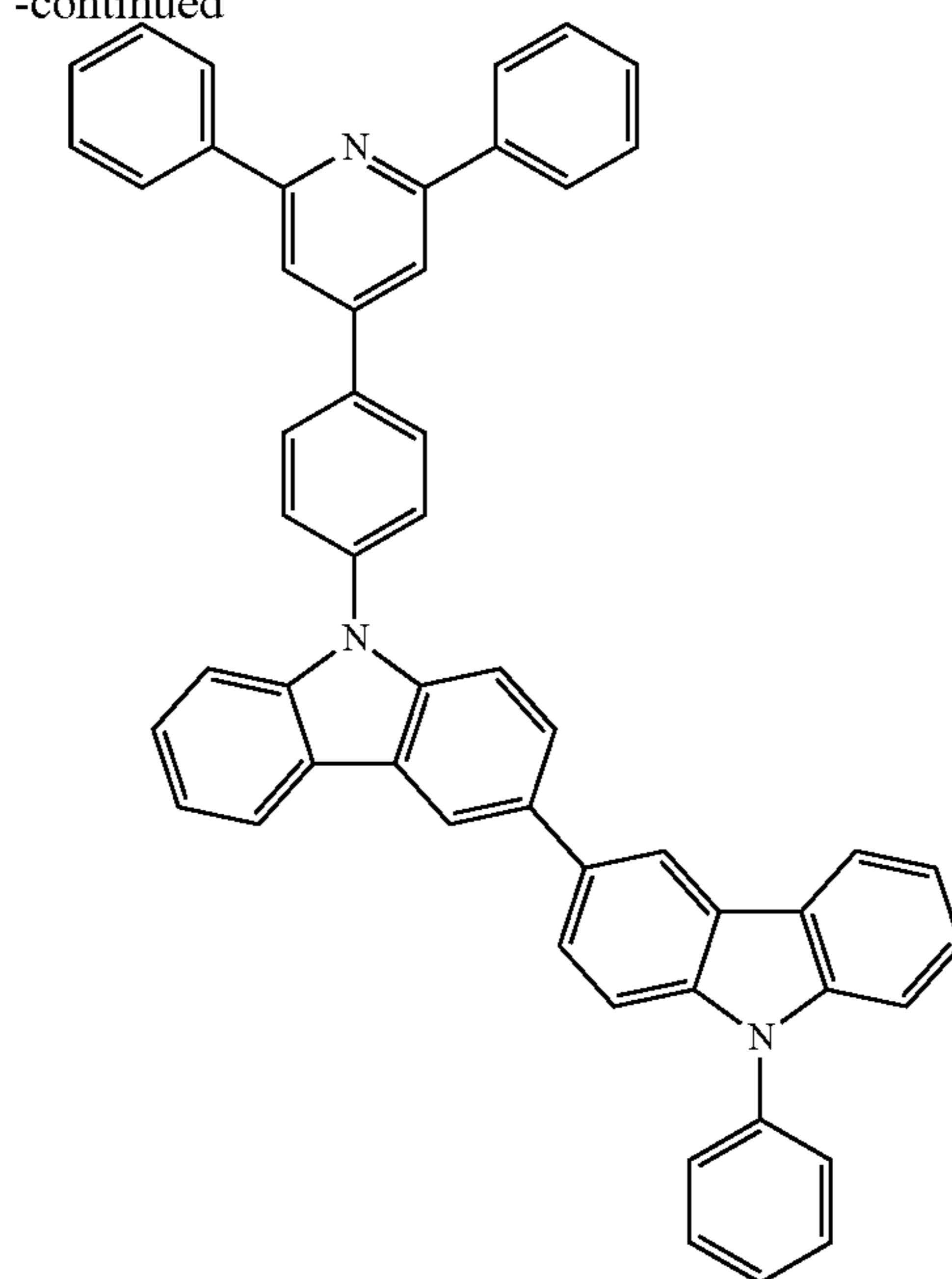
Compound 2
