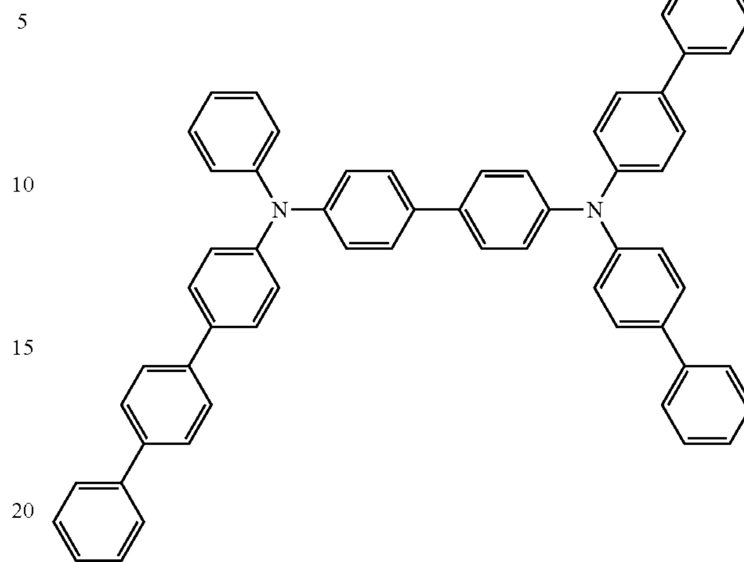
Compound A
