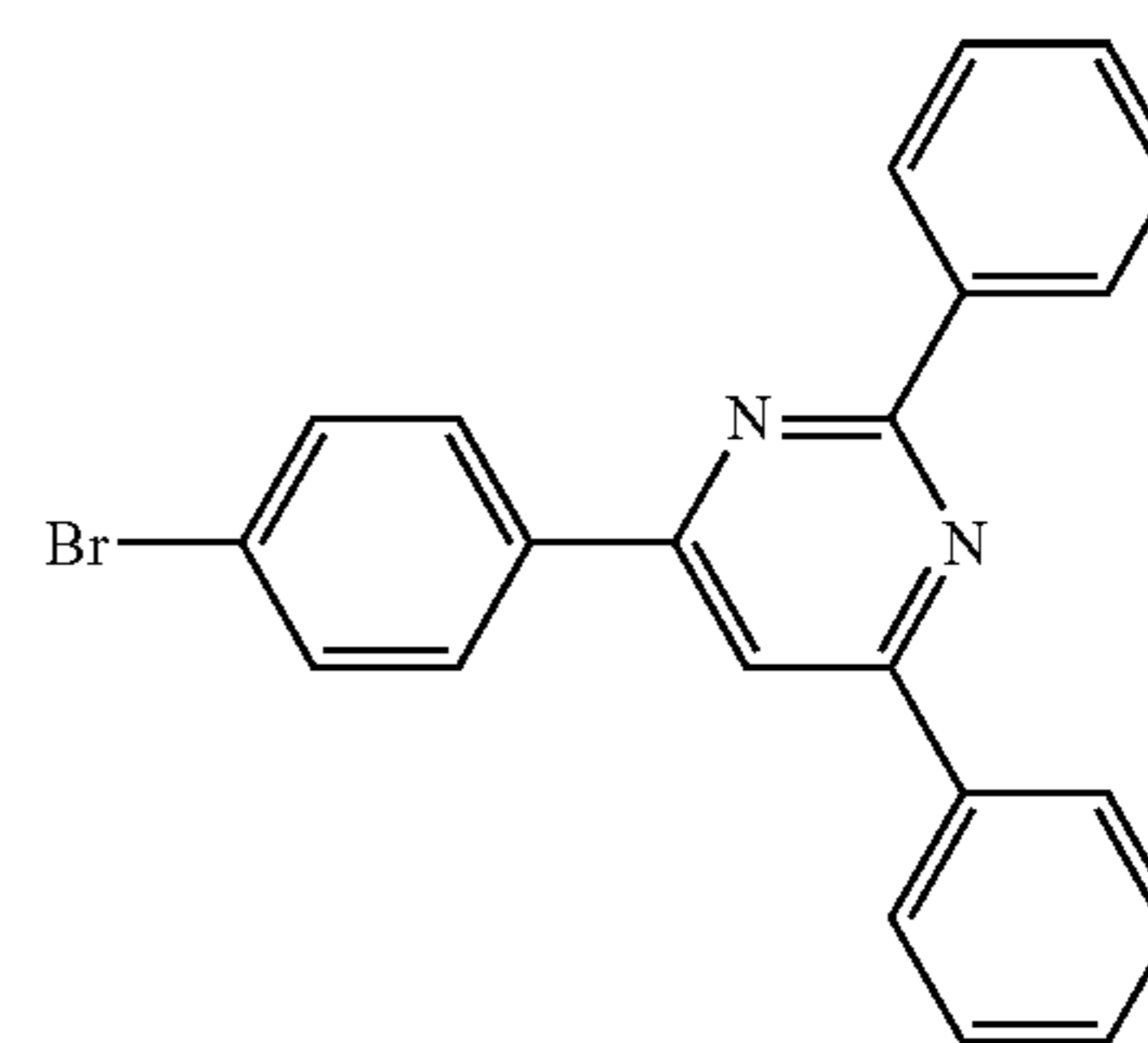
Intermediate body 1-2
