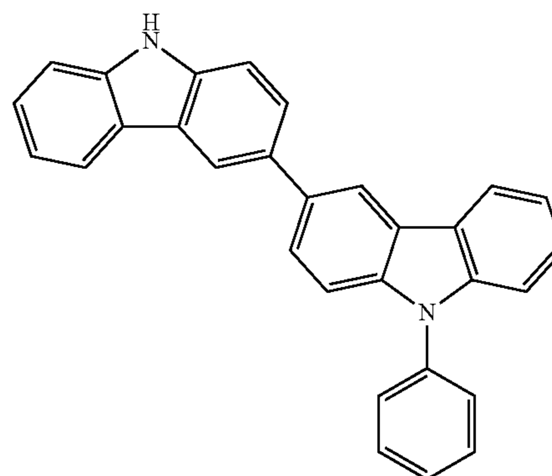
Intermediate body 1-4
