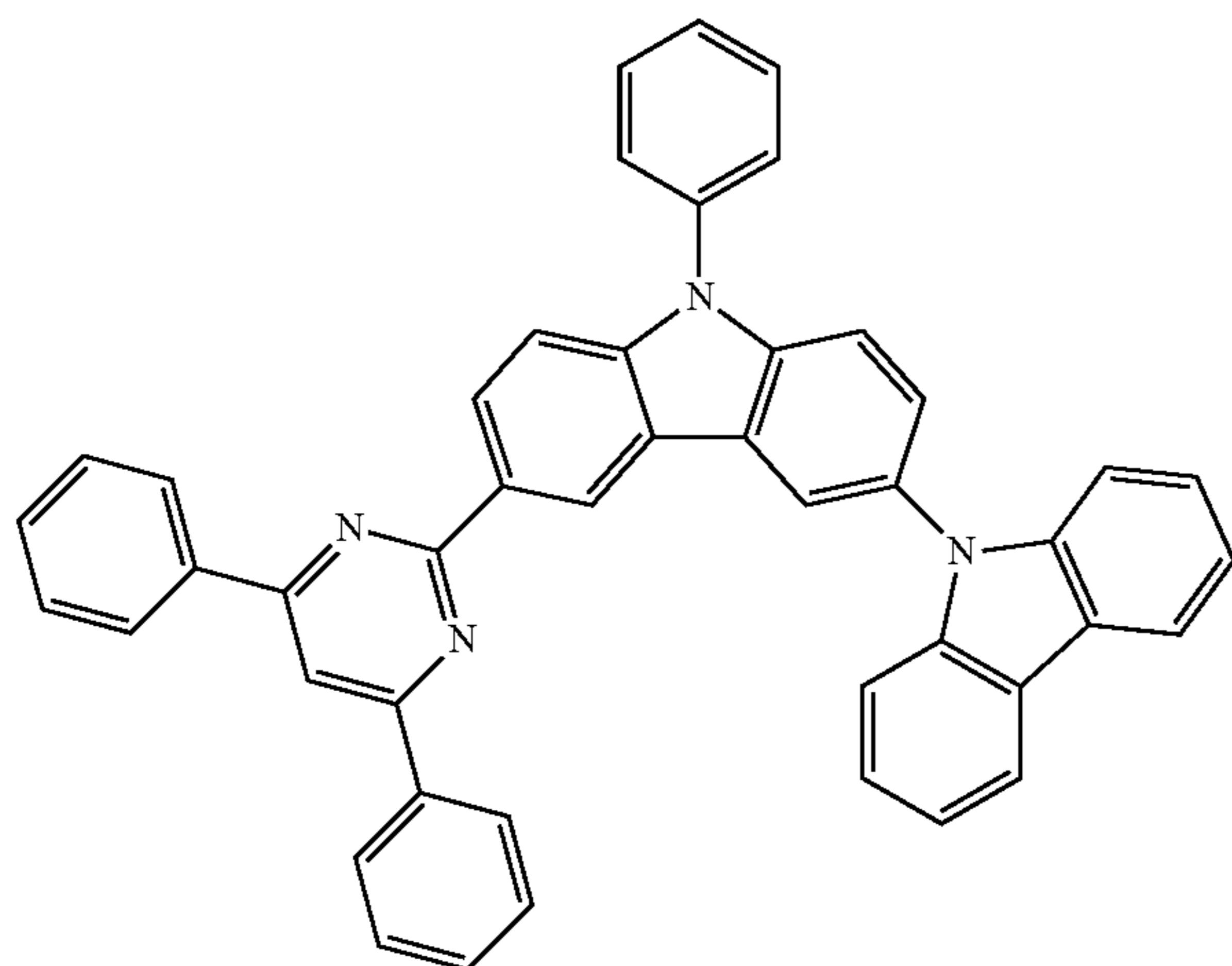
Compound G
