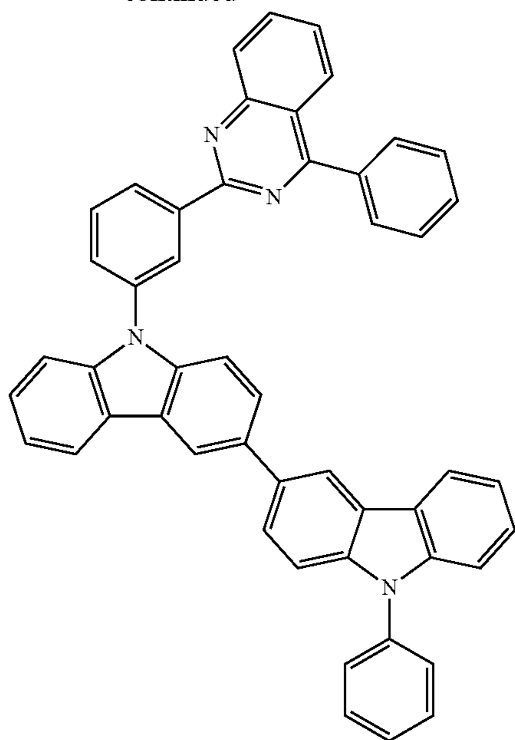
Compound 8
