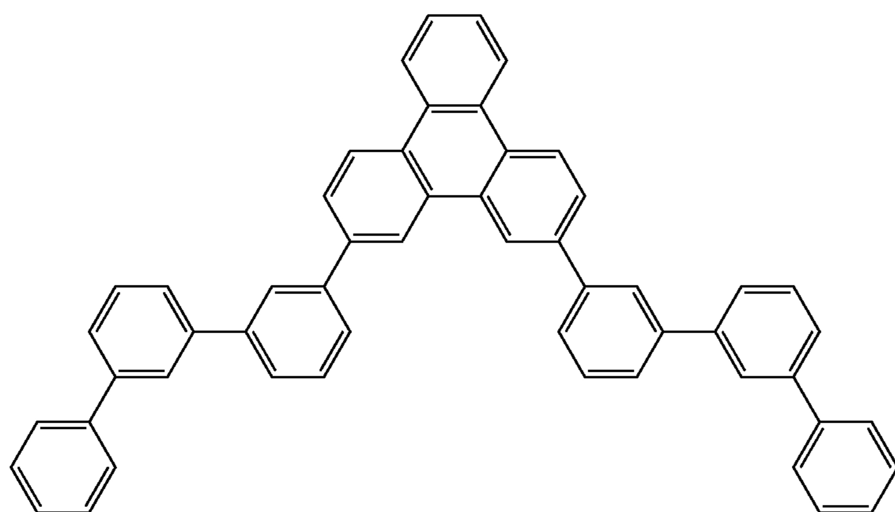
Compound 9
