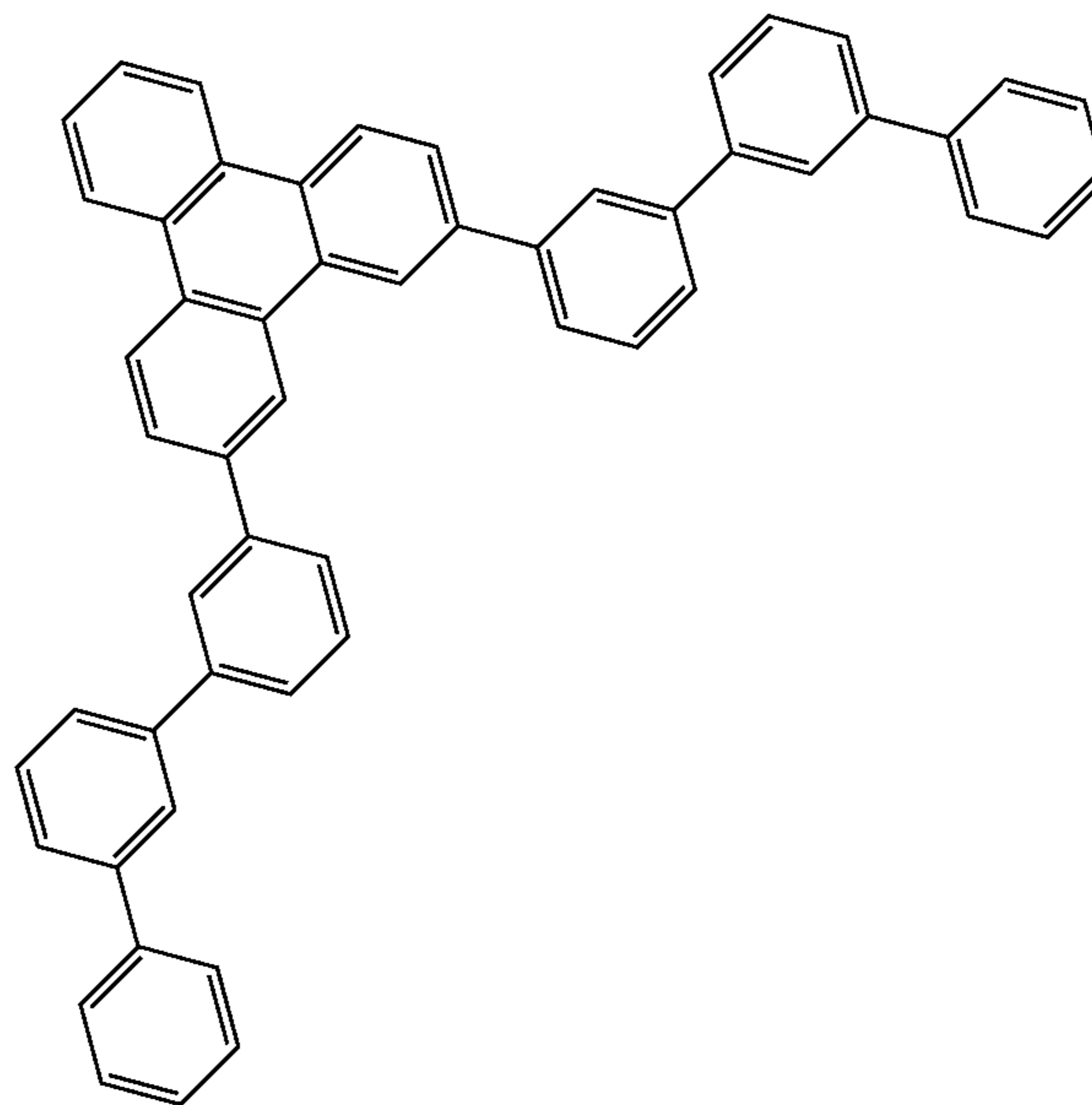
Compound 8
