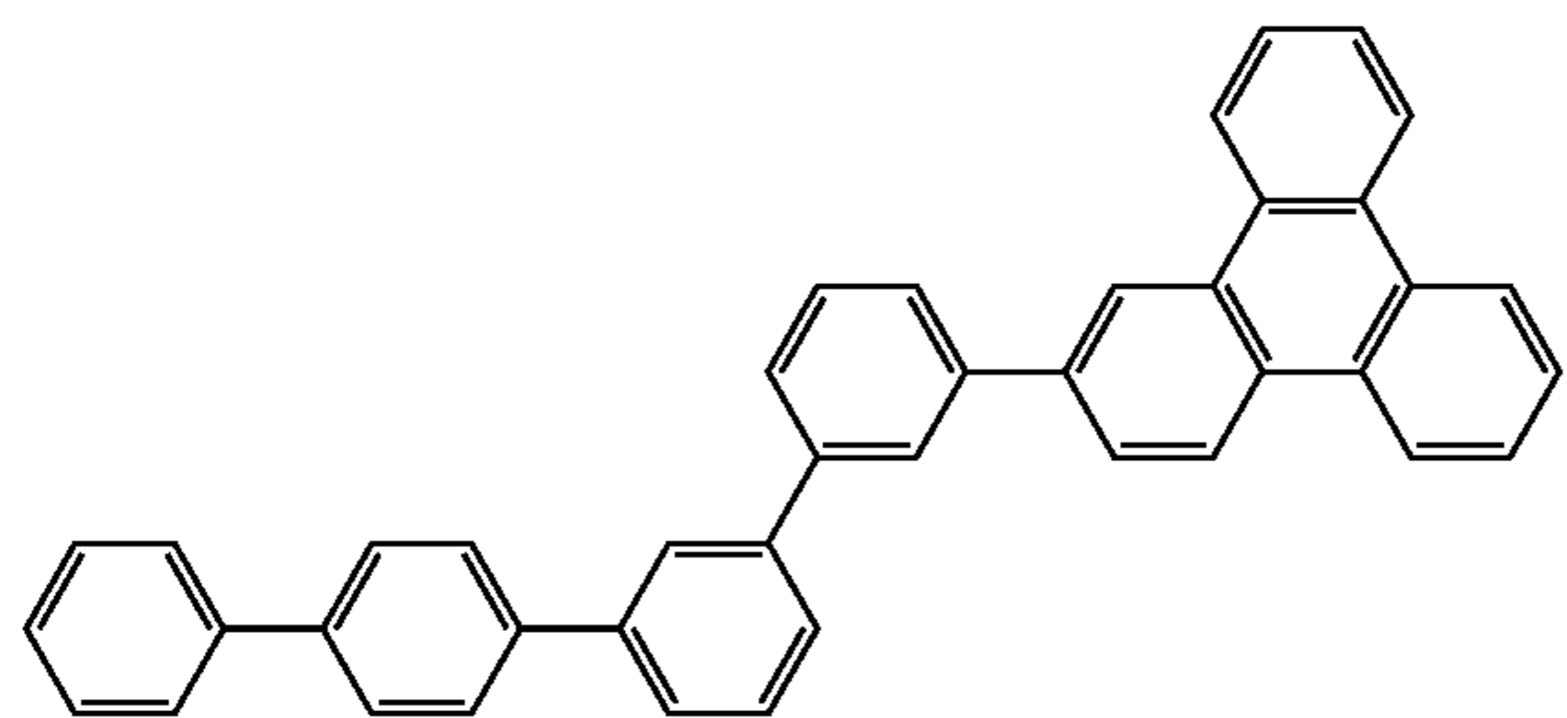
Compound 11
