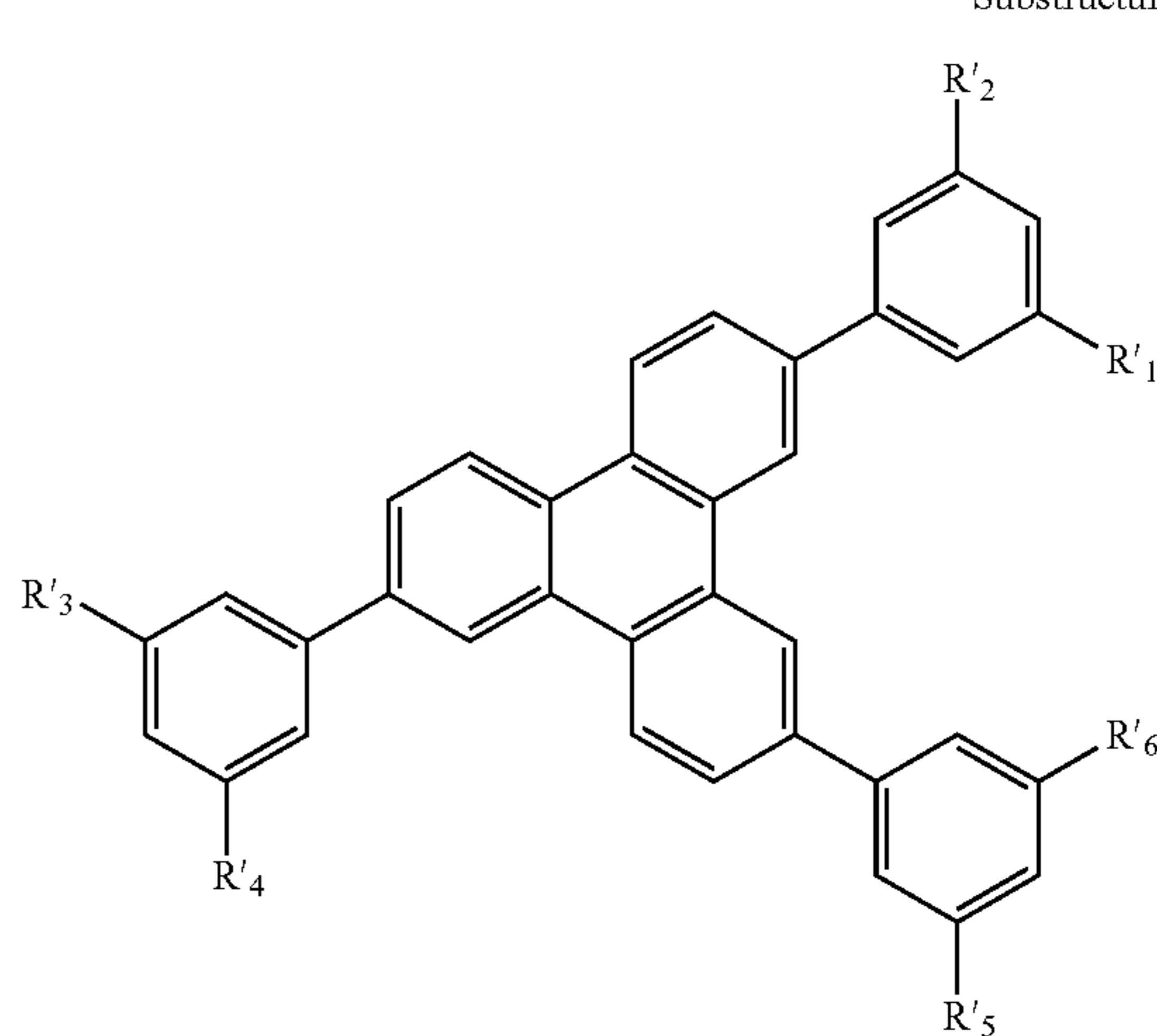
Substructure M
