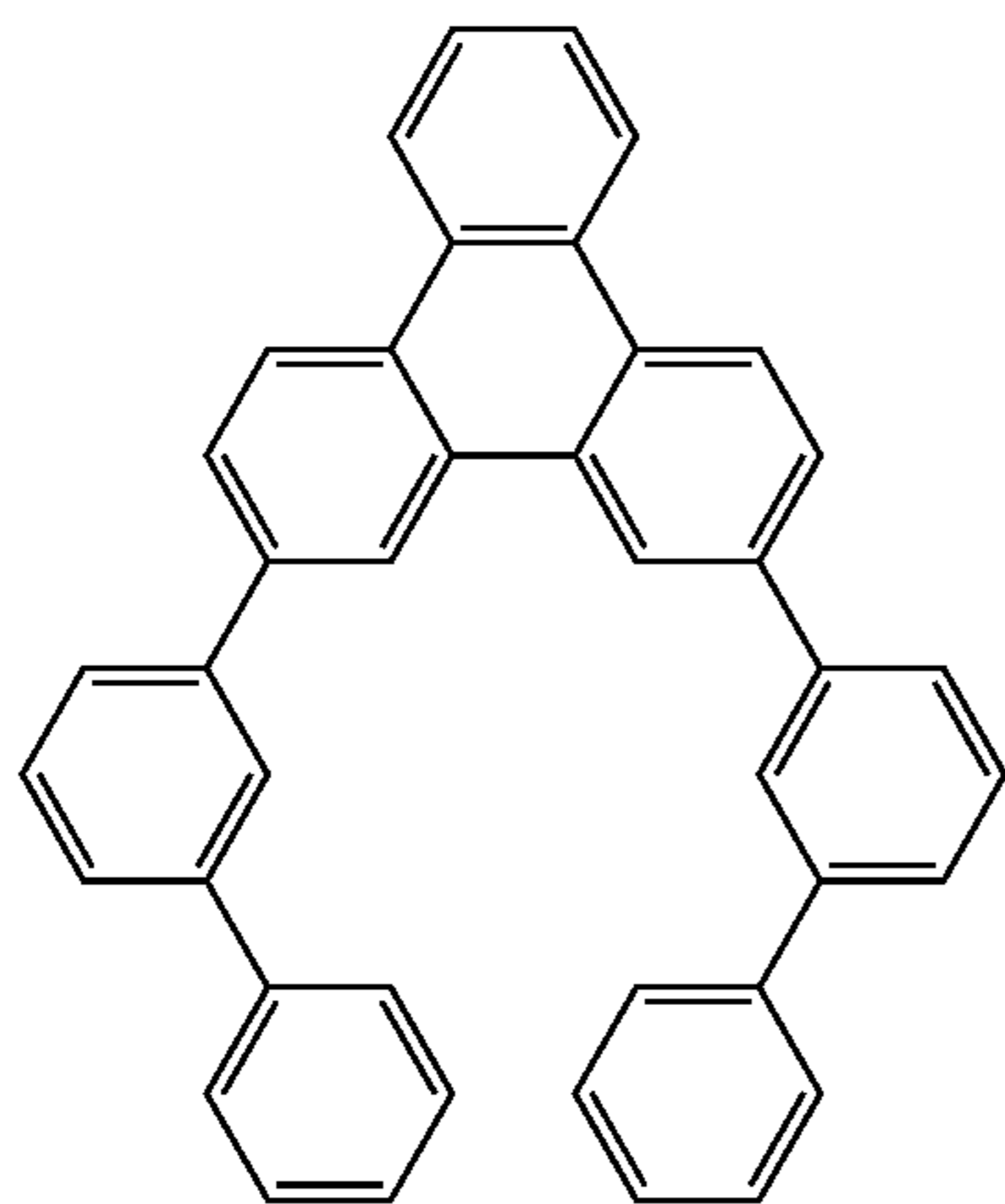
Compound 12 2,11-Di(phenyl-3-yl)triphenylene
