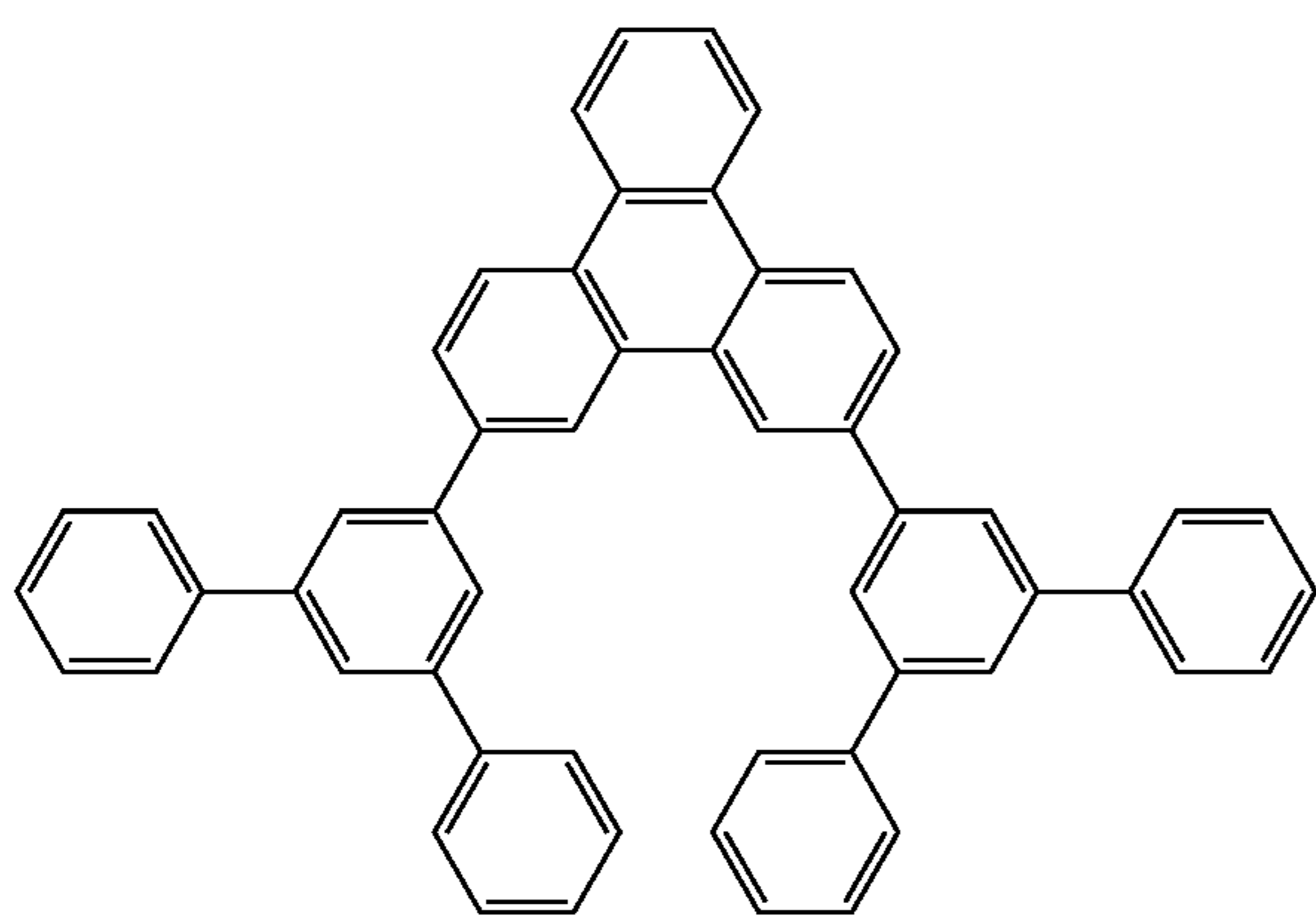
Compound 7
