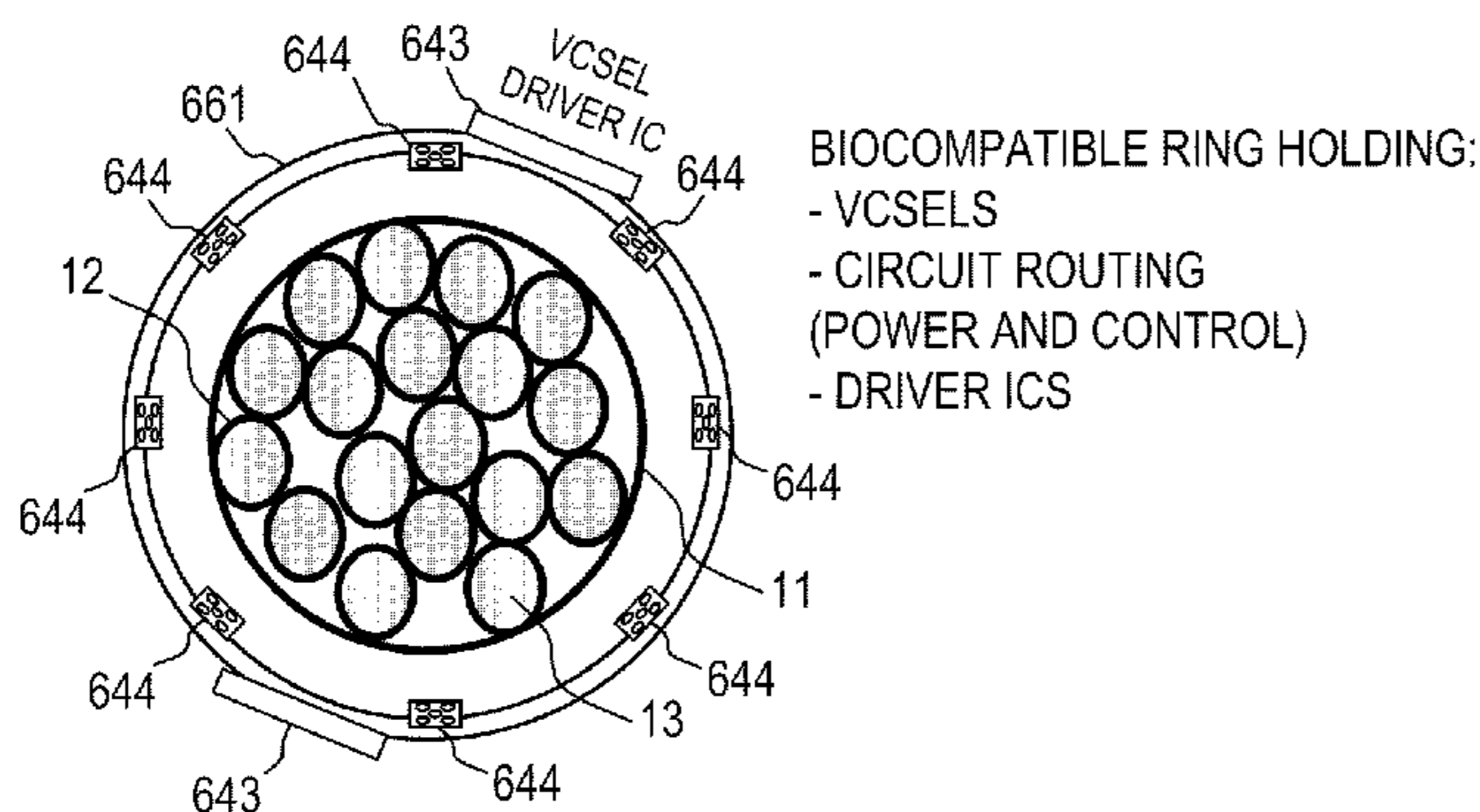
CIRCULAR CUFF OF VCSELS PACKAGED VCSEL
