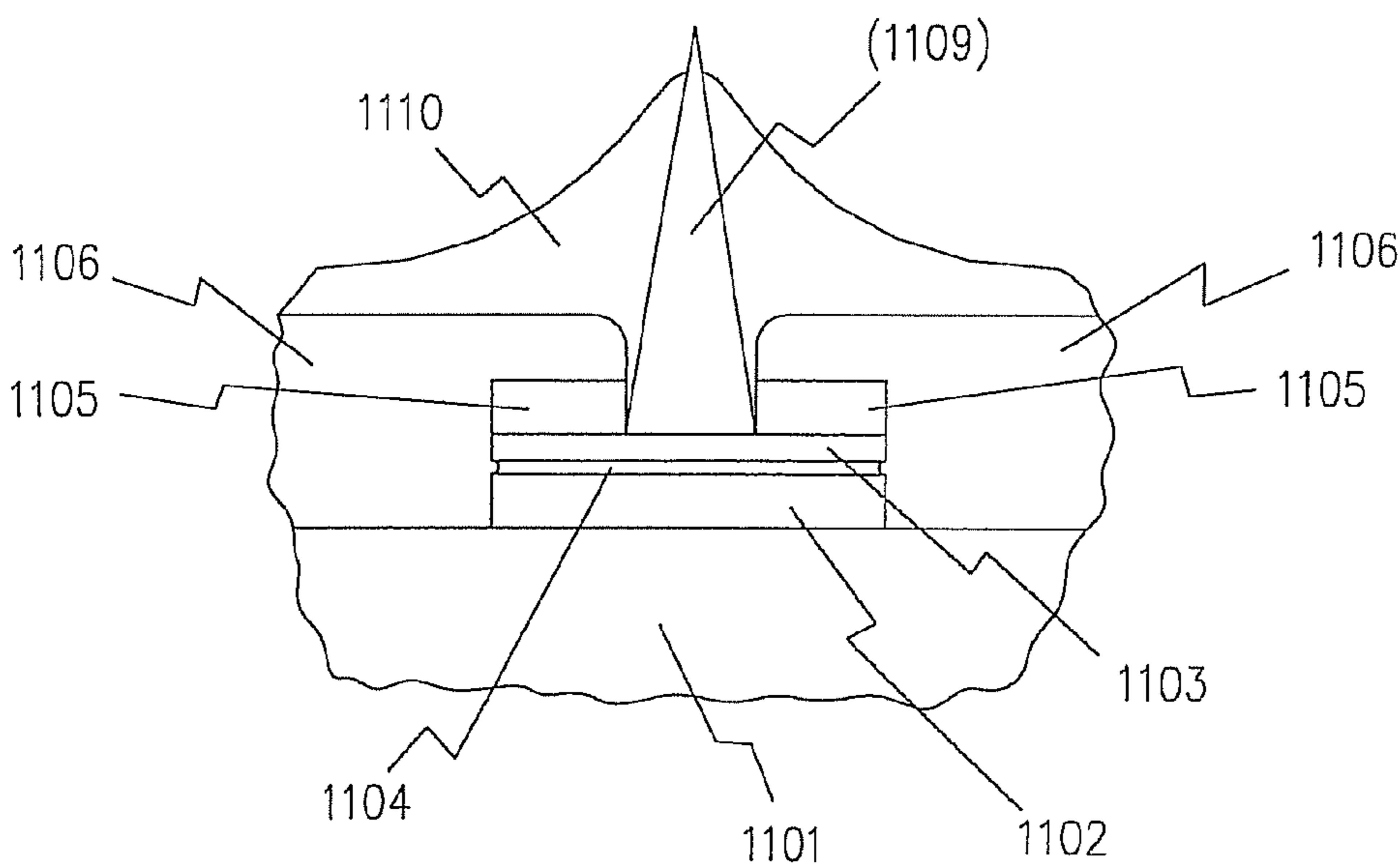
FIGURE 11b ELECTRODES
