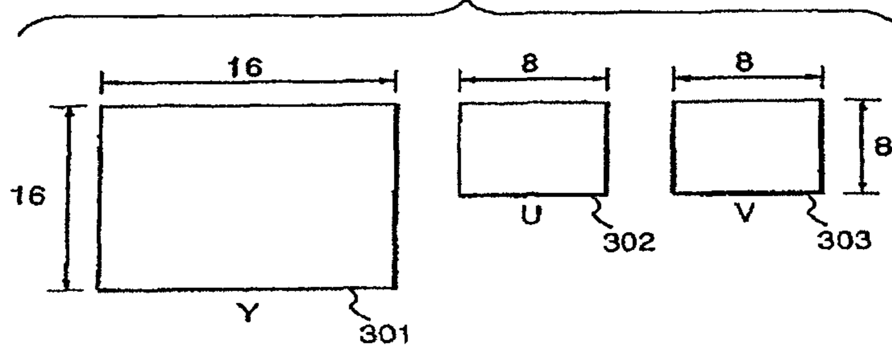
FIG. 3 (PRIOR ART)
