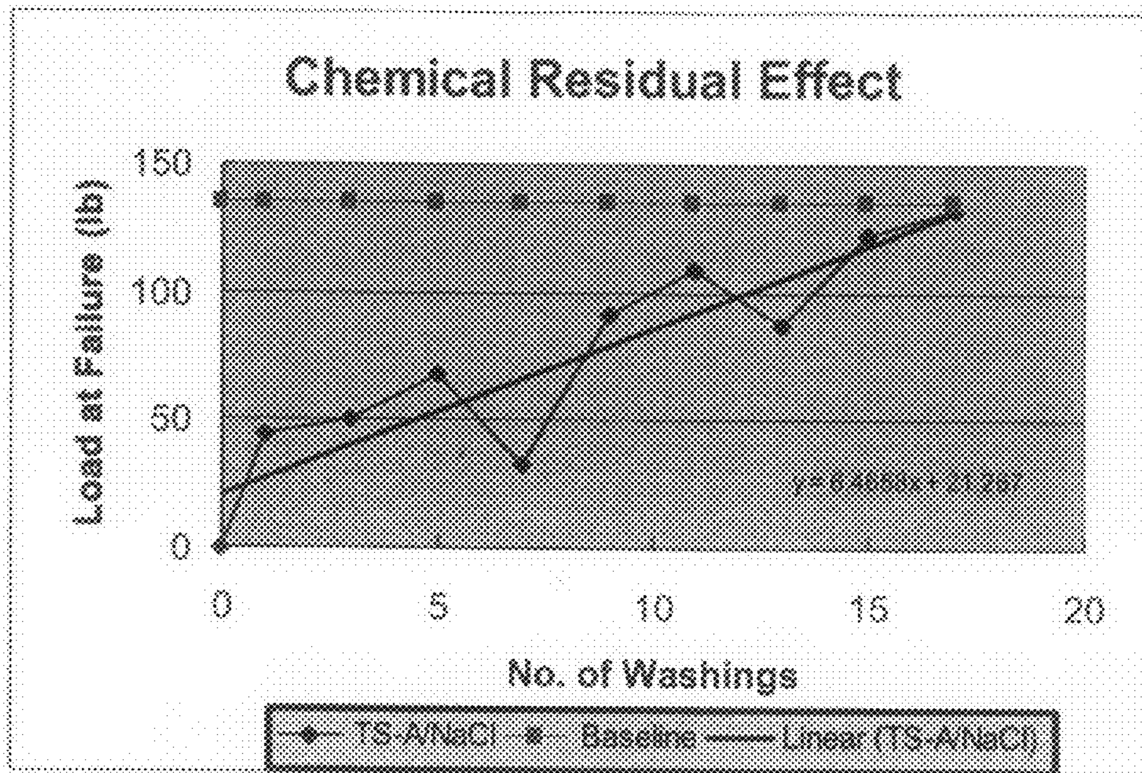
Figure 11. Bond Strength Reduction – TS-A/NaCl. Quarry Tile - Absorptivity = 0.27
