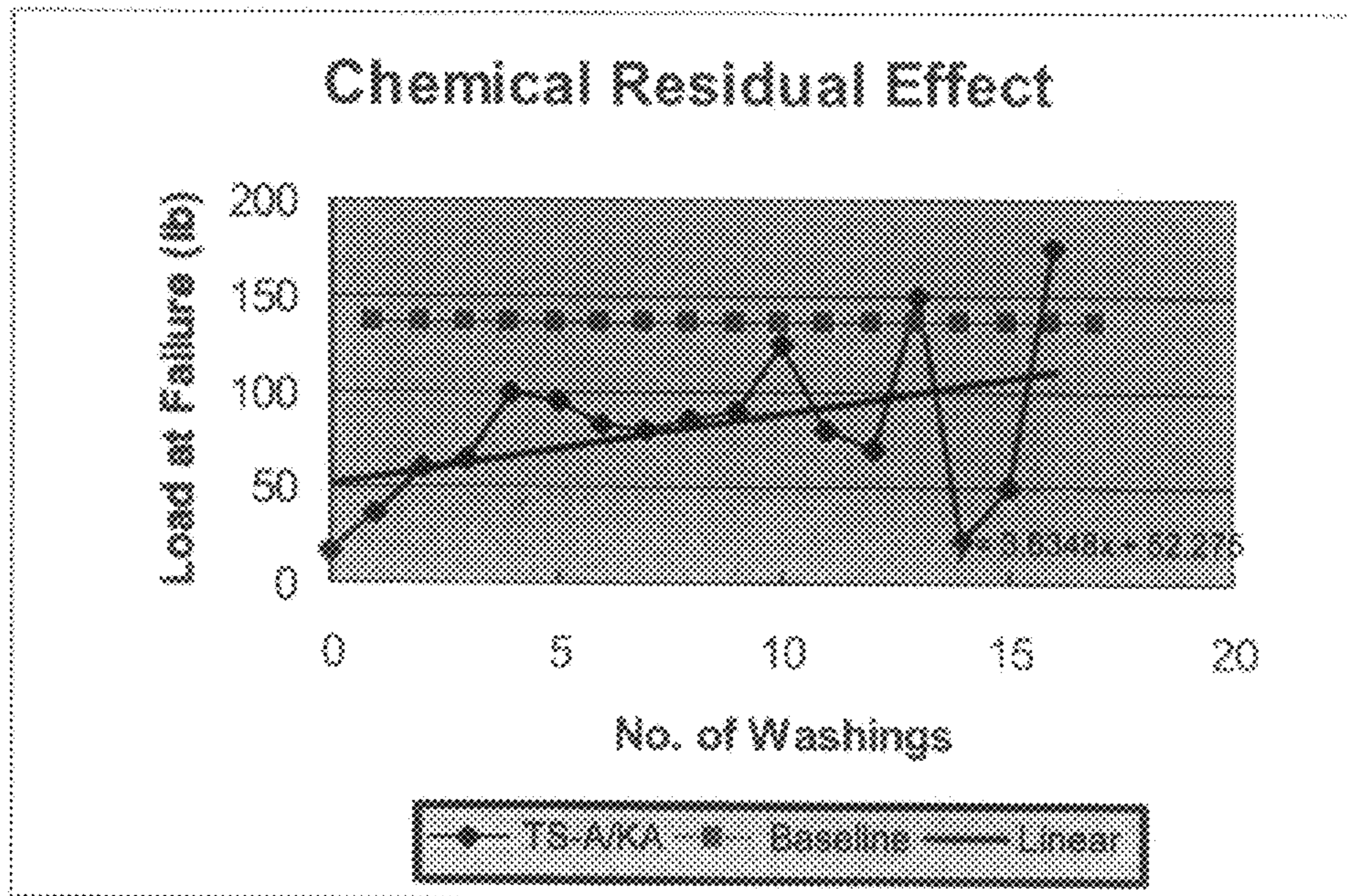
Figure 9. Bond Strength Reduction -- TS-A/KA. Quarry Tile - Absorptivity = 0.27
