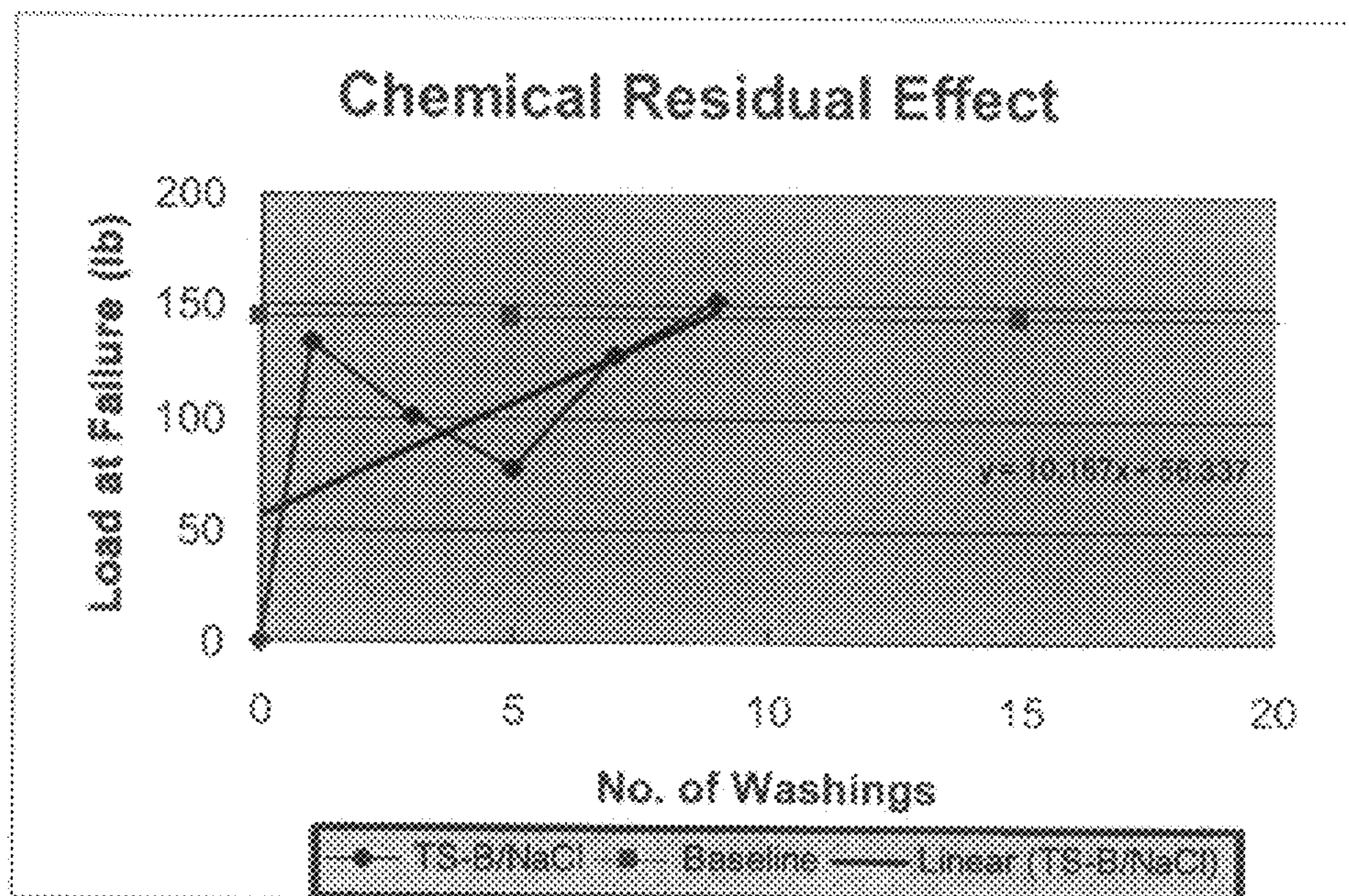
Figure 14. Bond Strength Reduction -- TS-B/NaCl. Levy Co. Slag - Absorptivity = 5.49
