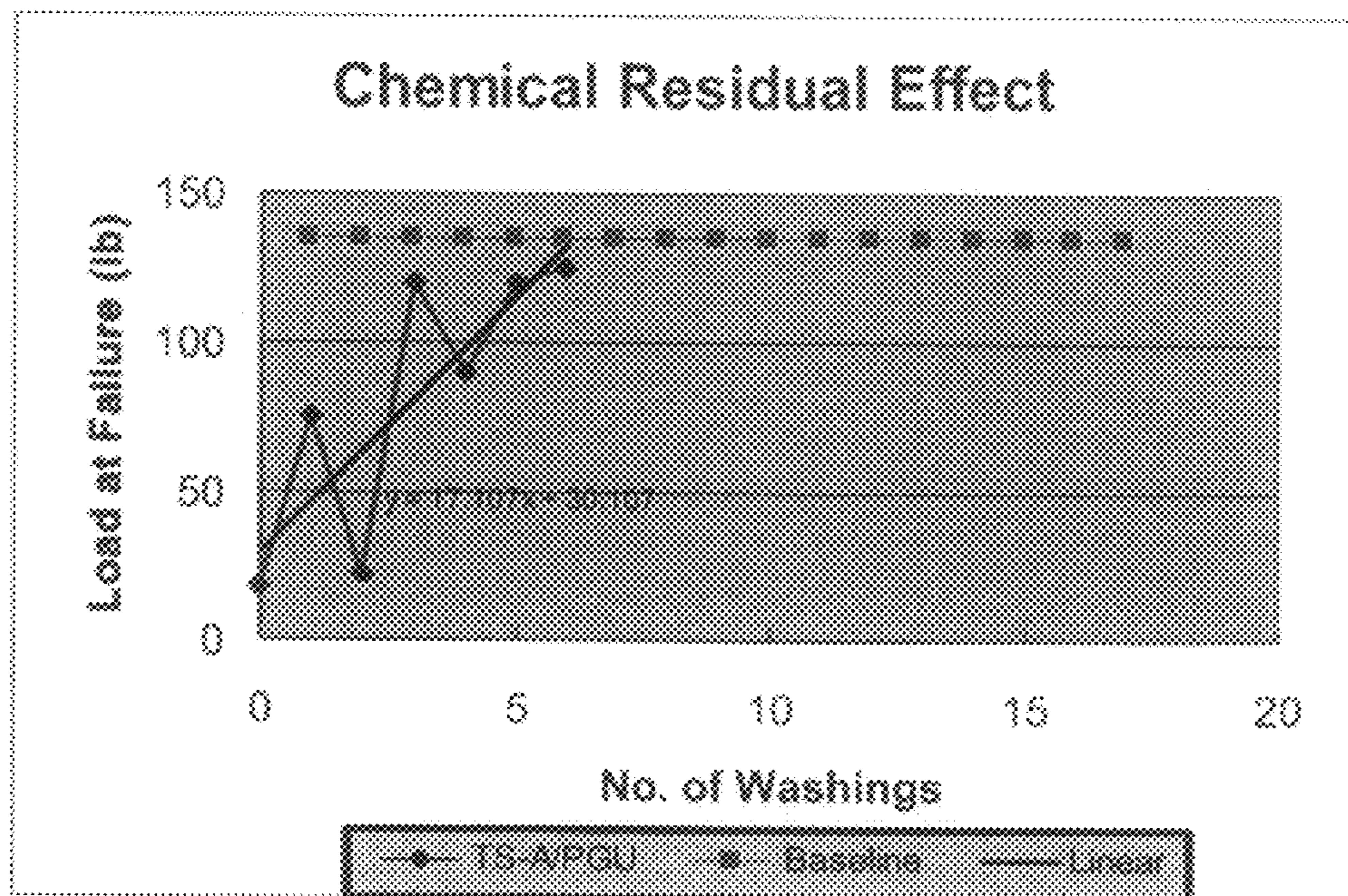
Figure 10. Bond Strength Reduction -- TS-A/PGU. Quarry Tile - Absorptivity = 0.27
