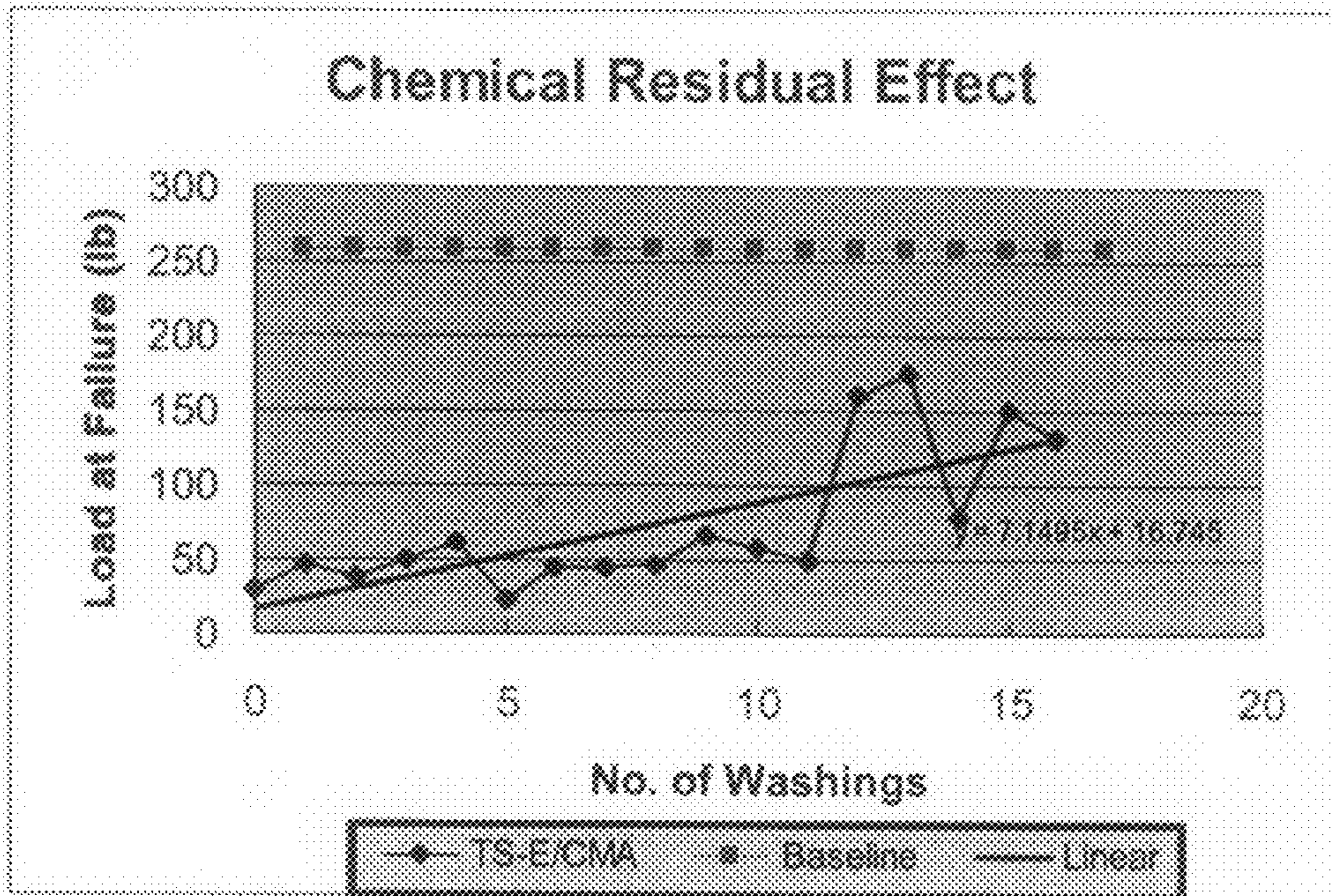
Figure 23. Bond Strength Reduction -- TS-E/CMA. Corps of Eng. Limestone - Absorptivity = 1.22
