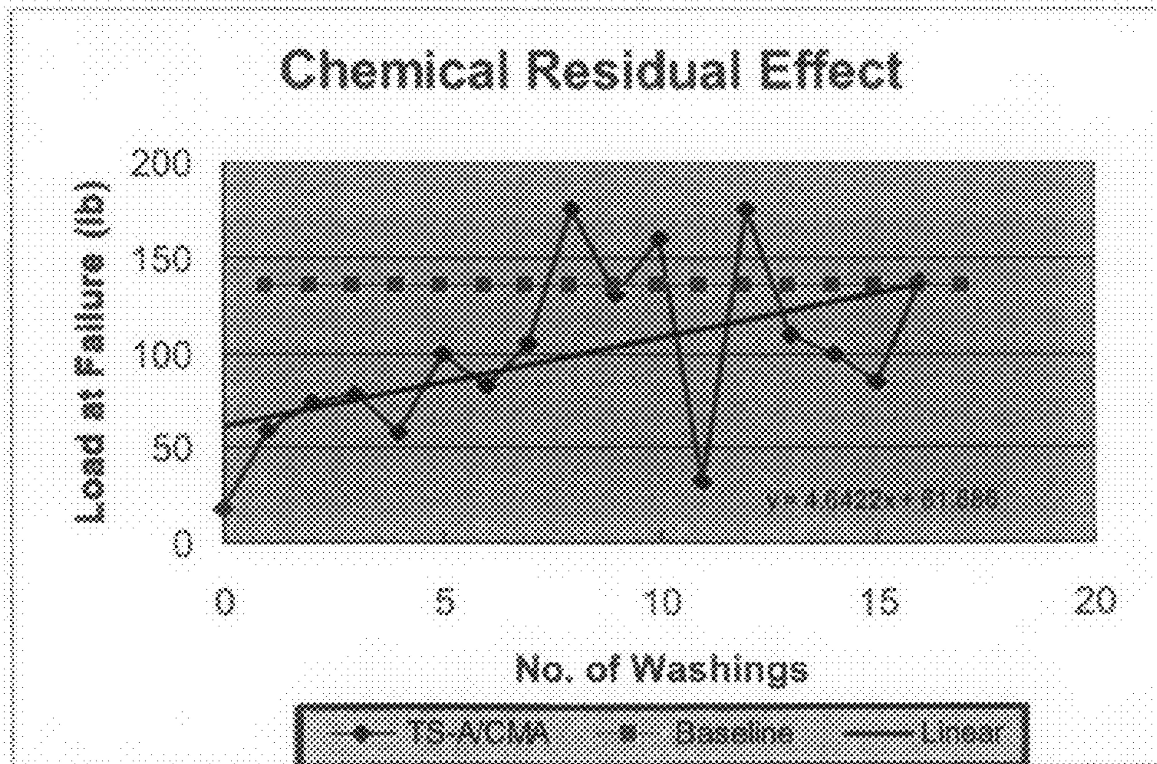
Figure 8. Bond Strength Reduction -- TS-A/CMA. Quarry Tile - Absorptivity = 0.27
