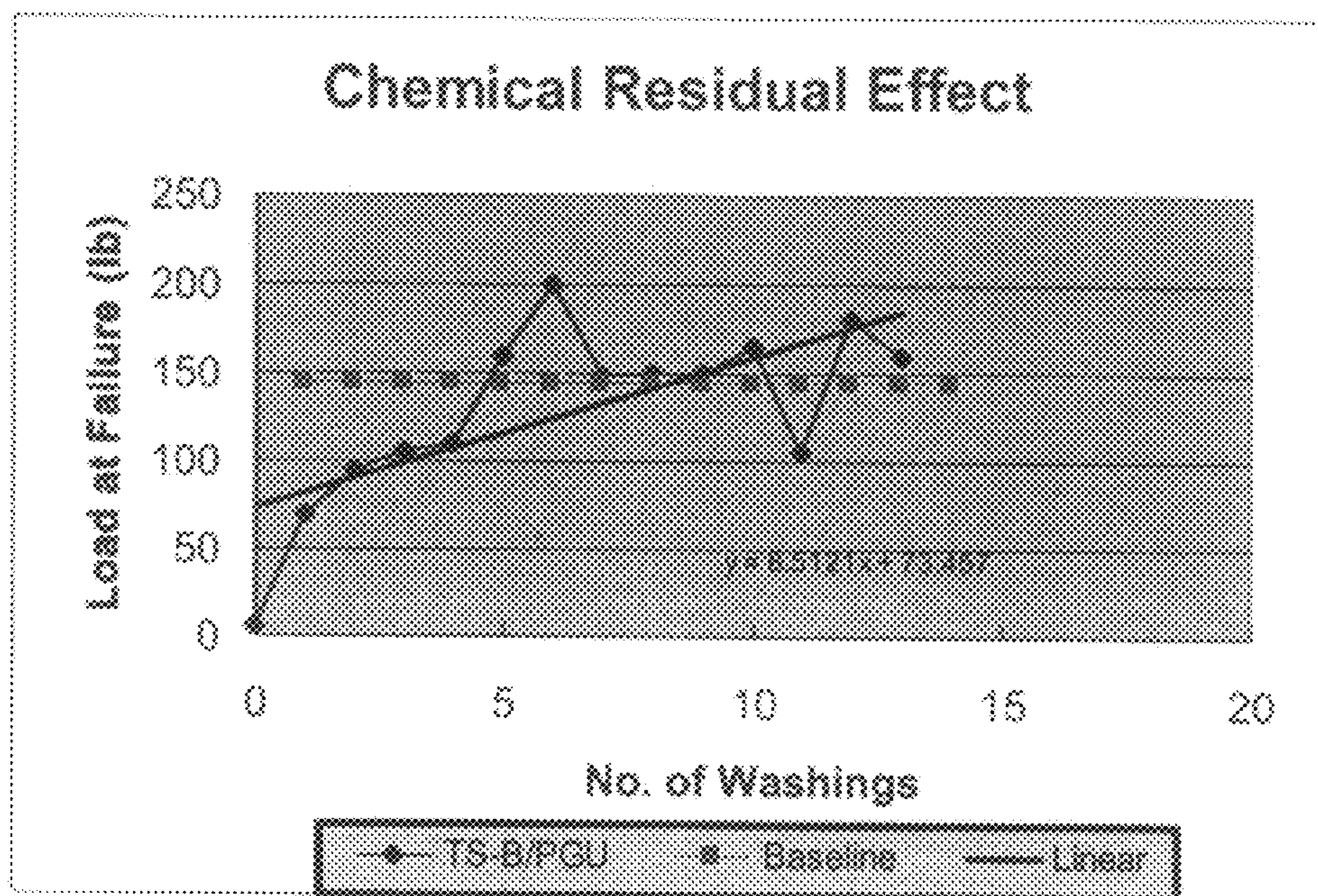
Figure 13. Bond Strength Reduction -- TS-B/PGU. Levy Co. Slag - Absorptivity = 5.49
