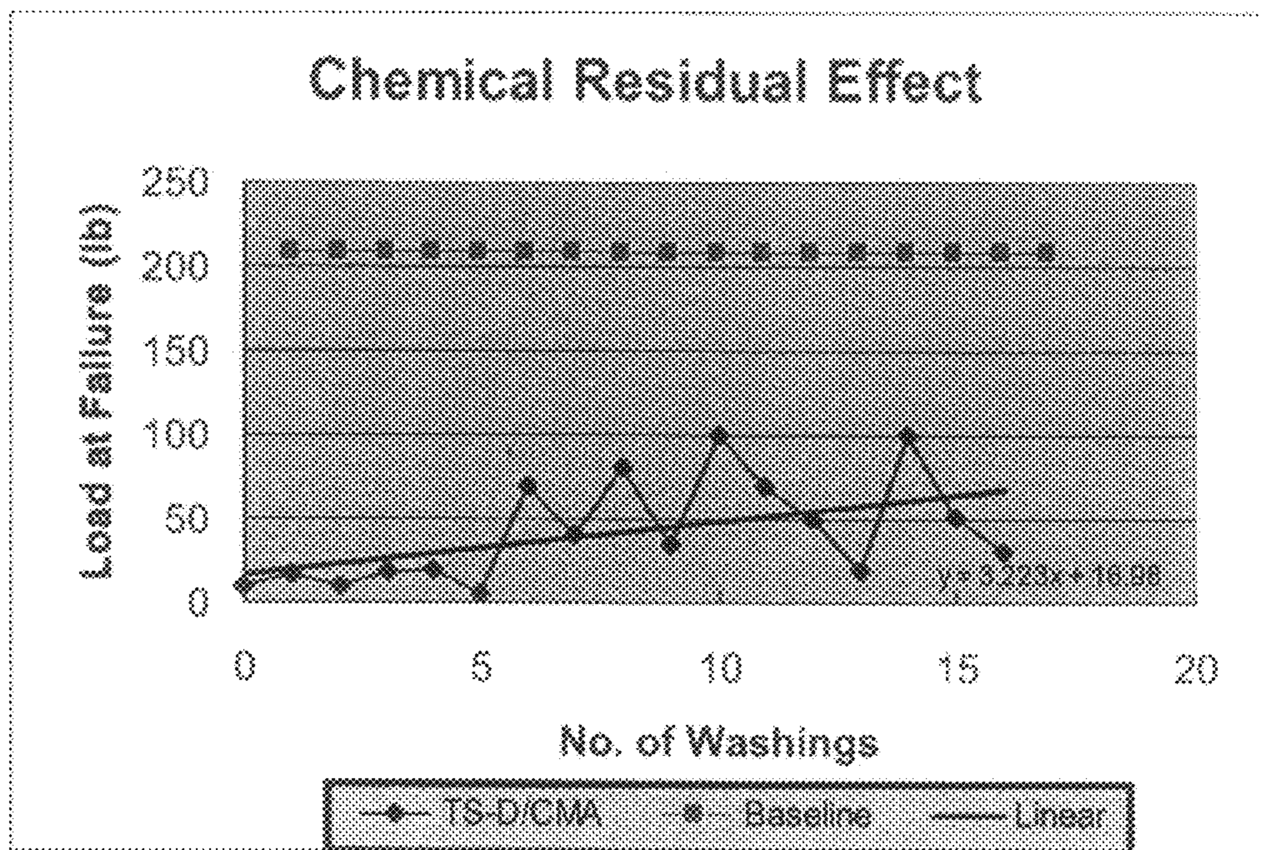
Figure 19. Bond Strength Reduction -- TS-D/CMA. Turunen, Inc. Limestone - Absorptivity = 1.73
