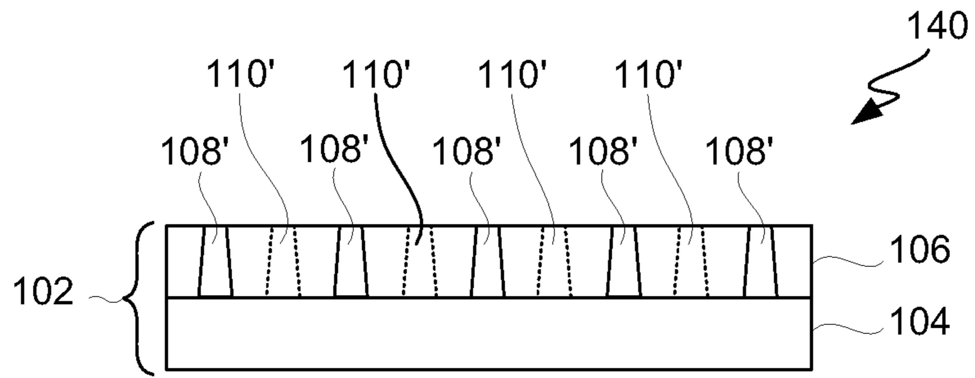
FIG. 1D
