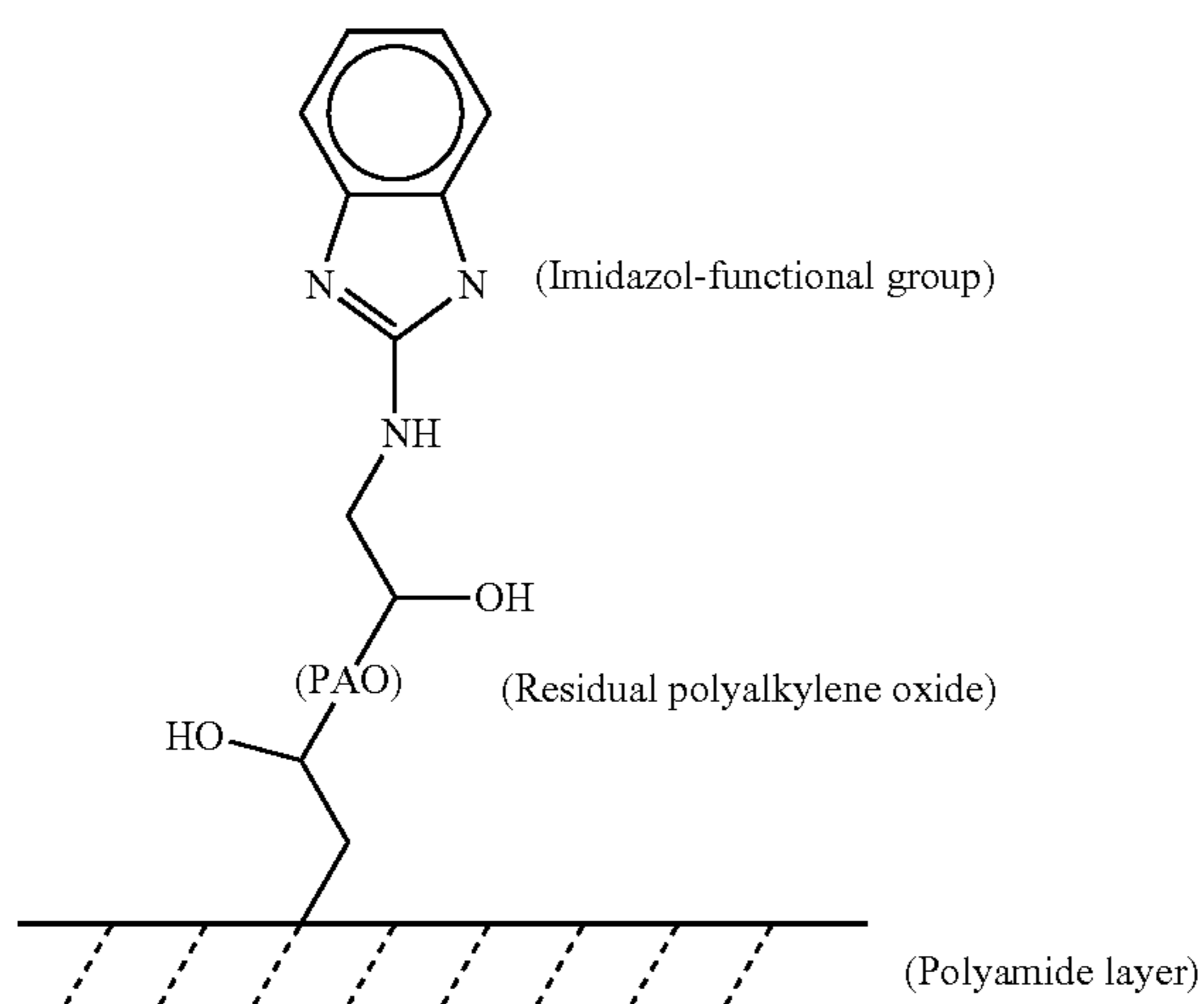
Formula (IV):
