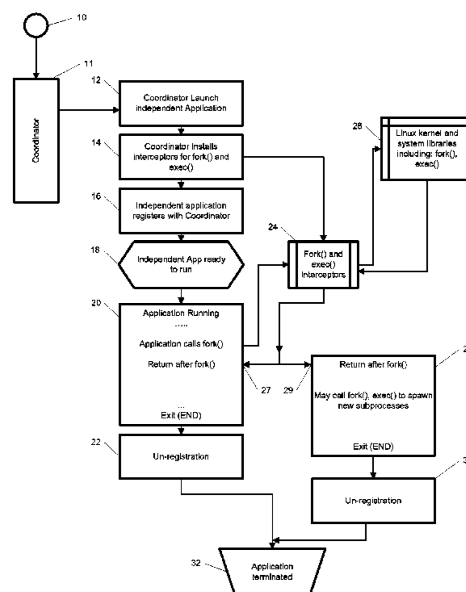
Core operation of fork()
