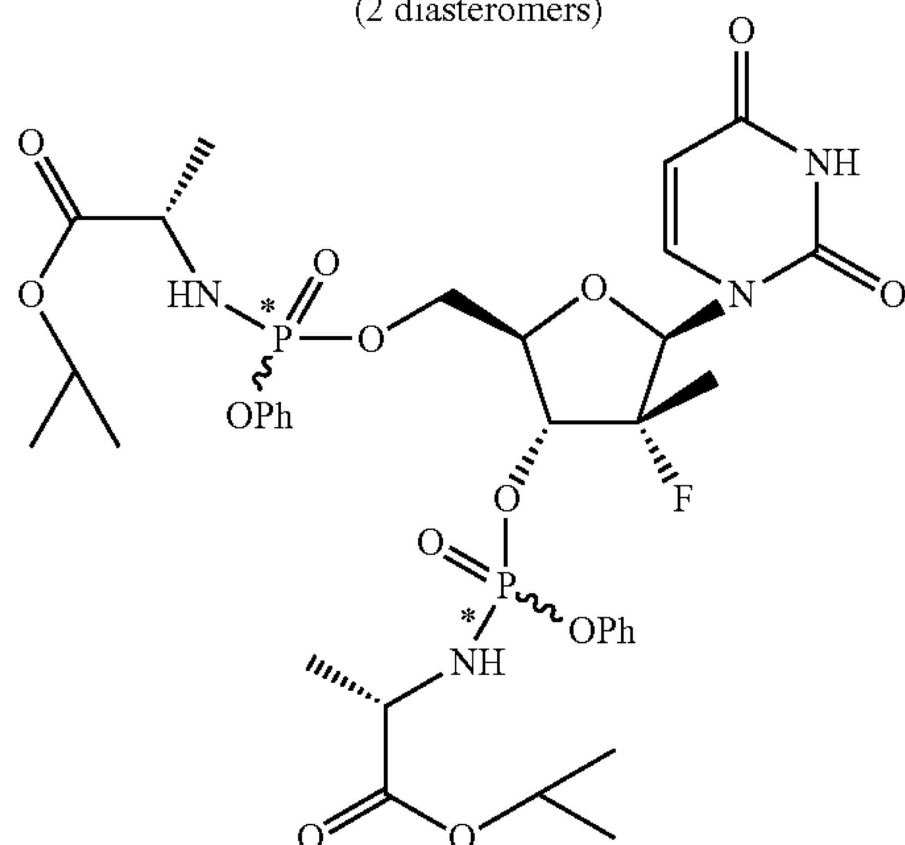
3',5'-bis-O-phosphoramidate (4 diastereomers)
