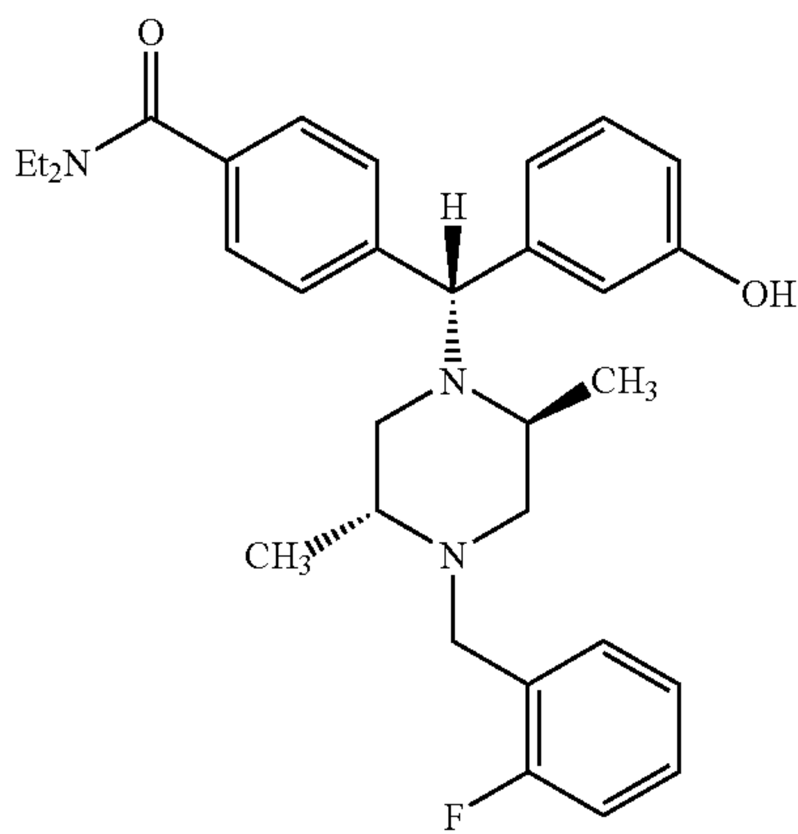
4-((Alpha-R)-Alpha-((2S,5R)-2,5-Dimethyl-4-(2-fluorobenzyl)-1-piperazinyl)-3-hydroxybenzyl)-N,N-diethylbenzamide
