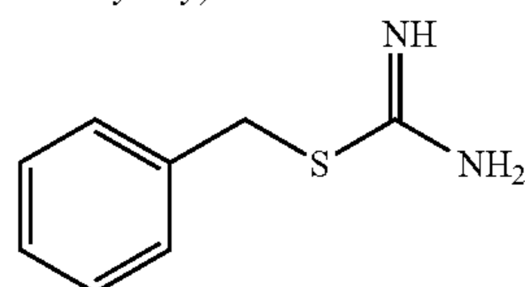
benzyl carbamimidothioate
