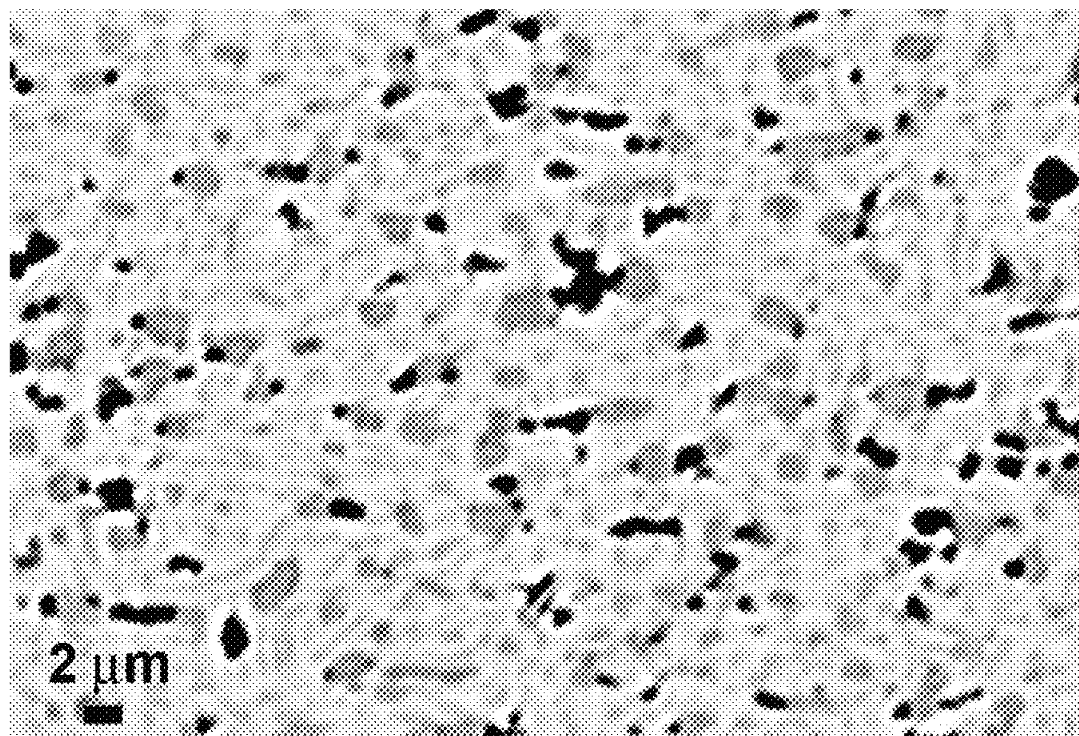
FIG. 63 The backscattered SEM micrograph of the gage microstructure of Alloy 20 specimen after tension at 700°C with tensile elongation of 88.5%.
