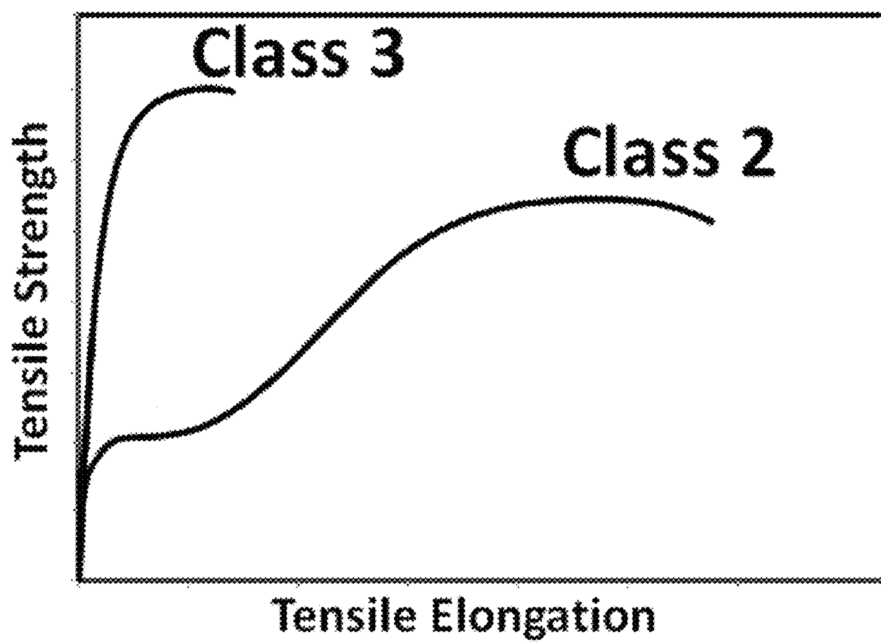
FIG. 6B Mechanical response of Class 3 steel upon tension at room temperature as compared to Class 2 steel.
