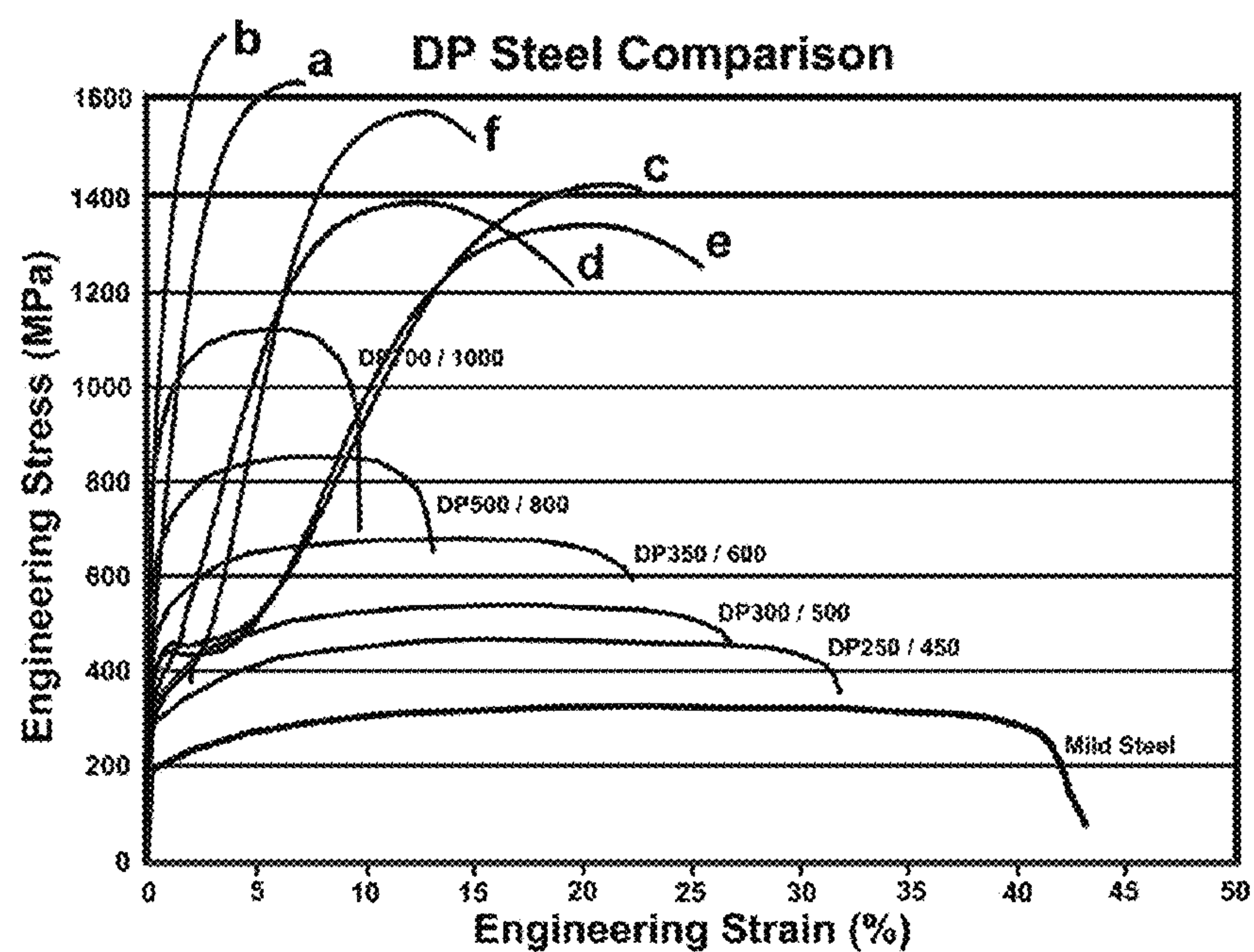
FIG. 9 Comparison of stress-strain curves of new non-stainless steel sheet types with existing Dual Phase (DP) steels.
