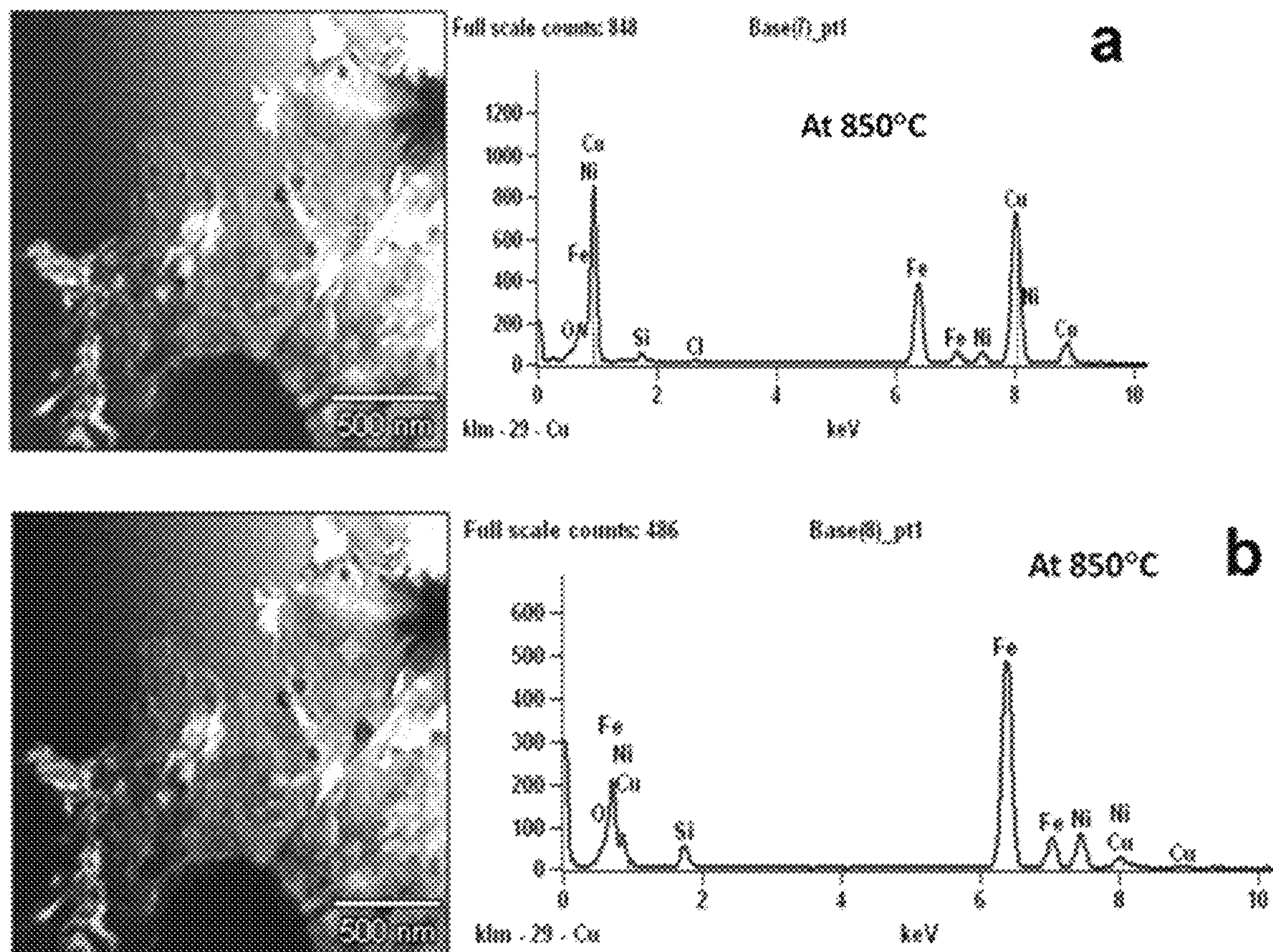
FIG. 69 TEM EDS analysis on the nano-precipitates formed in the Alloy 20 specimens.
