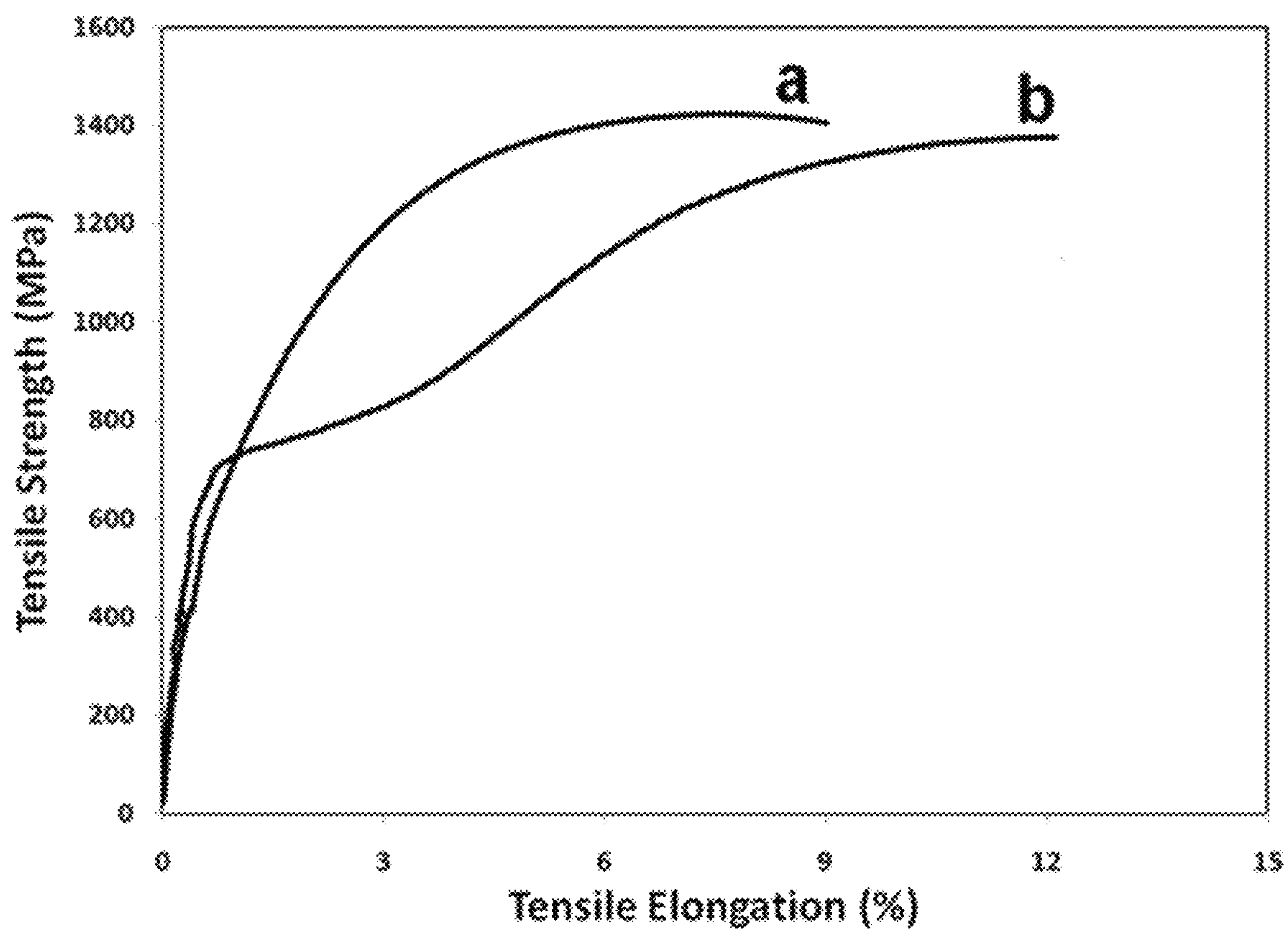
FIG. 44 Stress-strain curves recorded at tensile testing of specimens from the Alloy 5 plate after HIP cycle and heat treatment at 700 °C for 1 with cooling (a) in air and (b) with furnace.
