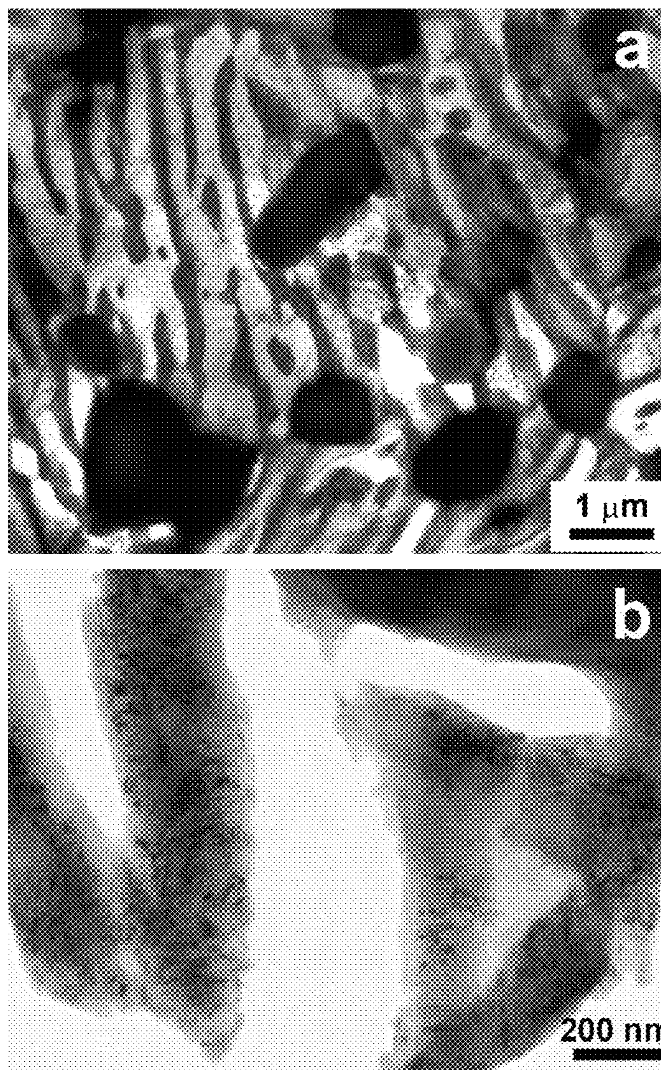
FIG. 27 The TEM micrographs of the microstructure in the Alloy 6 plate sample after HIP cycle at 1100°C for 1 hour and heat treatment at 700°C for 60 minutes with slow furnace cooling. (a) The precipitates grew slightly, but the lath structure in the matrix developed into lamellae structure. (b) A structure of the matrix at higher magnification.
