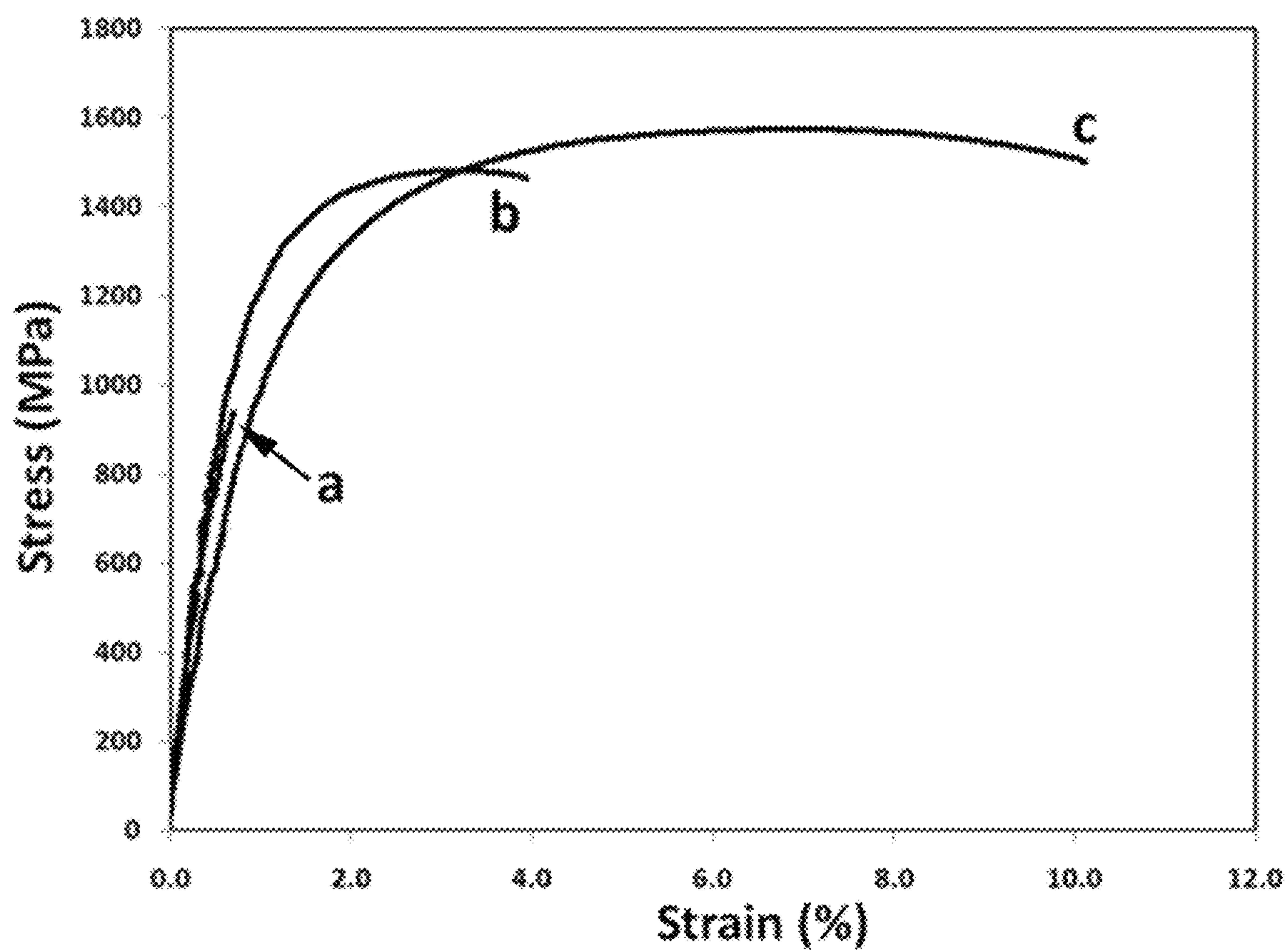
FIG. 34 Tensile properties of the specimens from the Alloy 6 plate in various conditions; a) As-cast, b) After HIP cycle at 1000°C for 1 hour, and c) After HIP cycle at 1100°C for 1 hour and heat treating at 700°C for 60 minutes with slow furnace cooling.
