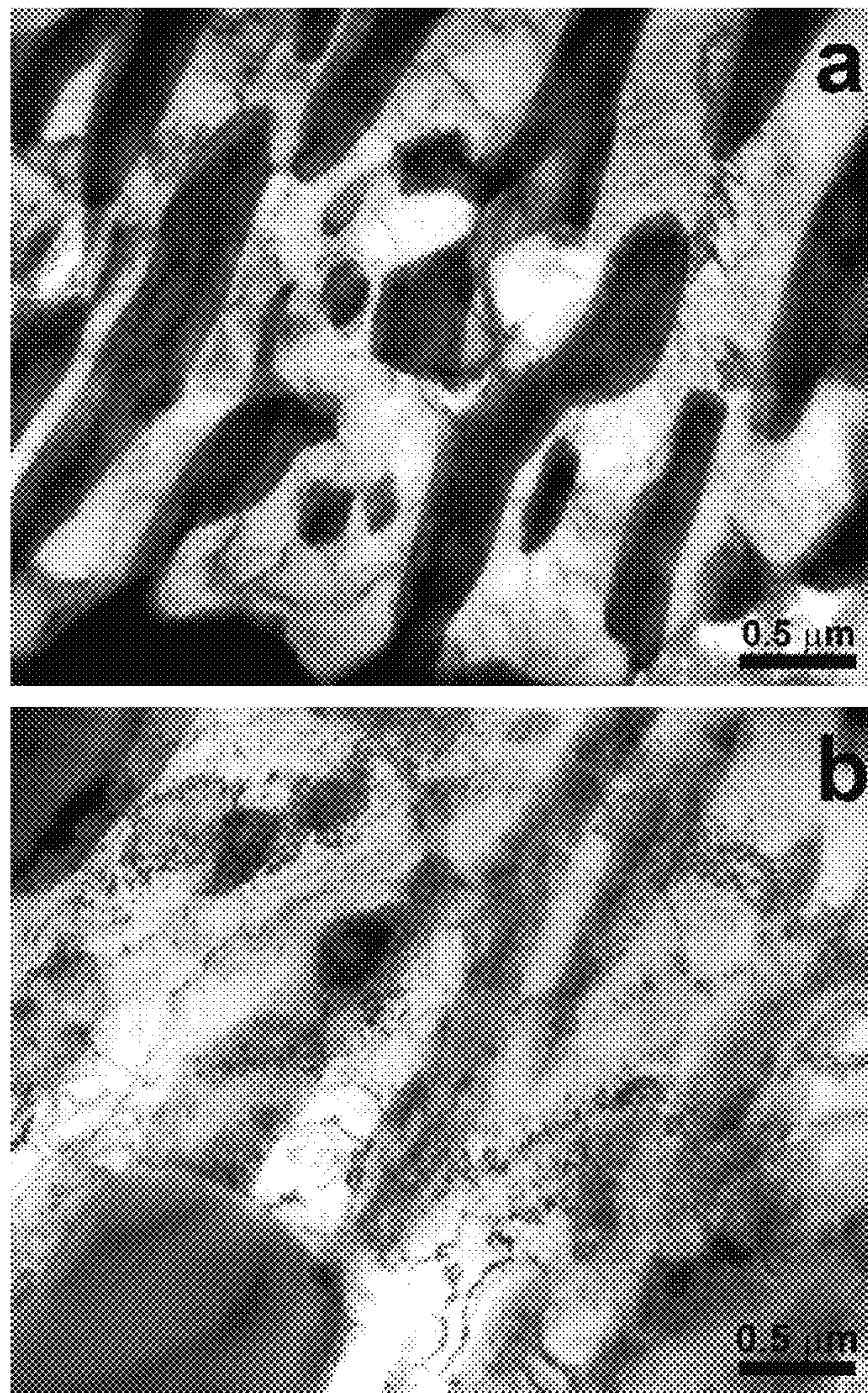
FIG. 39 TEM micrographs of the microstructure in the specimen from the Alloy 6 plate after HIP cycle at 1100°C for 1 hour and heat treatment at 700°C for 60 minutes with slow furnace cooling; a) Before tensile testing; b) After tensile testing.
