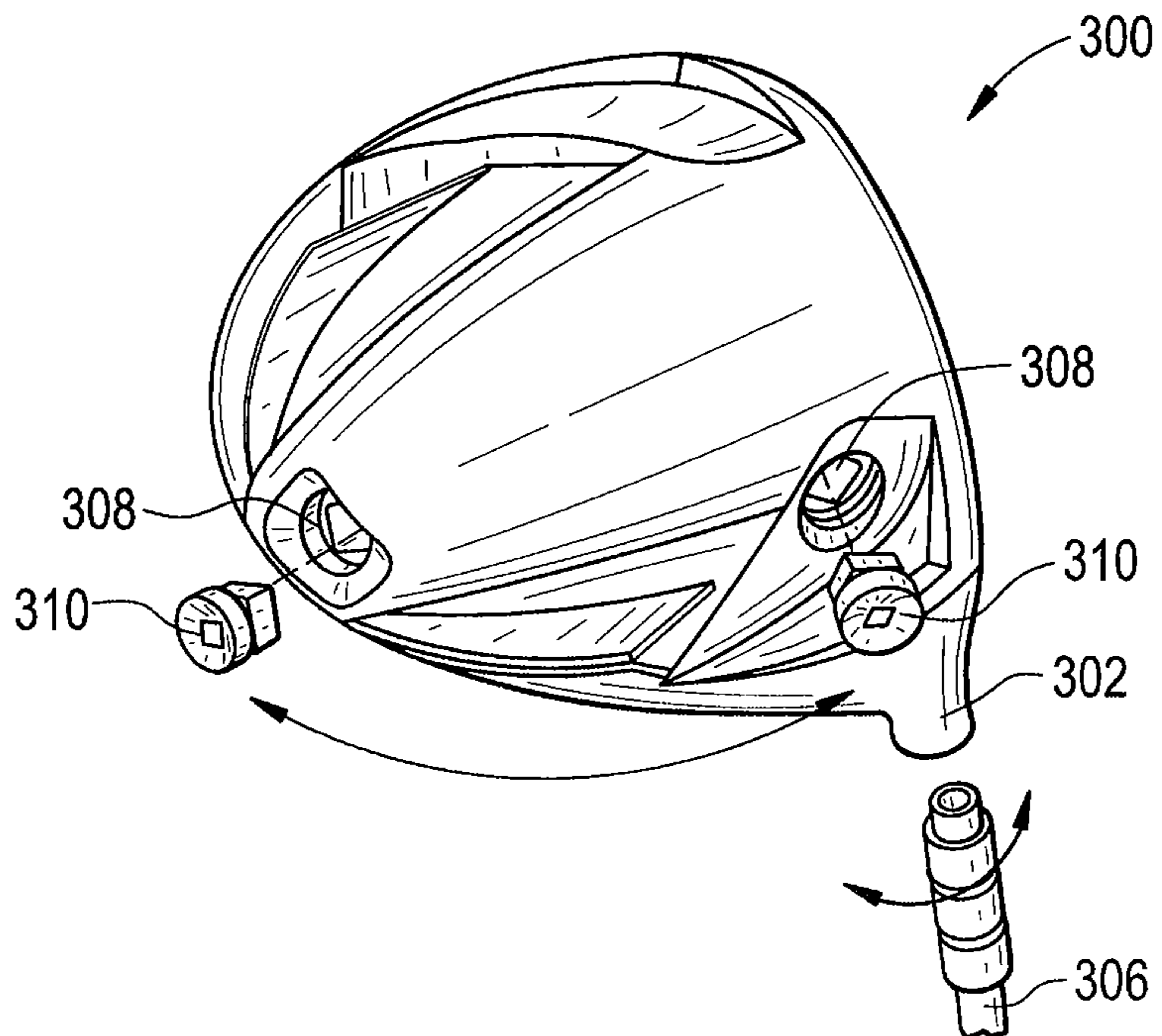
FIG. 3 Prior Art
