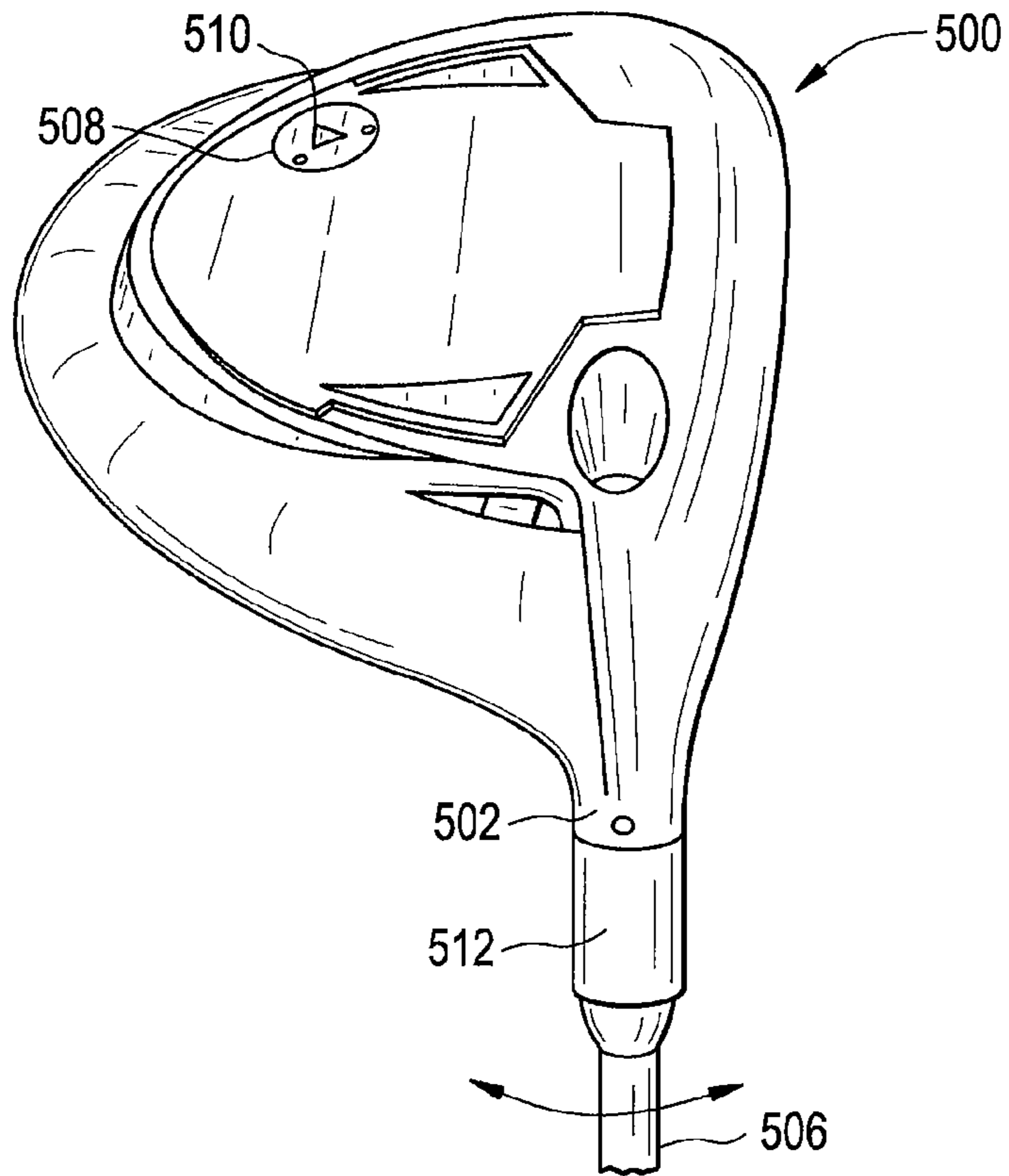
FIG. 5 Prior Art
