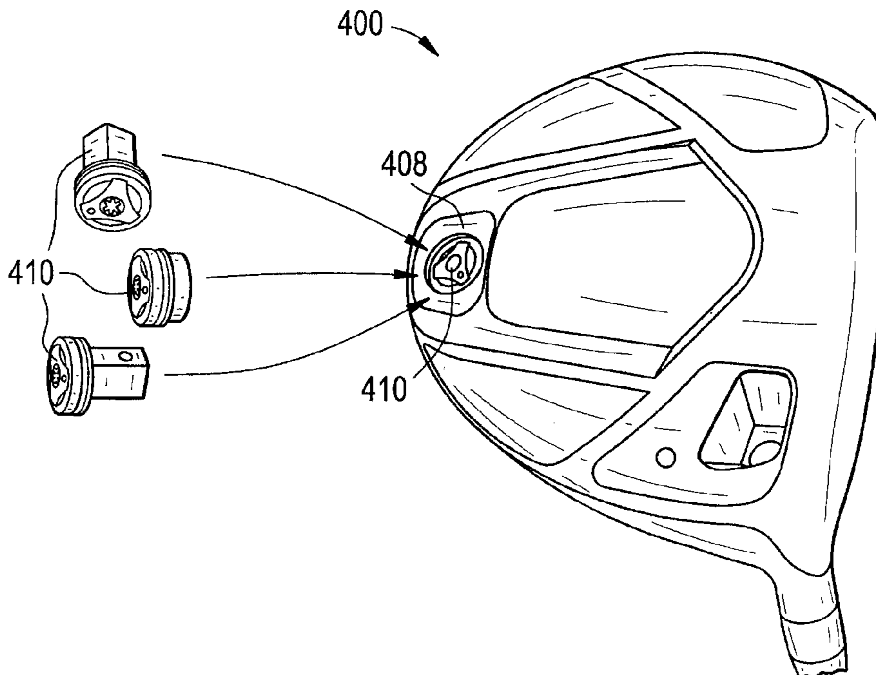
FIG. 4C Prior Art
