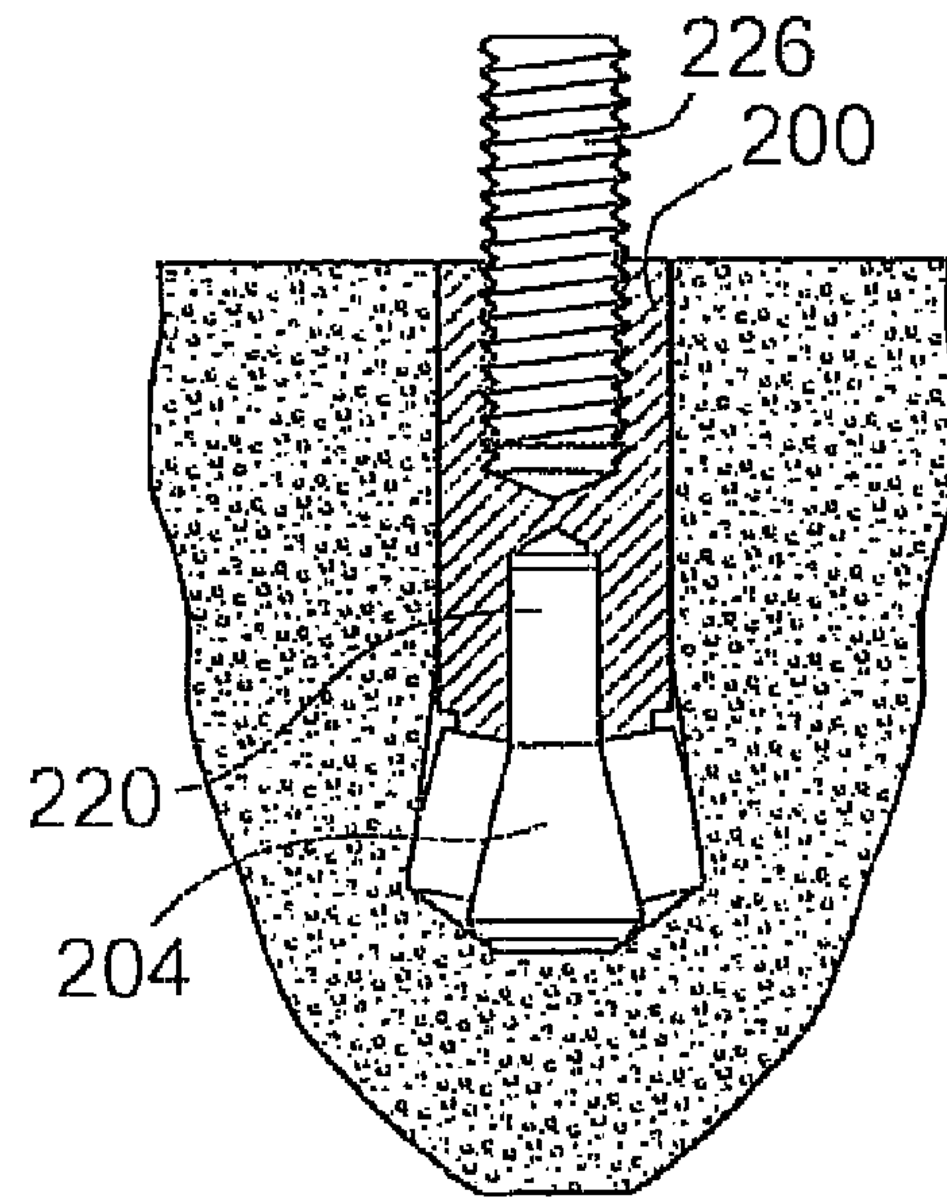
FIG. 20 PRIOR ART
