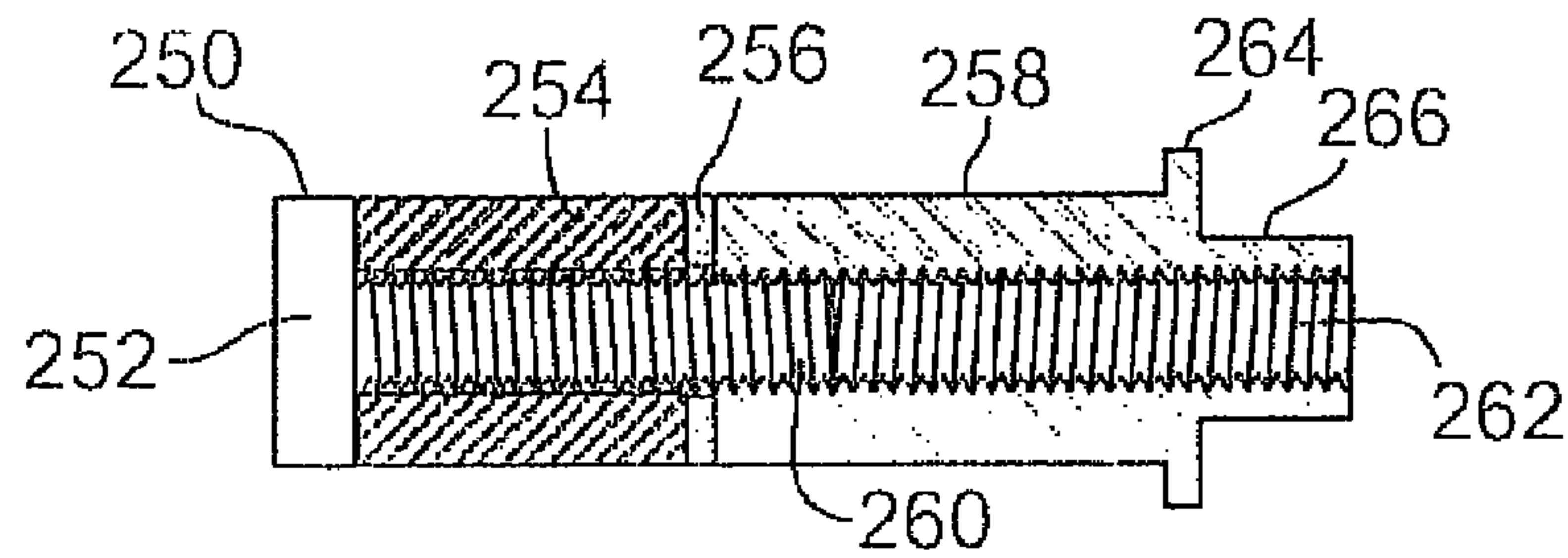
FIG. 22 PRIOR ART
