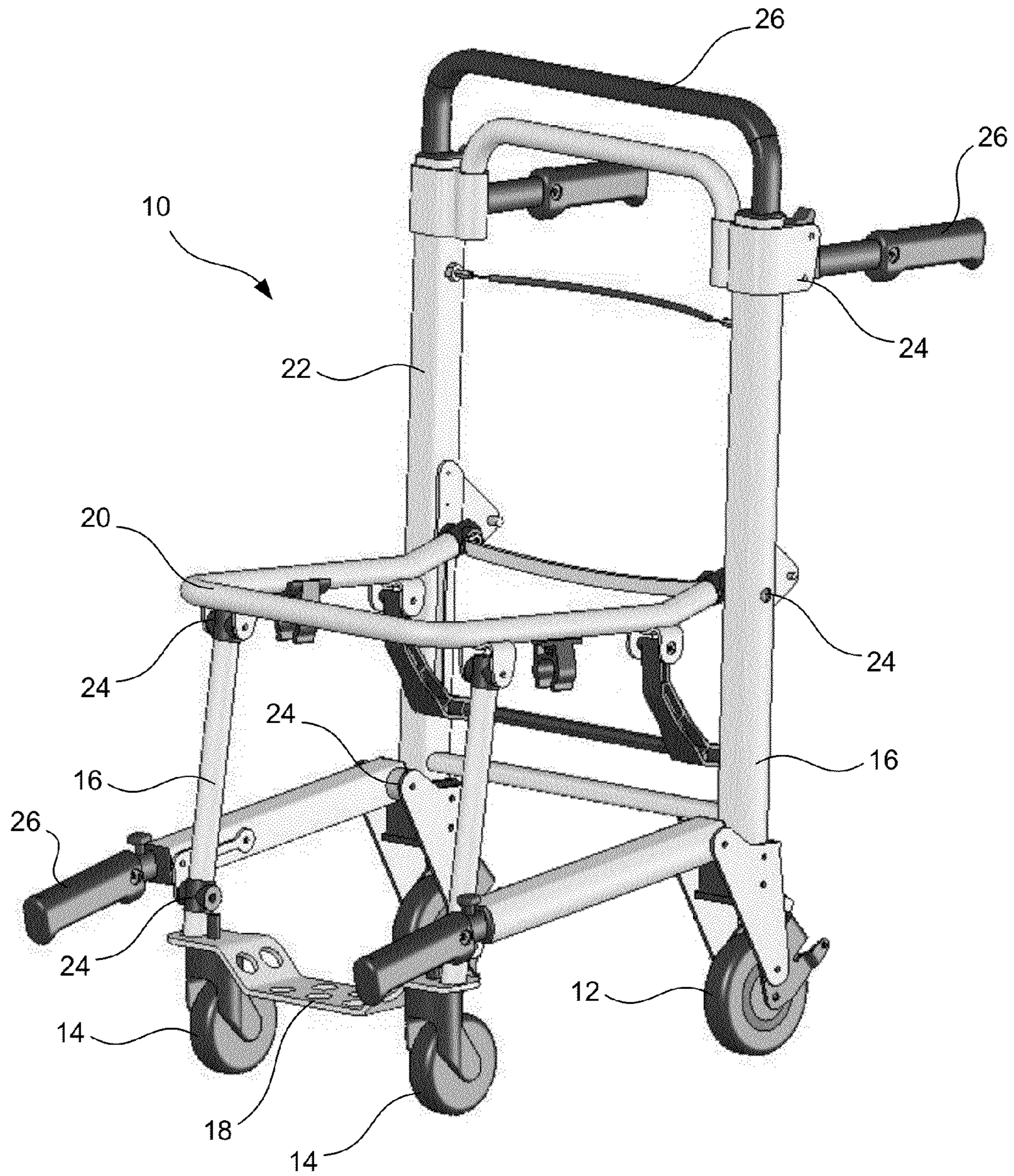
FIG. 1 (Prior Art)
