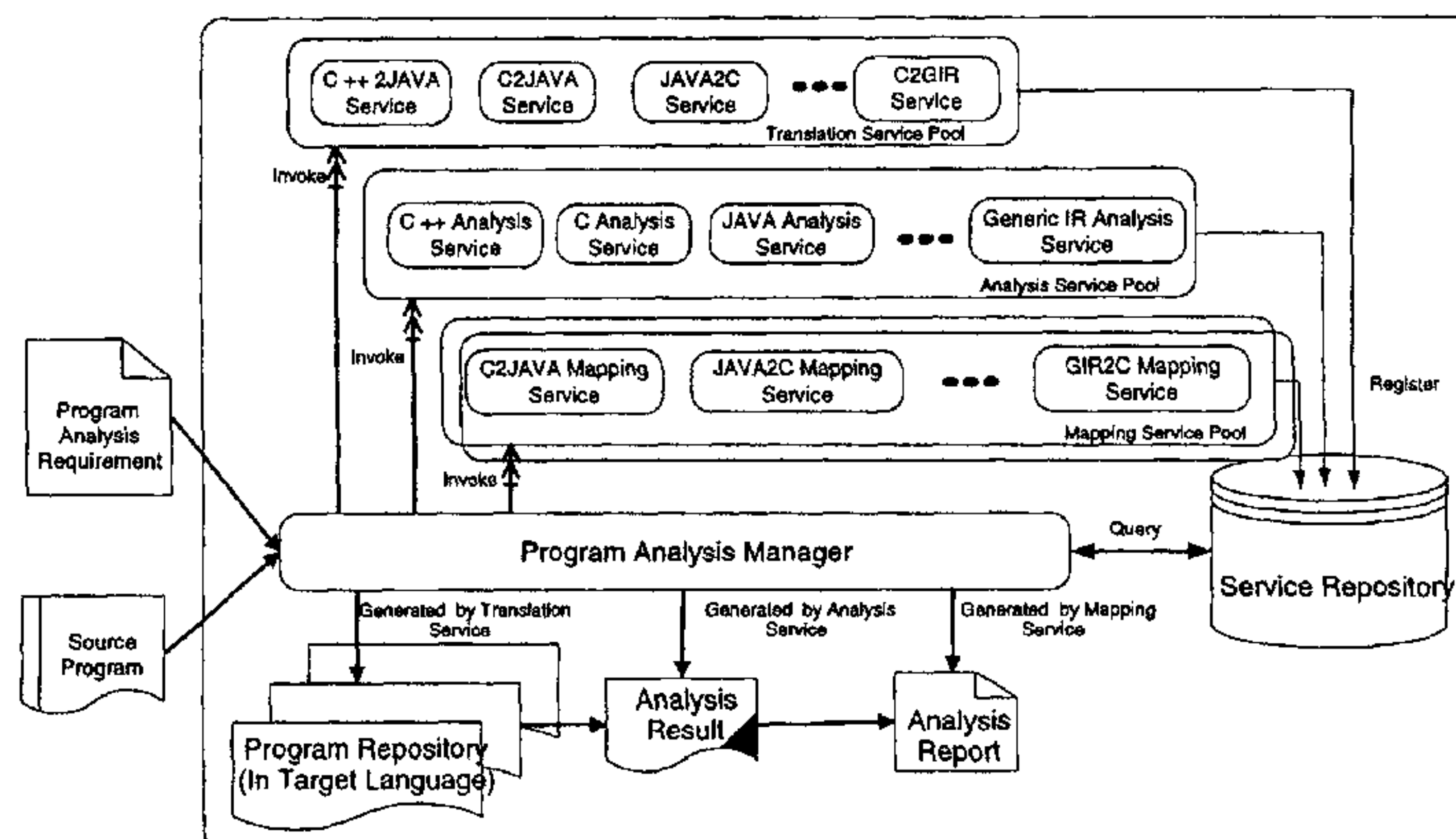
Architecture of a Unified Analysis Framework.
