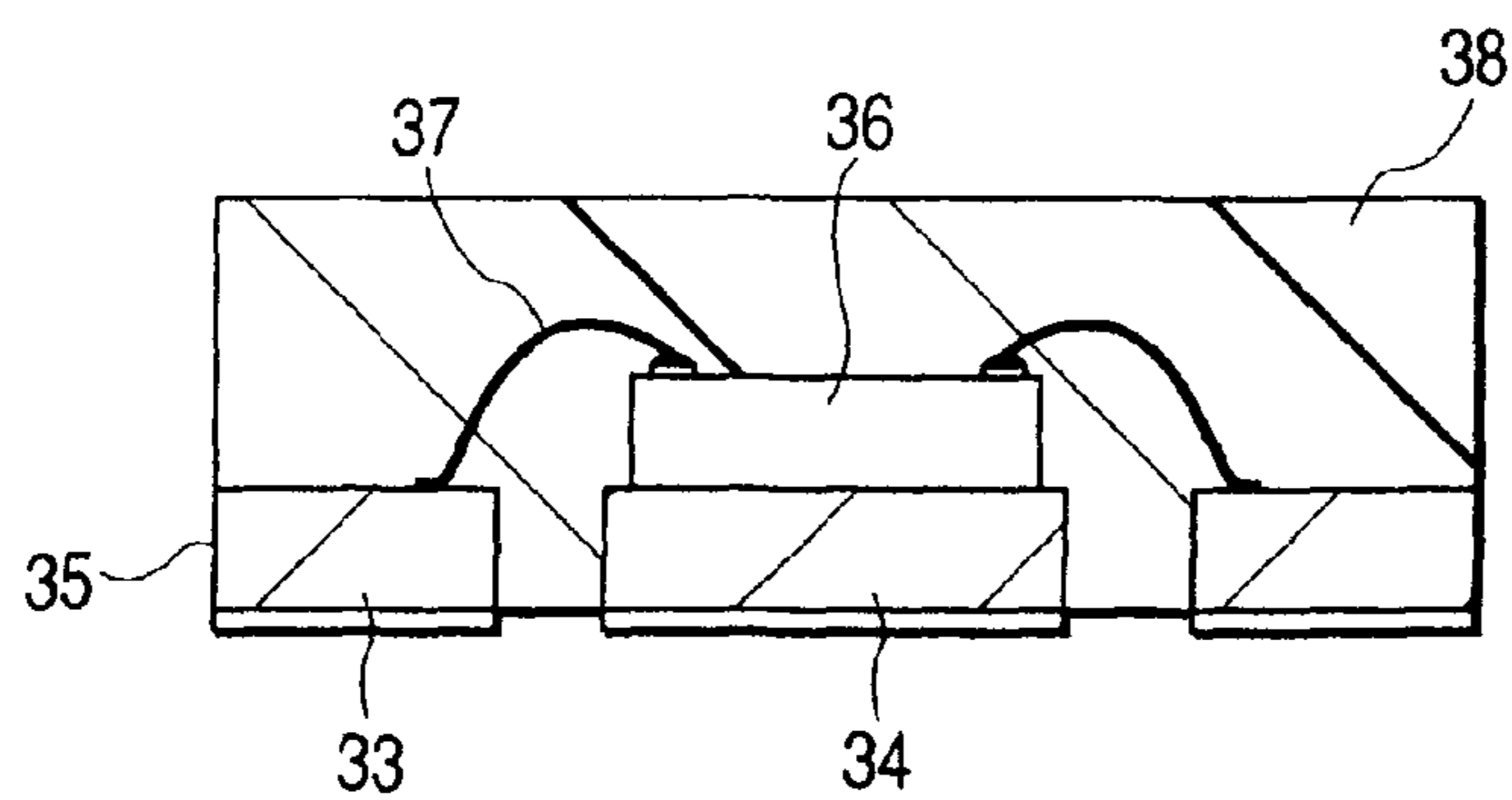
FIG. 29 PRIOR ART
