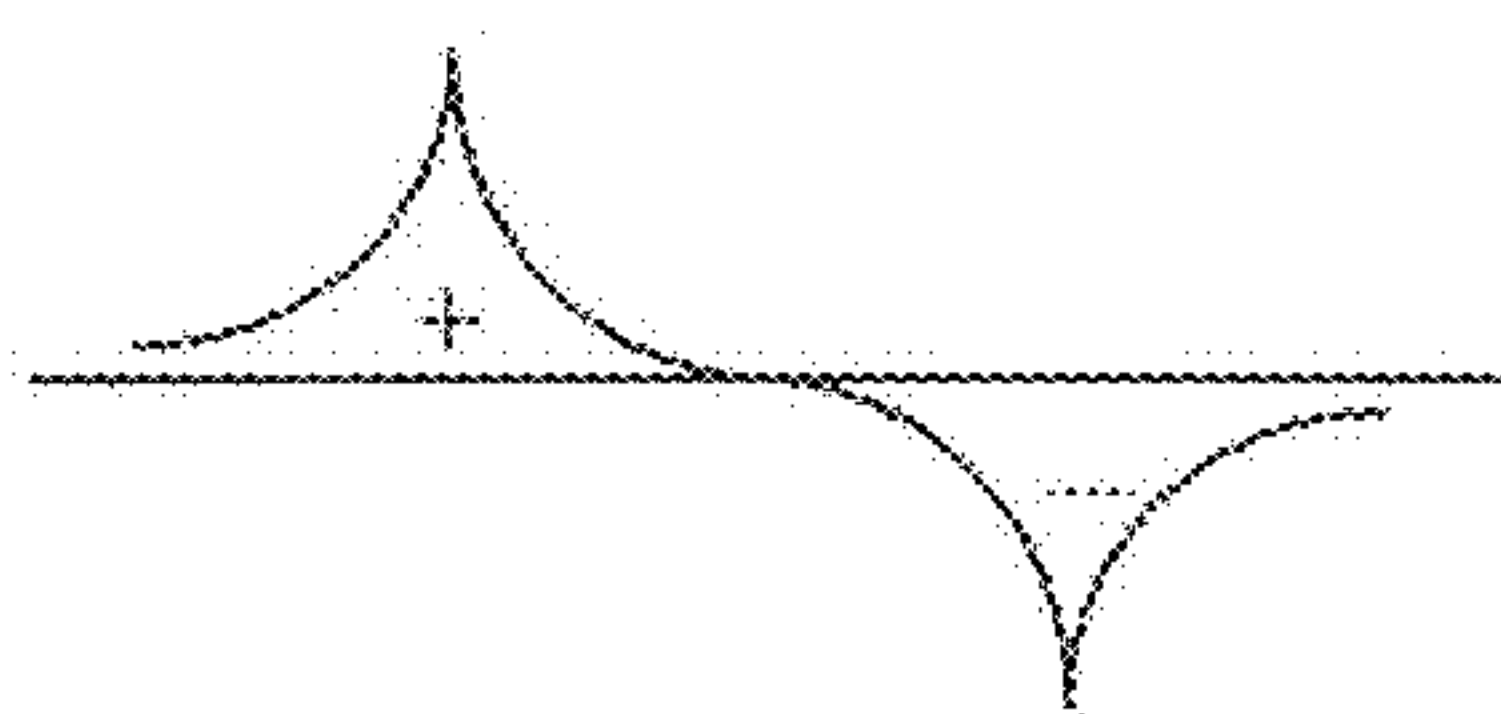
Antibonding orbital
