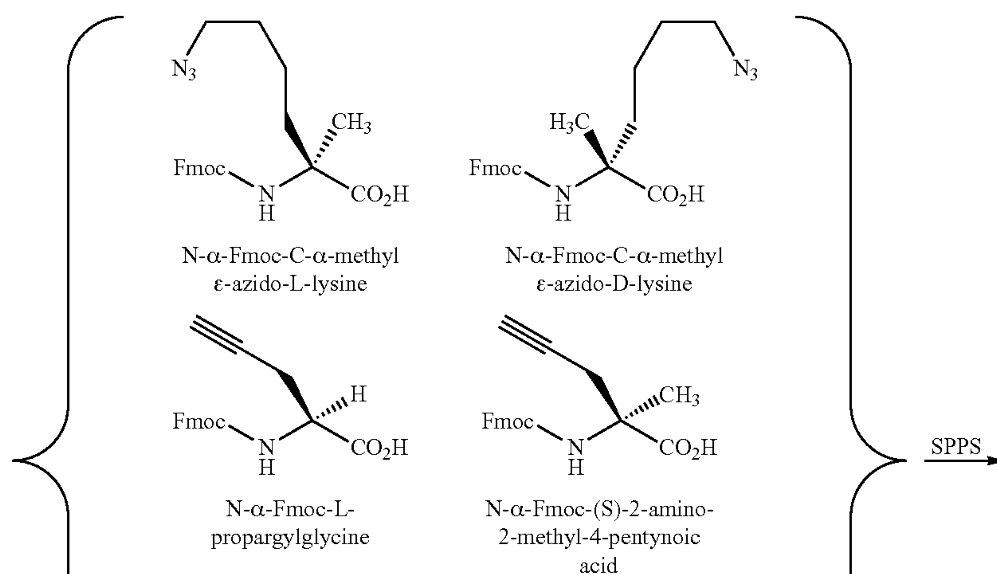
Synthetic Scheme 3:
