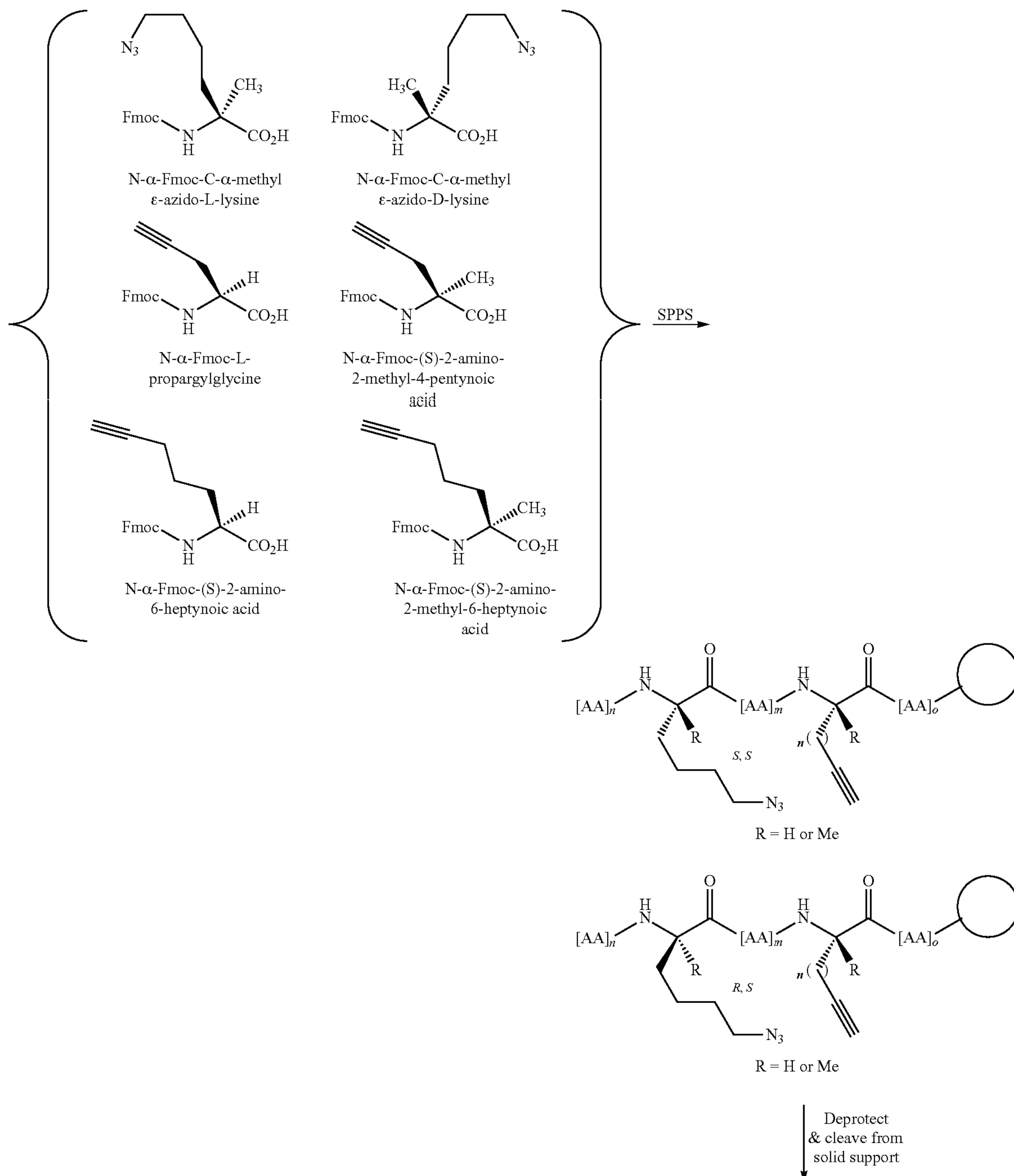
Synthetic Scheme 2:
