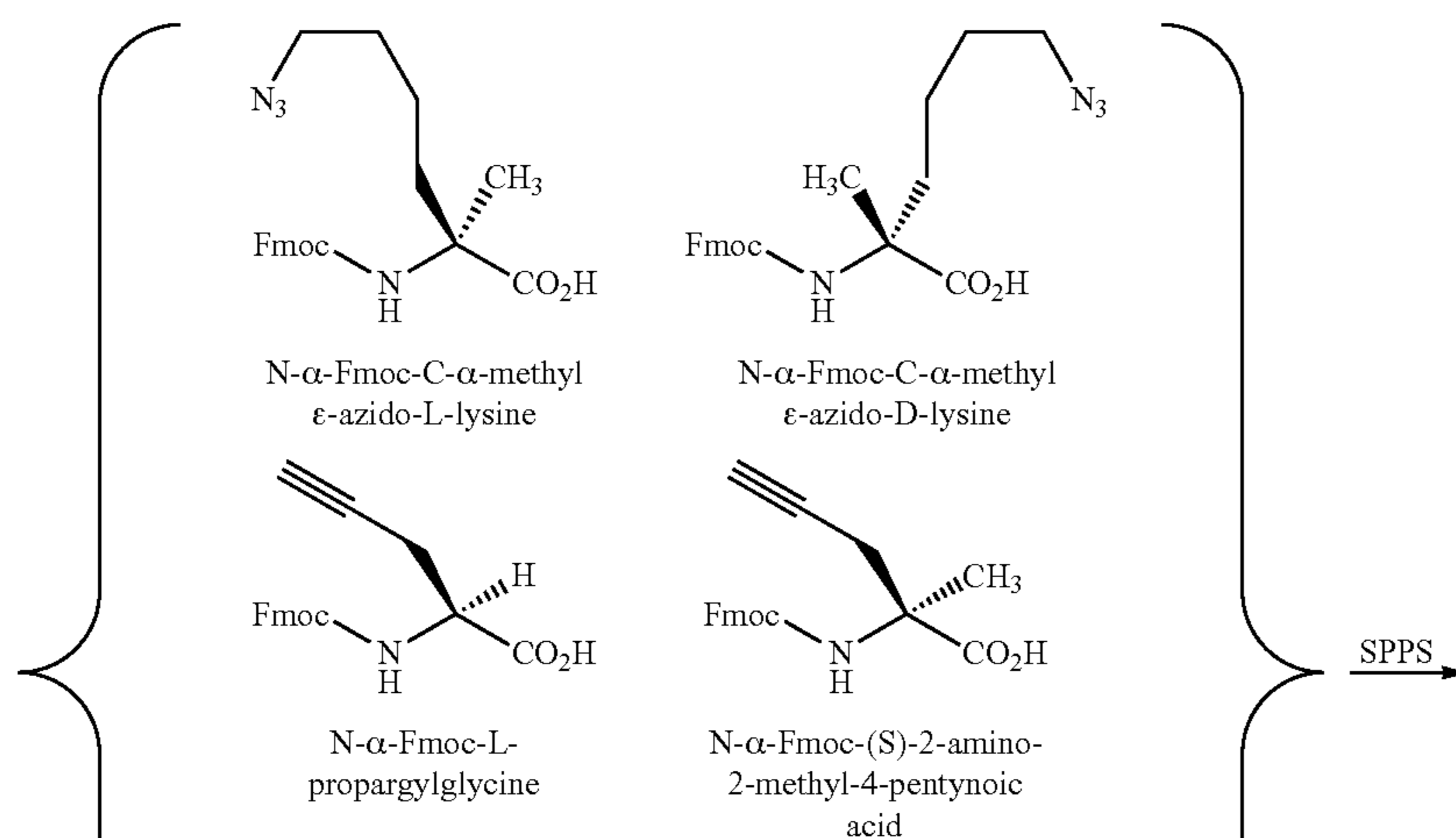
Synthetic Scheme 3:
