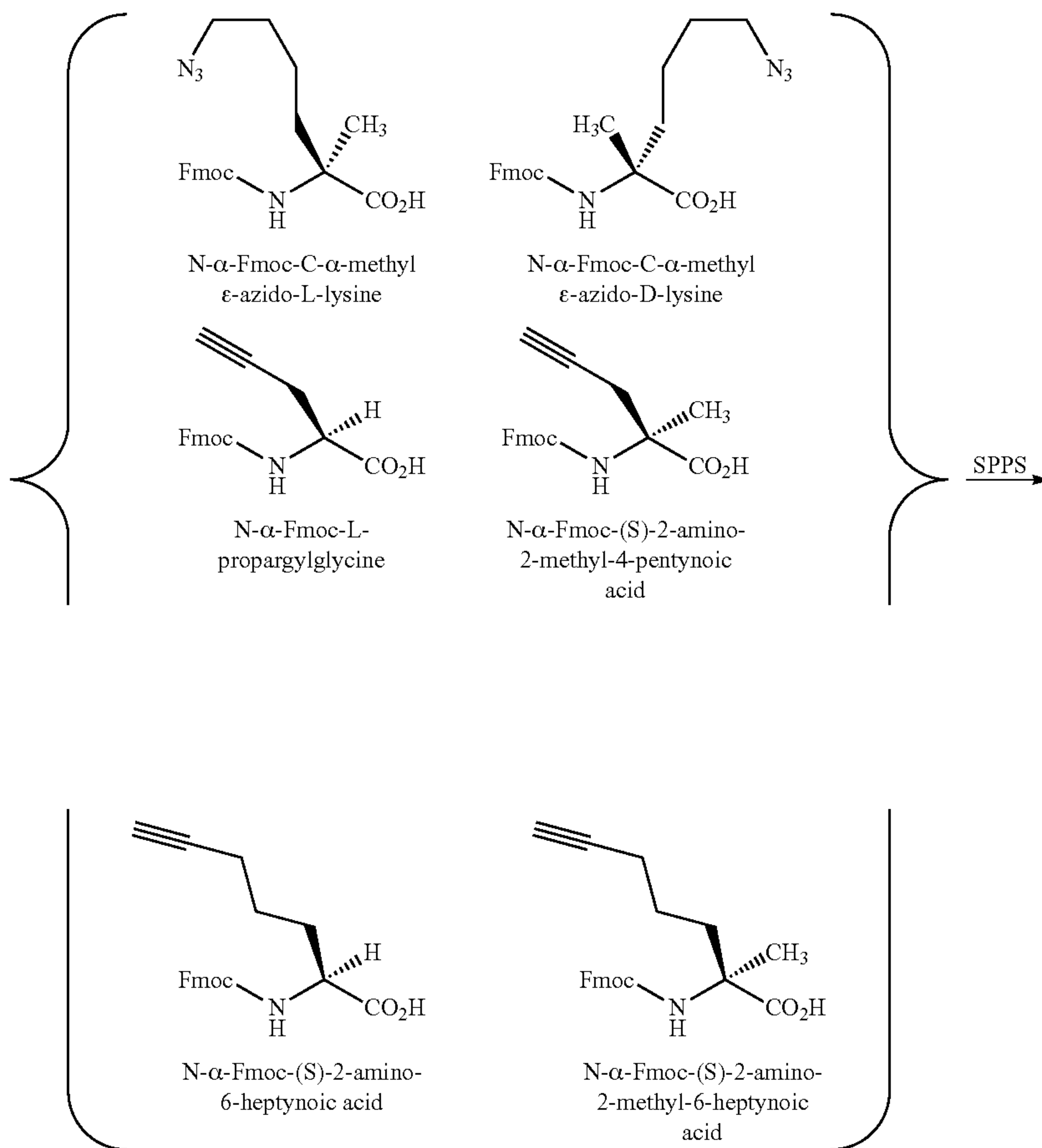
Synthetic Scheme 5:
