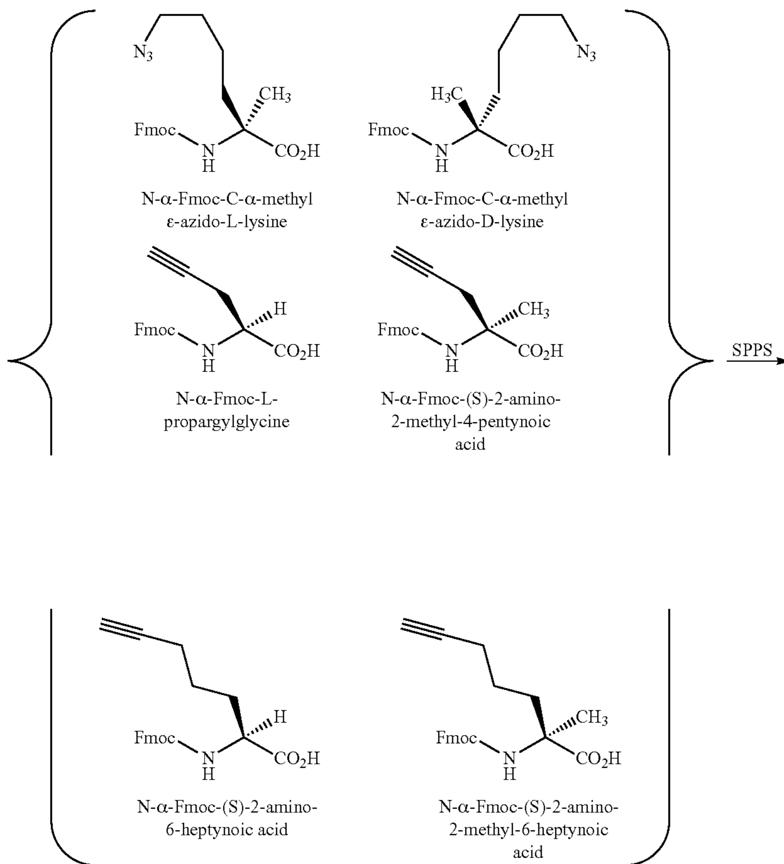
Synthetic Scheme 5:
