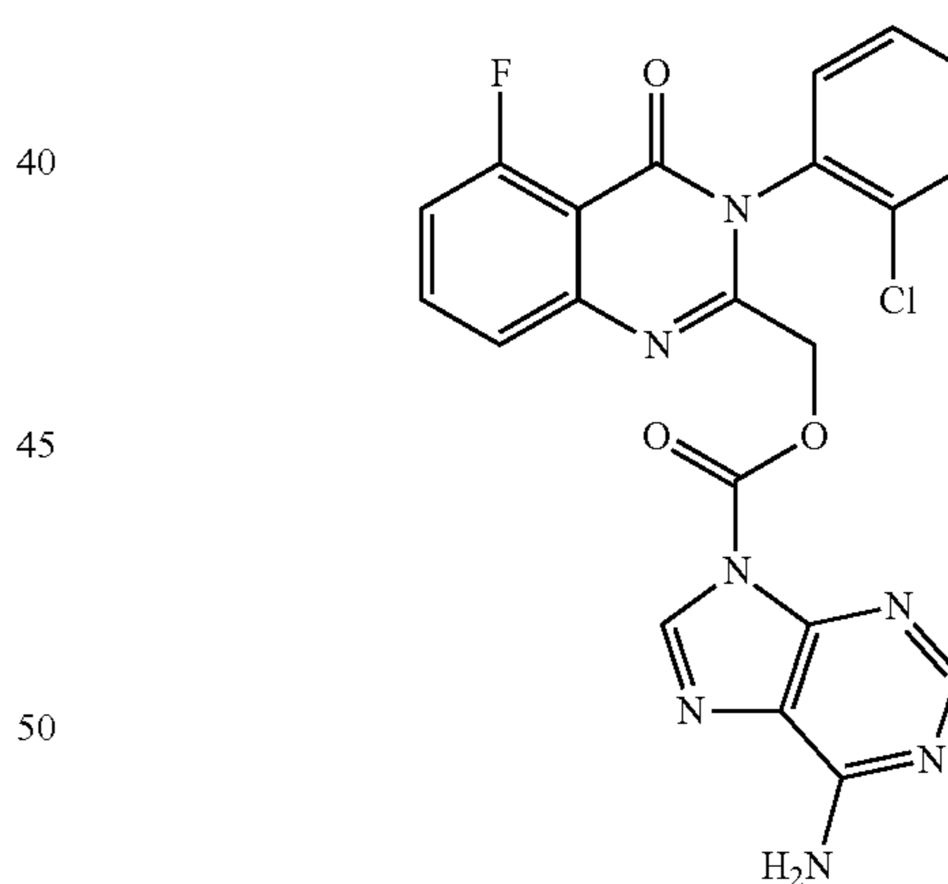
6-Aminopurine-9-carboxylic acid 3-(2-chlorophenyl)-5-fluoro-4-oxo-3,4-dihydro-quinazolin-2-ylmethyl ester (D-079)
