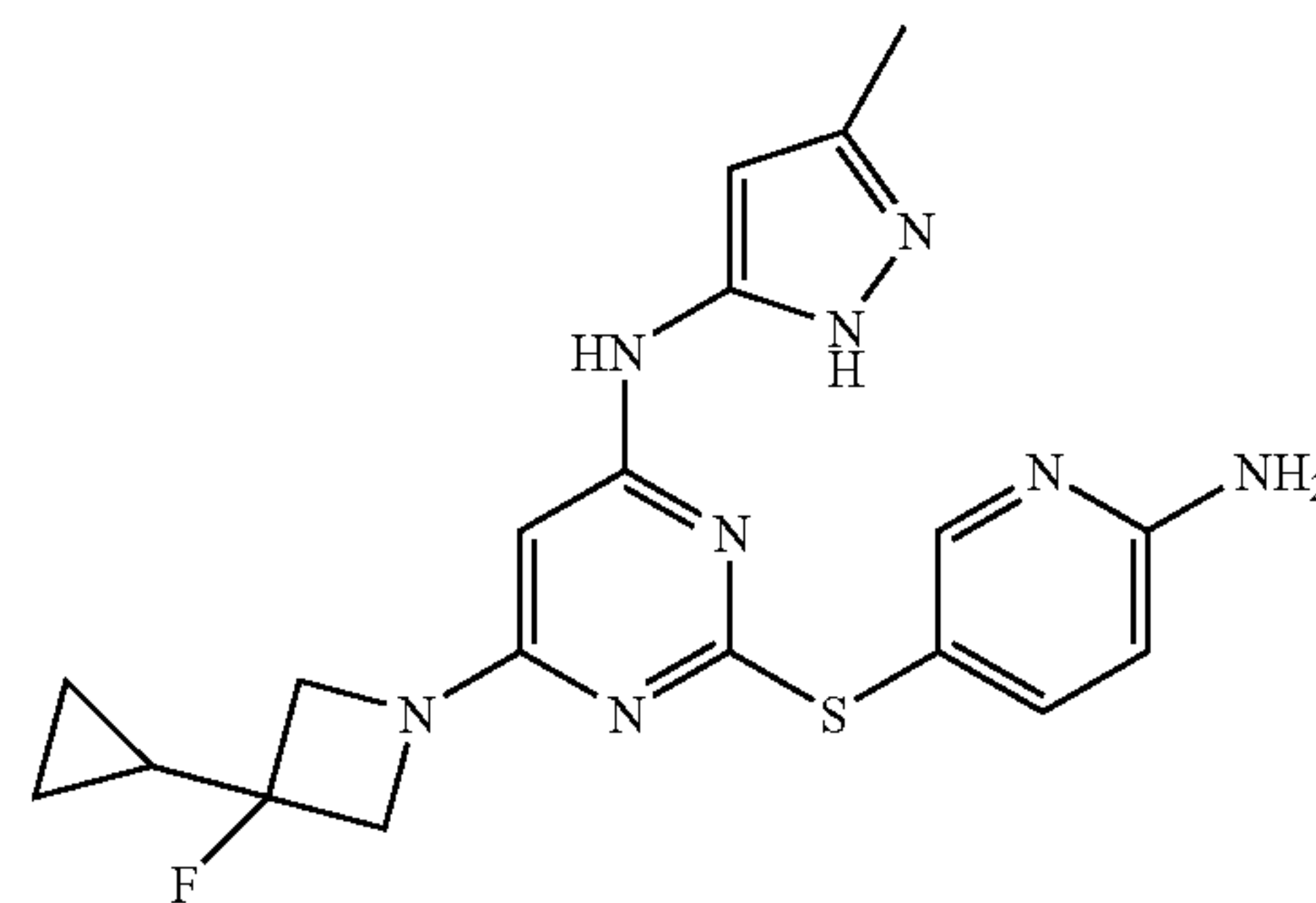
2-(6-(3-cyclopropyl-3-fluoroazetidin-1-yl)-6-(3-methyl-1H-pyrazol-5-yl)pyrimidin-4-ylthio)-6-aminopyridine-3-thiol
