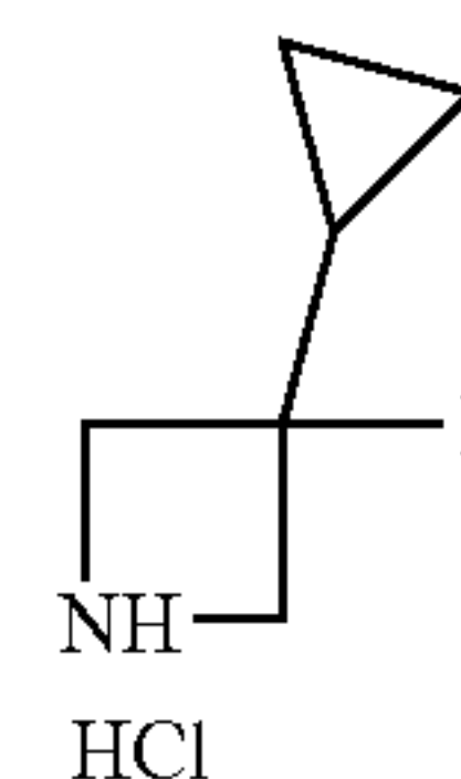
3-cyclopropyl-3-fluoroazetid-3-ol hydrochloride
