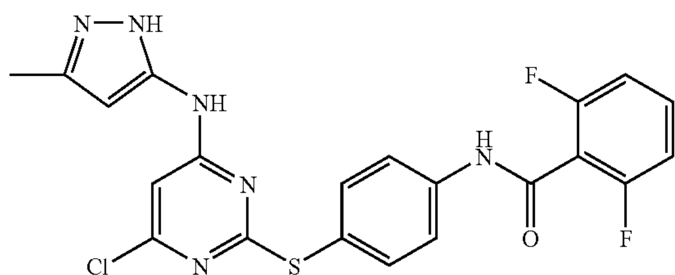
2,6-Difluoro-N-{4-[4-chloro-6-(5-methyl-2H-pyrazol-3-ylamino)-pyrimidin-2-ylsulfanyl]-phenyl}-benzamide
