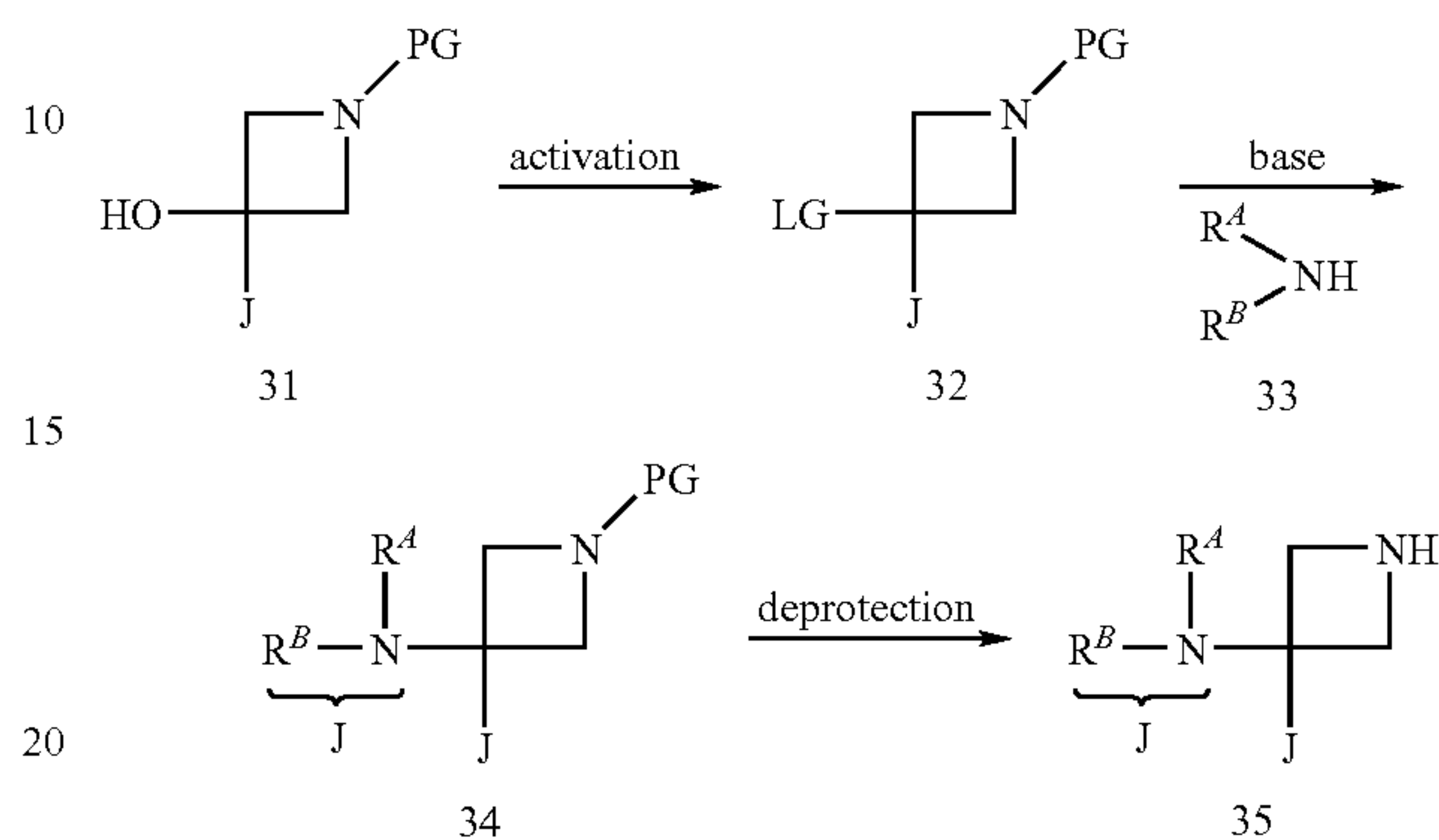
Scheme A
