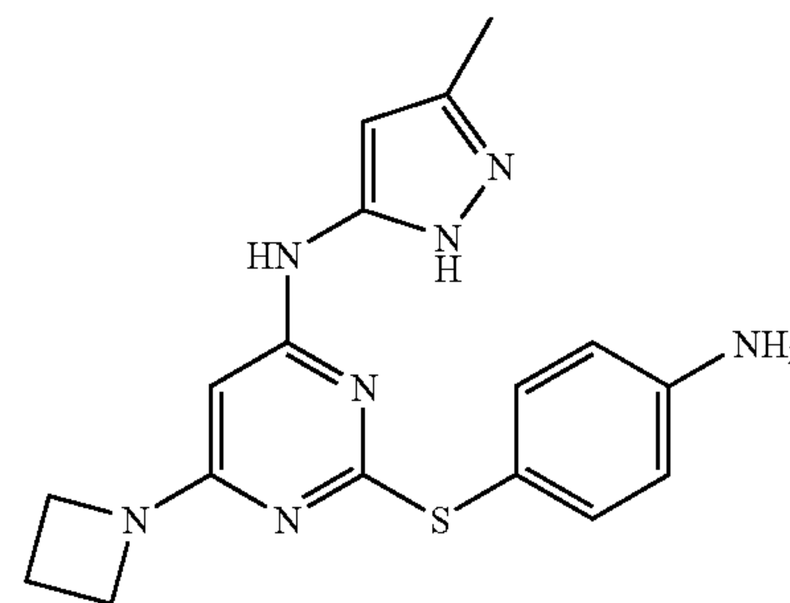
2-(4-aminophenylthio)-6-(azetidin-1-yl)-N-(3-methyl-1H-pyrazol-5-yl)pyrimidin-4-amine
