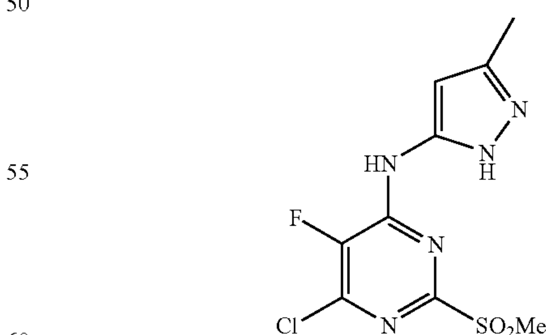
6-chloro-5-fluoro-N-(3-methyl-1H-pyrazol-5-yl)-2-(methylsulfonyl)pyrimidin-4-amine
