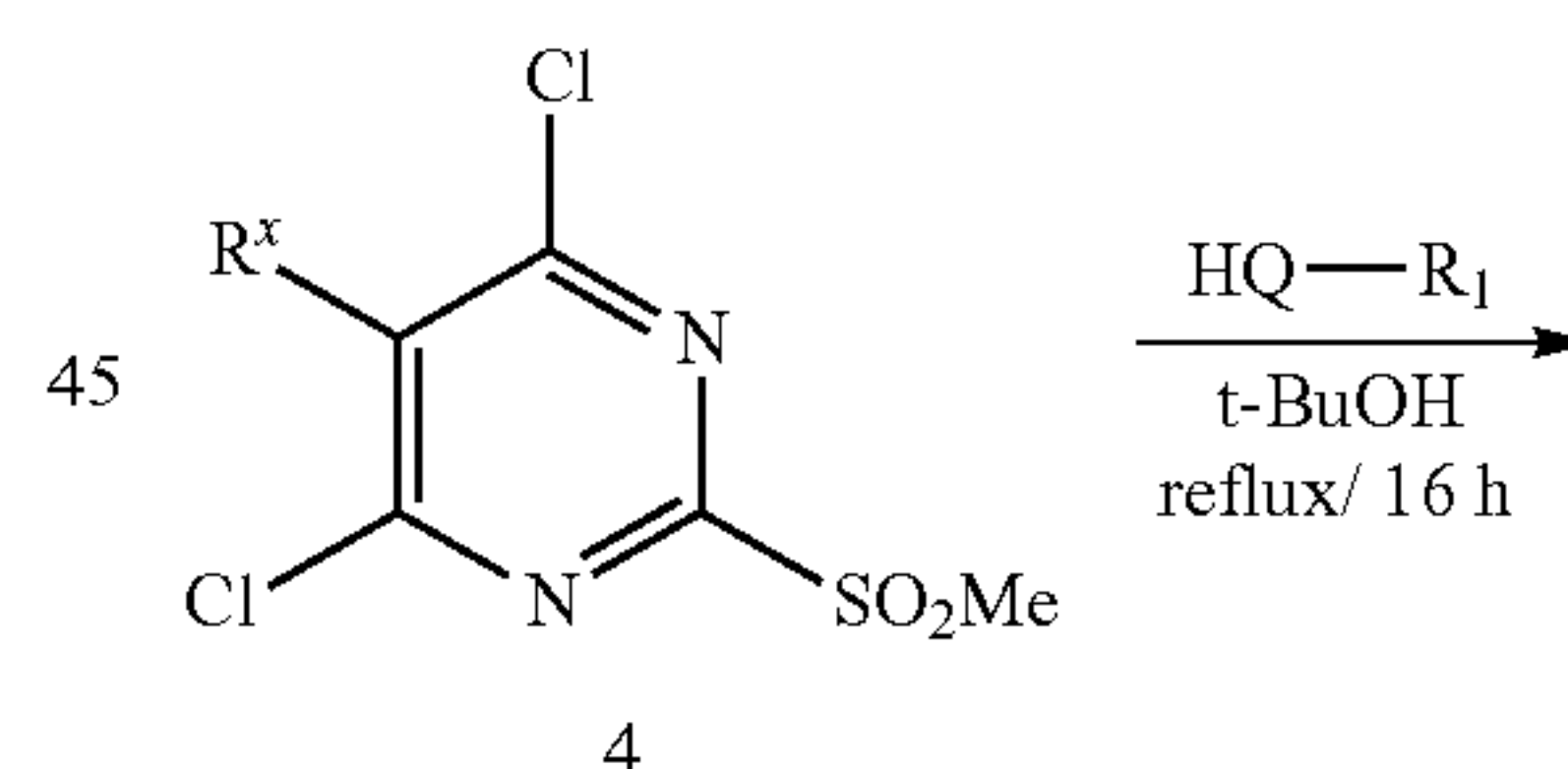
Scheme IV
