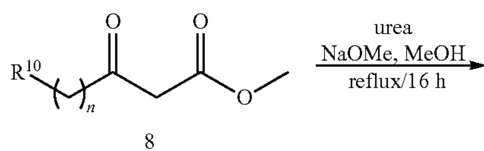
Scheme III
