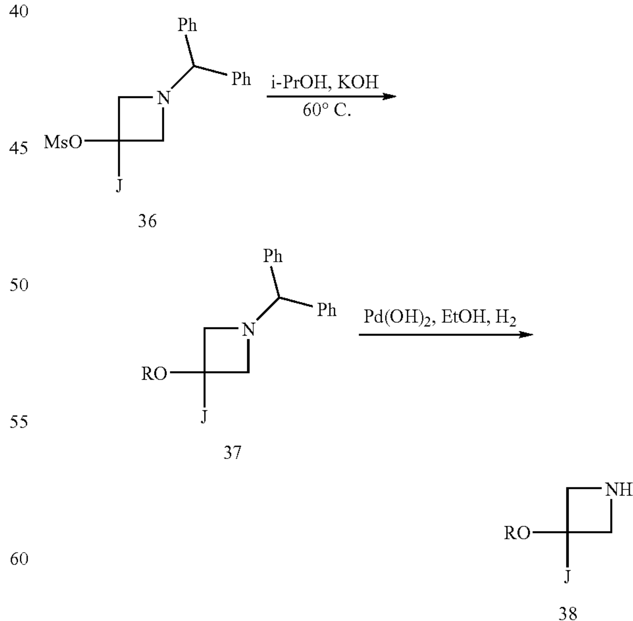
Scheme B
