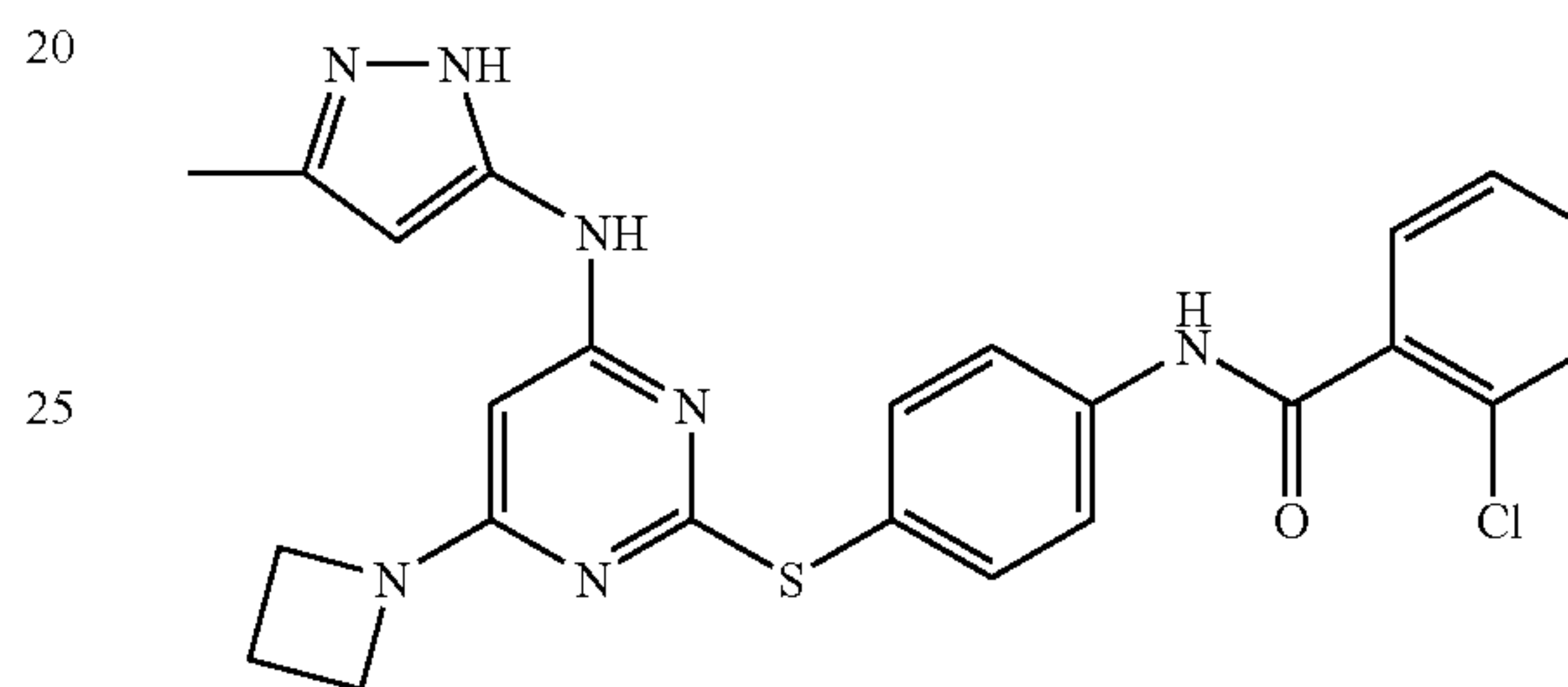
N-{4-[4-Azetidin-1-yl-6-(5-methyl-2H-pyrazol-3-ylamino)-pyrimidin-2-ylsulfanyl]-phenyl}-2-chloro-benzamide
