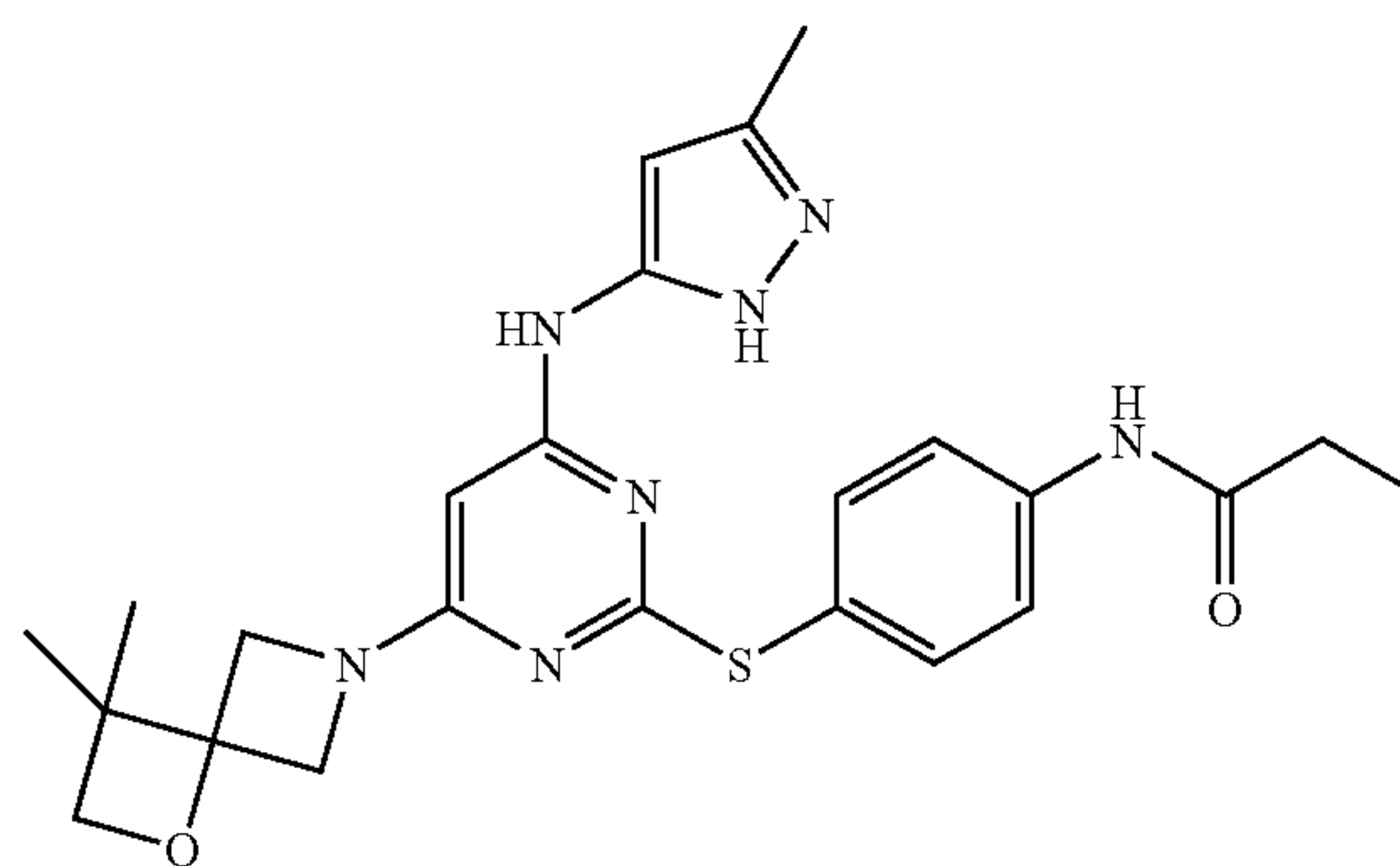
N-{4-[4-(3,3-Dimethyl-1-oxa-6-aza-spiro[3.3]hept-6-yl)-6-(5-methyl-2H-pyrazol-3-ylamino)-pyrimidin-2-ylsulfanyl]-phenyl}-propionamide
