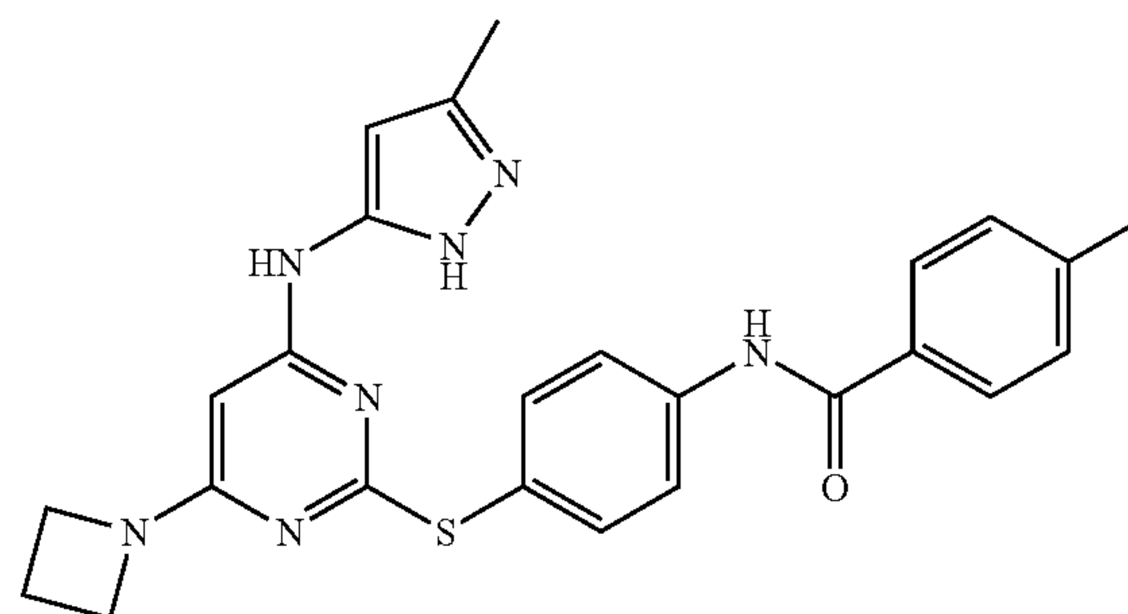
N-(4-(4-(3-methyl-1H-pyrazol-5-ylamino)-6-(azetidin-1-yl)pyrimidin-2-ylthio)phenyl)-4-methylbenzamide
