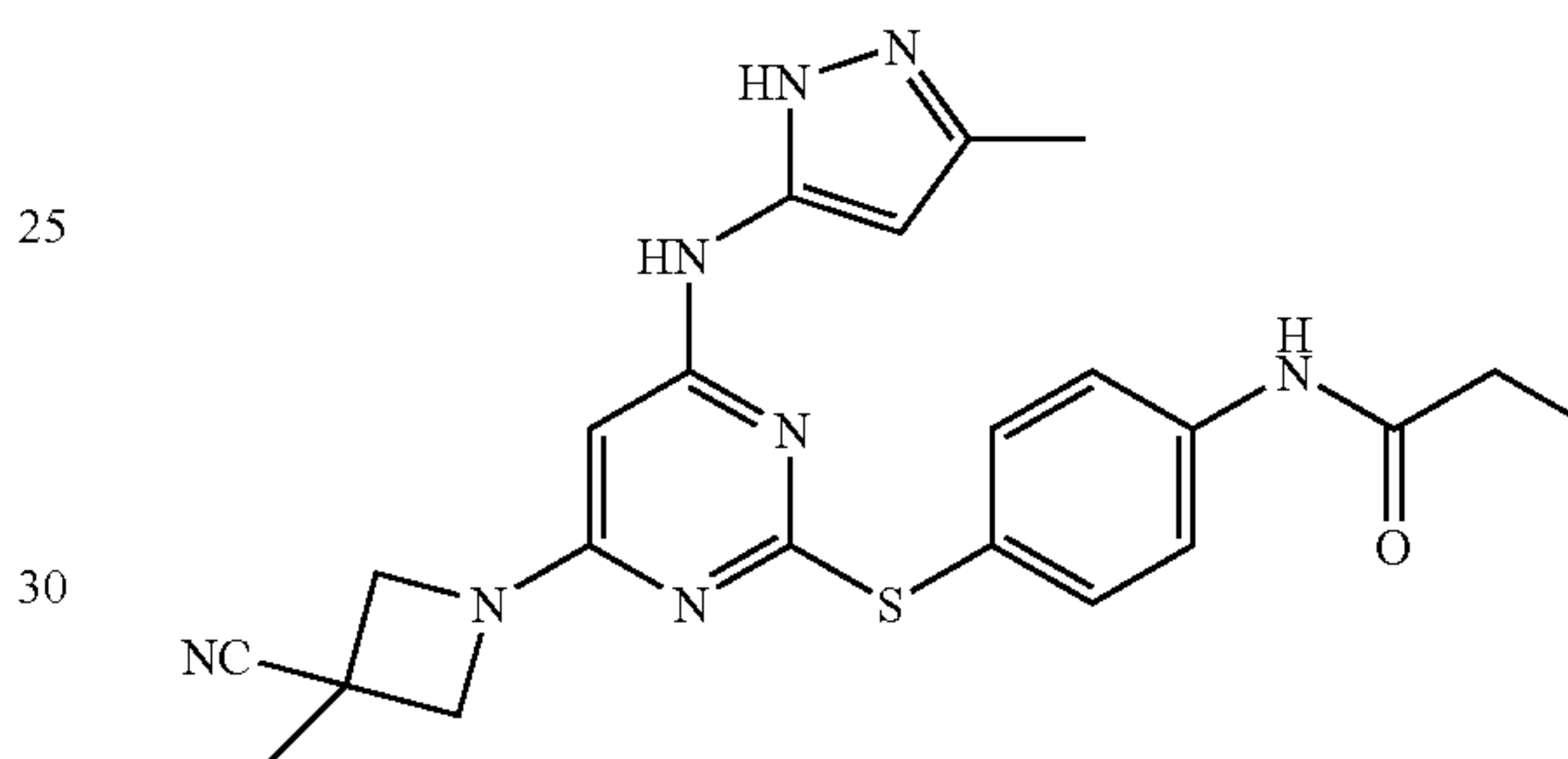
N-(4-((4-(3-methyl-1H-pyrazol-5-ylamino)-6-(3-cyano-3-methylazetidinium-1-yl)pyrimidin-2-yl)sulfonyl)phenyl)propionamide
