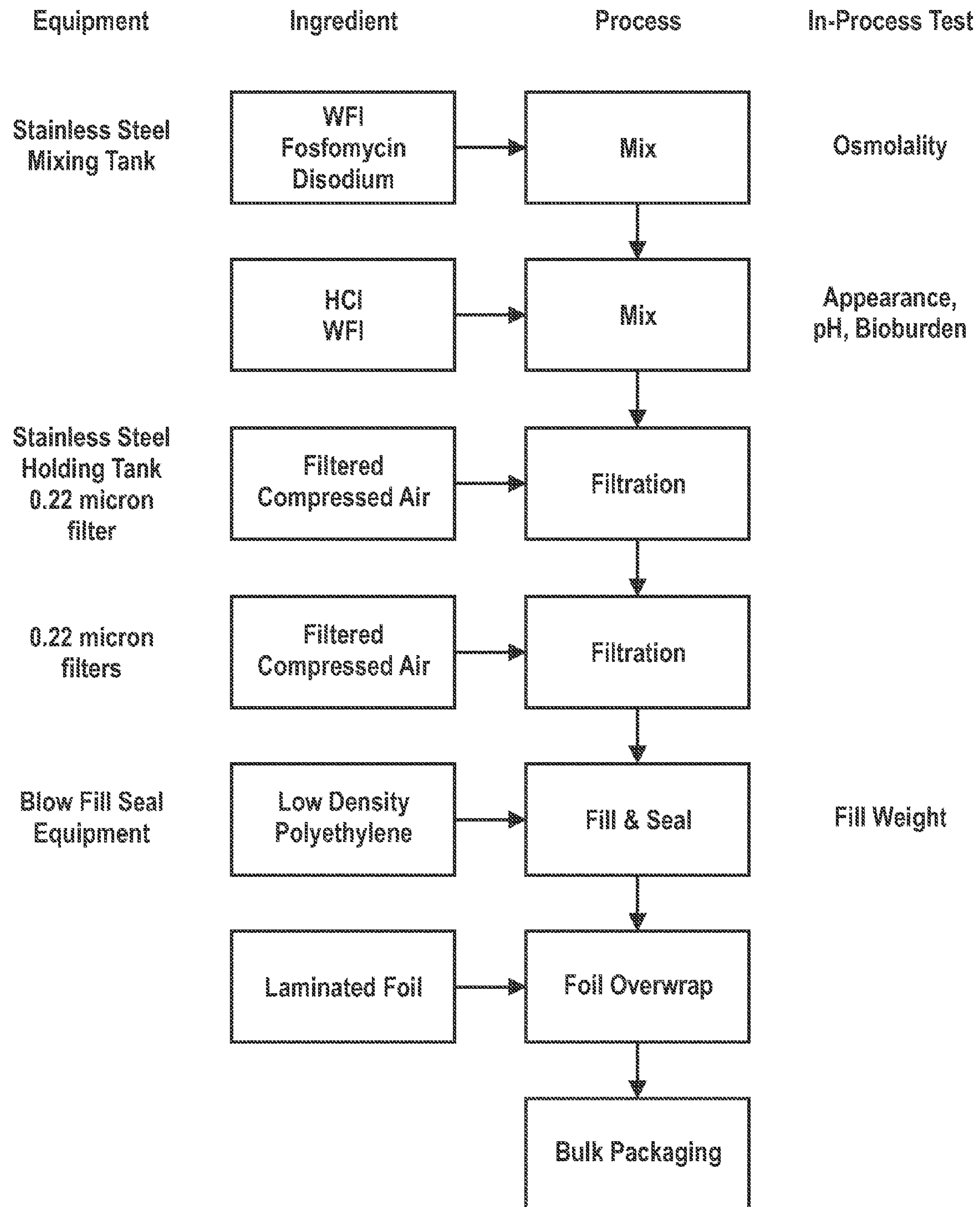
Figure 6 Fosfomycin Process Flow
