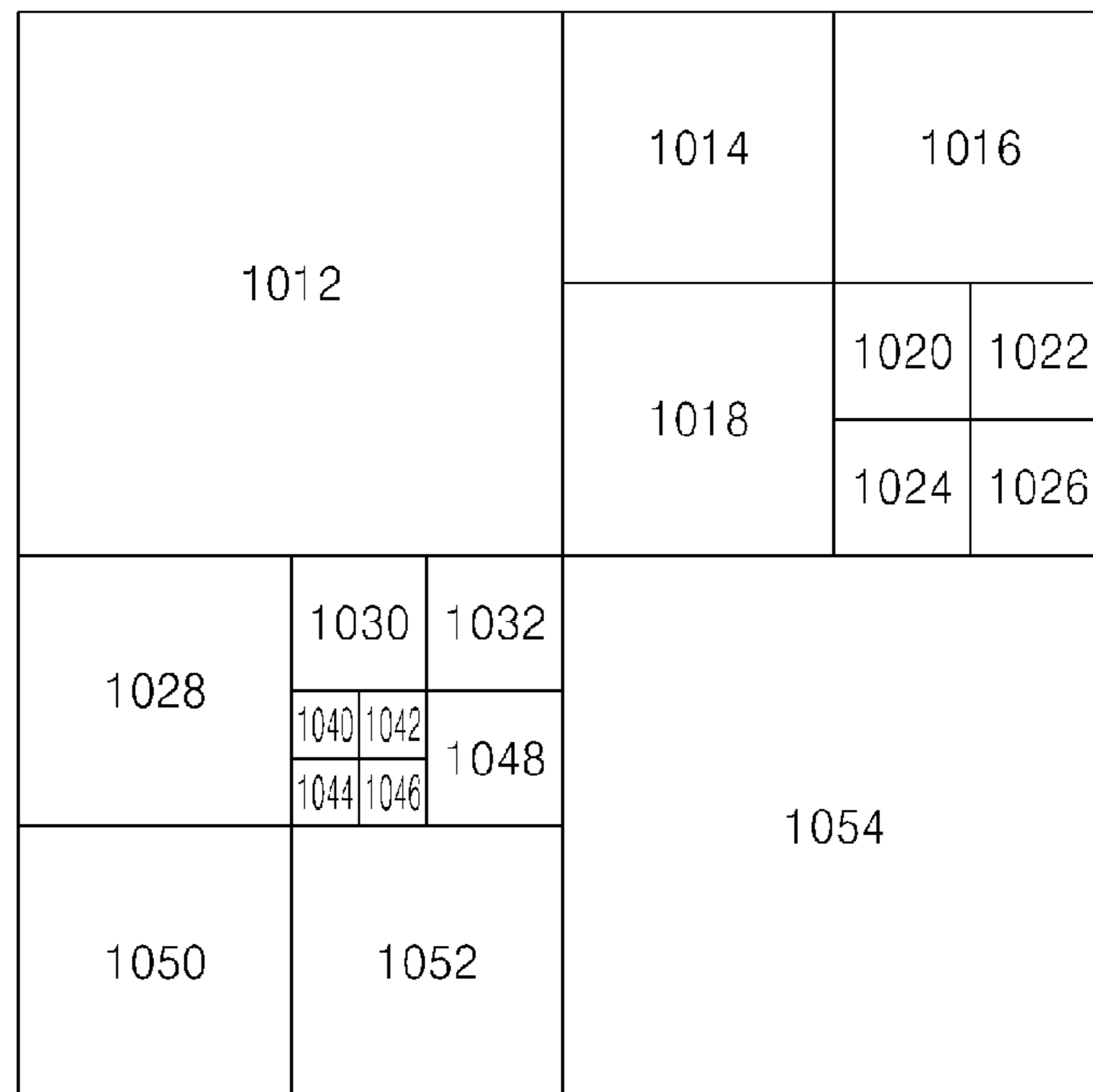
CODING UNITS (1010)
