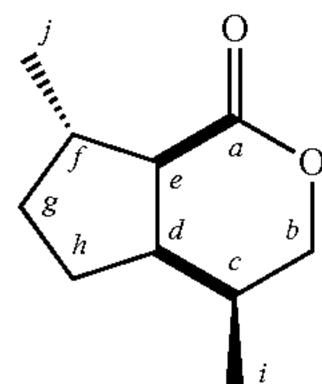
Formula 2 dihydronepetalactone of Formula 2 (9S, 5S, 1R, 6R)-5,9-dimethyl-3-oxabicyclo[4.3.0]nonan-2-one).
