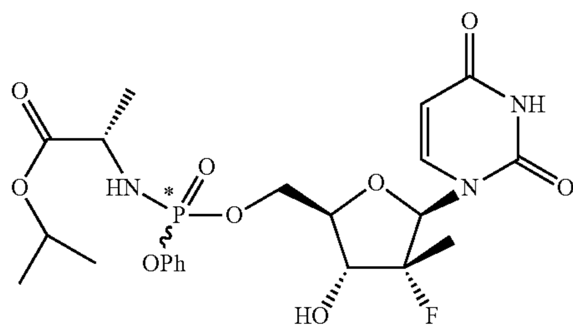
5'-O-phosphoramidate (2 diastereomers)
