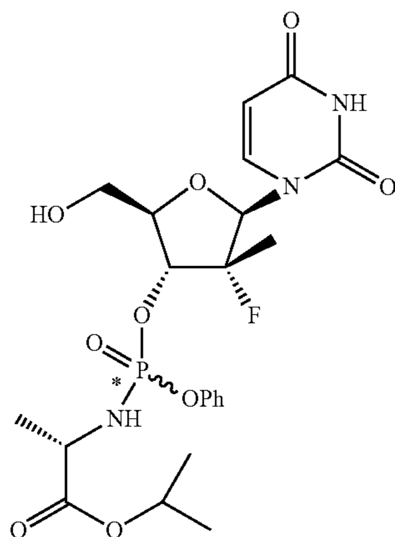
3'-O-phosphoramidate (2 diastereomers)
