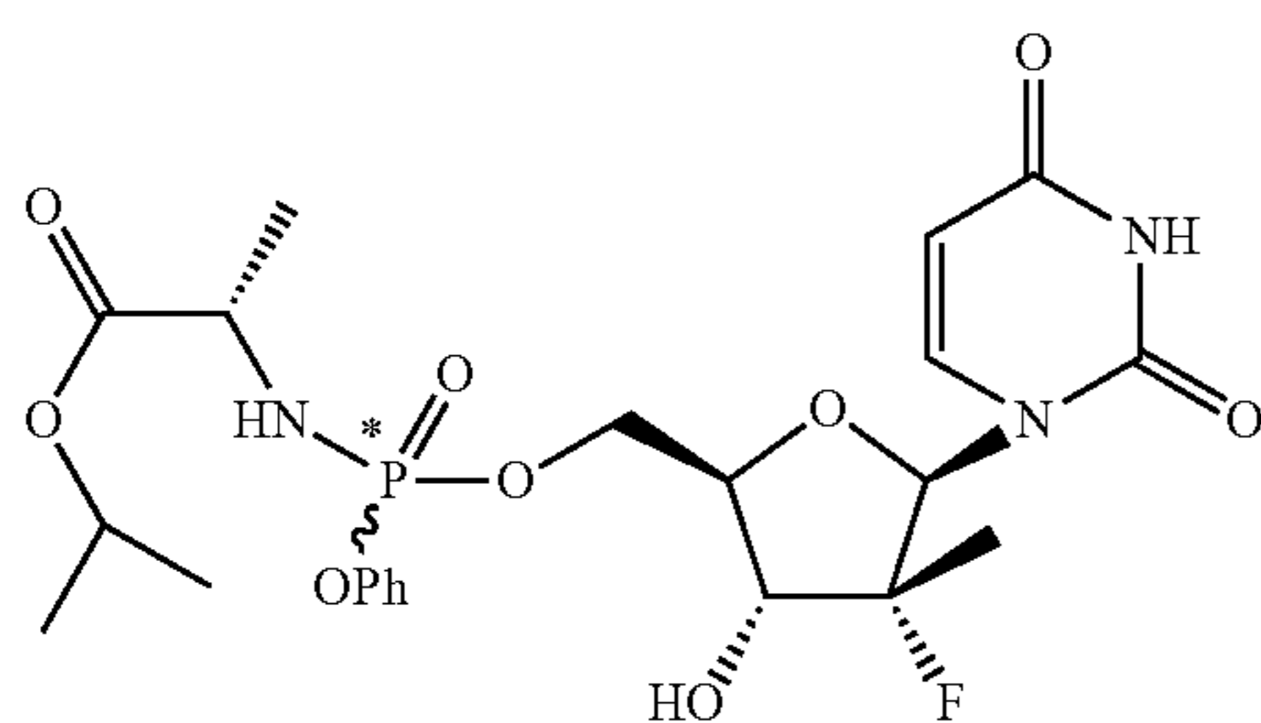
5'-O-phosphoramidate (2 diastereomers)
