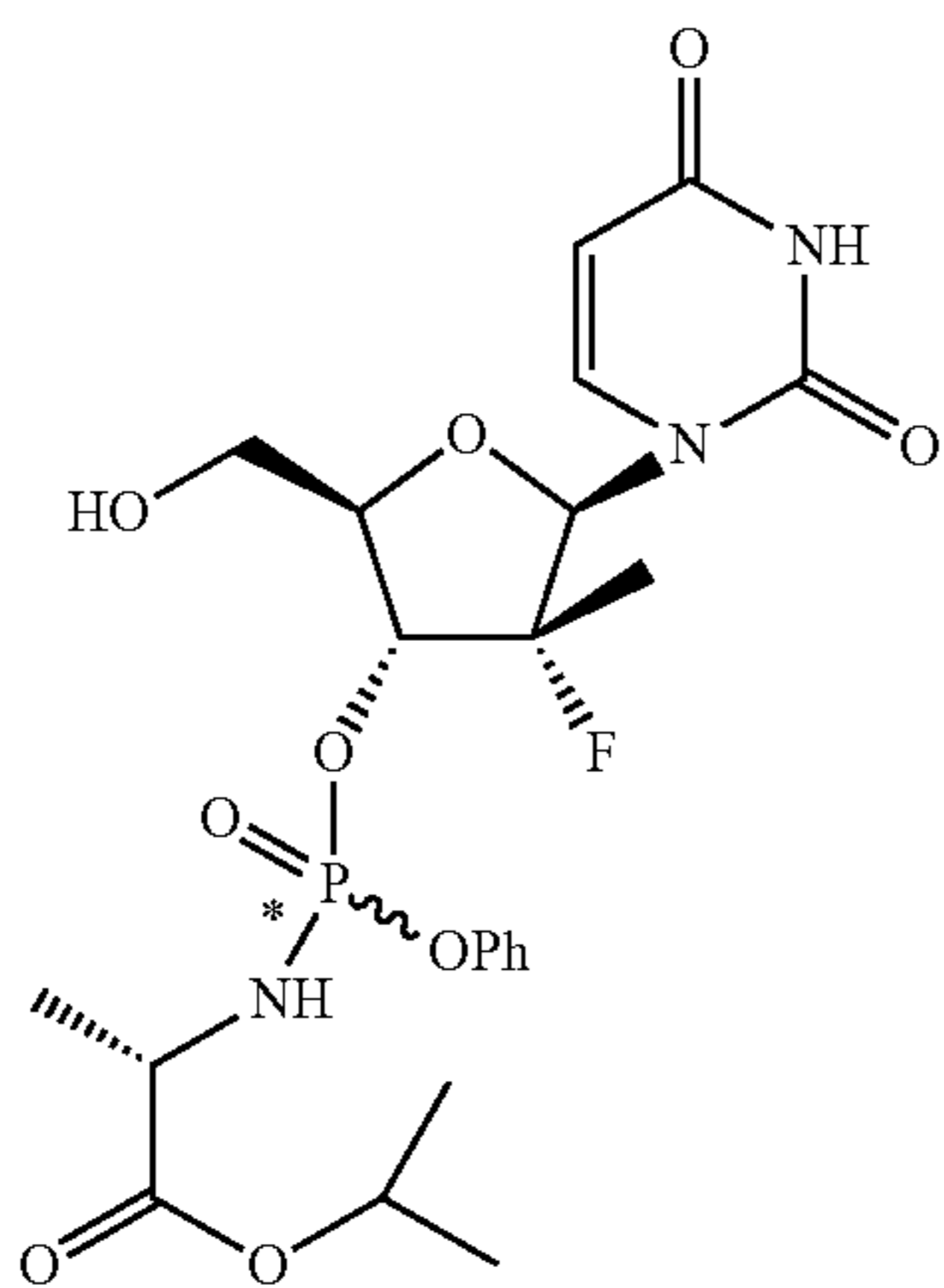
3'-O-phosphoramidate (2 diastereomers)
