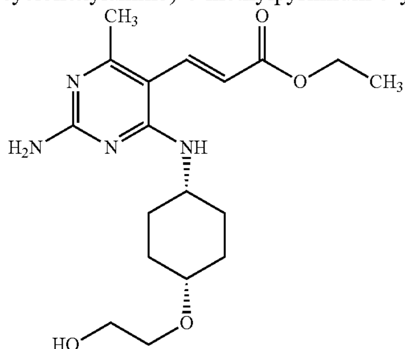
(E)-Ethyl 3-(2-amino-4-(cis-4-(2-hydroxyethoxy)cyclohexylamino)-6-methylpyrimidin-5-yl)acrylate
