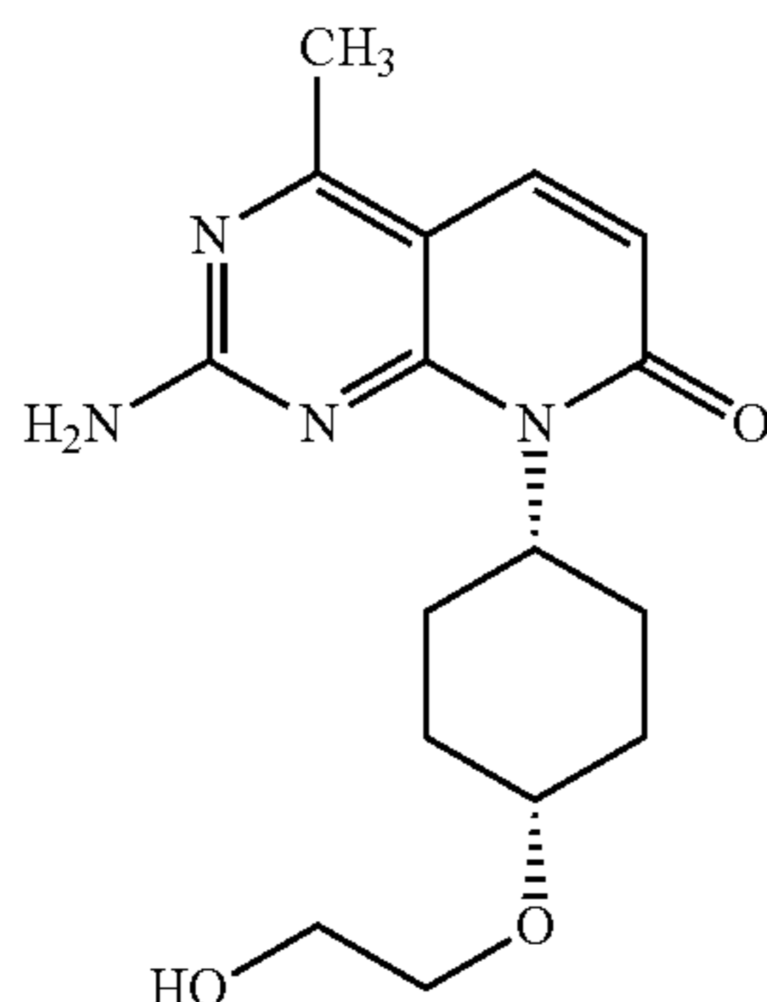
2-Amino-8-(cis-4-(2-hydroxyethoxy)cyclohexyl)-4-methylpyrido[2,3-d]pyrimidin-7(8H)-one
