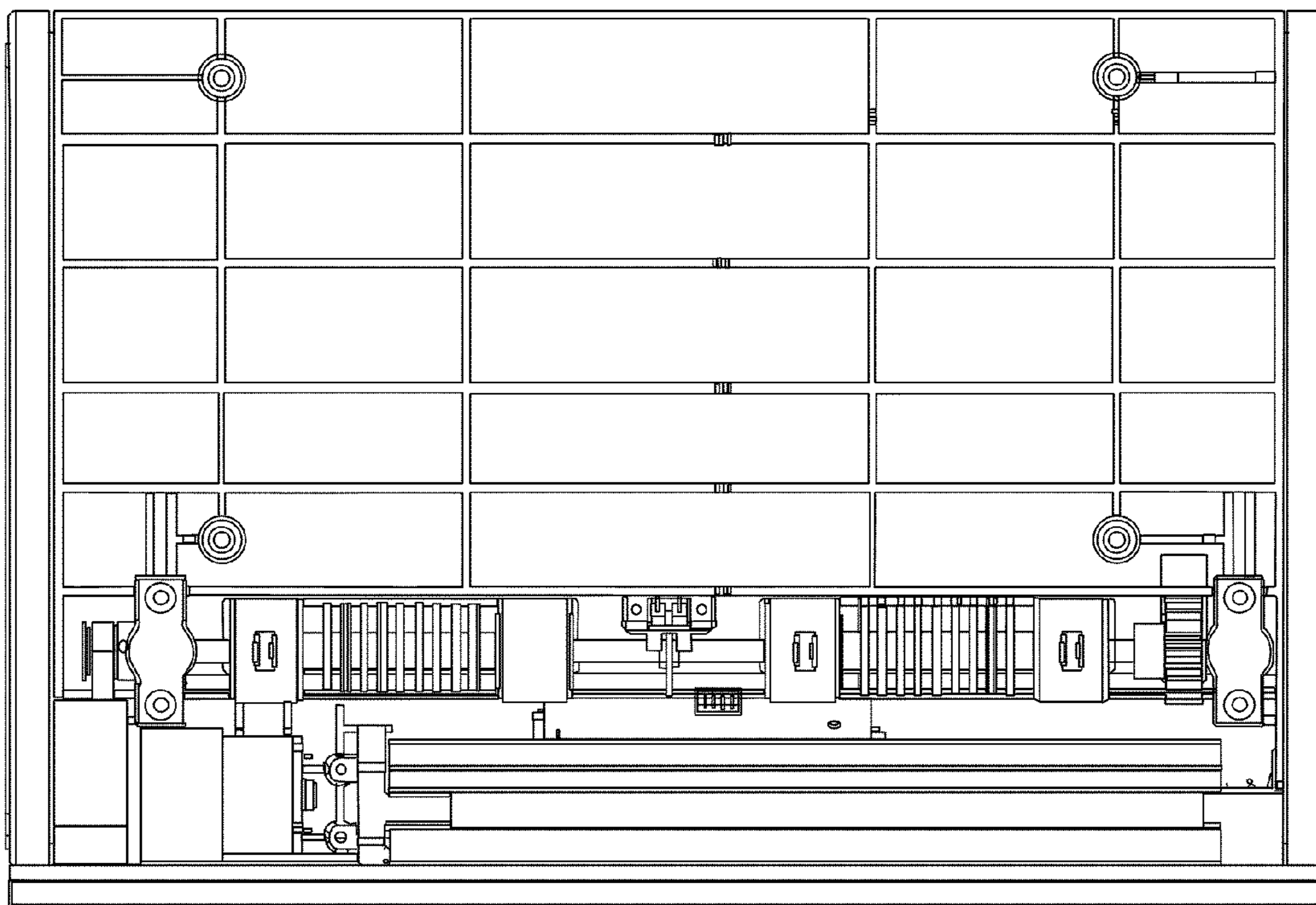
Top Plan View
