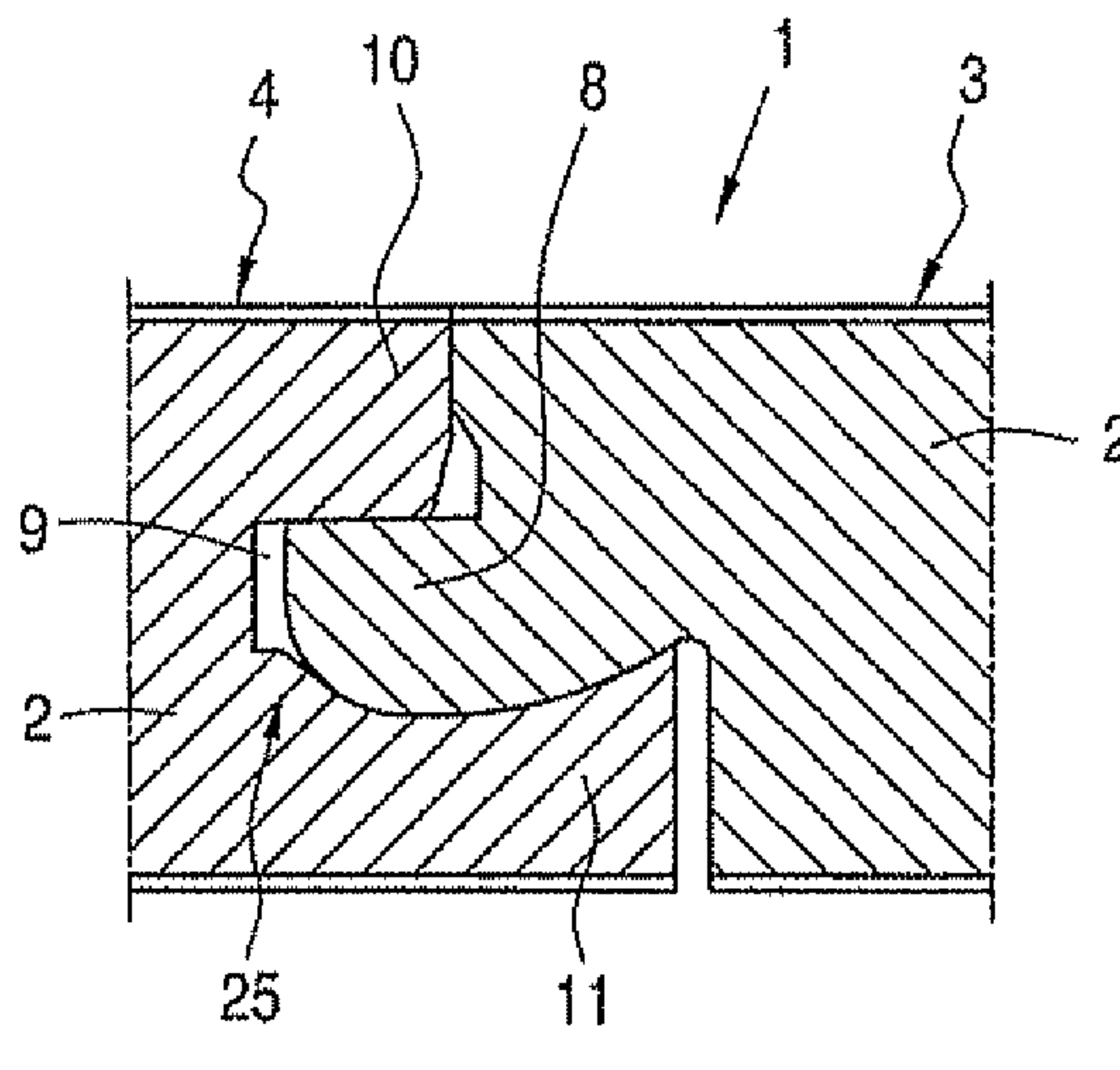
FIG. 5 PRIOR ART
