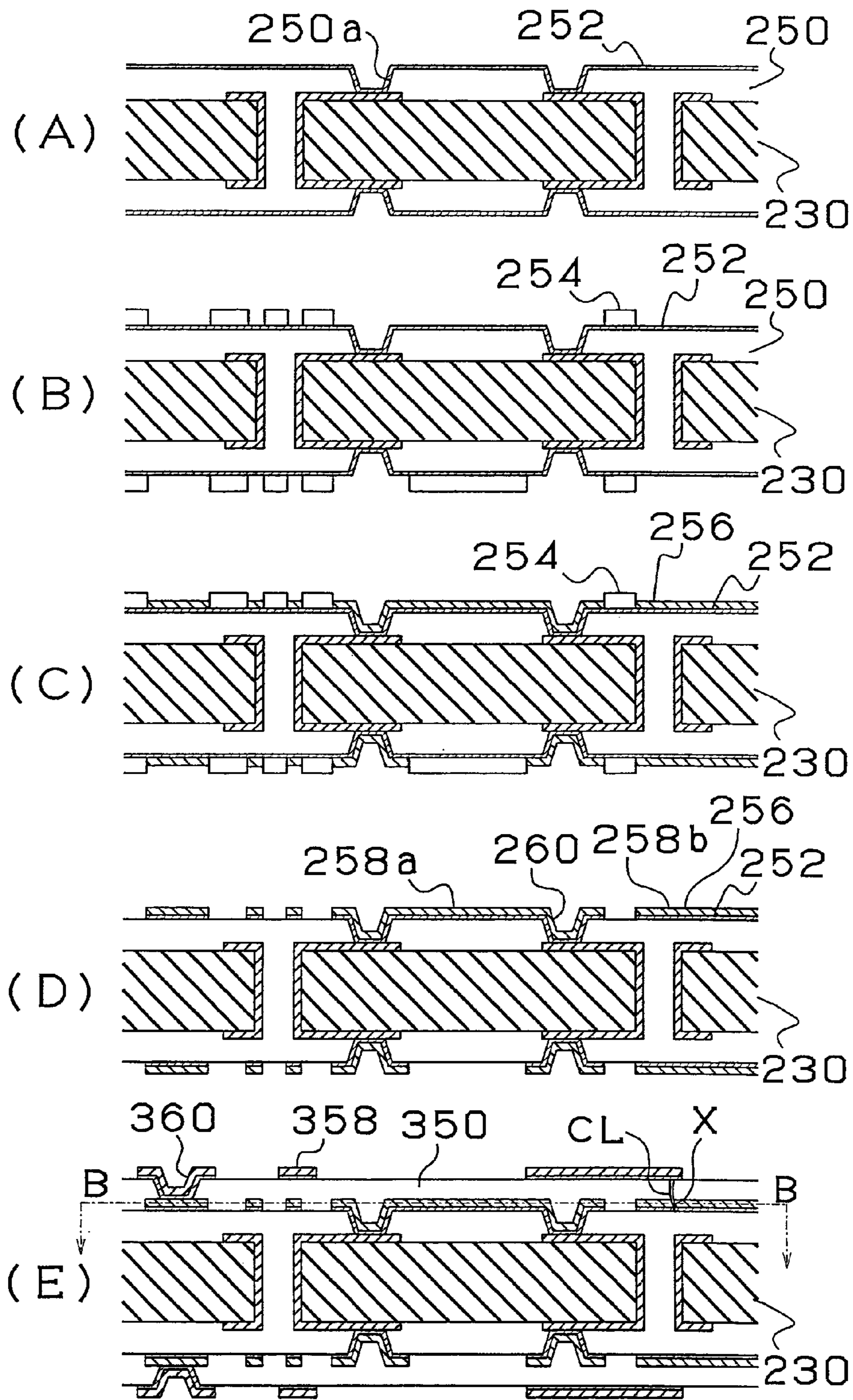
Fig. 32- PRIOR ART
