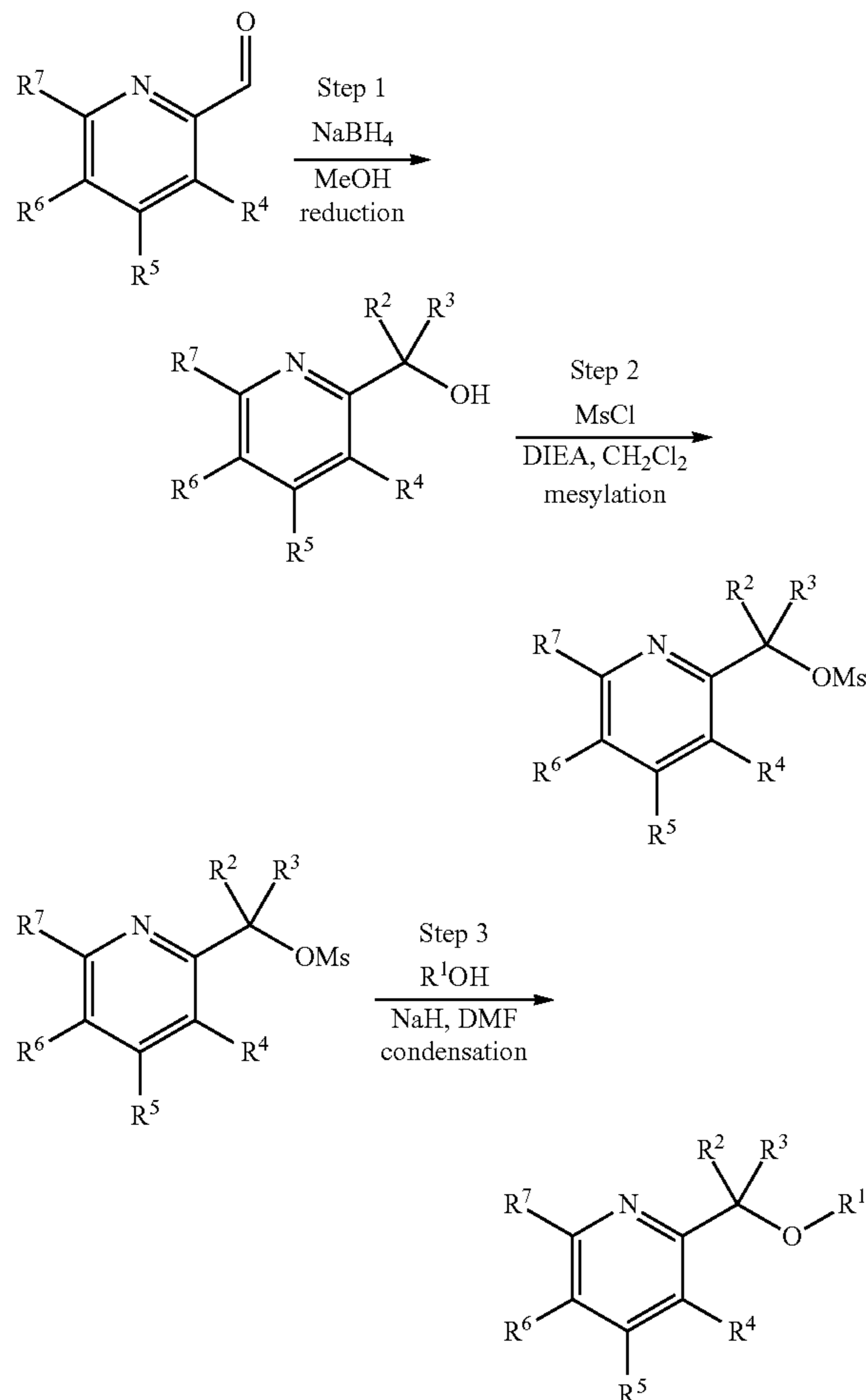
Scheme 1.
