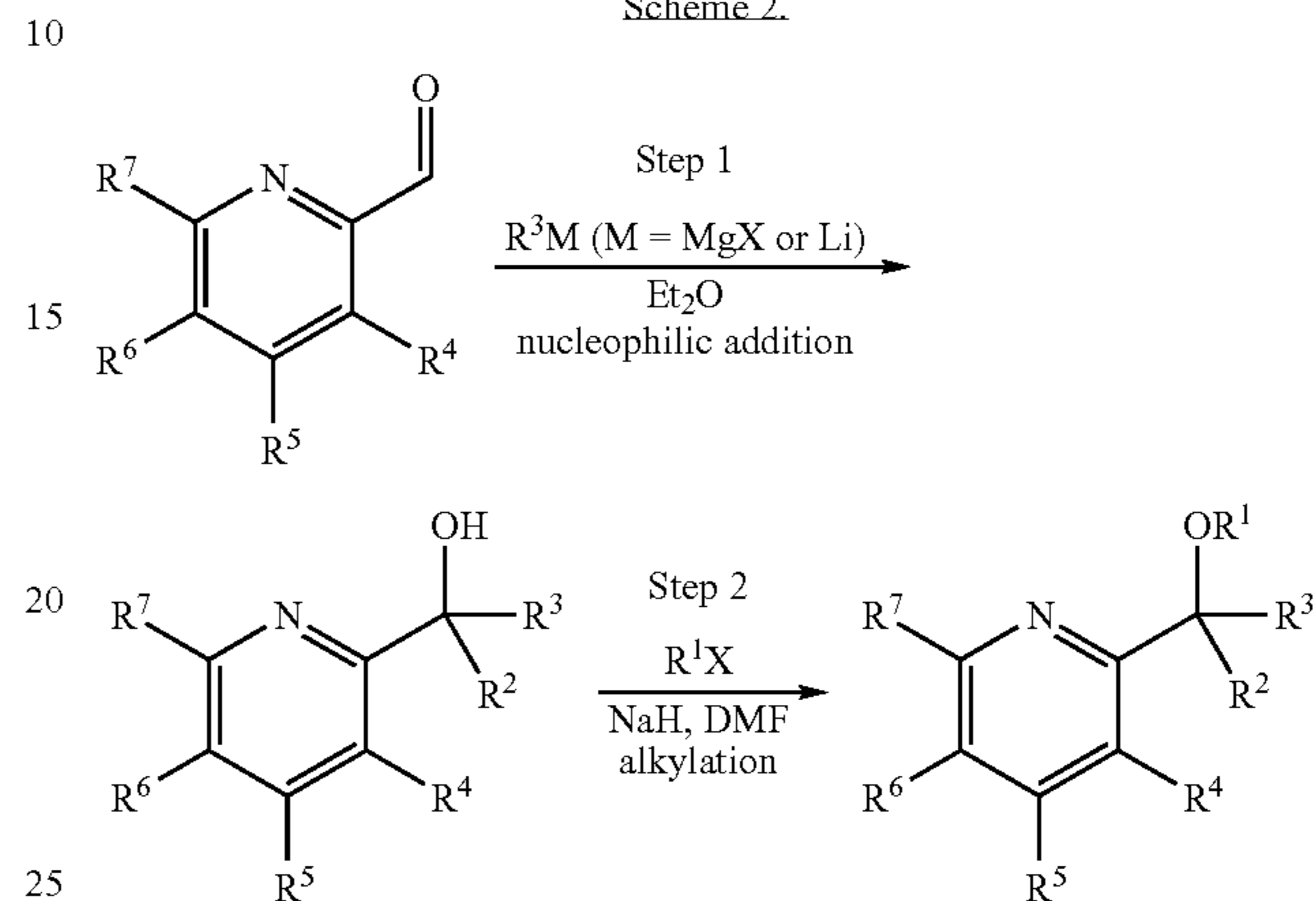
Scheme 2.
