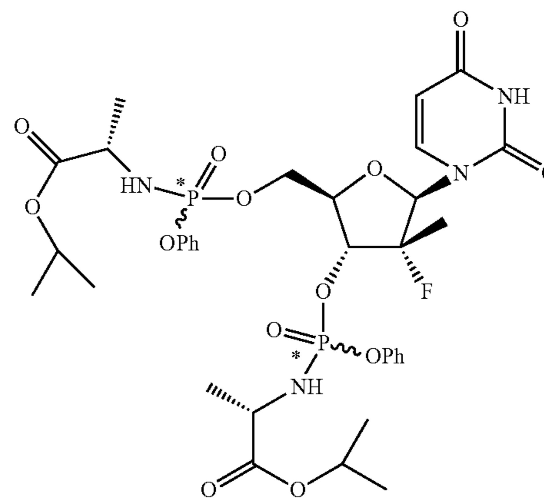
3',5'-bis-O-phosphoramidate (4 diastereomers)
