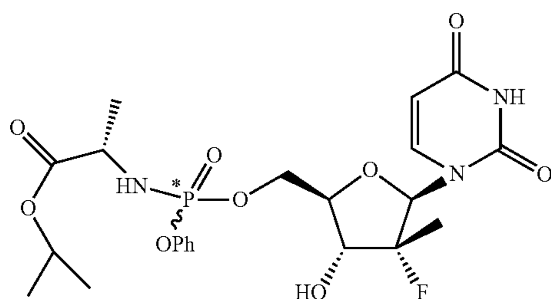
5'-O-phosphoramidate (2 diastereomers)
