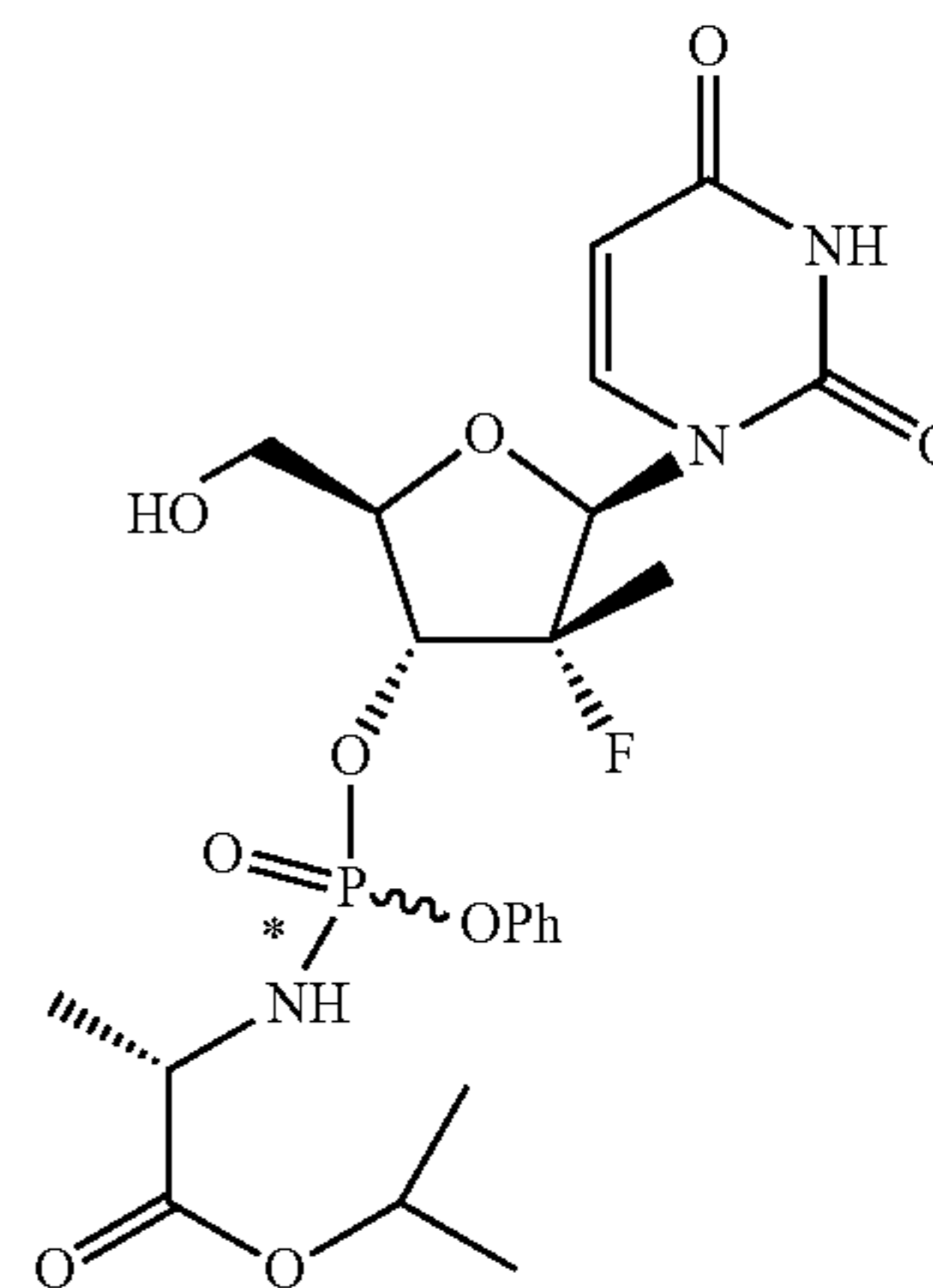
3'-O-phosphoramidate (2 diastereomers)
