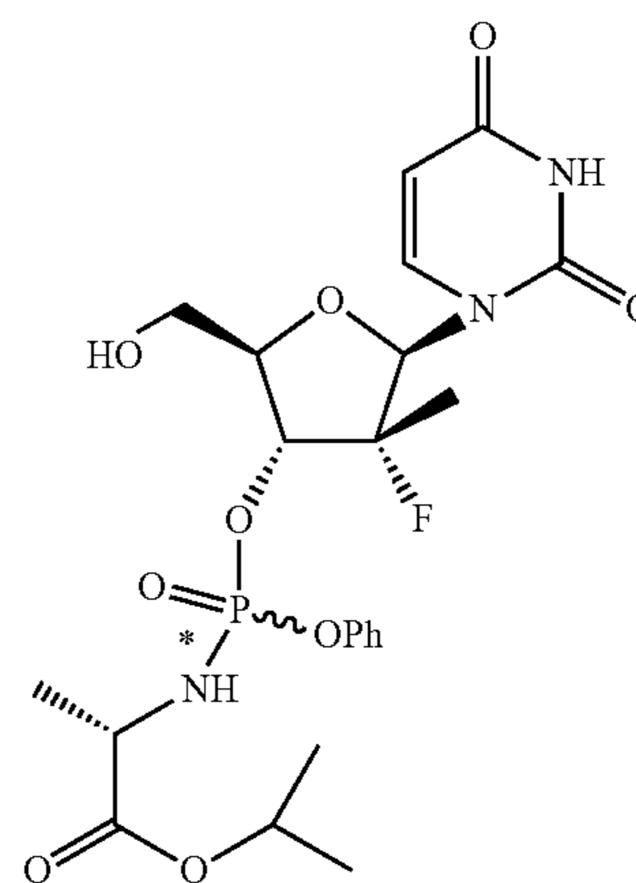
3'-O-phosphoramidate (2 diastereomers)
