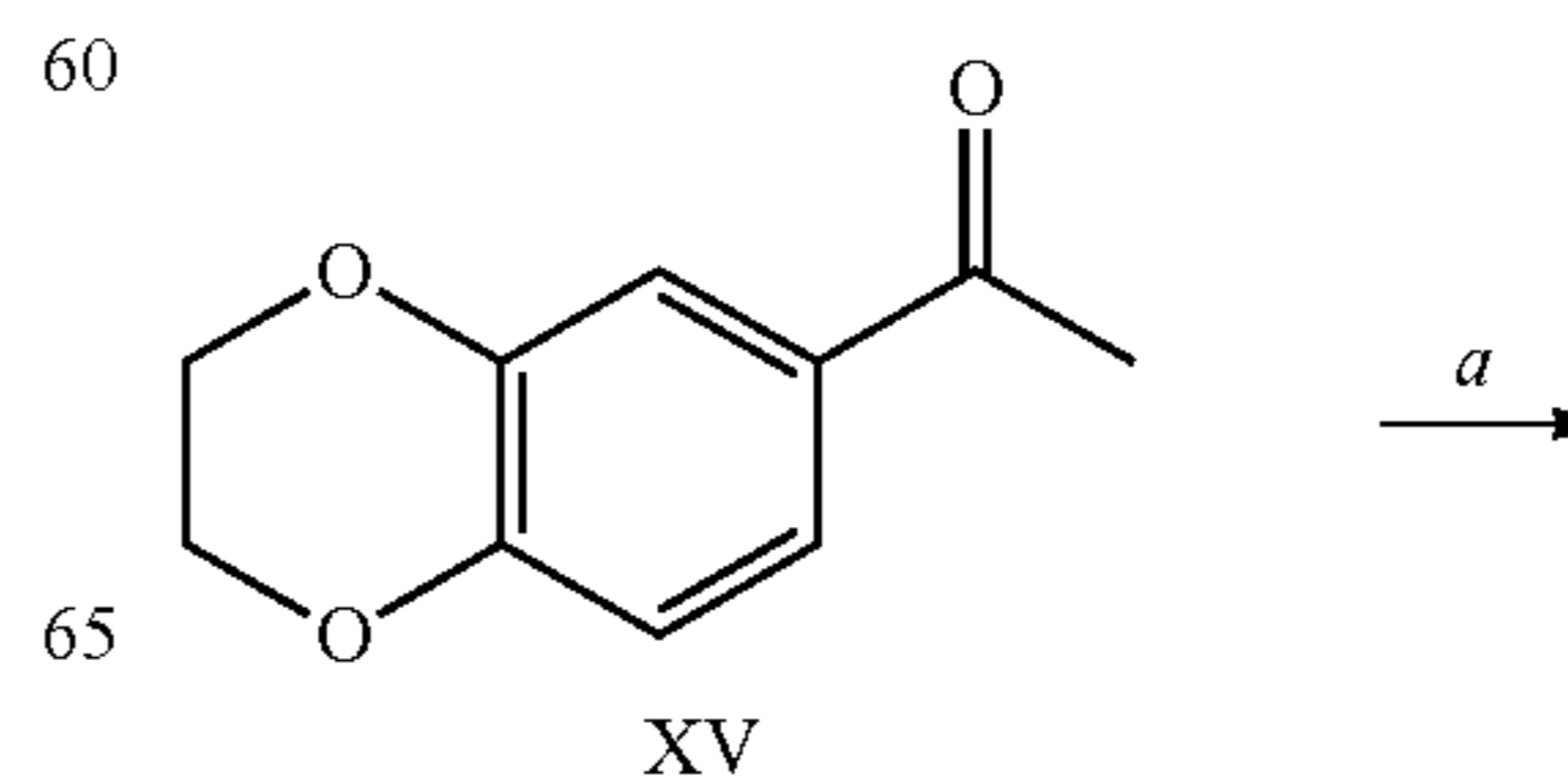
Scheme 5
