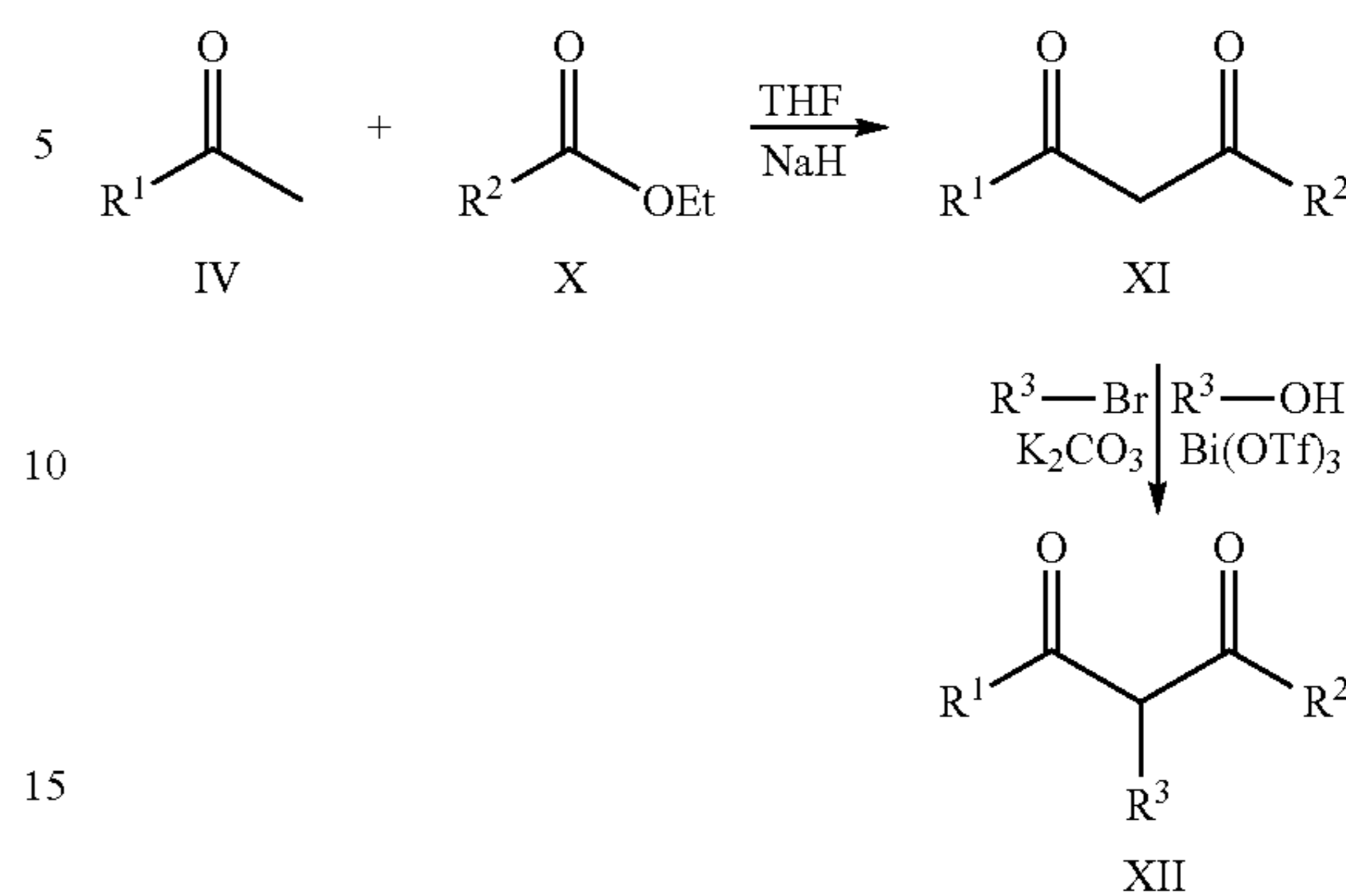
Scheme 3
