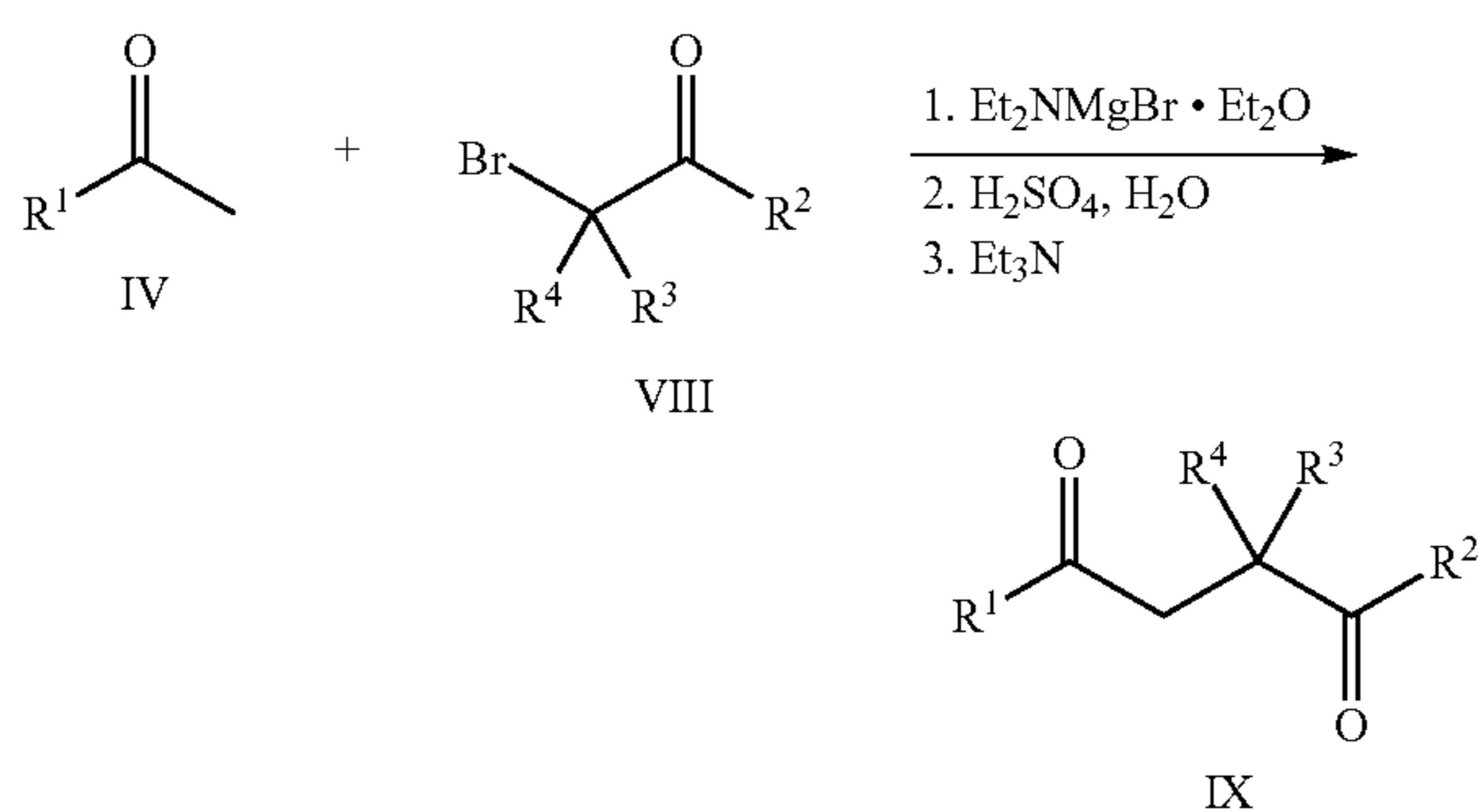
Scheme 2
