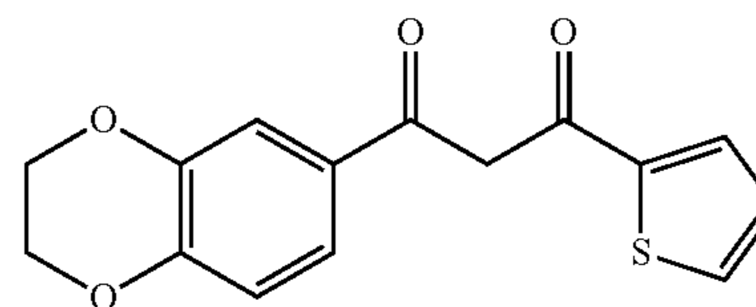
1-(2,3-dihydrobenzo[b][1,4]dioxin-6-yl)-3-(thiophen-2-yl)propane-1,3-dione 16
