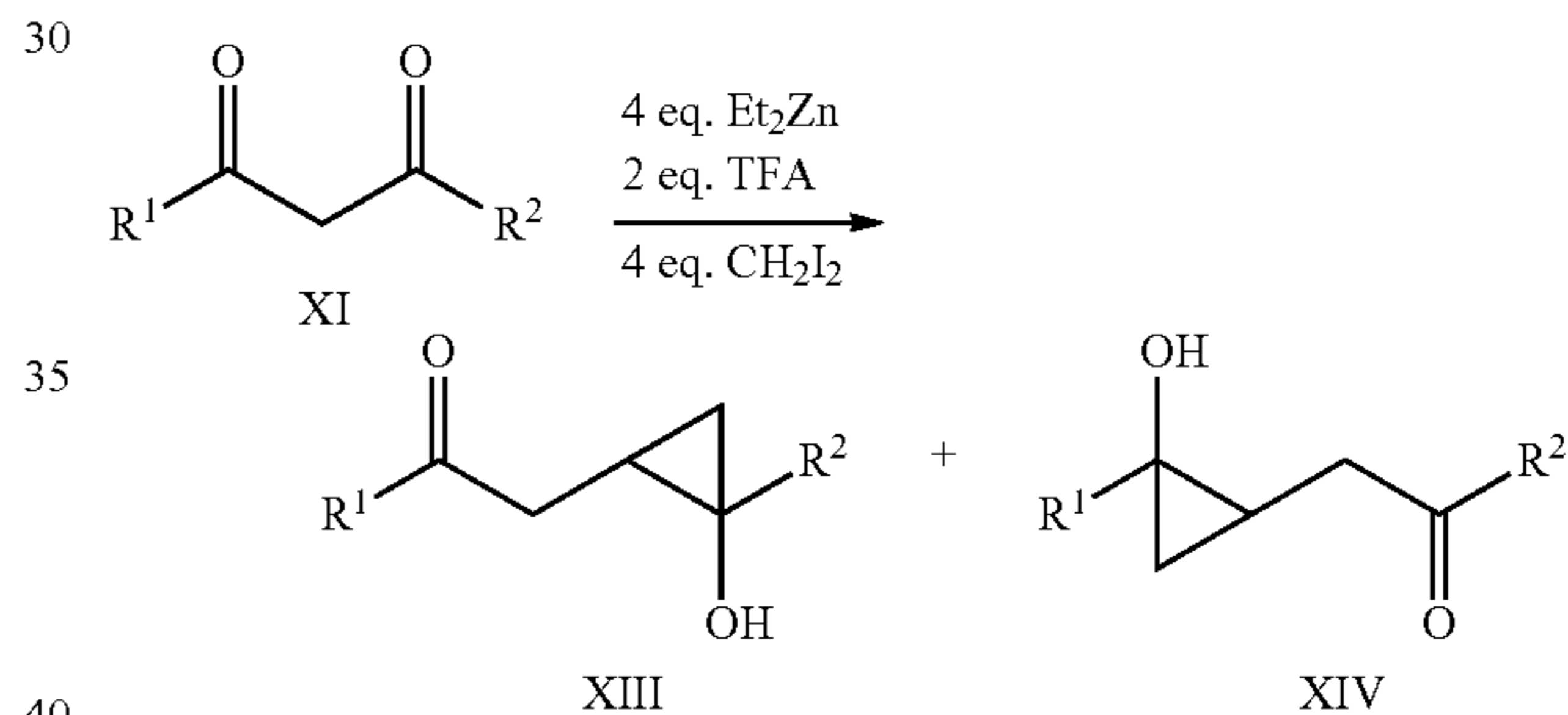
Scheme 4
