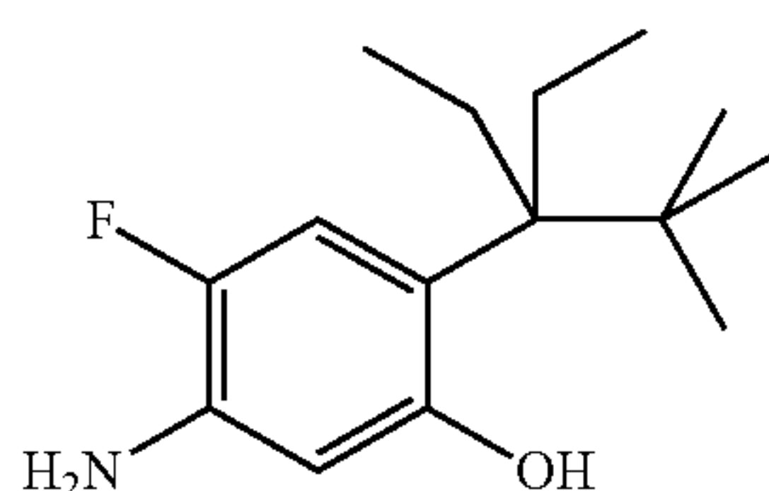
C-23; 5-Amino-2-(3-ethyl-2,2-dimethylpentan-3-yl)-4-fluoro-phenol
