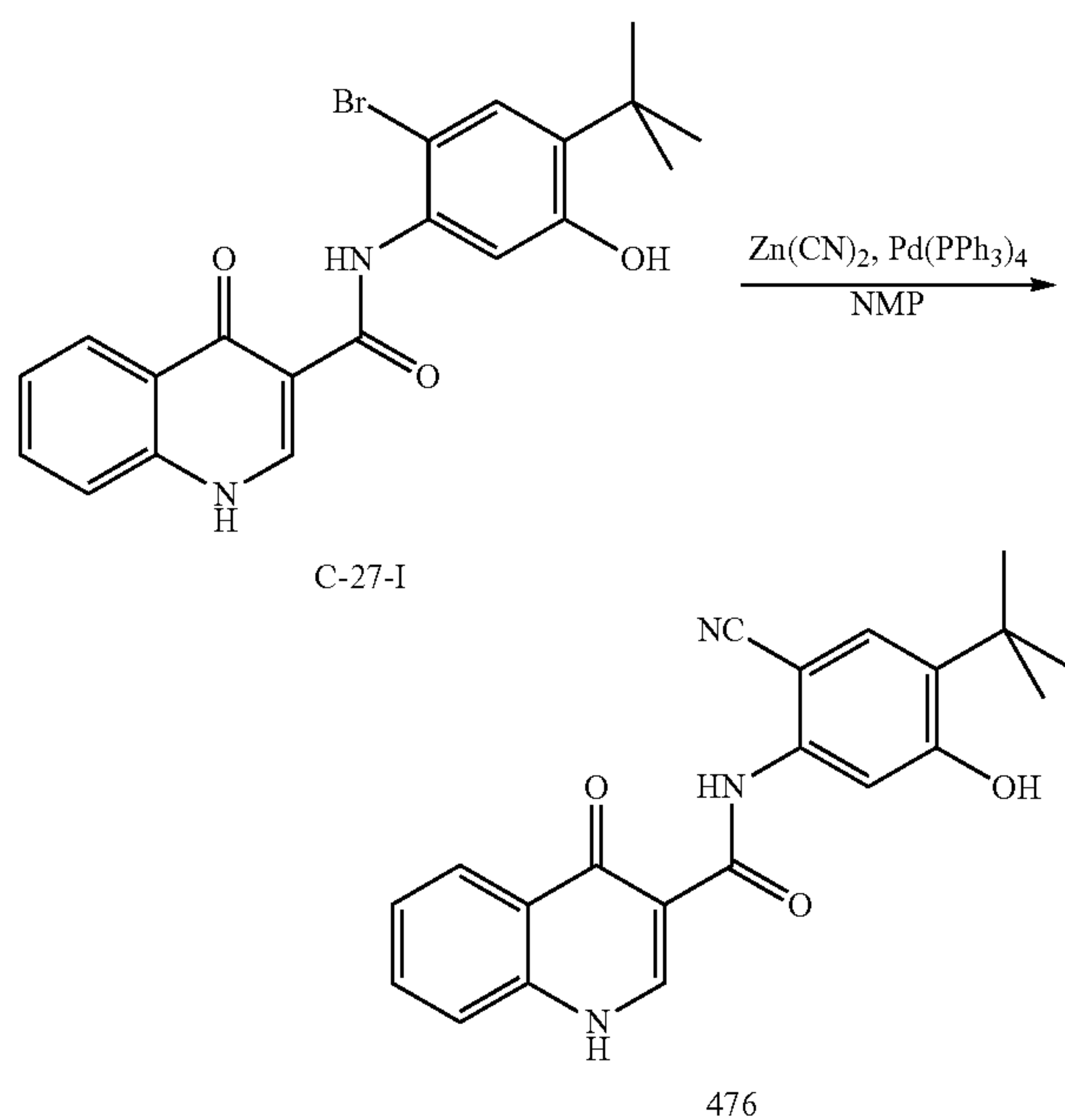
476; N-(4-tert-Butyl-2-cyano-5-hydroxyphenyl)-1,4-dihydro-4-oxoquinoline-3-carboxamide
