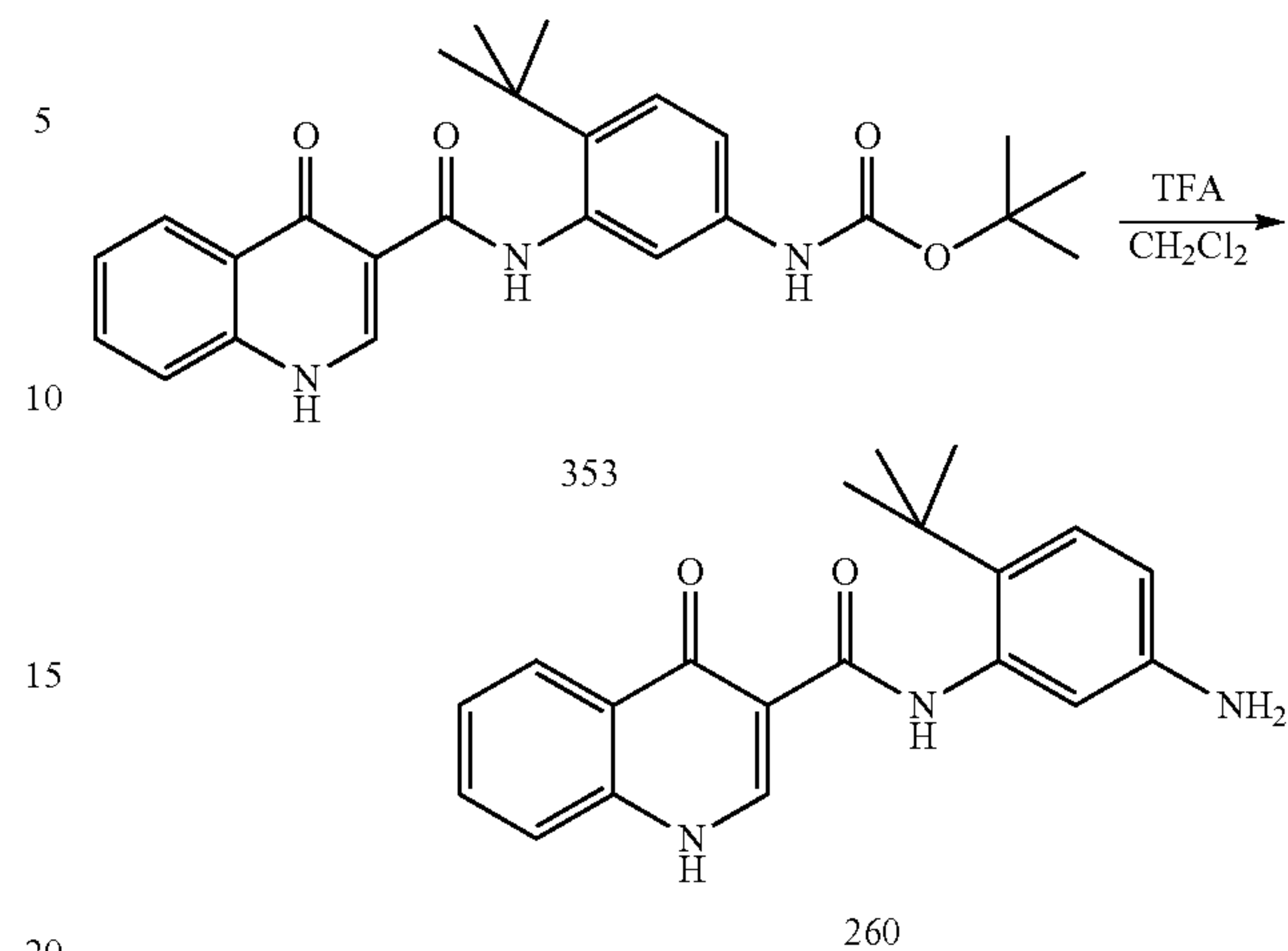
260; N-(5-Amino-2-tert-butyl-phenyl)-4-oxo-1H-quinoline-3-carboxamide
