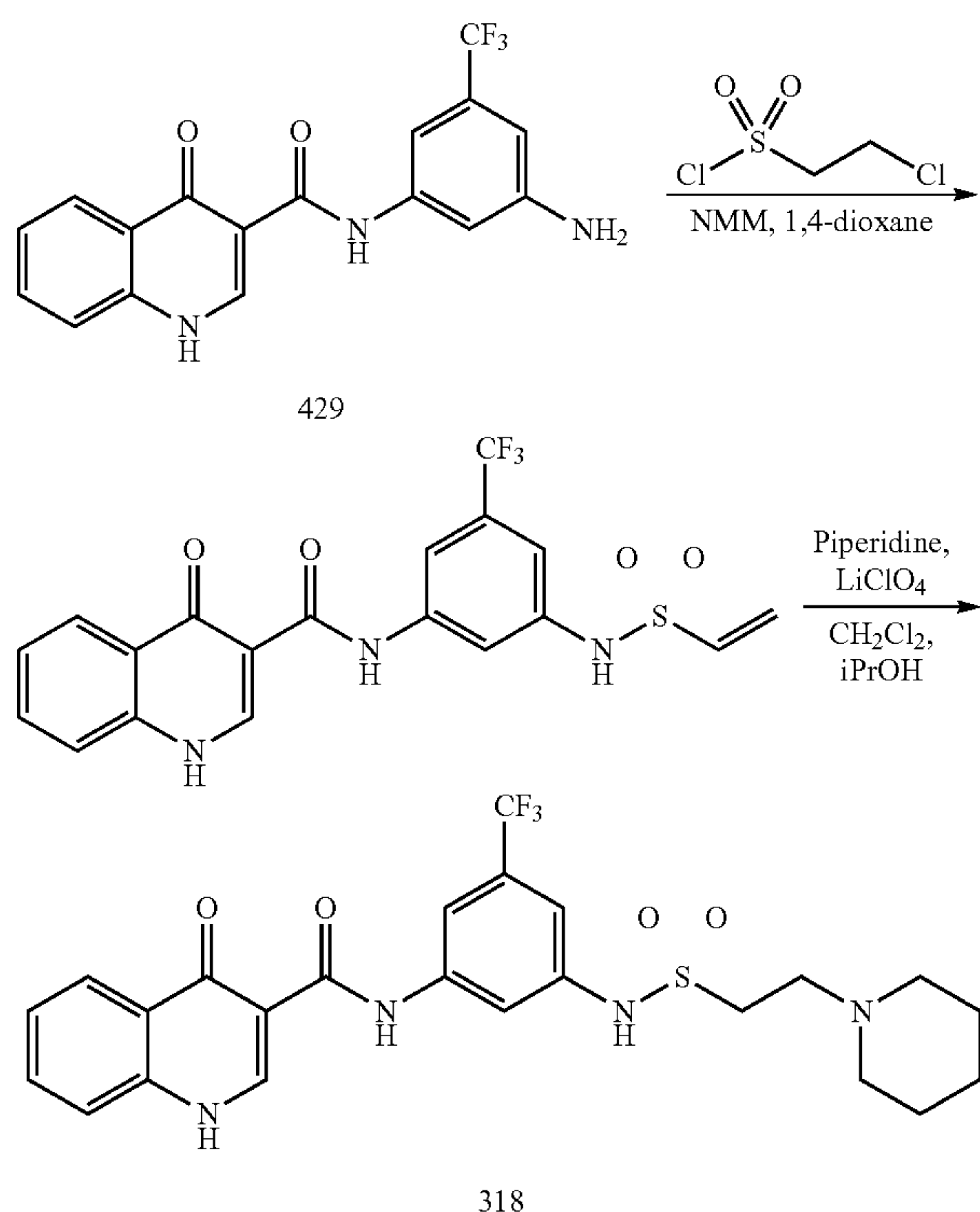
4-Oxo-N-[3-(trifluoromethyl)-5-(vinylsulfonylamino)phenyl]-1,4-dihydroquinoline-3-carboxamide
