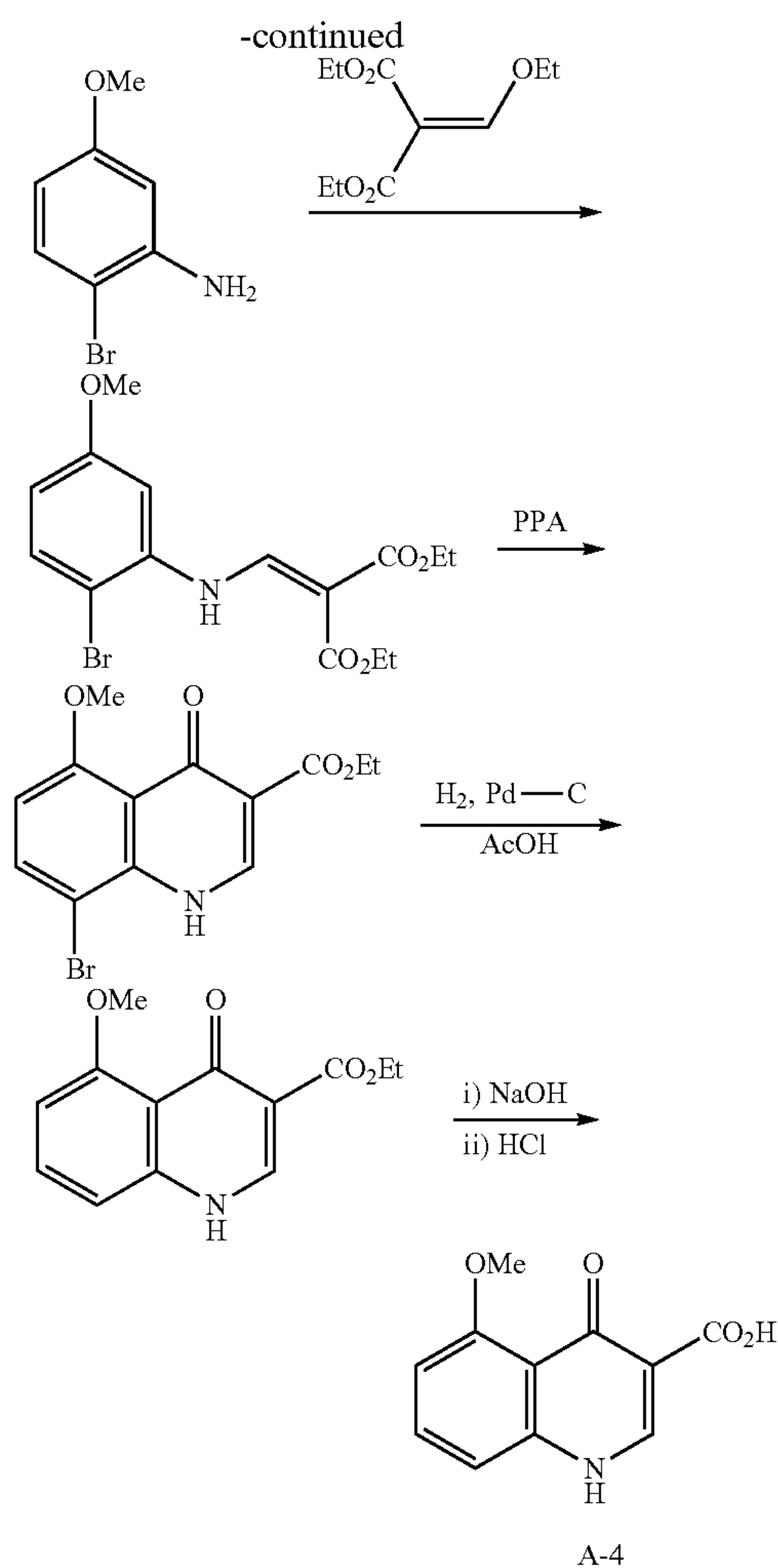
2-Bromo-5-methoxy-phenylamine
